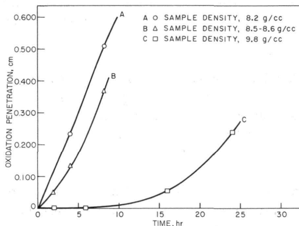
Figure 12. Oxidation Resistance of Reinforced Thoria
