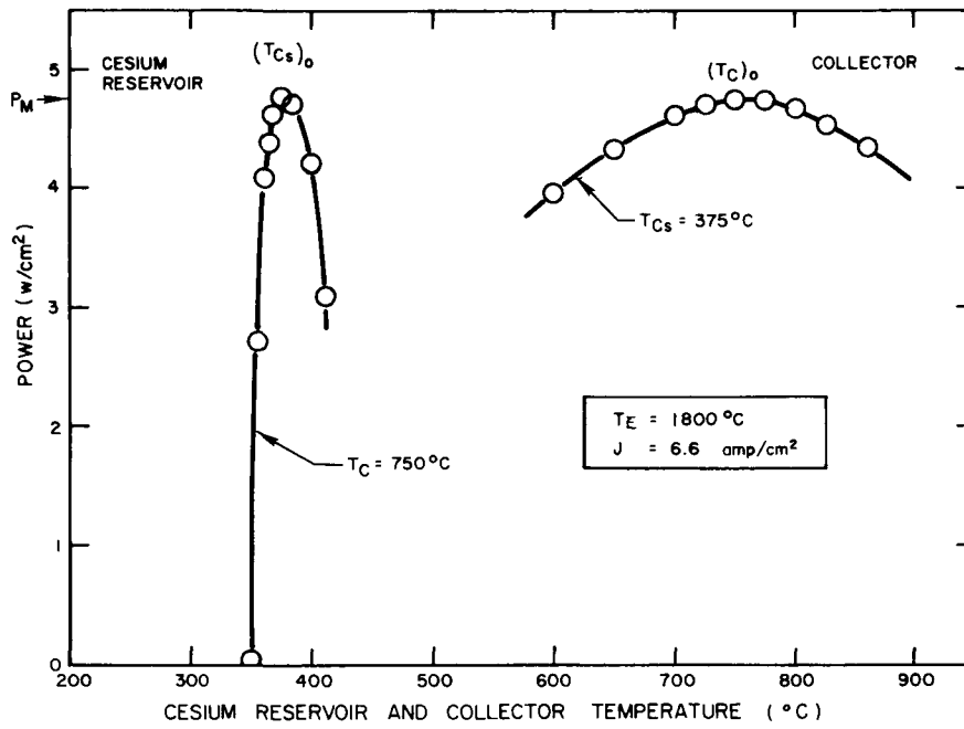
Figure 2. Optimization of Cesium Reservoir and Collector Temperature
