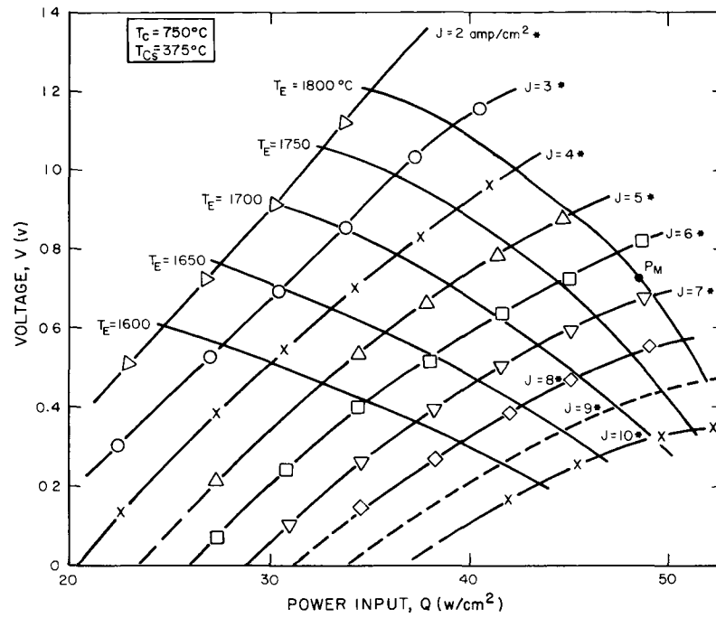
Figure 4. Voltage vs Power Input at T_C = 750^\circ C and T_{CS} = 375^\circ C
