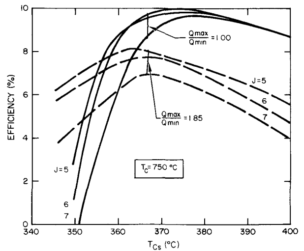
Figure 19. Efficiency of a Thermionic Reactor with 1000 Series-Connected Diodes
