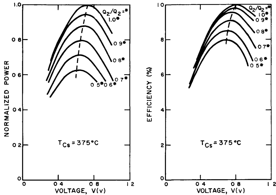
Figure 14. Normalized Power Output and Efficiency of Two Diodes in a Parallel Circuit with Power Inputs Q_1 and Q_2 ( Q_1 is the power input of T_E = 1800^\circ\text{C} )
