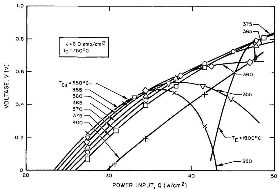
Figure 6. Voltage vs Power Input at J = 6 \text{ amp}/cm^2 and T_C = 750^\circ C
