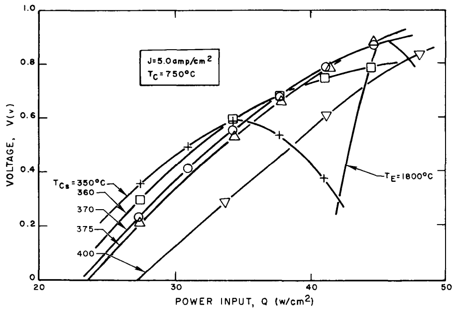
Figure 5. Voltage vs Power Input at J = 5 amp/cm^2 and T_C = 750^\circ C
