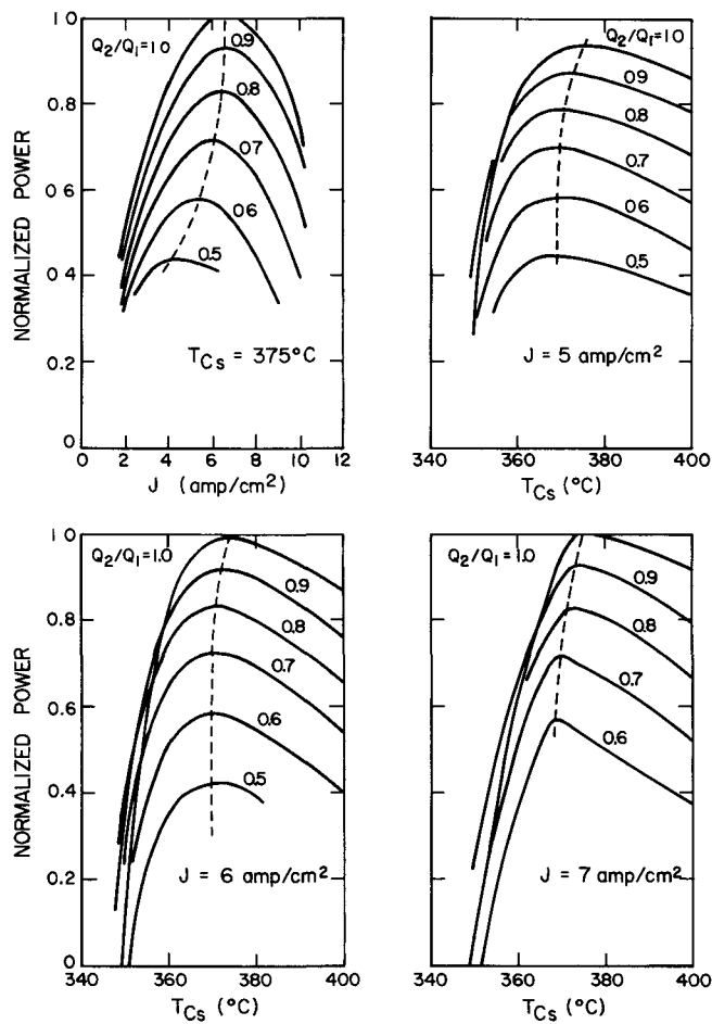
Figure 12. Normalized Power Output of Two Diodes in a Series Circuit With Power Inputs Q_1 and Q_2 ( Q_1 is the power at T_E = 1800^\circ\text{C} )
