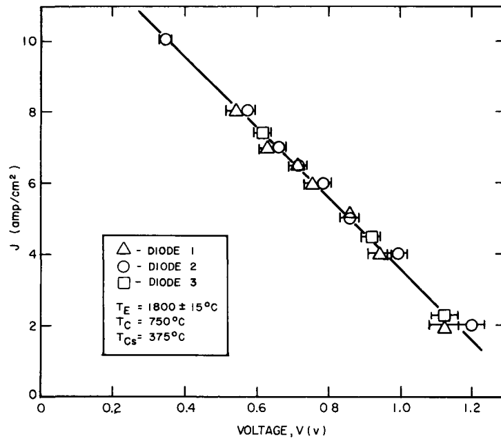
Figure 9. Comparison of the Individual Performances of the Three Diodes at T_E = 1800 \pm 15^\circ\text{C}
