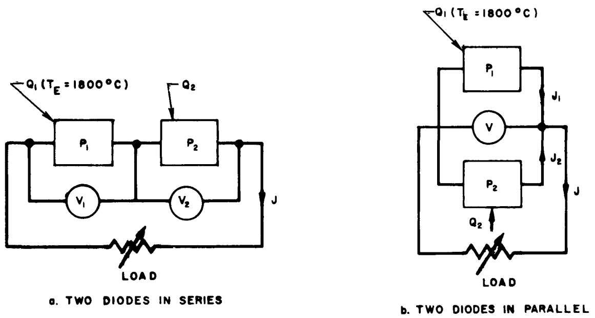
Figure 11. Circuit Diagrams
