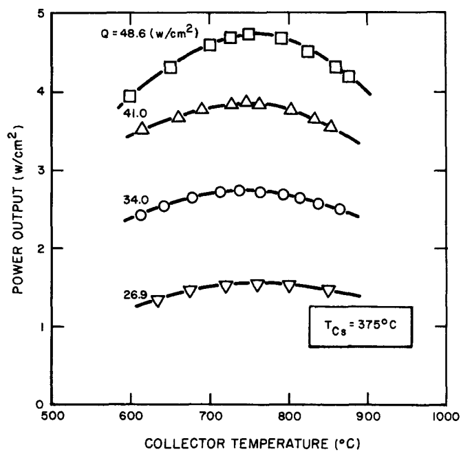
Figure 8. Effect of Collector Temperature on Power Output at T_{Cs} = 375^{\circ}\text{C}
