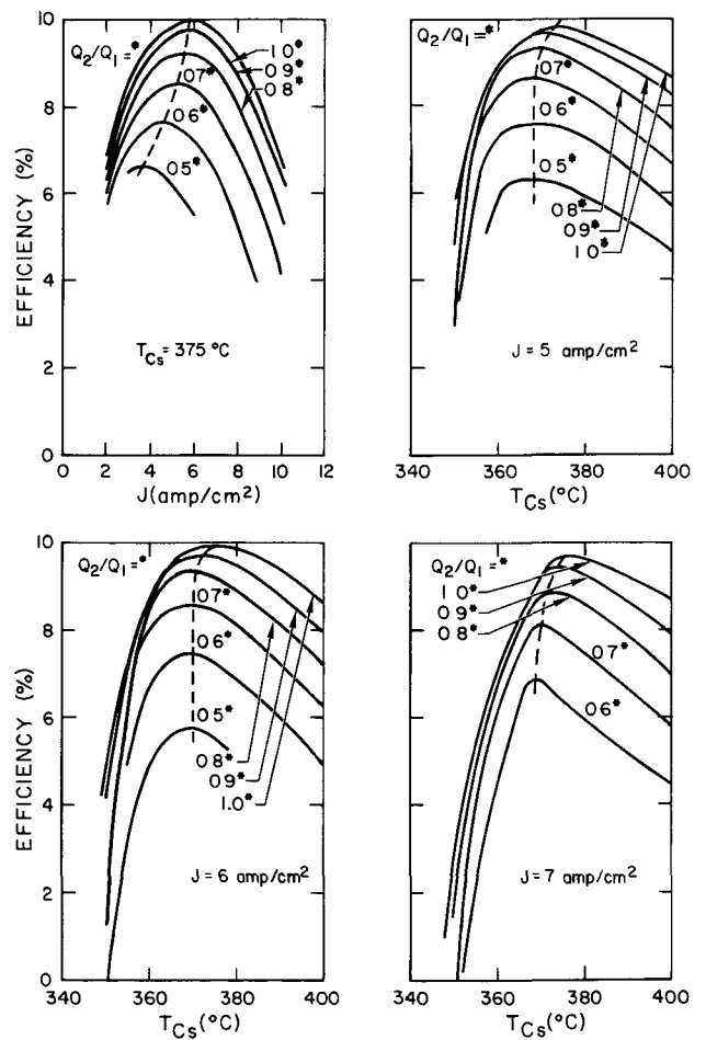
Figure 13. Efficiency of Two Diodes in a Series Circuit With Power Inputs Q_1 and Q_2 ( Q_1 is the power input at T_E = 1800^\circ\text{C} )
