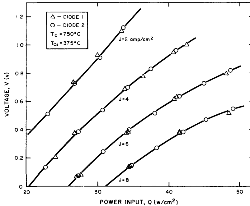
Figure 10. Comparison of Diodes 1 and 2 at T_{CS} = 375^\circ\text{C} and T_C = 750^\circ\text{C} (These two diodes are tested in series and parallel circuits)
