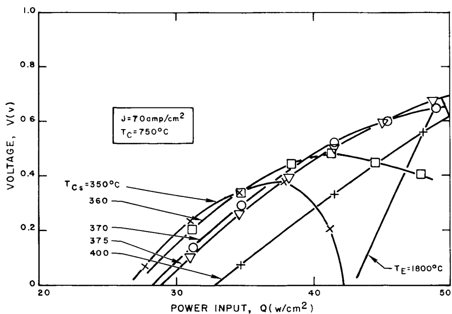
Figure 7. Voltage vs Power Input at J = 7 \text{ amp}/cm^2 and T_C = 750^\circ C
