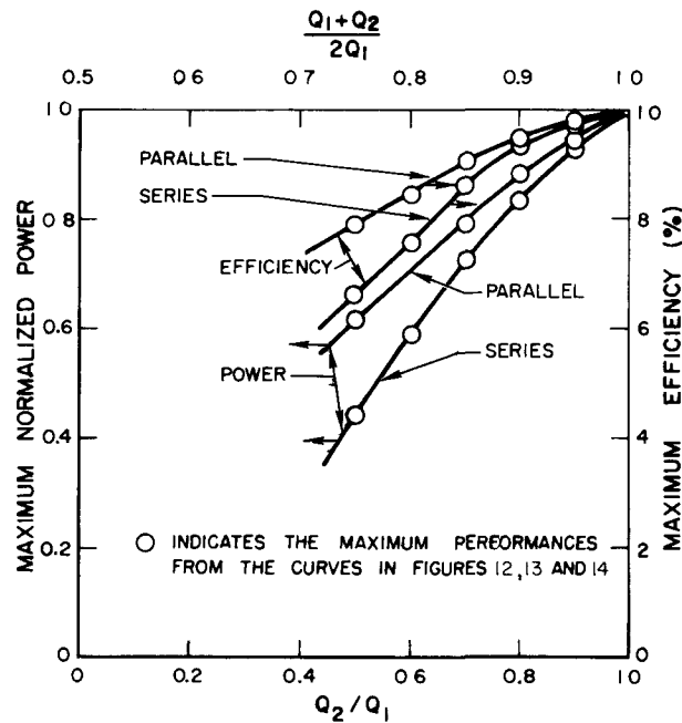
Figure 15. Maximized Power and Efficiency of Two Diodes in Series and Parallel Circuits vs Q_2/Q_1
