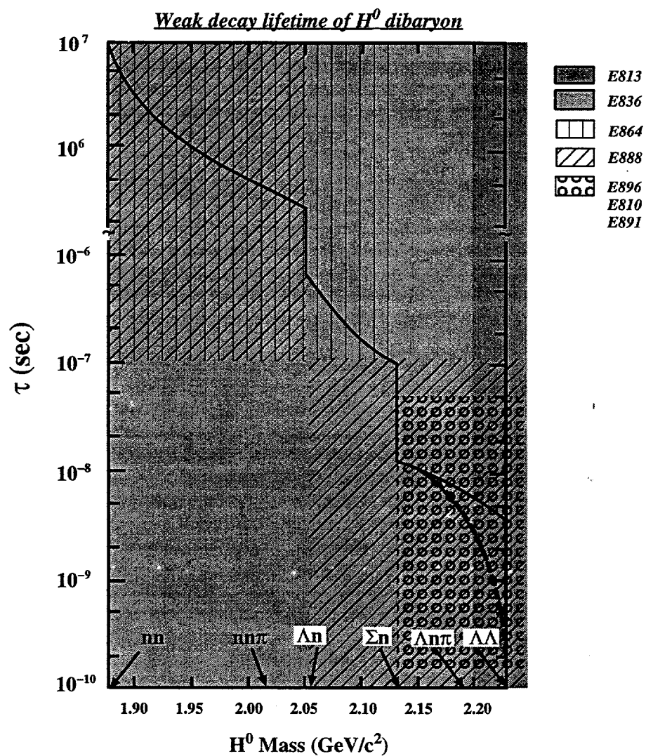
Figure 1: Regions of sensitivity of several AGS experimental searches for the H particle compiled by Philip Pile. The curve is the relationship between \tau_H and m_H according to the calculation of Donoghue et al.
