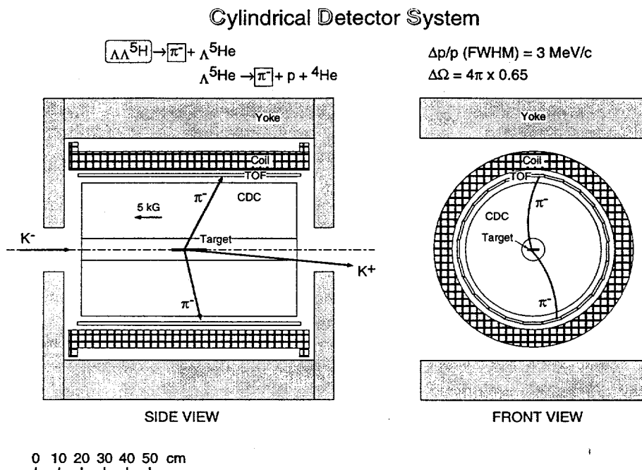
Figure 5: Cylindrical Detector System used in AGS 906
