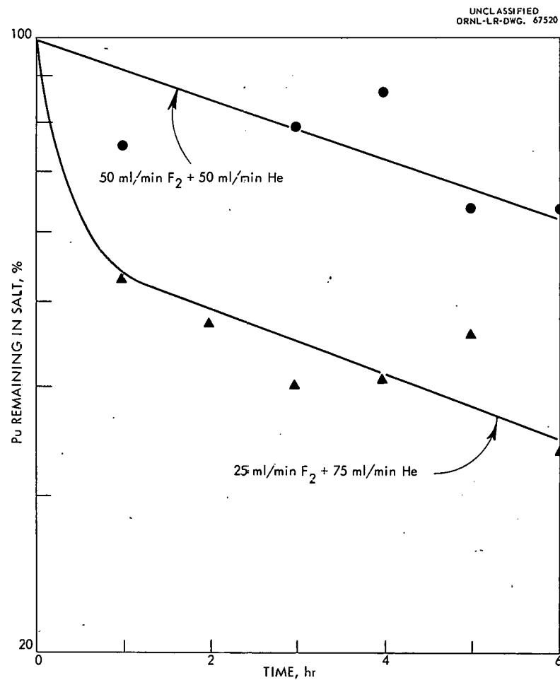
Fig. 4. Effect of dilution of fluorine with helium in volatilization of PuF 5 from 31-24-45 mole % LiF-NaF-ZrF 4 salt at 600°C.
