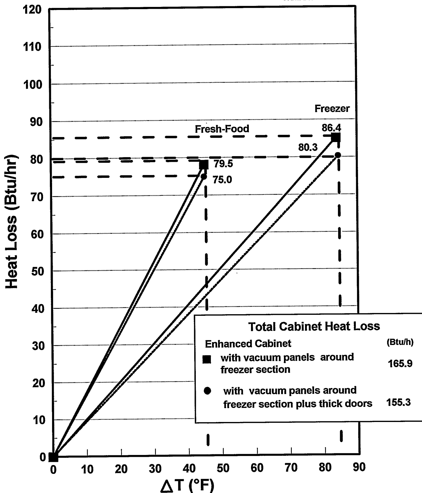
Fig. 3. Reverse heat loss results for enhanced cabinet
