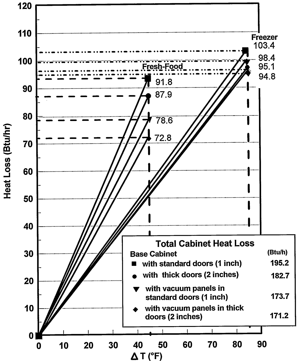
Fig. 2. Reverse heat loss results for base cabinet
