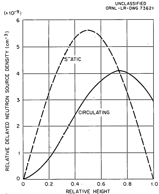
Fig. 2.15. Effect of Fuel Circulation on Axial Distribution of Source Density of Group 4 Delayed Neutrons. Fuel circulating at 1200 gpm.
