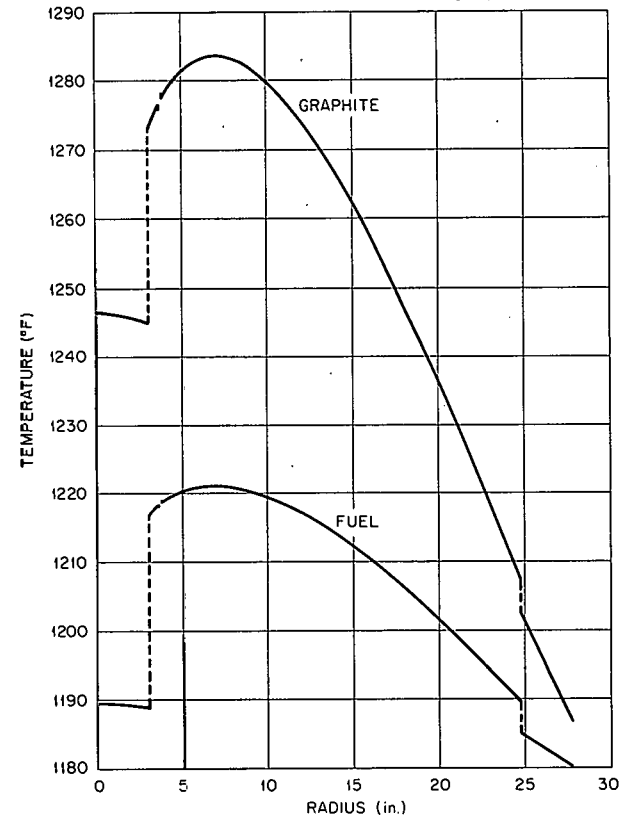
Fig. 2.10. Radial Temperature Profiles in MSRE Core Near Midplane.
