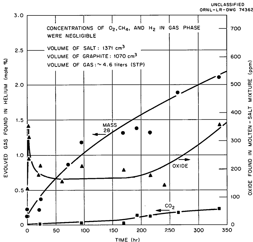
Fig. 6.7. Removal of Adsorbed Gas from AGOT Graphite Immersed in LiF-BeF 2 (66-34 mole %) at 600°C.
