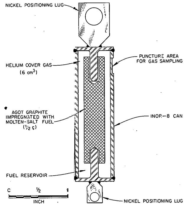
Fig. 5.5. Impregnated-Graphite-Molten-Salt Capsule.
