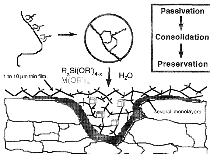
Figure 1. Schematic diagram of treatment for weathered limestone surface on a sculpted "nose". The gray area is the passivant that couples the limestone to the \text{SiO}_2 -based consolidant above it. The \text{R}_x and M groups shown in the schematic can be tailored to increase the consolidant's hydrophobicity and strength respectively.
