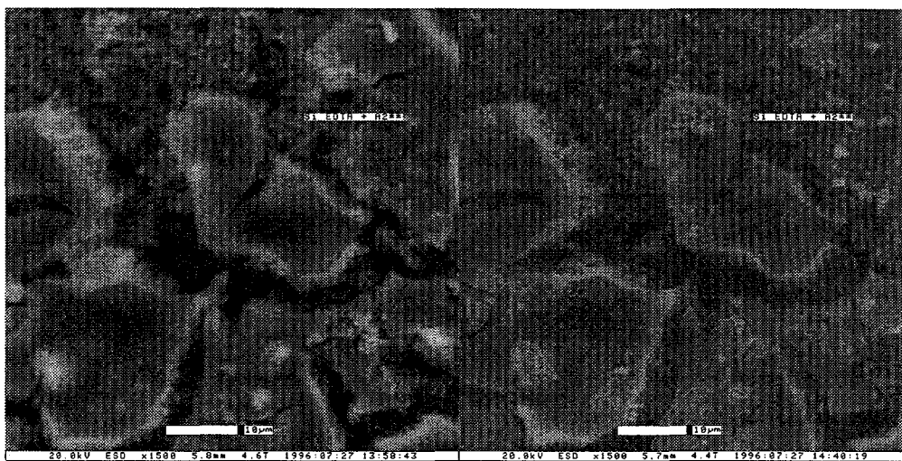
Figure 6a & b. Treated limestone before addition of concentrated sulfuric acid (Figure 6a). Inadequate coupling by the SAAC passivant led to shrinkage of the consolidant. Micron bar=10 µm. Figure 6b shows the same region after addition of acid. The consolidated areas remain unaffected although the layer is cracked. Better coupling passivants and thinner consolidating layers can prevent the cracking.
