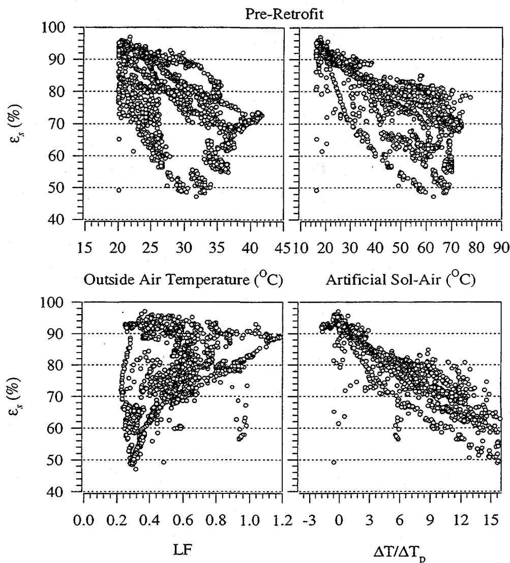
FIGURE 5. Return effectiveness ( \epsilon_s ) vs. outside air temperature, sol-air temperature, load factor and a scaling parameter \Delta T/\Delta T_p
