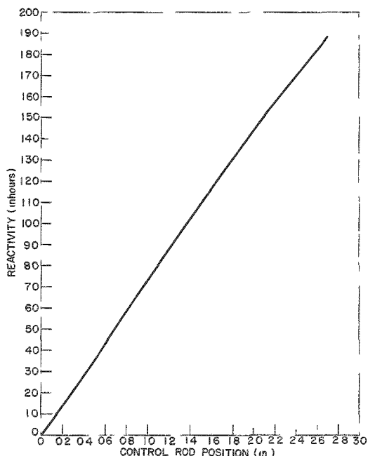
Fig. 13. Calibration of Control Rod No. 10
