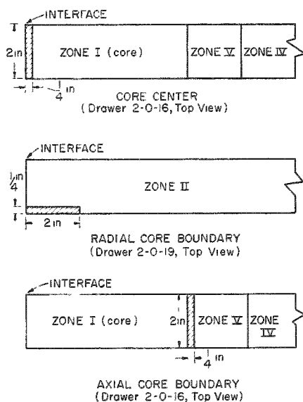
Fig. 14. Fissile Sample Locations for Reactivity Coefficient Measurements
