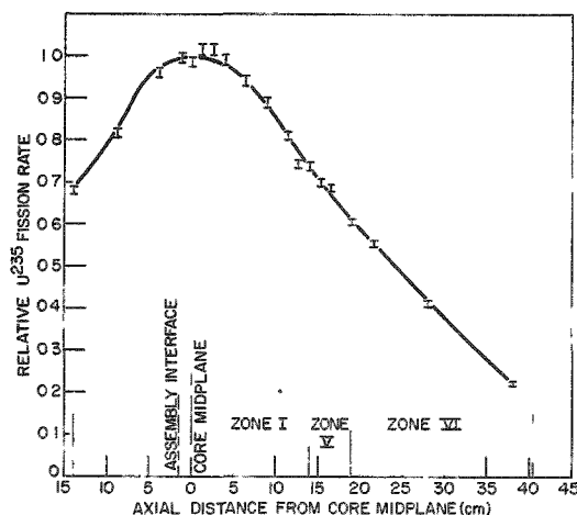
Fig. 20. U^{235} Axial Fission Traverse
