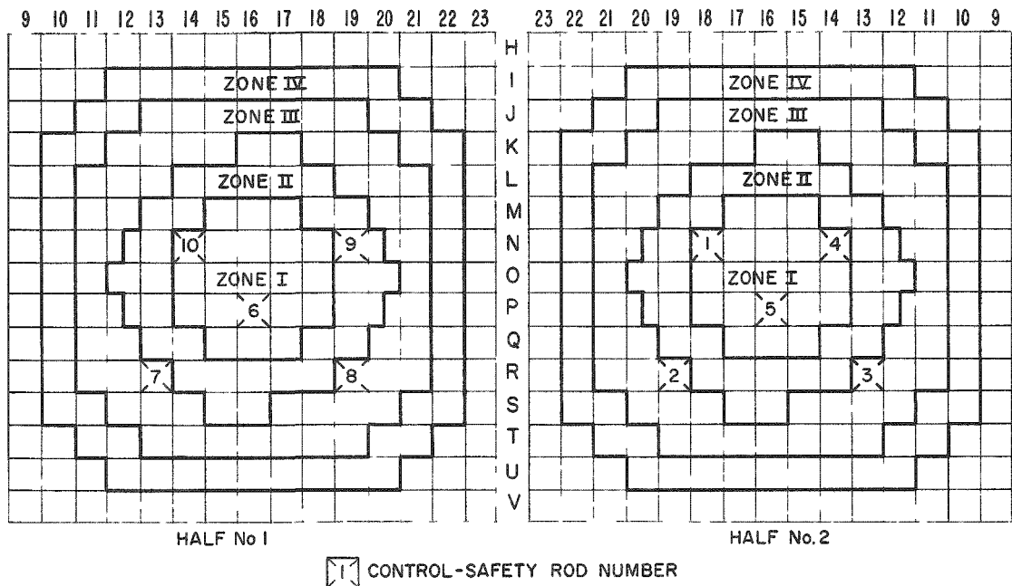
Fig. 2. Interface Views of Assembly 40
