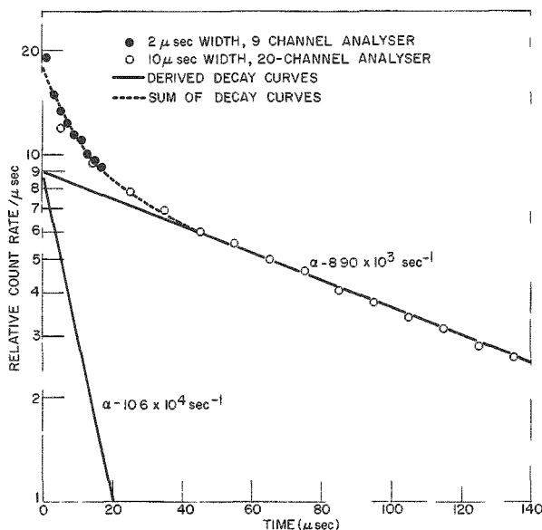
Fig. 23. Typical Rossi-alpha Measurements
