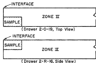
Fig. 16. Nonfissile Sample Locations for Reactivity Coefficient Measurements at Radial Core Boundary
