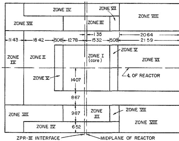
Fig. 1. Horizontal Cross Section of Assembly 40 (Cylindrical Symmetry)
