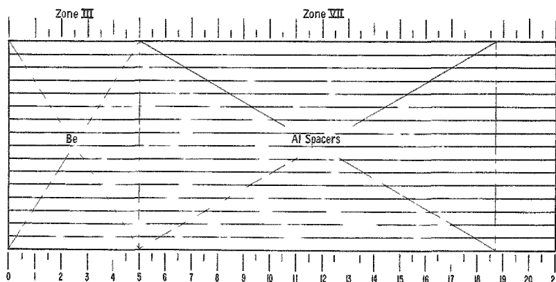
Fig. 7. Zone III Drawer Master Loading Chart (Half No. 1)
