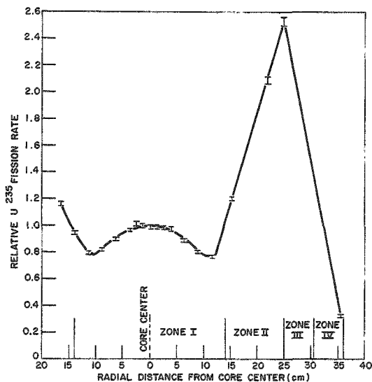
Fig. 18 U 235 Radial Fission Traverse
