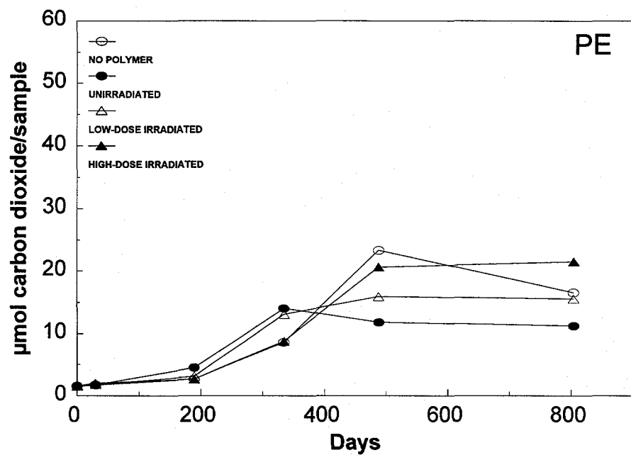
Figure 6. Carbon dioxide produced in anaerobic unamended samples containing polyethylene.
