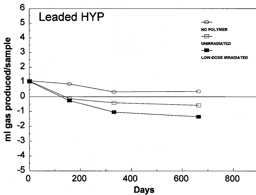
Figure 33. Total gas produced in aerobic unamended samples containing leaded hypalon.
