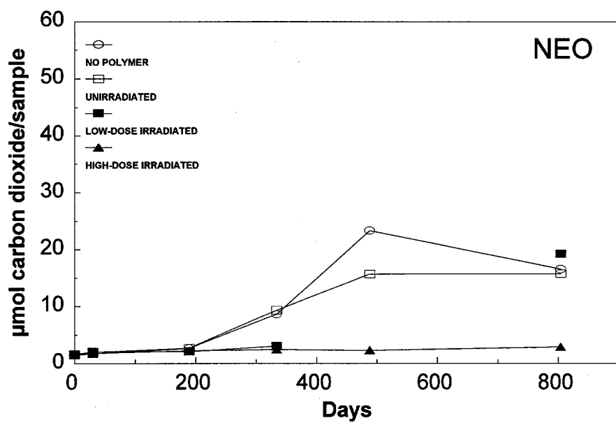
Figure 22. Carbon dioxide produced in anaerobic unamended samples containing neoprene.
