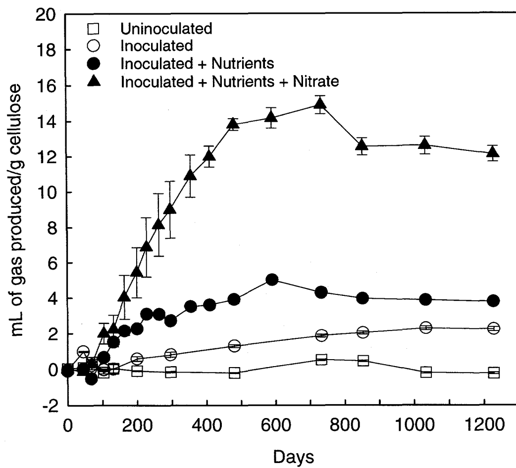
Figure 13. Total gas produced in anaerobic samples.
