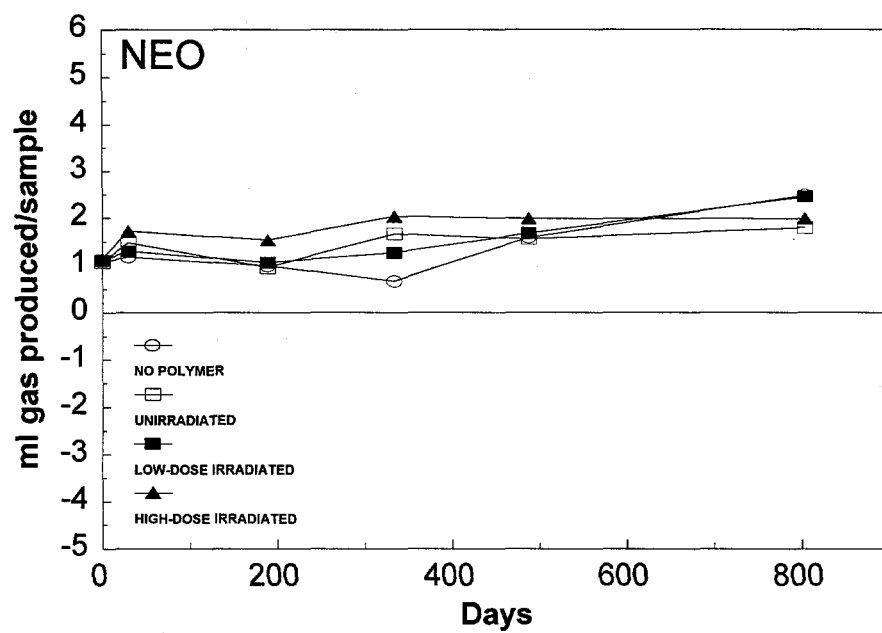
Figure 21. Total gas produced in anaerobic unamended samples containing neoprene.
