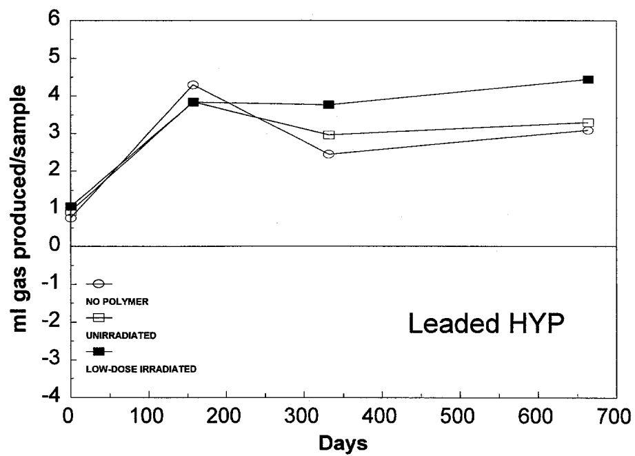
Figure 39. Total gas produced in anaerobic amended samples containing leaded hypalon.
