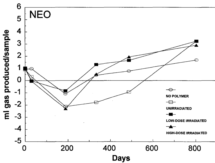
Figure 17. Total gas produced in aerobic unamended samples containing neoprene.
