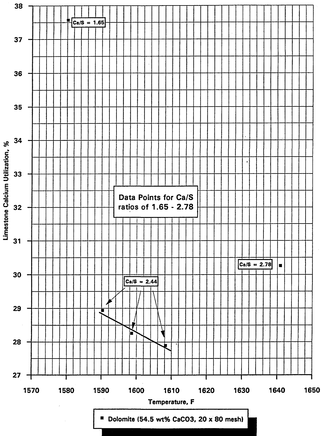
Figure 4-9. Calcium utilization versus temperature for dolomitic limestone
