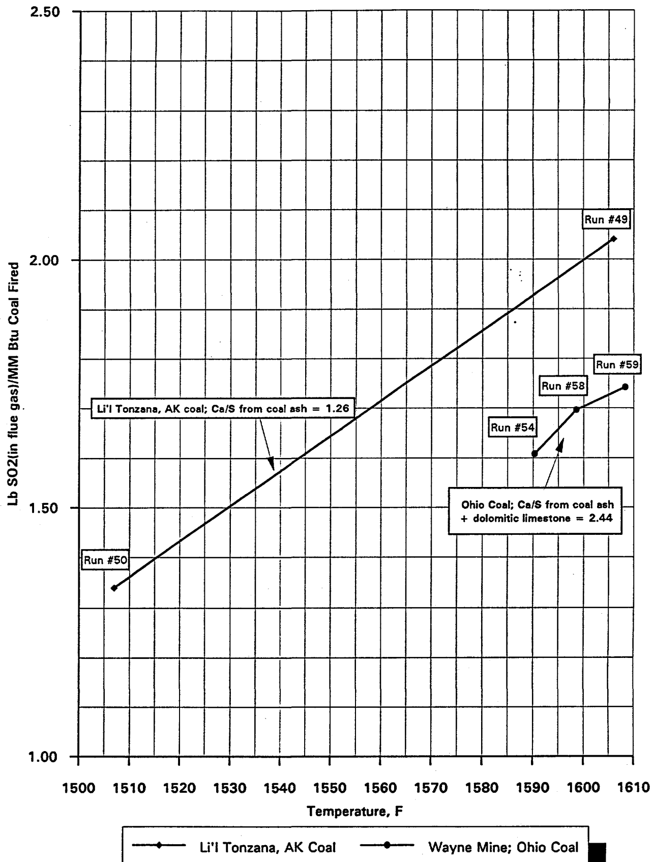
Figure 4-7. SO2 emissions versus bed temperature
