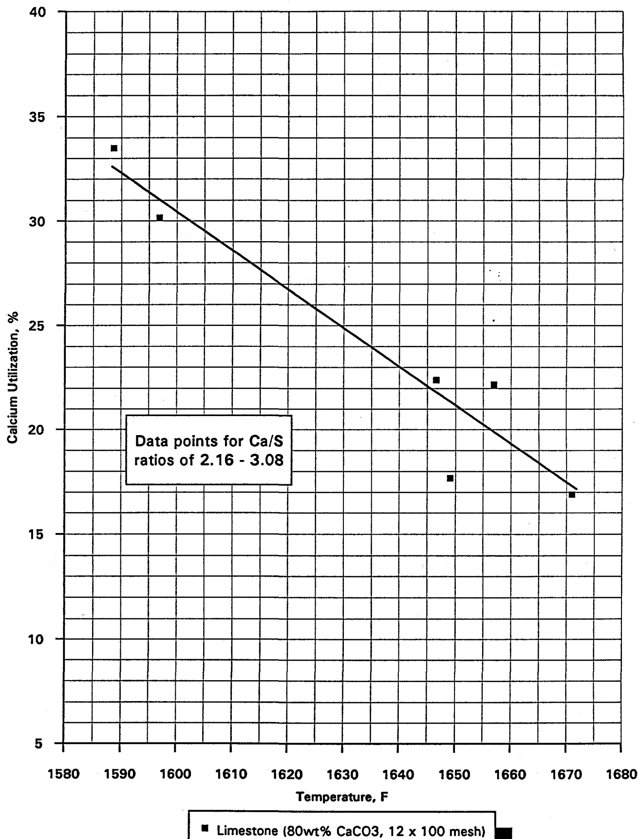
Figure 4-8. Calcium utilization versus temperature for calcitic limestone
