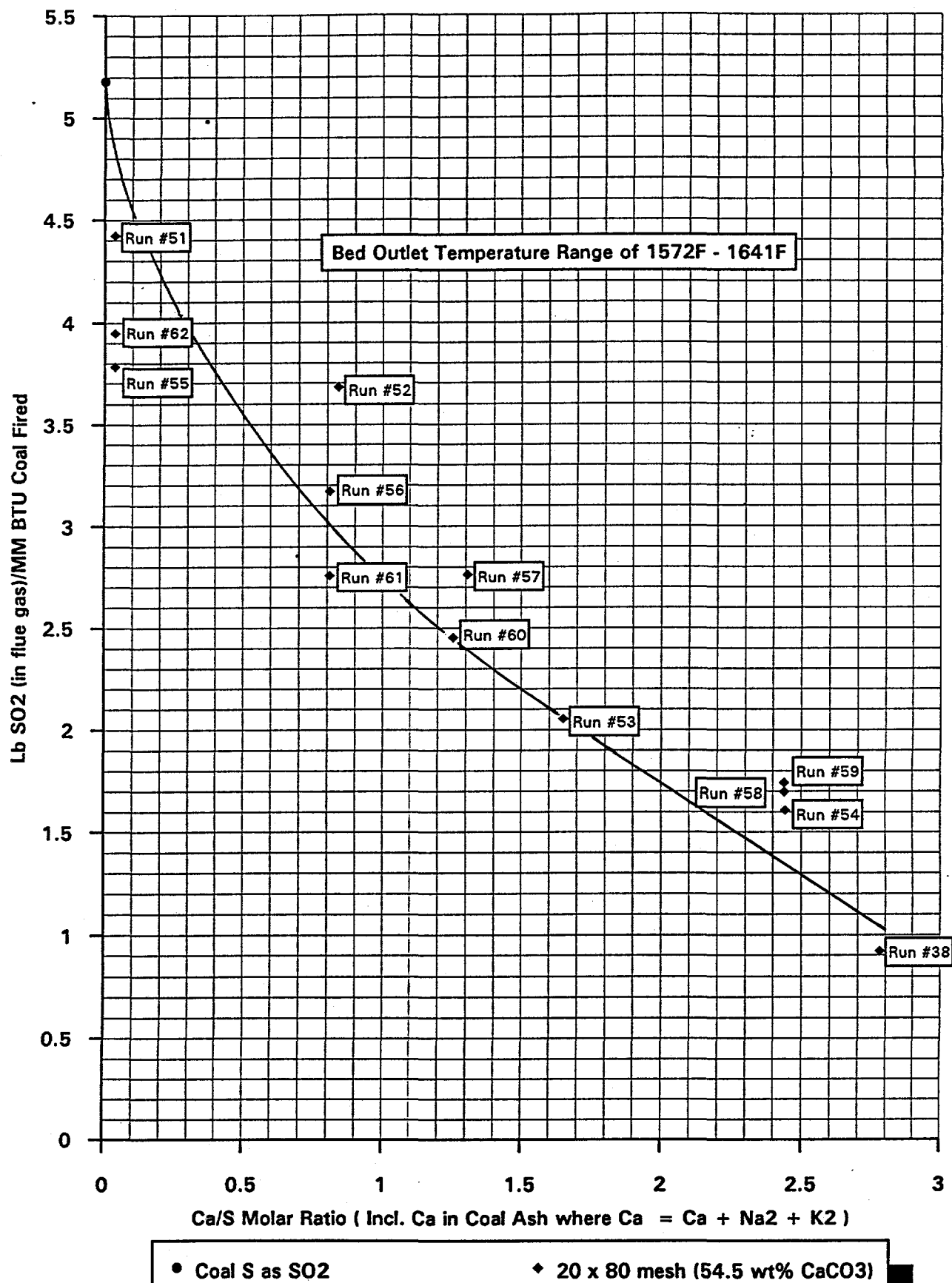
Figure 4-5. Ca/S Ratio versus SO 2 w/dolomitic limestone
