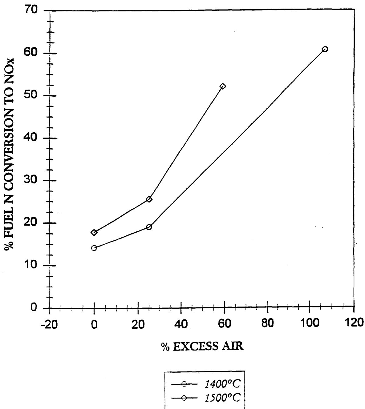
Figure 12 Effects of Excess Air and Temperature on \text{NO}_x Emissions for Wannian Anthracite
