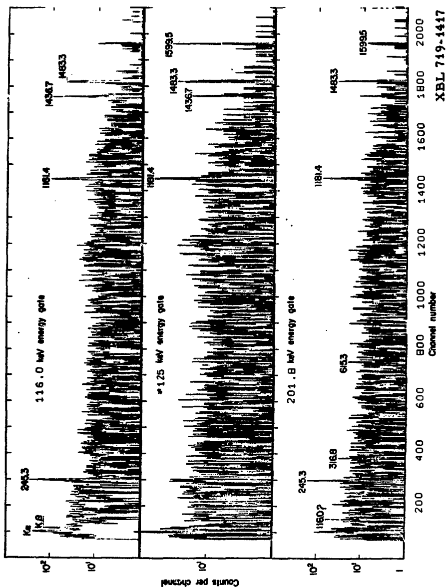
Fig. 14. Gamma-ray spectra in prompt coincidence with E_{\gamma} = 116.0 keV (top), E_{\gamma} \approx 125 keV (middle) and E_{\gamma} = 201.8 keV (bottom).
