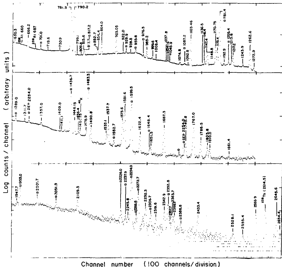
Fig. 51. Gamma-ray spectrum of a mixed source of astatine in the energy range of 630-2660 keV taken with a coaxial Ge(Li) spectrometer. The symbol \square is used to denote gamma-rays due to the decay of ^{210}\text{At} .
