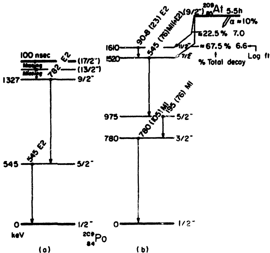
Fig. 48. Summary of previous studies of ^{209}\text{Po} level structure. (a) Level scheme of ^{209}\text{Po} proposed by Yamazaki and Matthias 74 . (b) Decay scheme of ^{210}\text{At} proposed by Stoner 36 .
