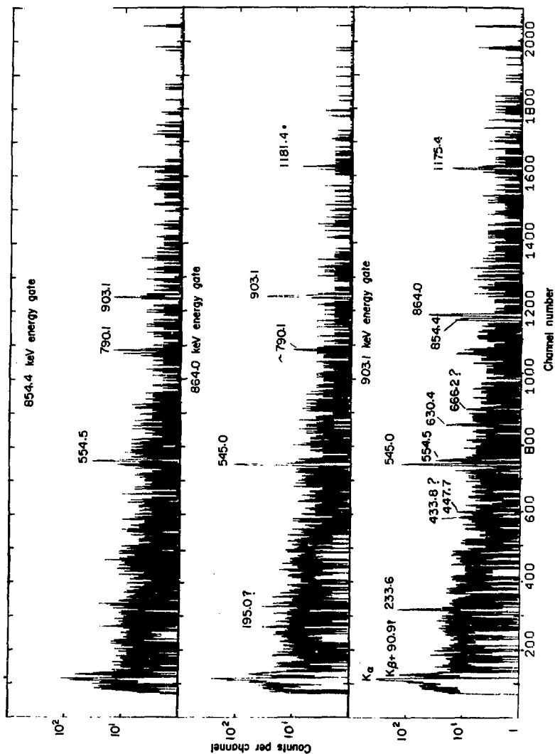
Fig. 65. Gamma-ray spectra in prompt coincidence with E_Y = 854.4 keV (top), E_Y = 864.0 keV (middle) and E_Y = 903.1 keV (bottom).
