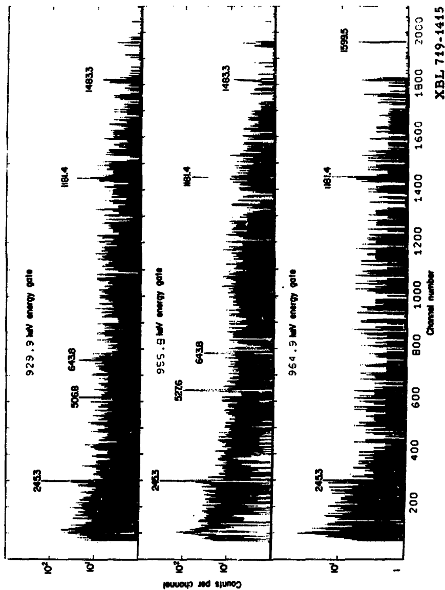
Fig. 24. Gamma-ray spectra in prompt coincidence with E_Y = 929.9 keV (top), E_Y = 955.8 keV (middle) and E_Y = 964.9 keV (bottom).
