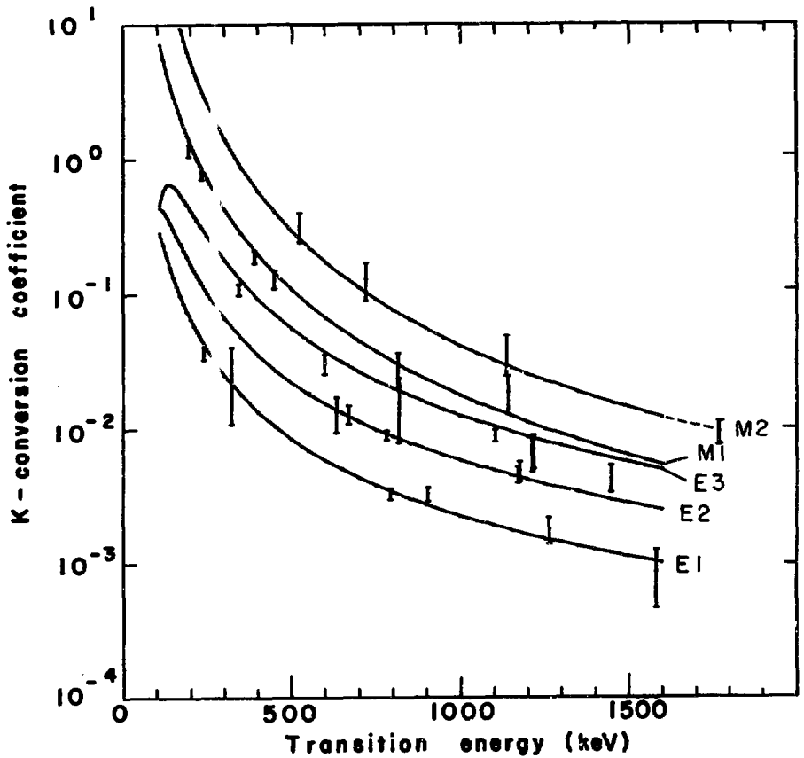
Fig. 77. Comparison of the experimental K-conversion coefficients of some ^{209}\text{At} transitions with the theoretical values of Hager and Seltzer 42 ). Lines are theoretical values 42 ) and points are experimental values measured relative to the 545.0 keV E2 transition. The values for M2 transitions were extrapolated (dotted line) to 1770 keV.
