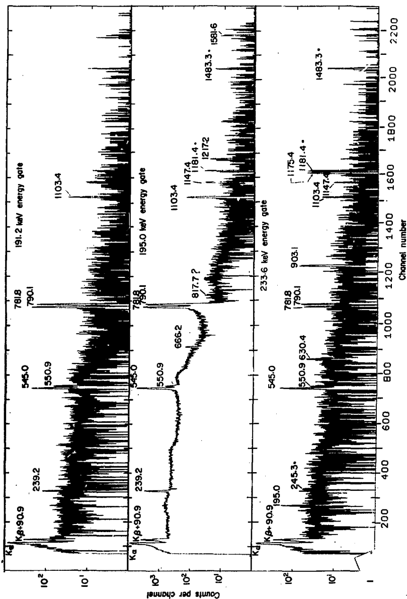
Fig. 57. Gamma-ray spectra in prompt coincidence with E_Y = 191.2 keV (top), E_Y = 195.0 keV (middle) and E_Y = 233.6 keV (bottom).
