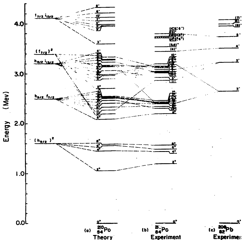
Fig. 47. Comparison of the experimental level scheme of ^{210}\text{Po} (b) with a shell model calculation 41) (a) and with the experimental level scheme ^{208}\text{Pb} 35) (c). The dotted lines connect levels believed to have components due to the same configuration. The zero-order energies of the two-proton configurations in ^{210}\text{Po} are shown to the left.
