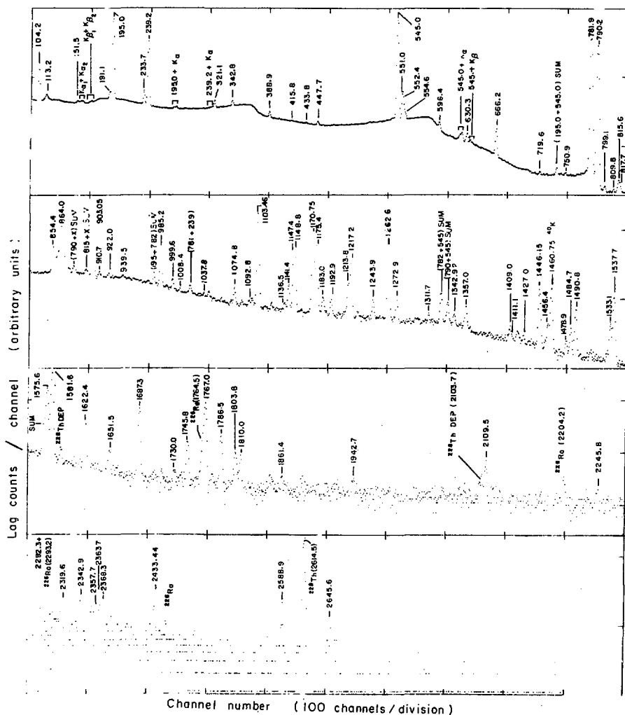
Fig. 52. Gamma-ray spectrum of a mass separated ^{209}\text{At} source in the energy range of 100-2700 keV taken with a coaxial Ge(Li) spectrometer.
