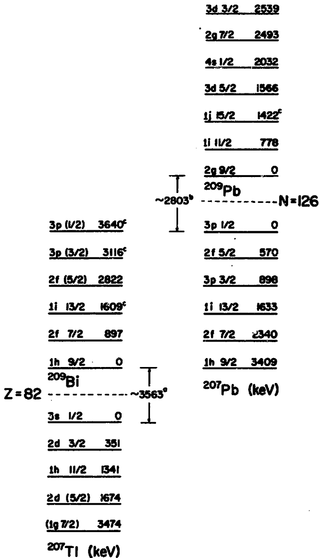
Fig. 4. Experimental 9) single-particle states in the lead region.
