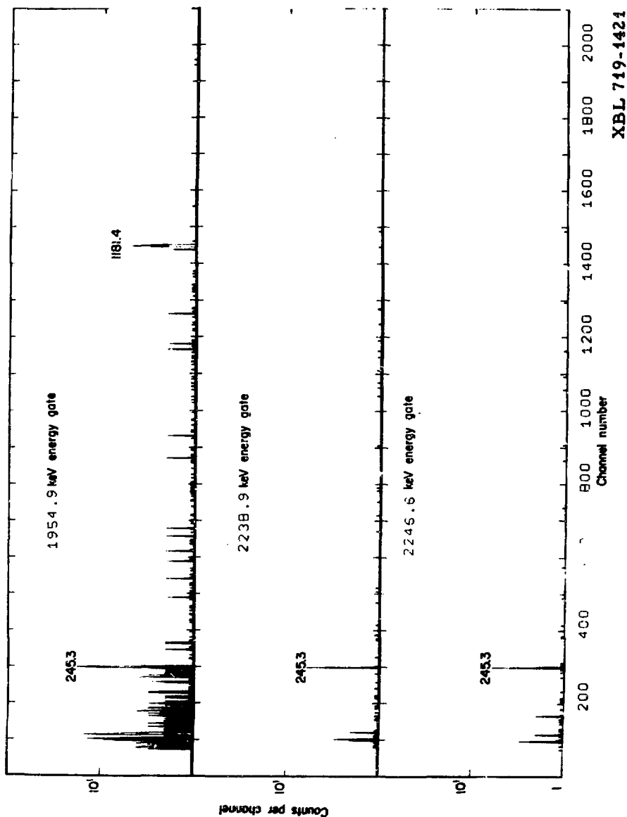
Fig. 30. Gamma-ray spectra in prompt coincidence with E_Y = 1954.9 keV (top), E_Y = 2237.9 keV (middle) and E_Y = 2246.6 keV (bottom). (Note that middle spectrum should read: 2237.9 keV energy gate.)
