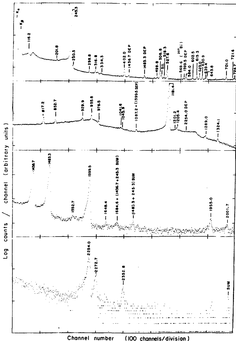
Fig. 11. "Gross" \gamma - \gamma coincidence spectrum for the 40-cm 3 (active volume) coaxial Ge(Li) detector.
