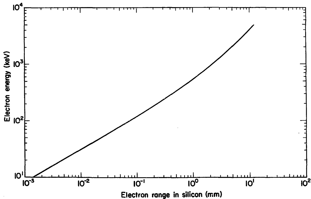
Fig. 5. Range 12 of electrons in silicon.
