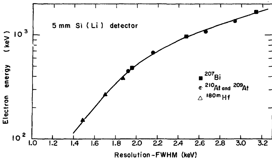
Fig. 3. Resolution of the Si(Li) spectrometer for electrons. Points are experimental.
