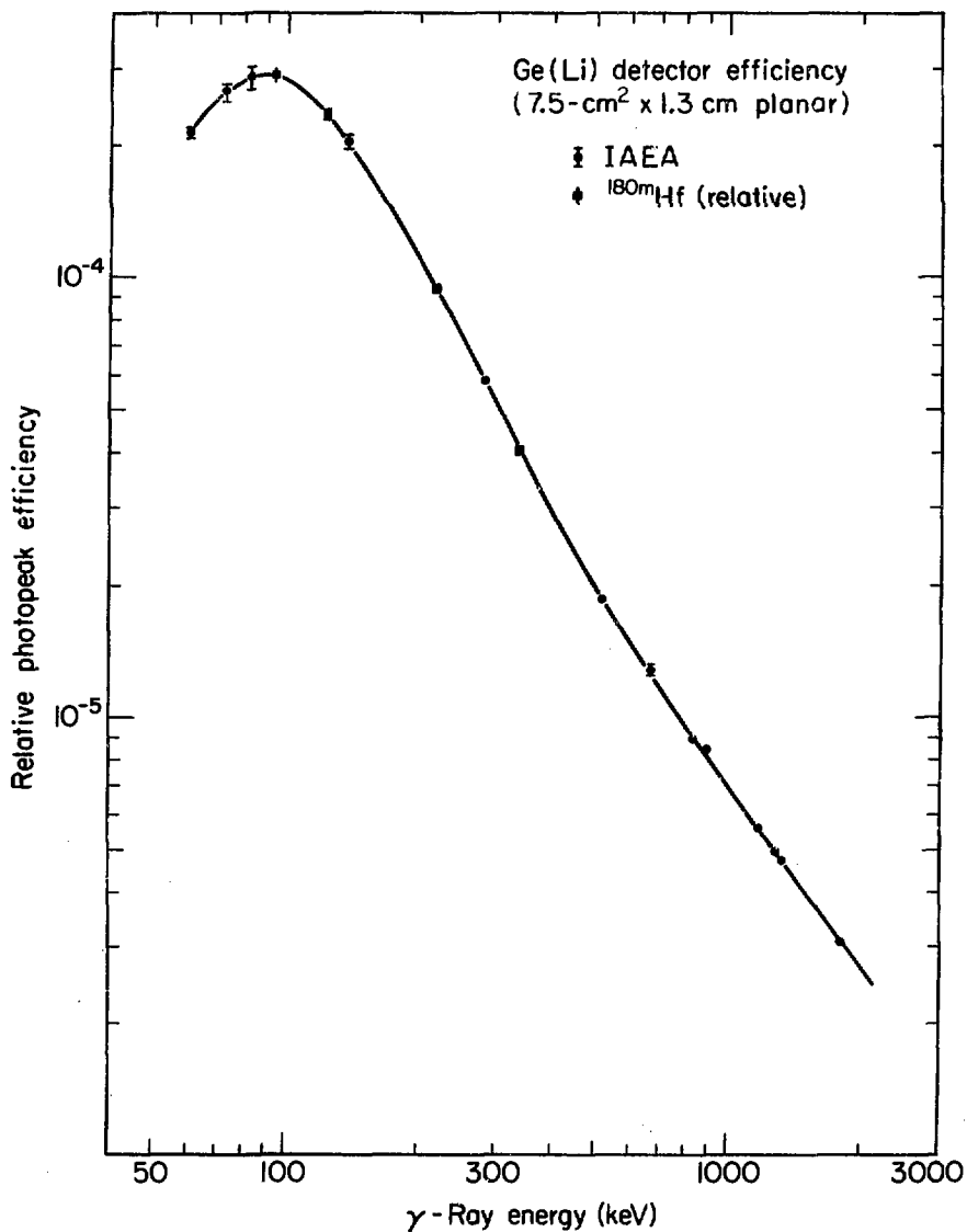
Fig. 1. The relative photopeak efficiency curve for the 10-cm 3 Ge(Li) detector as a function of gamma-ray energy.
