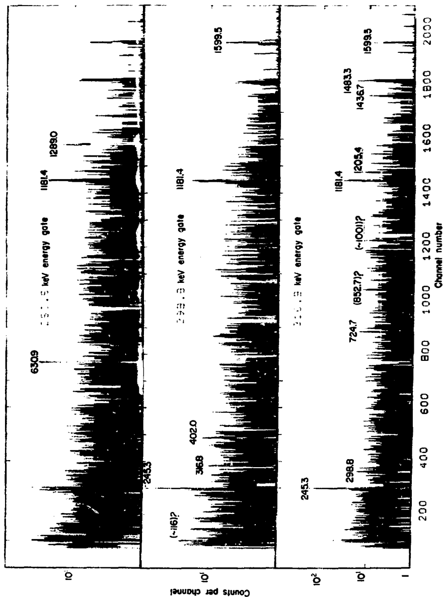
Fig. 16. Gamma-ray spectra in prompt coincidence with E_Y = 250.5 keV (top), E_Y = 298.8 keV (middle) and E_Y = 316.8 keV (bottom).
