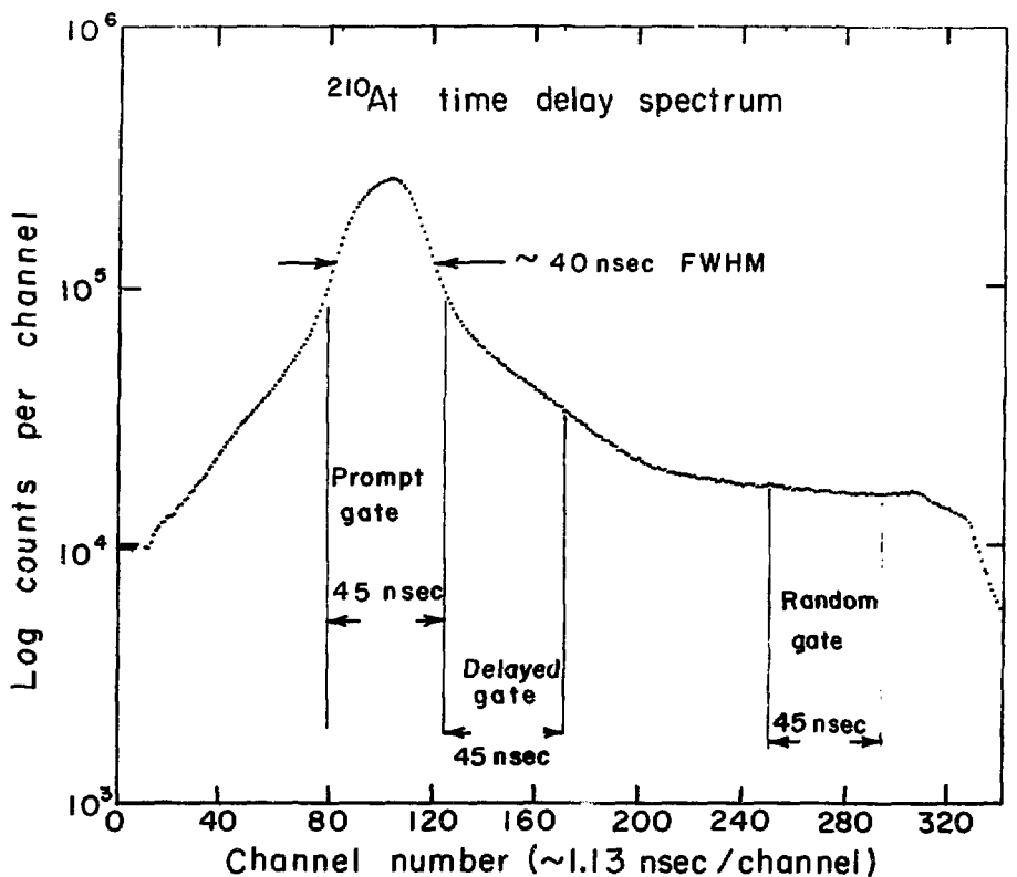
Fig. 13. "Gross" time distribution for the ^{210}\text{At} \gamma - \gamma coincidence data. The 45 nsec gates were used to obtain the coincidence events shown in figs. 14-34.
