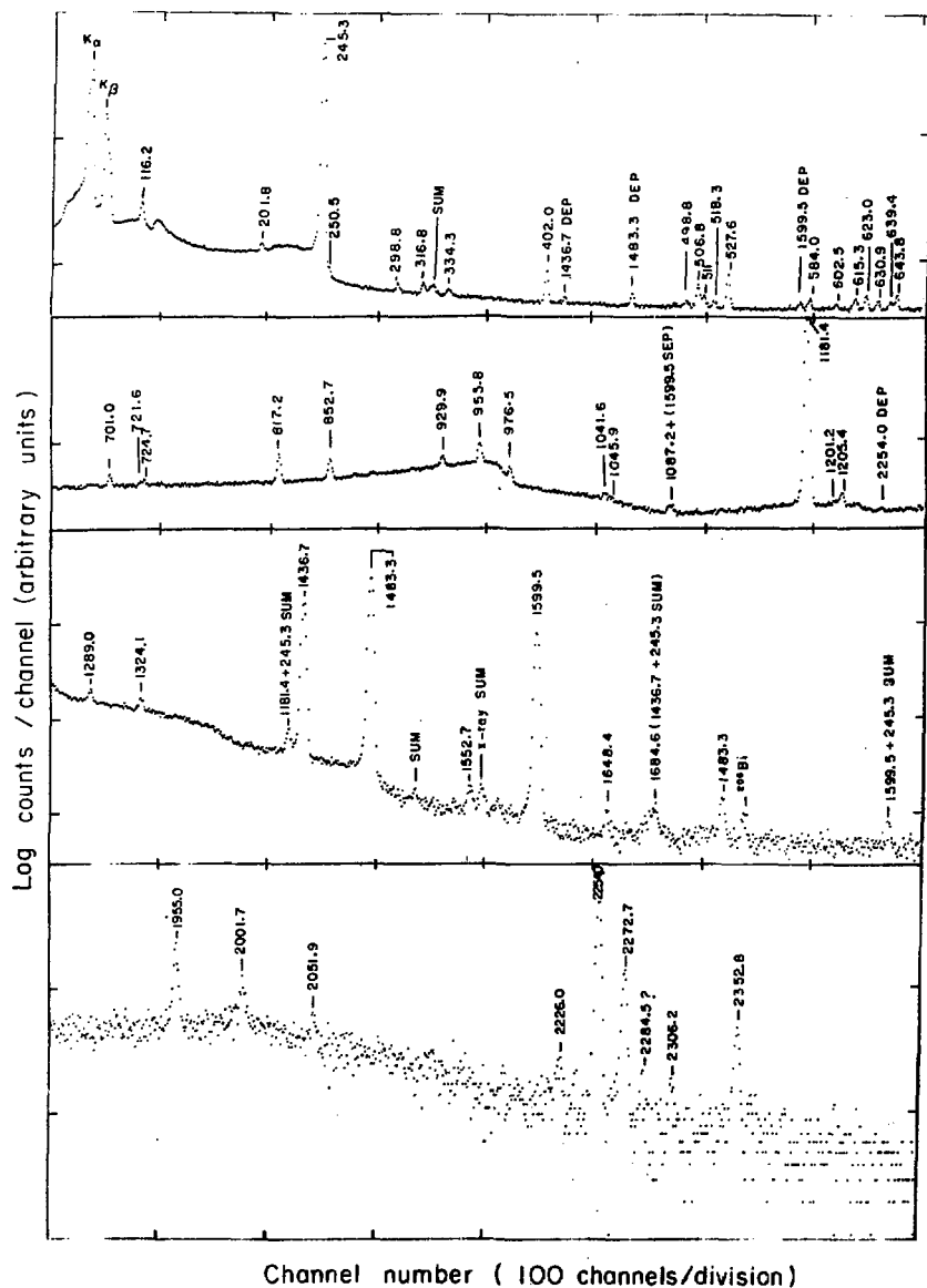
Fig. 12. "Gross" \gamma - \gamma coincidence spectrum for the 35-cm 3 (active volume) coaxial Ge(Li) detector.
