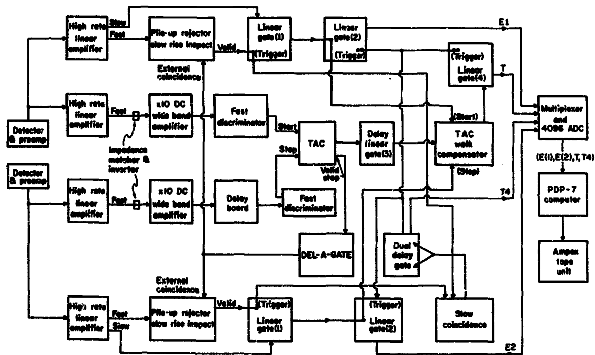
Fig. 4. Block diagram of the Y-Y coincidence system.
