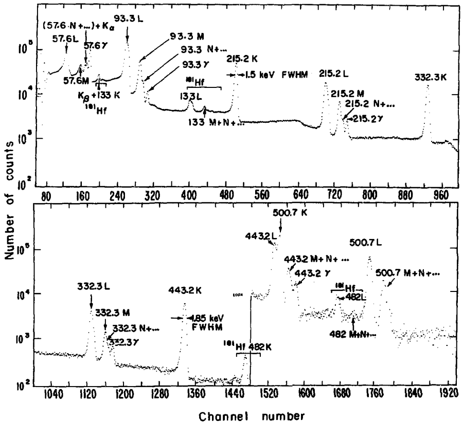
Fig. 4. Conversion electron spectrum of ^{180m}\text{Hf} decay.
