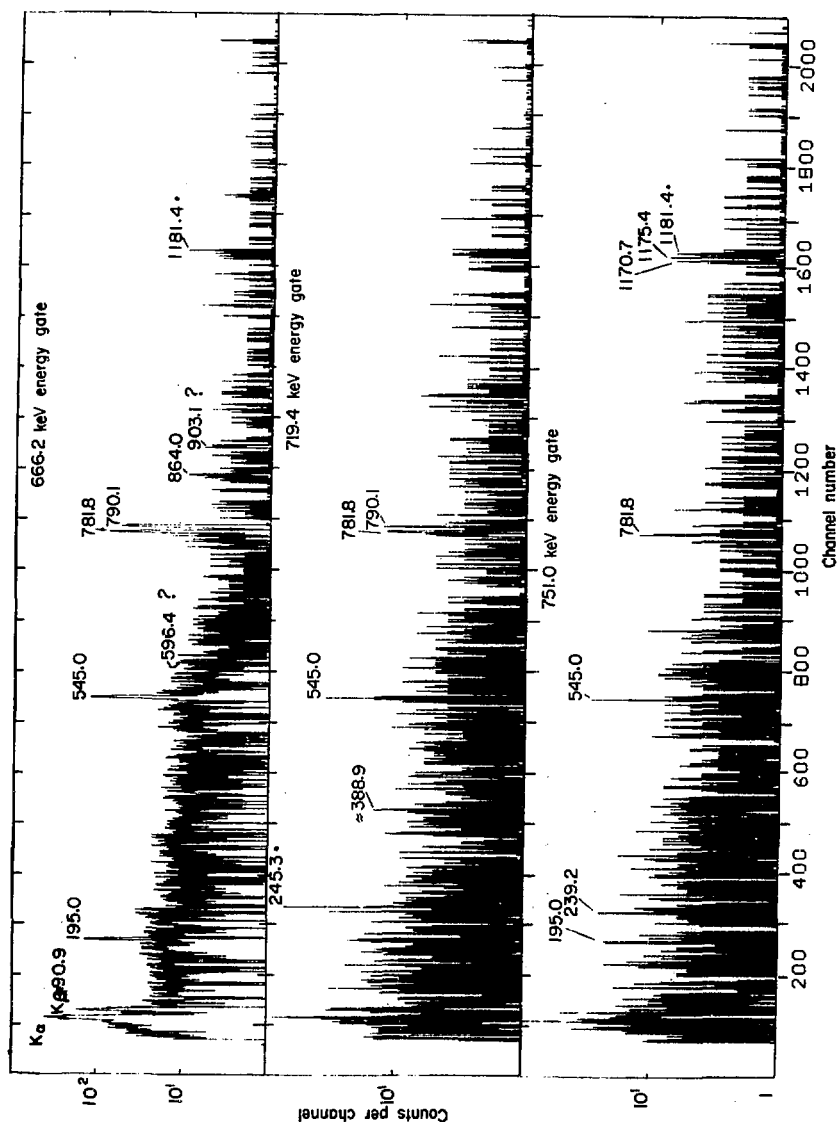
Fig. 62. Gamma-ray spectra in prompt coincidence with E_Y = 666.2 keV (top), E_Y = 719.4 keV (middle) and E_Y = 751.0 keV (bottom).
