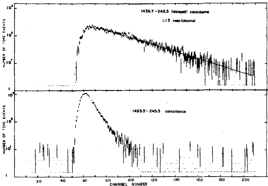
Fig. 41. Time distribution curves for the 1436.7-245.3 and 1483.3-245.3 keV gamma-ray cascades. Stop pulses (with a fixed delay) for the pulse-height circuitry were supplied by the 245.3 keV photopeak and start pulses by the 1436.7 and 1483.3 keV photopeaks.
