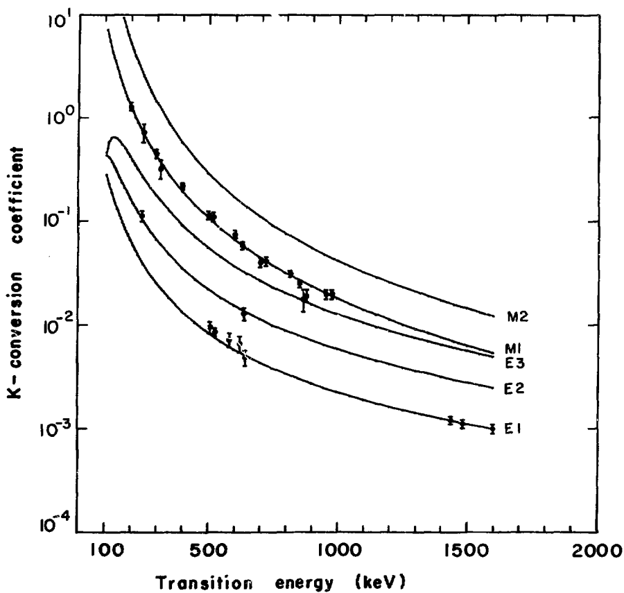
Fig. 7. Comparison of the experimental K-conversion coefficients from the decay of ^{210}_{85}\text{At} with the theoretical values of Hager and Seltzer 11 ).
