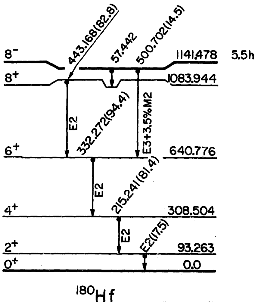
Fig. 2. The ^{180}\text{Hf} decay scheme used in the photopeak efficiency determination. The energies (keV) are based on the measurements of Gujrathi and D'Auria 30 ). The absolute gamma-ray intensities expressed in per cent from this study are shown in parenthesis.
