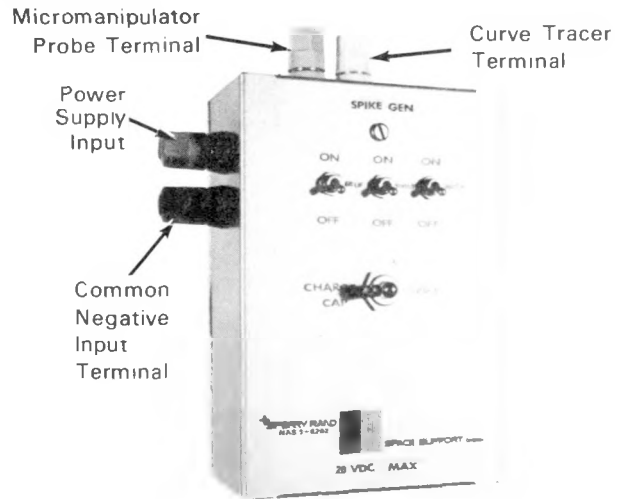
Figure 1a. Assembled Generator, One Half Actual Size.
