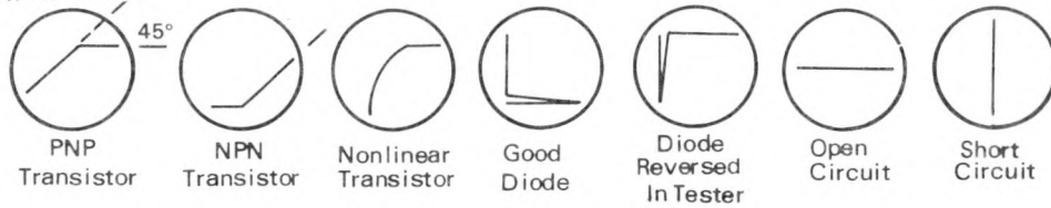
Figure 1B. Typical Waveforms of Devices Undergoing Test
