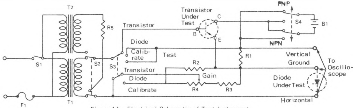
Figure 1A. Electrical Schematic of Test Instrument
