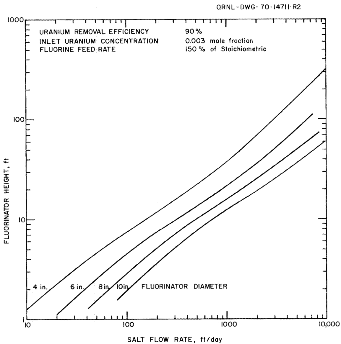
Fig. 14. Variation of Calculated Fluorinator Height with Salt Flow Rate and Fluorinator Diameter for a Uranium Removal Efficiency of 90%.
