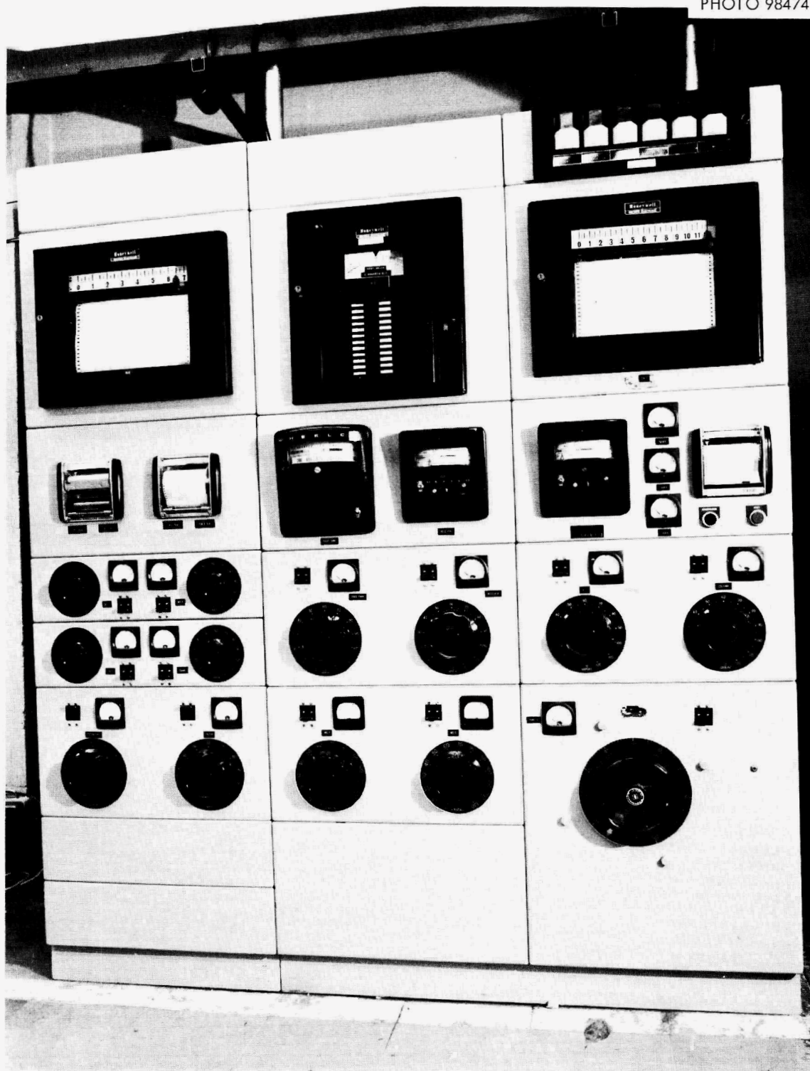
Fig. 26. Panelboard for Salt Purification Equipment. Temperature, level, and pressure recorders and heater controls are included.
