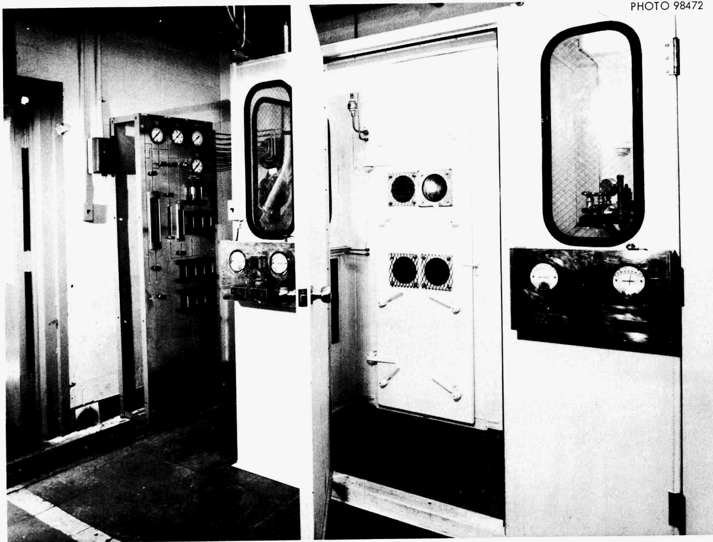
Fig. 27. Gas Flow Panelboard and Cell Entrance for Salt Purification Equipment.
