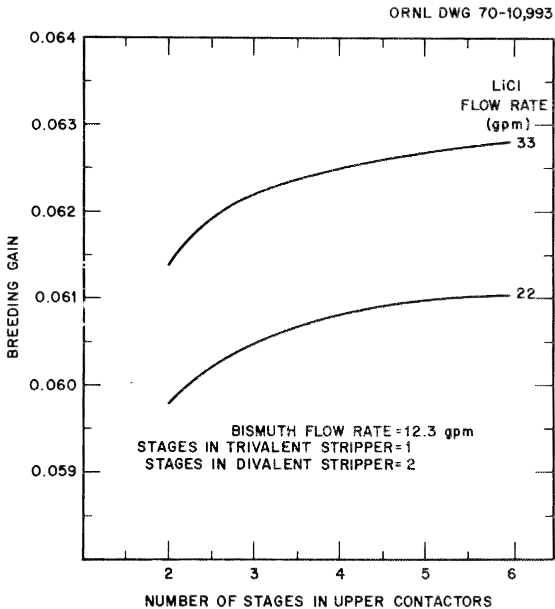
Fig. 6. Effect of the Number of Stages in the Fuel Salt--Bismuth and LiCl-Bismuth Contactors on MSBR Performance.
