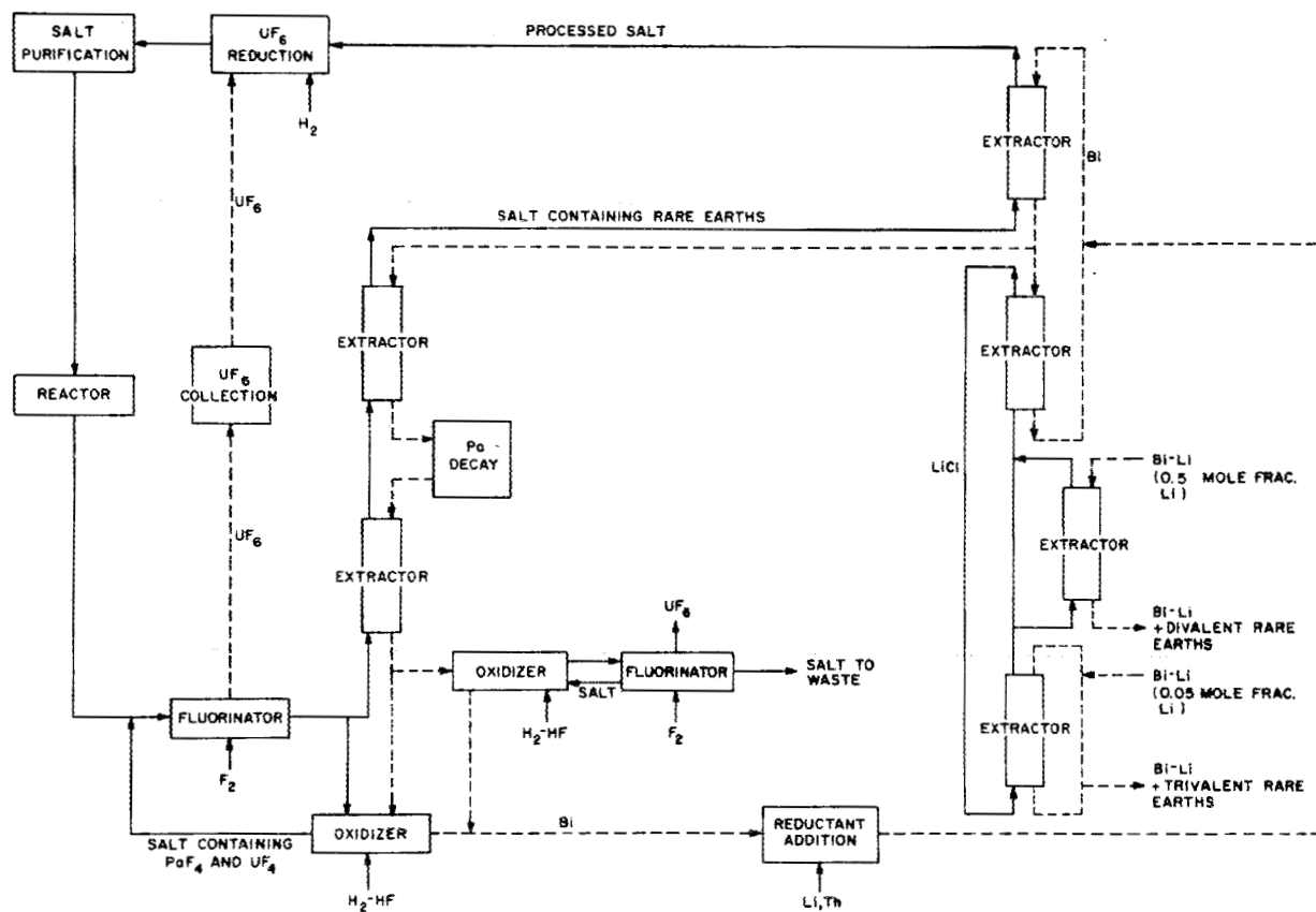
Fig. 1. Flowsheet for Processing a Single-Fluid MSBR by Fluorination-Reductive Extraction and the Metal Transfer Process.
