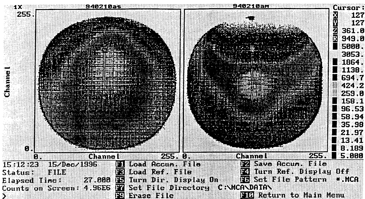
Fig. 12. Channeling patterns for scattering of 70 keV O^{7+} from Au(110) slightly above the surface reconstruction phase transition temperature of 650K (i.e., for [1 \times 1] random surface reconstruction), and slightly below (i.e., for [2 \times 1] "missing row" surface reconstruction).
