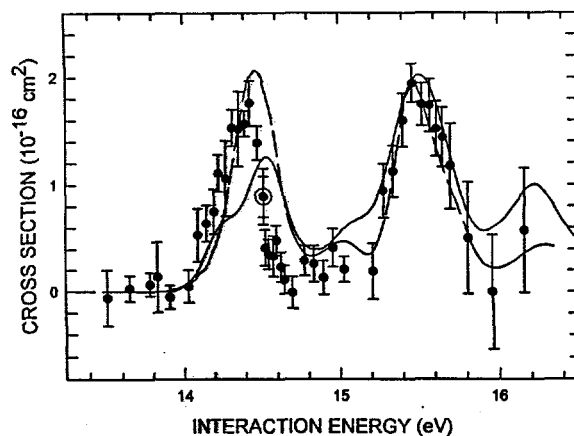
Fig. 6. Electron impact excitation cross section of \text{Ar}^{6+} vs. electron energy.
