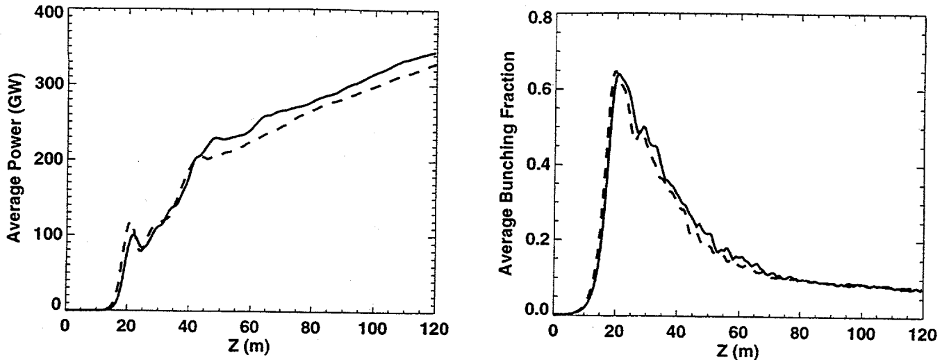
Figure 6. Average power and bunching fraction versus z for two 1-D LCLS-like GINGER simulation run. The solid line is from a run with a shot noise start while the dotted line is from a constant P(\omega) (i.e. broadband spectrum) start with no shot noise.
