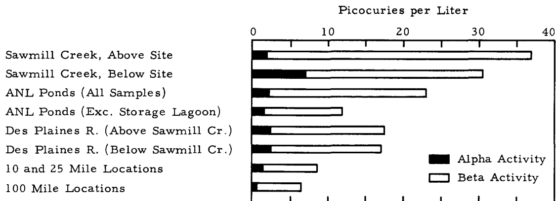
Figure 5 AVERAGE RADIOACTIVITY IN BOTTOM SILT, 1961
