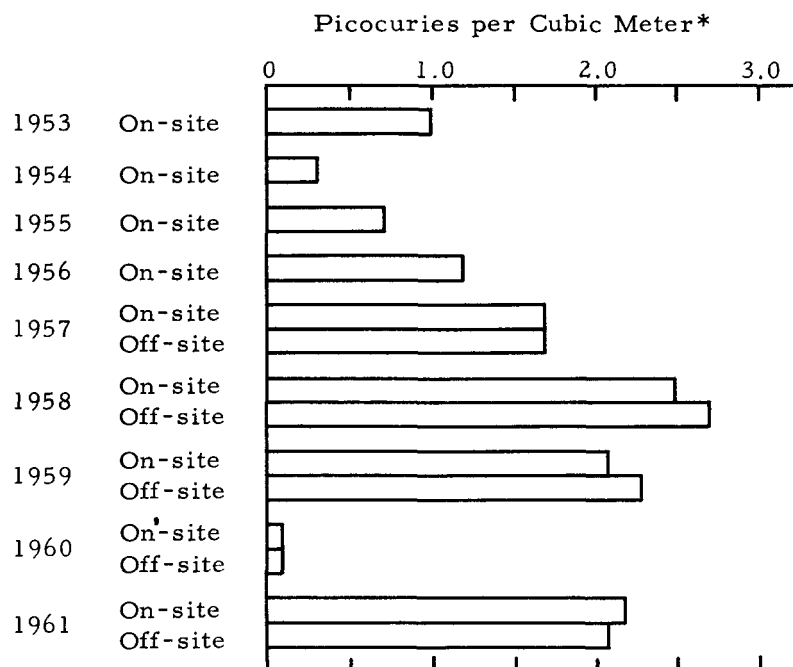
Figure 12 AVERAGE BETA ACTIVITY IN WEEKLY AIR FILTER SAMPLES, 1953-61
