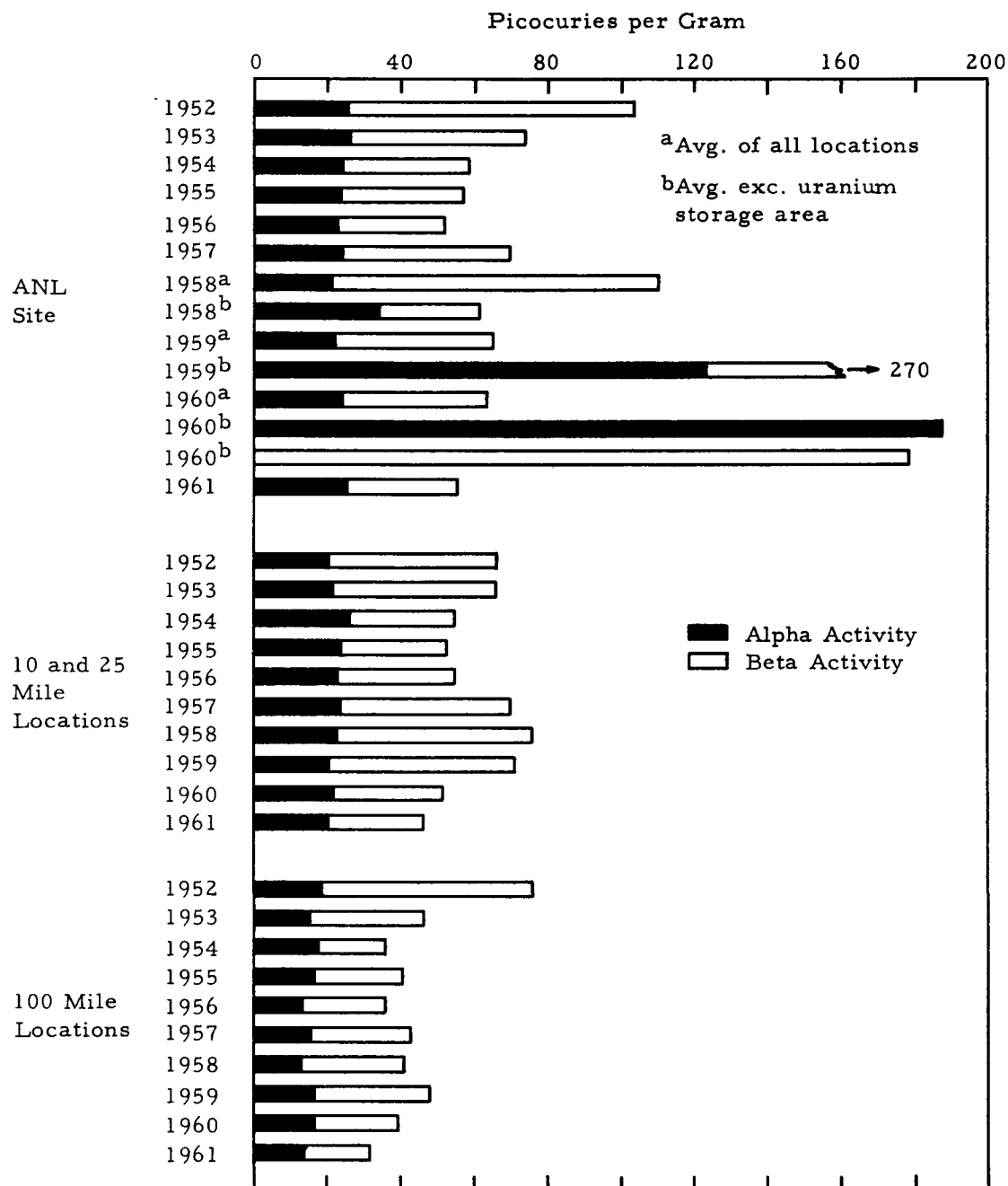
Figure 9 AVERAGE RADIOACTIVITY IN SOIL, 1952-61
