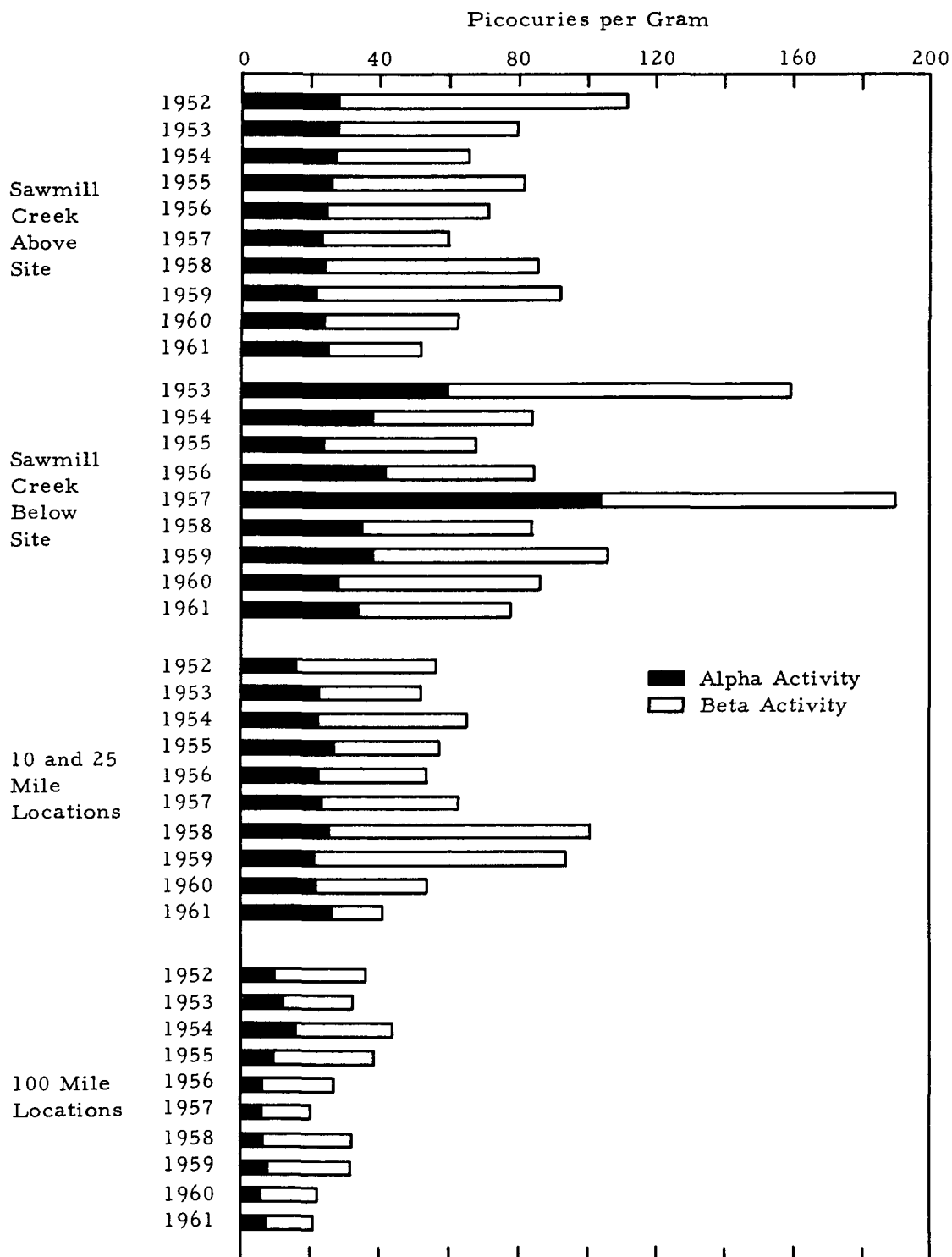
Figure 8 AVERAGE RADIOACTIVITY IN BOTTOM SILT, 1952-61
