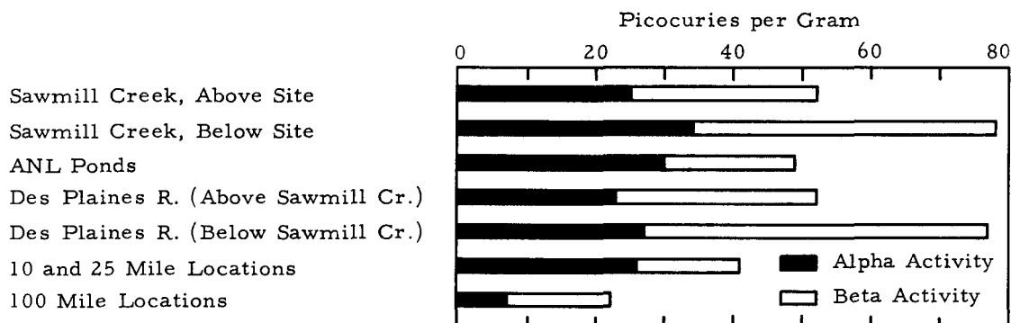
Figure 6 AVERAGE RADIOACTIVITY IN SOIL AND PLANTS, 1961
