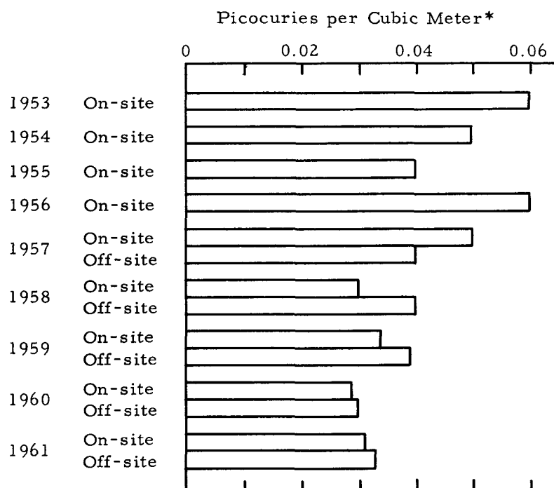
Figure 11 AVERAGE ALPHA ACTIVITY IN WEEKLY AIR FILTER SAMPLES, 1953-61
