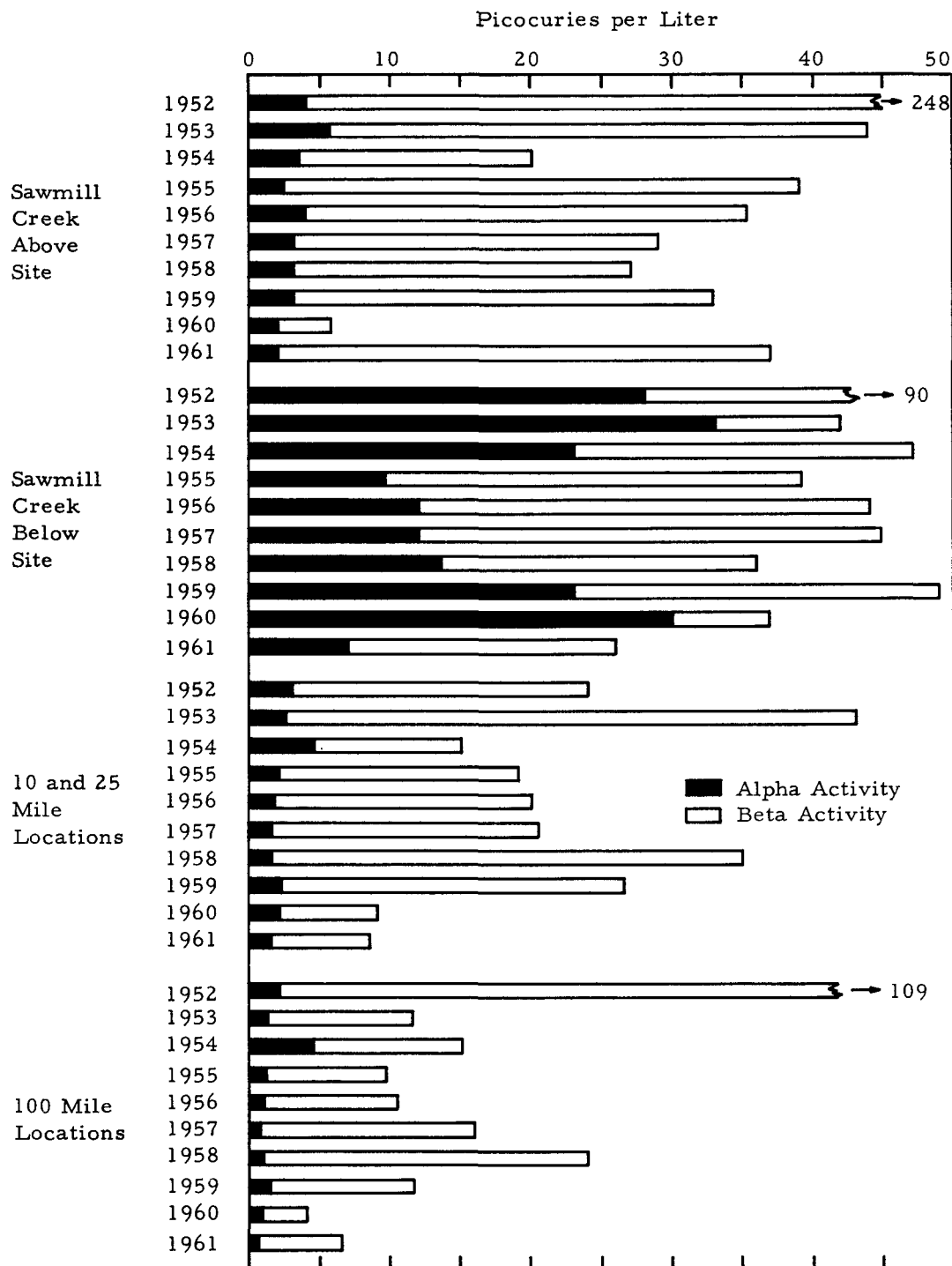
Figure 7 AVERAGE RADIOACTIVITY IN SURFACE WATER, 1952-61
