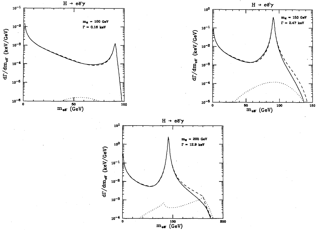
FIG. 2. The invariant mass distribution of the decay mode H \rightarrow f\bar{f}\gamma for several Higgs masses is shown. The solid line is the full calculation, the dashed line is the pole contribution and the dotted line is the box contribution.
