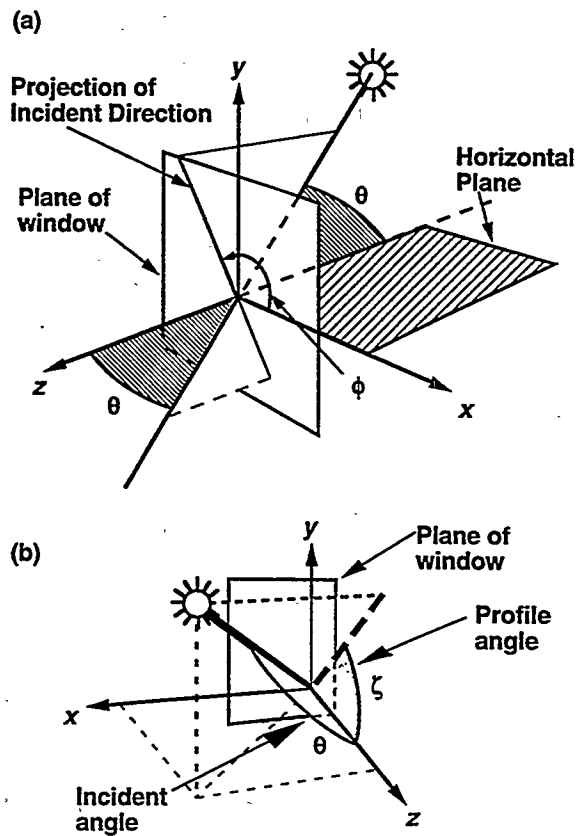
Figure 2. Definition of angles. (a) Incident and azimuthal angles, (\theta, \phi) . (b) Profile angle, \zeta , compared with incident angle.
