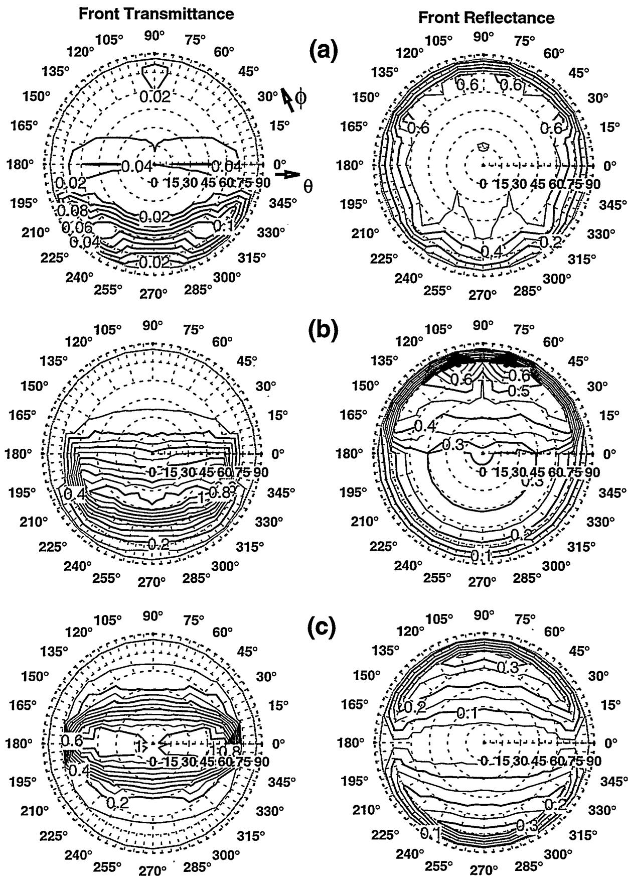
Figure 3. Directional-hemispherical front transmittance and reflectance of the venetian blind for three slat positions. (a) Closed (downward), (b) 45° tilt (downward) (c) Open (horizontal). Contours of constant transmittance or reflectance are displayed in a polar plot projection (window plane, looking outward) in which the radius is the angle \theta (degrees) and the azimuth is the azimuthal angle \phi about the normal to the window plane.
