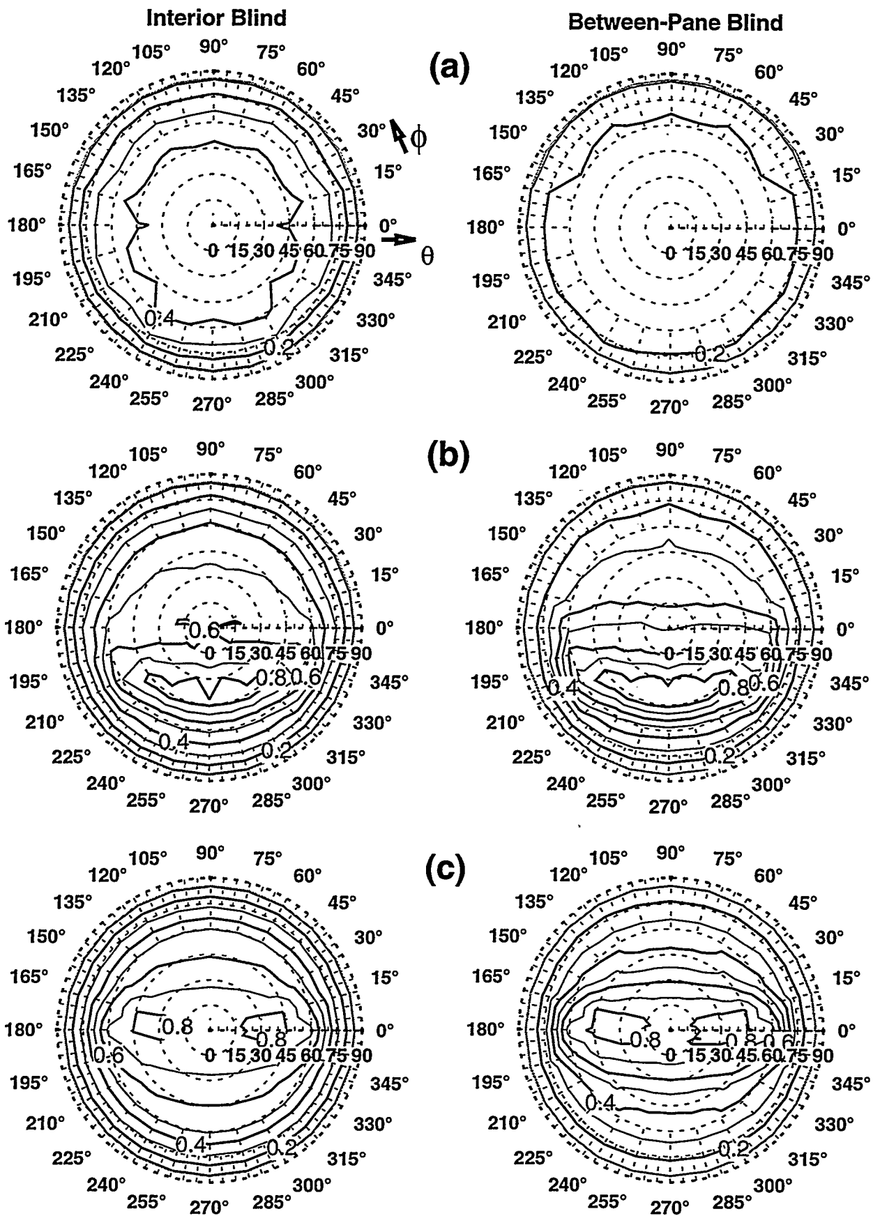
Figure 5. Solar heat gain coefficient for double glazing interior and between-pane blinds. The measurement-derived solar heat gain coefficient as a function of incident direction for clear double glazing in combination with the buff blind placed as an interior blind (left-hand plots) or between-pane blind (right-hand plots) for three slat adjustments: (a) Closed (downward), (b) 45° tilt (downward) (c) Open (horizontal). Contours of constant transmittance or reflectance are displayed in a polar plot projection (window plane, looking outward) in which the radius is the angle \theta (degrees) and the azimuth is the azimuthal angle \phi about the normal to the window plane.
