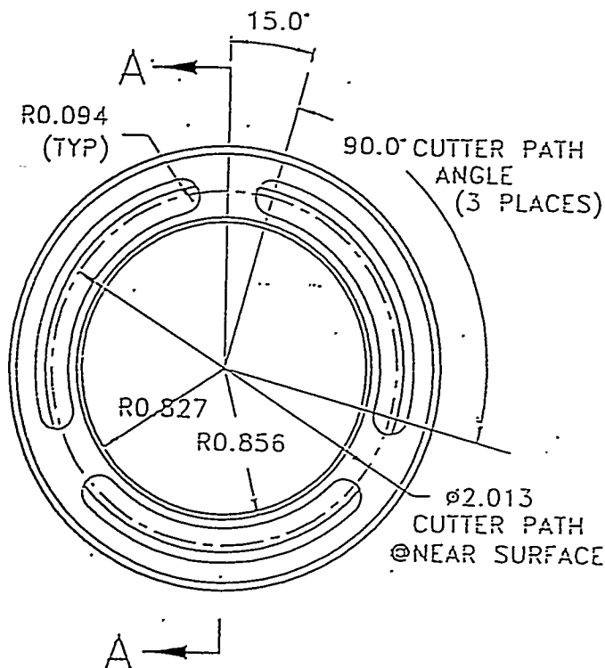
CUTTER ANGLE FOR SLOTS
