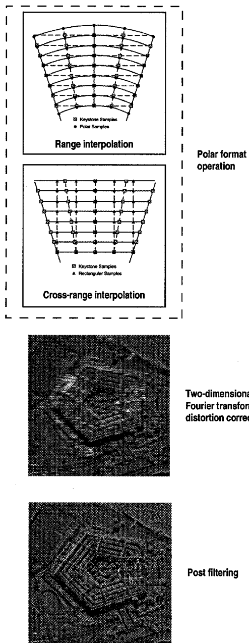
Figure 2: Processing steps for the polar-formatting with post-filtering algorithm (PF2).
