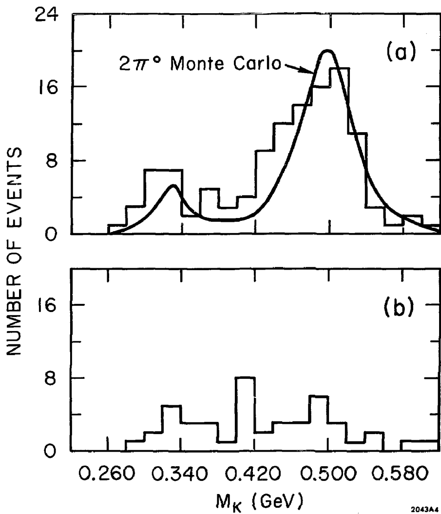
FIG. 7-- K_L^0 mass for 4 \gamma regenerator, (a) unlatched (b) latched.
