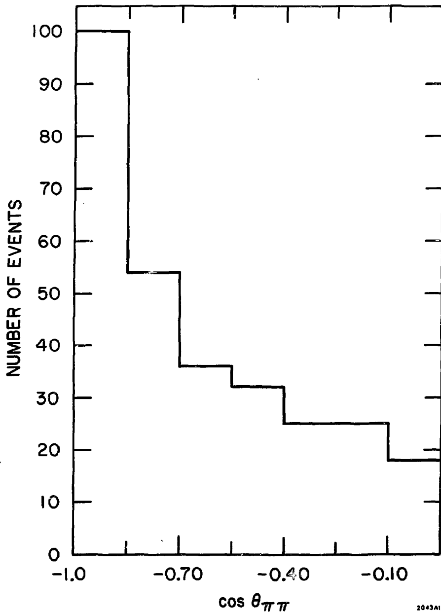
FIG. 8-- \cos \theta_{\pi\pi} for 4\gamma regenerator, unlatched.
