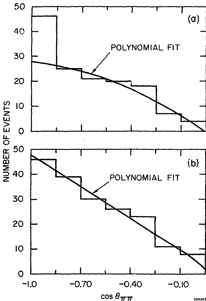
FIG. 11-- \cos \theta_{\pi\pi} for normal running 4\gamma with kinematical cuts (a) unlatched (b) latched.
