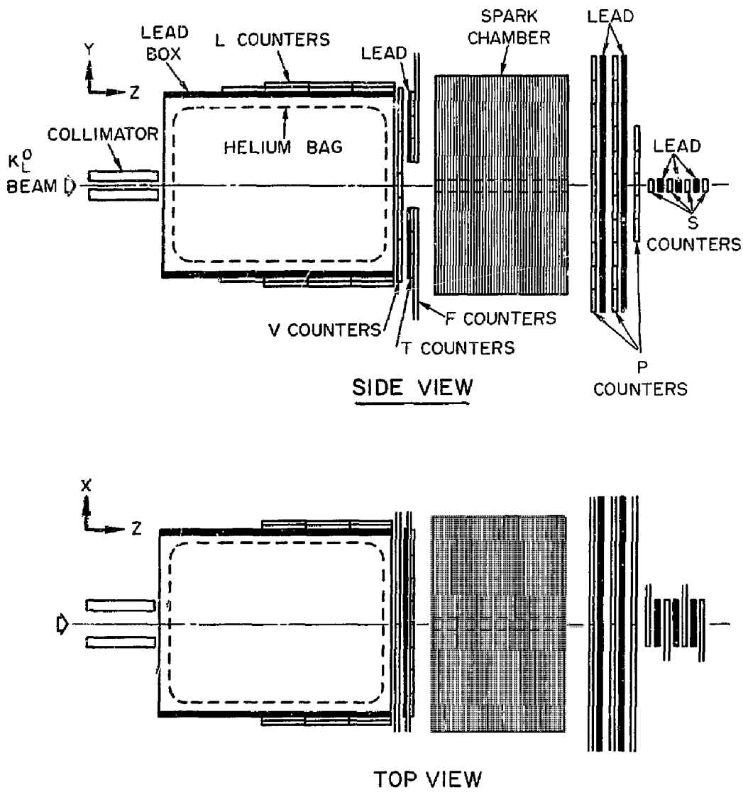
FIG. 3--Detection apparatus (collimation for first data run).
