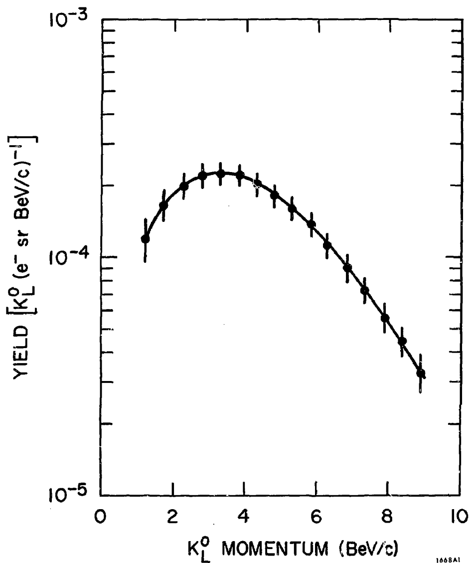
FIG. 2-- K_L^0 momentum spectrum at target.
