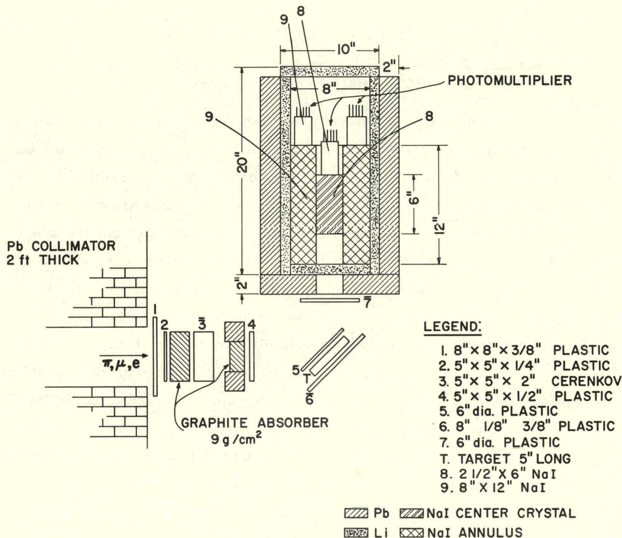
Fig. 24. Physical arrangement of apparatus for measurement of muonic x rays. An x-ray event which is to be analyzed is identified by coincidence ( 245\overline{367}; 89 ). A calibration event consists of coincidence ( 89; 157 ). Counter 8 is the center crystal of the NaI anticoincidence spectrometer.
