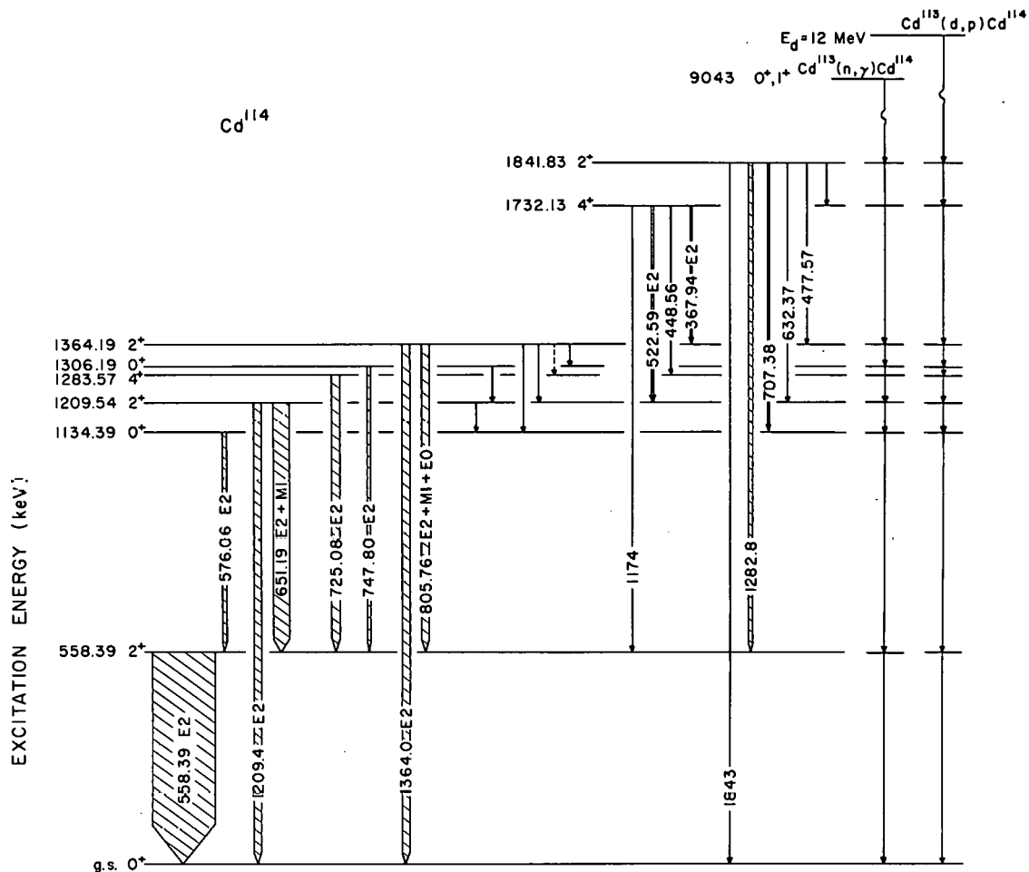
Fig. 4. Proposed level scheme of \text{Cd}^{114} . The excitation energies and proposed spin assignments are given to the left of each level. The energy and multipole assignment (when made) is given on each line. All energies are in keV. The high-energy Ge-diode data and the (d, p) data are presented on the right-hand side of the figure. Each arrow-head indicates an observed transition to the appropriate level.
