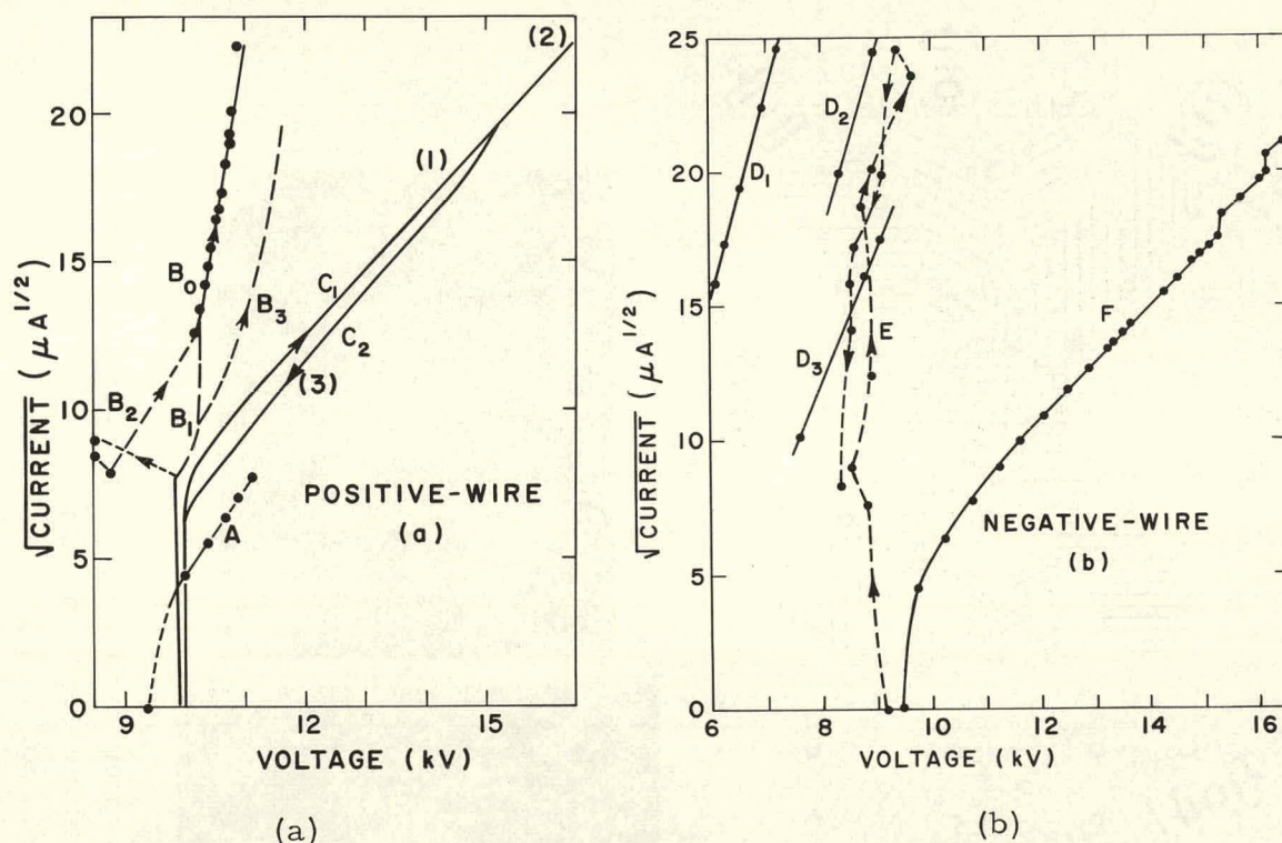
Fig. 9. Corona current between a wire and a cylinder in a closed system containing 80% \text{N}_2 , 20% \text{CO}_2 at 1 atm. (a) Positive-wire corona. Curve A is for fresh gas. After "conditioning" by running at \sim 60 \mu\text{A} for about 30 min, the discharge became much more luminous and the curves became somewhat unreproducible as illustrated by curves B_1 - B_0 , B_2 - B_0 , and B_3 obtained in different tests. After "aging" the same gas for several days (no current flowing), curve C_1 - C_2 was followed—with noticeable sparking initially at (1), later at (2), and finally around (3). Curves A and C were fairly reproducible. (b) Negative-wire corona for the same gas and equipment. Curve D_1 is for fresh gas. "Conditioning" with several hundred microamperes for about 30 min shifts the curve first to D_2 and then D_3 . The negative-wire current seems to flow only from a few luminous points on the wire and fluctuates if the number or positions of the points changes. Curve E was obtained just after the same "positive-wire conditioning" that gave curve B. Curve F was obtained for the "aged" gas that gave the positive-wire curve C.
