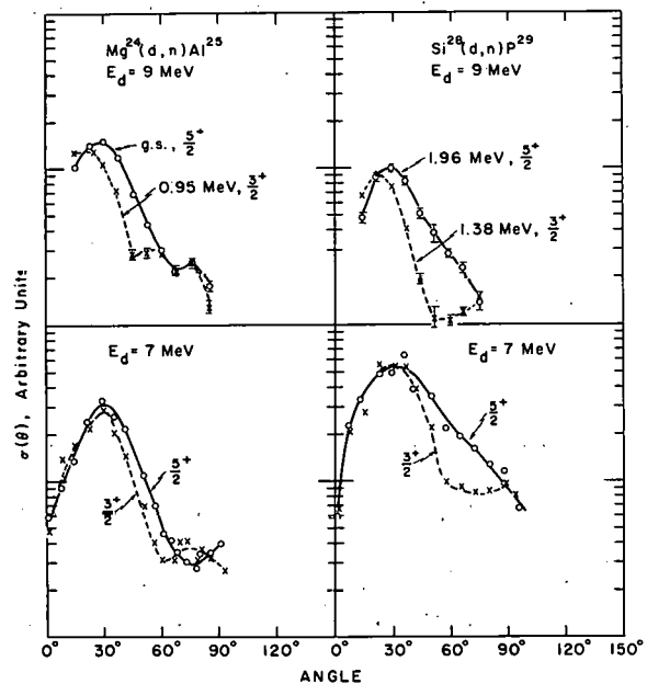
Fig. 12. Differential cross sections for the reactions Mg^{24}(d,n) and Si^{28}(d,n) at 7 and 9 MeV. These illustrate the J dependence for l_p=2 transitions.
