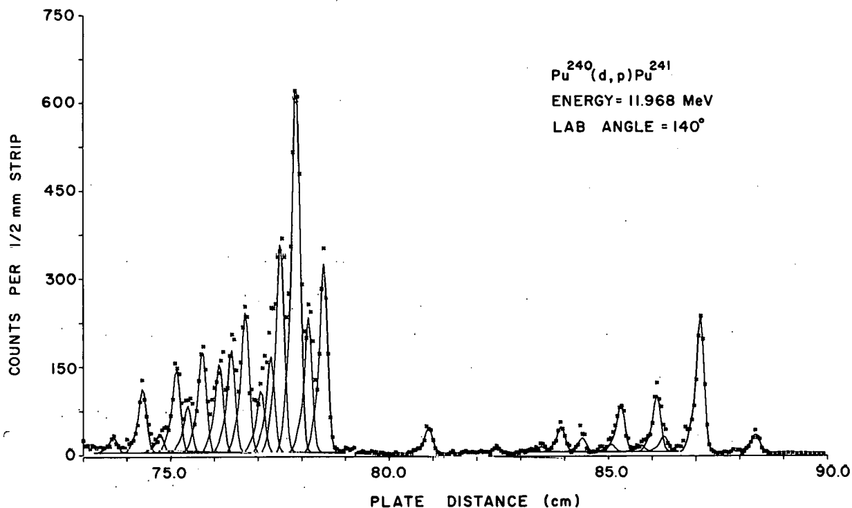
Fig. 19. Spectrum of protons observed at 140° from a \text{Pu}^{240} target bombarded with 11.96-MeV deuterons. (See Sec. I. C. 6. k.) The points are the raw data; the lines represent the best computer fit of the reference peak to the raw data.
