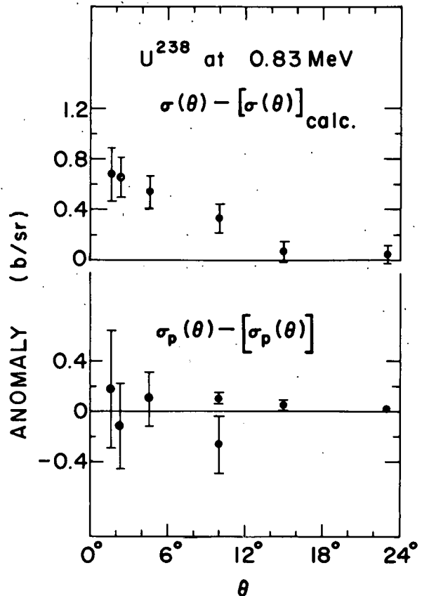
Fig. 26. The difference between the measured and calculated values of the differential and polarization cross sections.
