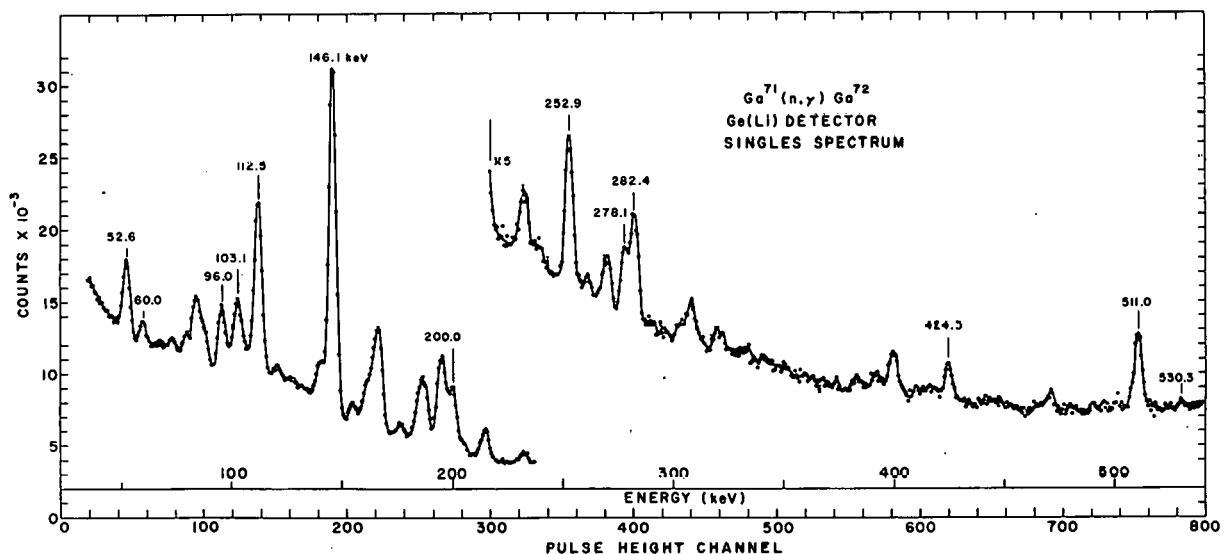
Fig. 2. Typical low-energy gamma-ray spectra in Ga 72 following thermal-neutron capture in Ga 71 .
