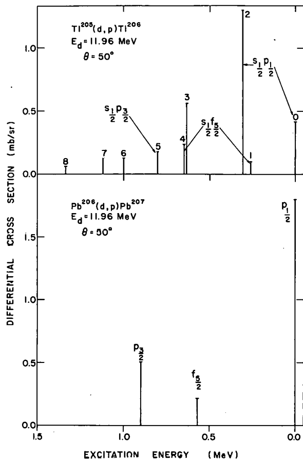
Fig. 18. A comparison of proton spectra from the Tl^{205}(d,p)Tl^{206} and Pb^{206}(d,p)Pb^{207} reactions taken at the same scattering angle and bombarding energy. The data are presented in the form of a bar graph in which the absolute differential cross sections of the reactions leading to the various excited states are plotted on an energy scale at the appropriate excitation energies. The levels are labeled with the configuration assignments discussed in the text.
