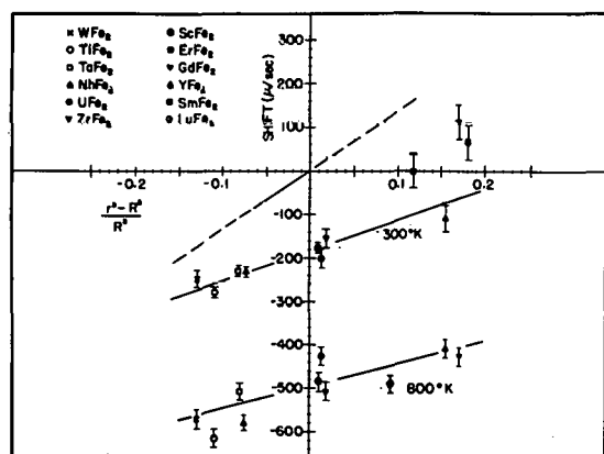
Fig. 28. Shift of the centroid, plotted against fractional change in volume for XFe 2 compounds. Shift and volume change are relative to Fe 57 in a iron. The line passing through the origin is a fit to the high-pressure results (Pipkorn et al.) in a iron. The points taken at 800°K are the most significant for two reasons: First, the shift is insensitive to possible small differences in Debye temperature
