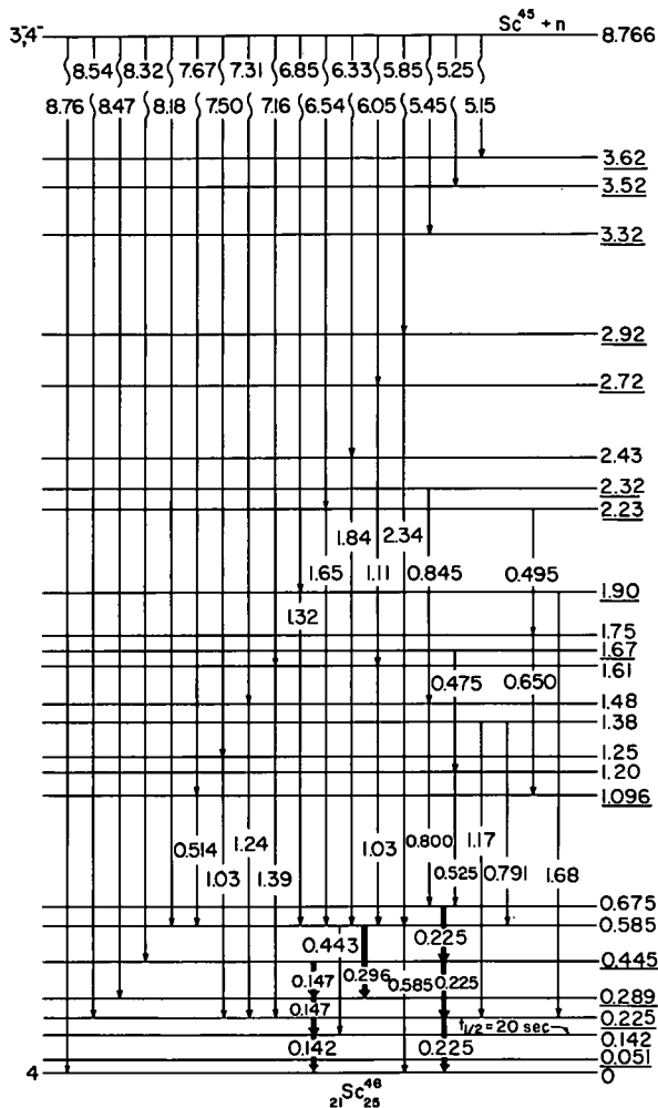
Fig. 1. Proposed decay scheme for levels up to an excitation energy of 3.62 MeV. The underlined excitation energies denote those states observed in previously reported (d,p) reaction studies.
