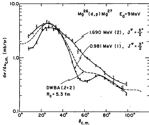
Fig. 15. Angular distributions from the reaction \text{Mg}^{26}(\text{d},\text{p})\text{Mg}^{27} at E_d = 9.0 MeV. The angular distribution (open circles) from the second excited state was multiplied by 1.82.
