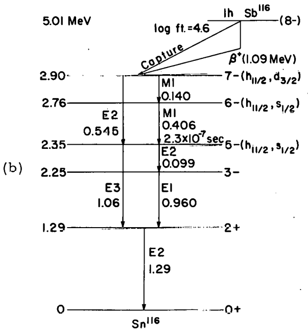
Fig. 23. (a) Systematic trends of the energy levels of the even-A isotopes of Sn: left, experimental; right, theoretical [R. Avieau, thesis, L'Universite de Paris, Institut du Radium, 1962 (unpublished)]. (b) Proposed decay schemes of \text{Sn}^{116} . Left: Transitions following the decay of 54-min \text{In}^{116} . The dashed lines show the pertinent features of the decay scheme of 13-sec \text{In}^{116} [P. Fettweis and J. Vervier, Phys. Letters 3 , 36 (1962)]. Right: Transitions following the decay of 1-hour \text{Sb}^{116} . All energies are in MeV.
