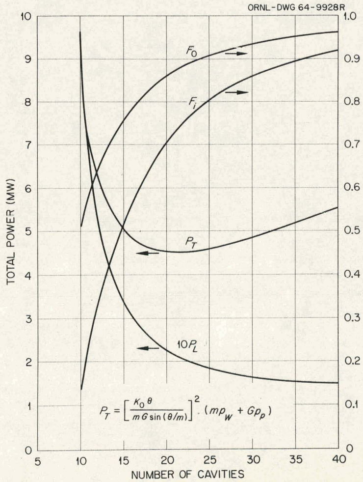
Fig. 4. RF power loss vs number of cavities for a typical SOC.
