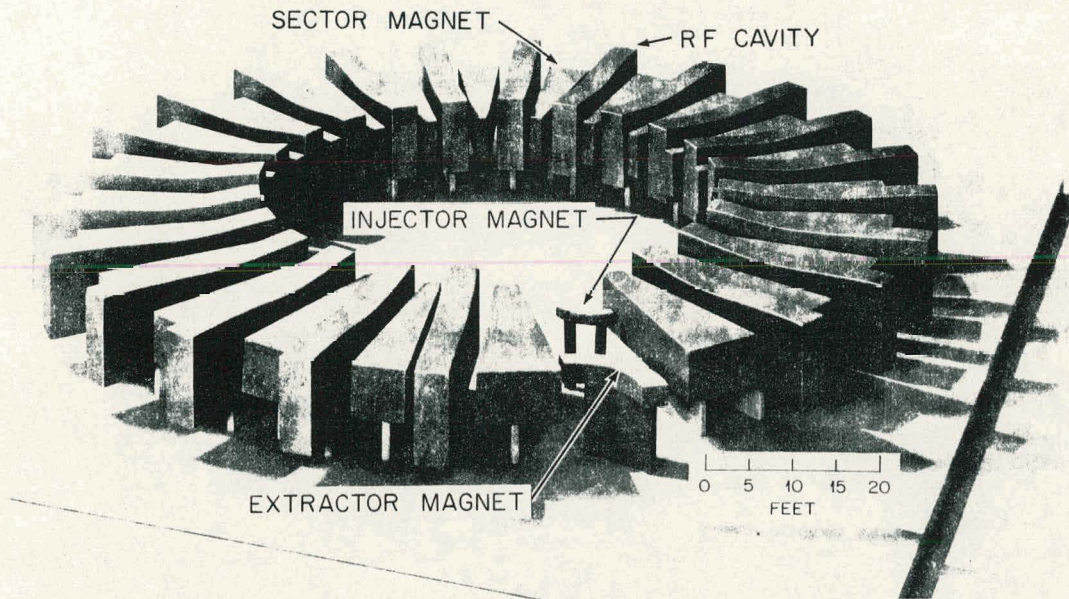
Fig. 1. Conceptual model of an SOC.
