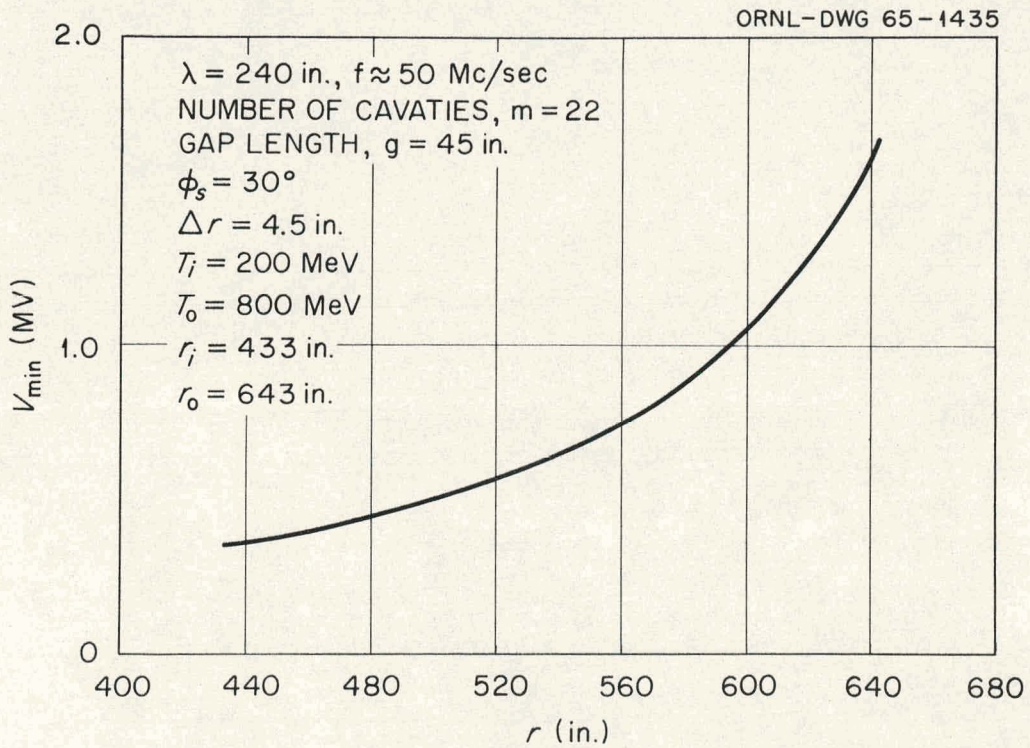
Fig. 2. Minimum accelerating voltage as a function of radius.
