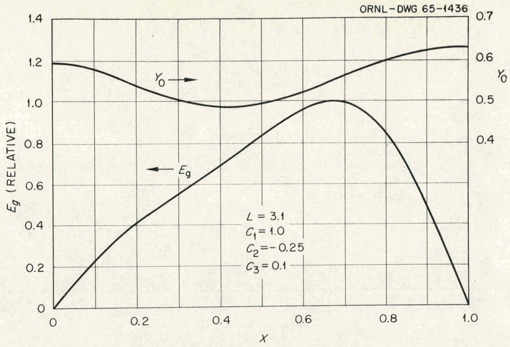
Fig. 3. Height and gap field for a shaped rectangular cavity.
