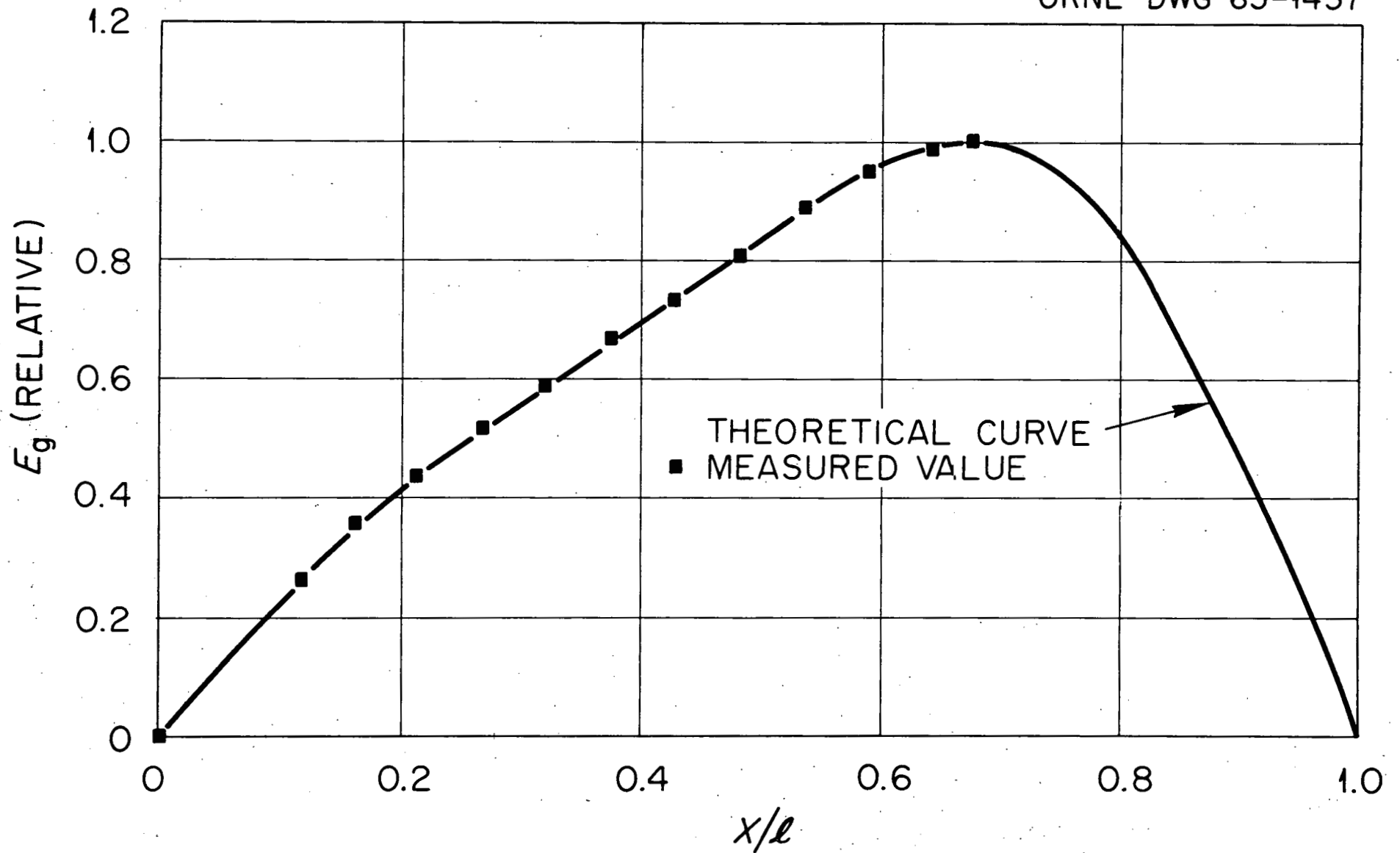
Fig. 7. Measured field in gap of model cavity.
