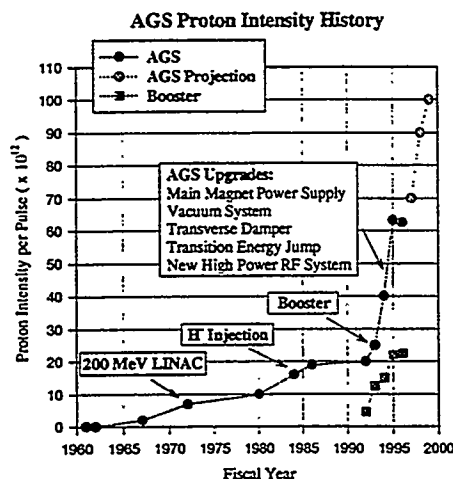
Figure 1: The history of the proton beam intensity in the Brookhaven AGS.
