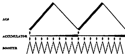
Figure 3: A 1.5 GeV accumulator in the AGS tunnel can be used for both slow-extracted beam (SEB) and fast-extracted beam (FEB) to improve the machine duty cycle. Operation scenarios for these two modes are shown with the thickness of the line indicating the beam intensity.
