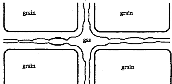
Figure 2c. Formation of open porosity structure.
