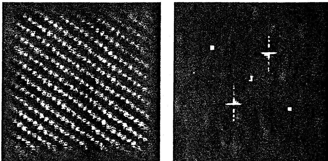
Fig. 2. Image of NiO in the [112] projection with Fourier transform showing transfer down to 1.26\text{\AA} .
