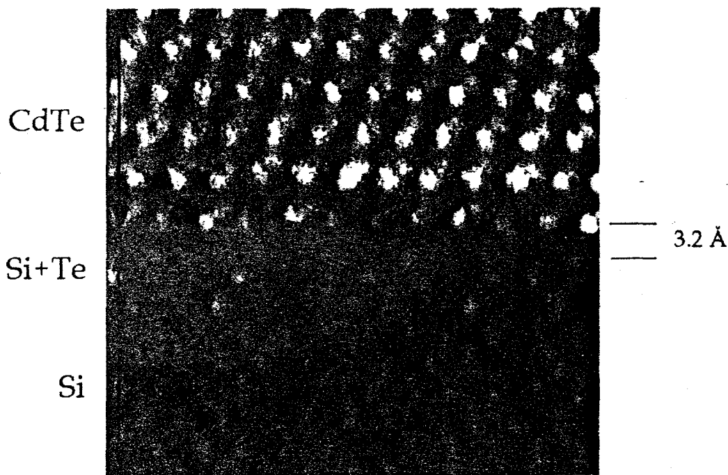
Figure 7. Z-Contrast image of a CdTe(111)/Si(100) interface showing its incommensurate nature.
