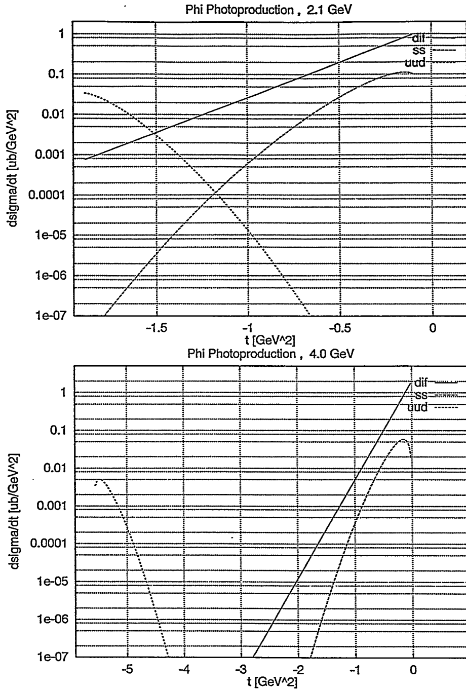
Figure 2: Cross-sections for \phi production at 2.1 and 4.0 GeV. Contributions from 3 mechanisms are shown: diffractive, s\bar{s} knockout, and u\bar{u}d knockout. The knockout is from the theory and calculations of Ref. [7]. The diffractive is based on the experimental cross-sections of H. J. Besch, et al. [8] at 2.1 GeV, and of H. -J. Behrend, et al. [9], at 4.0 GeV.
