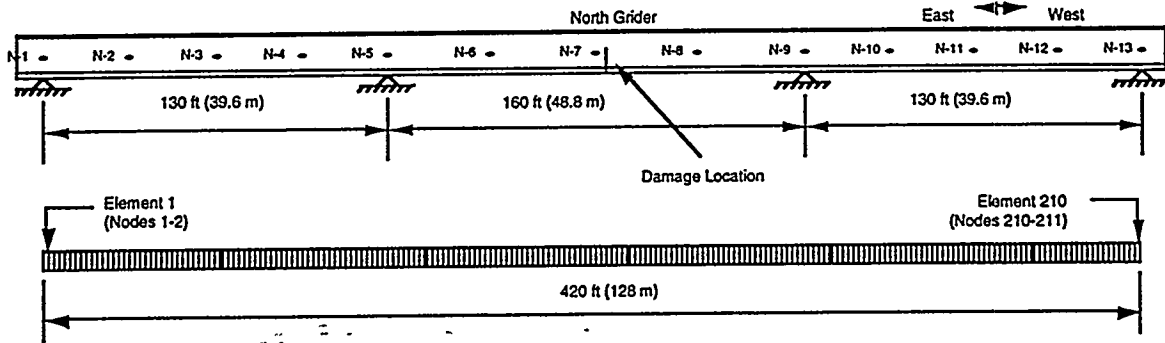
Figure 4. Coarse accelerometer locations.
