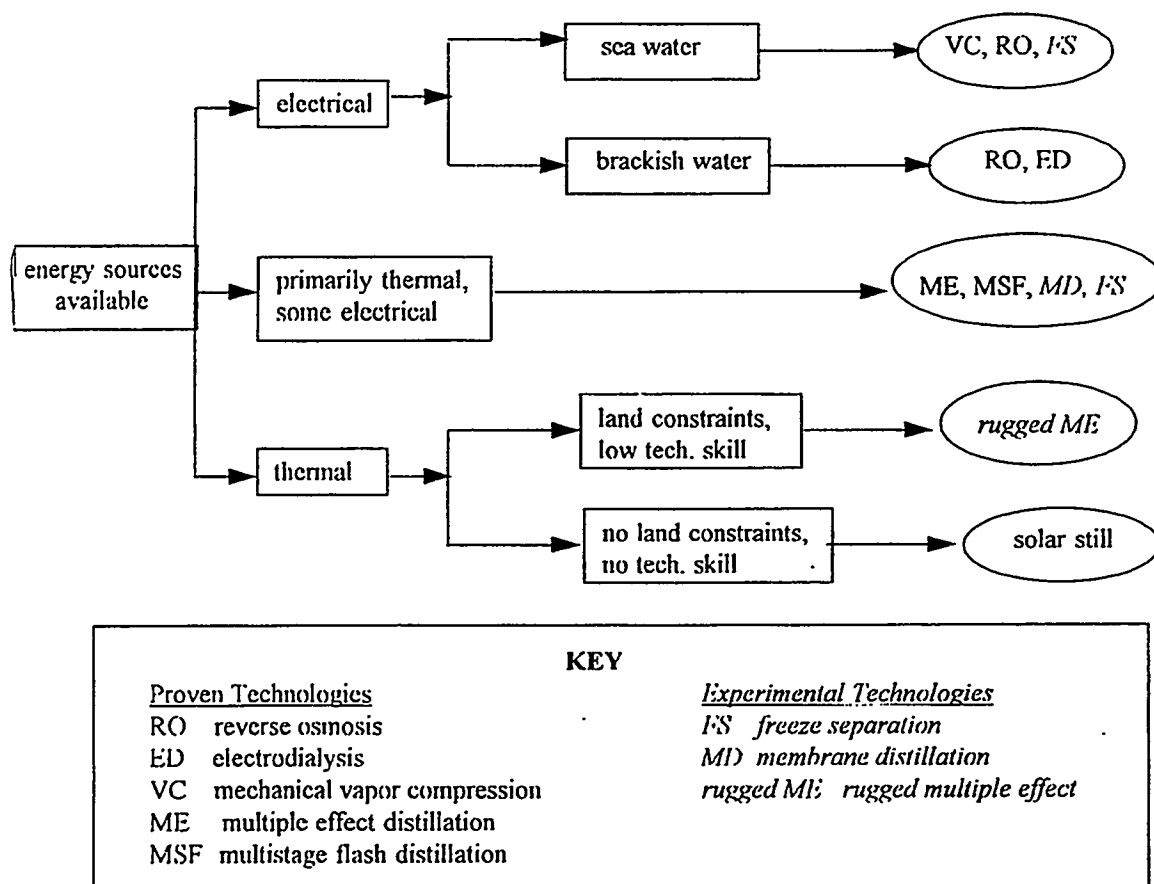
Figure 10: Choosing the Appropriate Desalination Technology (Thomas, in press)
