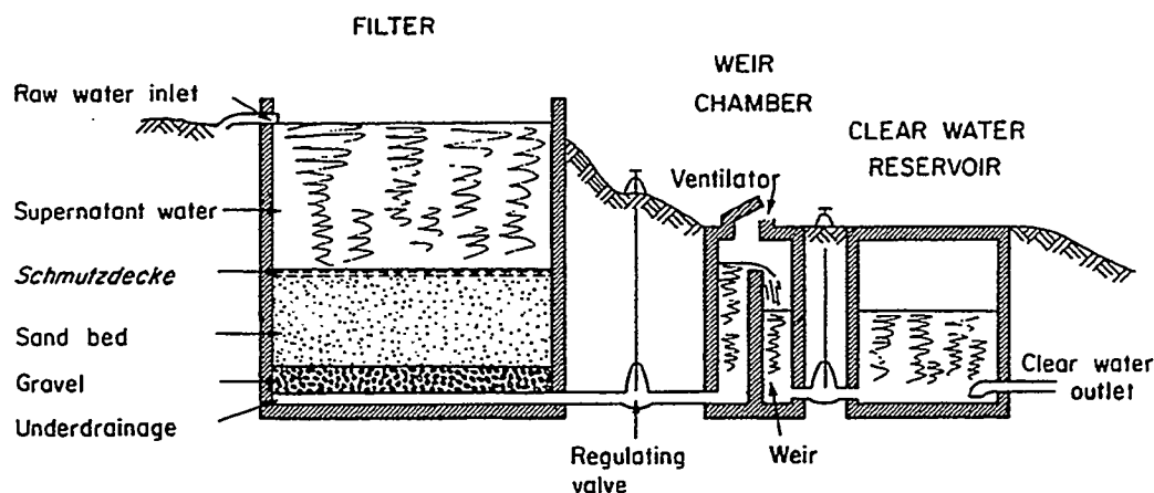
Figure 8: Slow Sand Filter (Pickford 1978)
