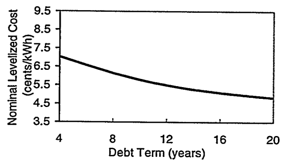
Figure 3-8. Impact of Debt Term on Wind Power Costs
