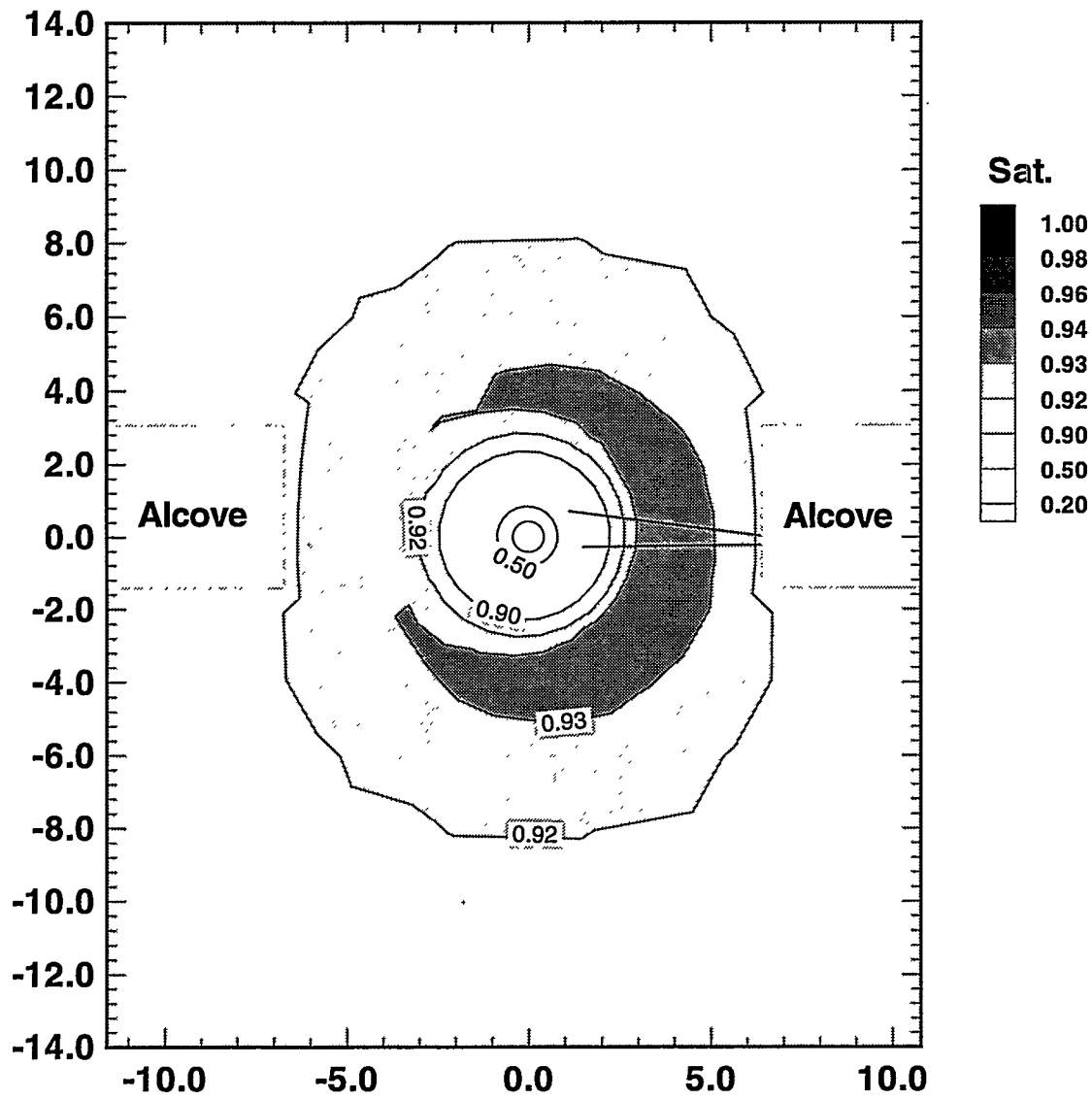
Figure 4.2-13 Equivalent continuum liquid saturation for Base Case at 15 months after 1 year heating period in XZ - cross section at Y = 4.25 m.
