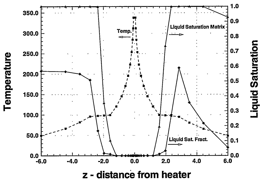
Figure 6.6-4 Temperature / liquid saturation for case with low matrix permeability in 2D - simulation at 1 year along Z - axis at X = 0.0 m.
