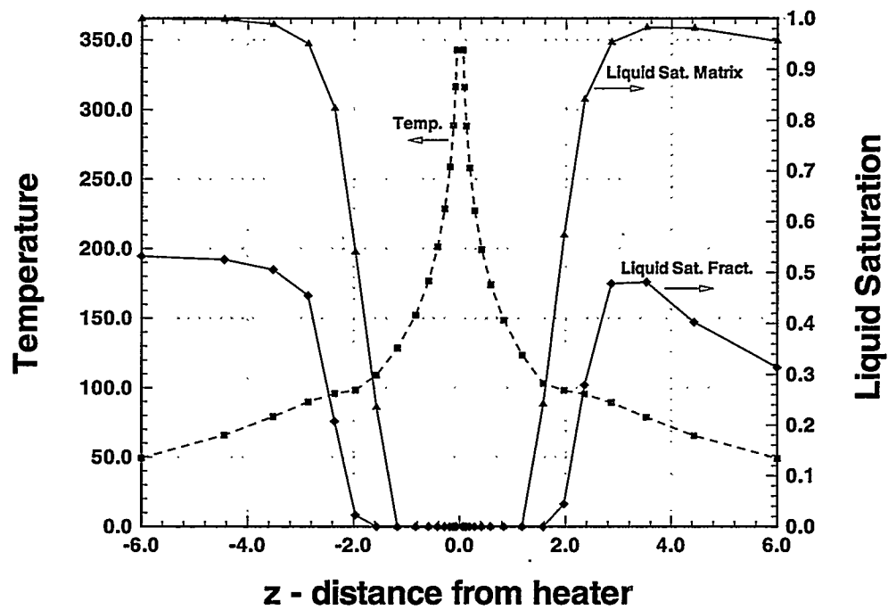
Figure 6.4-4 Temperature / liquid saturation for dual-permeability model in 2D - simulation at 1 year along Z - axis at X = 0.0 m.
