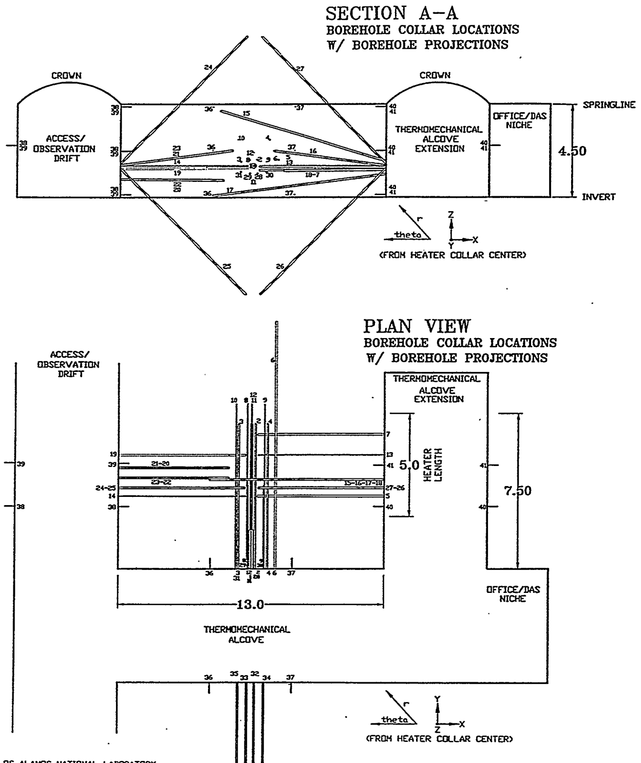
Figure 3.1-1 Layout and borehole arrangement in the Single Heater Test.
