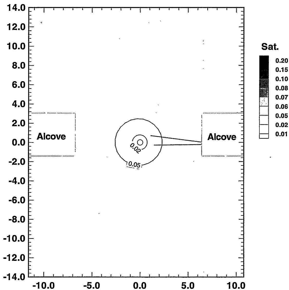
Figure 4.2-16 Fracture liquid saturation for Base Case at 15 months after 1 year heating period in XZ - cross section at Y = 4.25 m.
