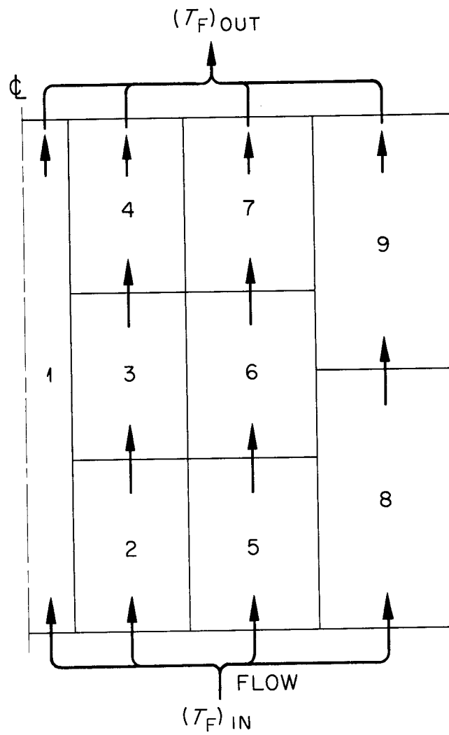
Fig. 5. Schematic Diagram of Nine-Region Core Model.
