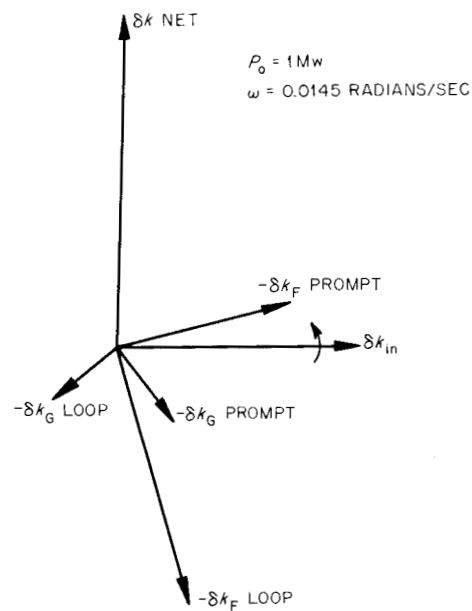
Fig. 17. Directed-Line Diagrams of Reactivity Feedback Effects at 1 and 10 Mw for Complete Model.
