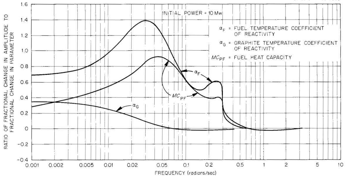
Fig. 18. Frequency-Response Sensitivities of Complete Model.
