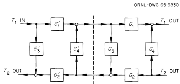
Fig. A.3. Diagram for Computing Transfer Functions for Two Lumps in Series.
