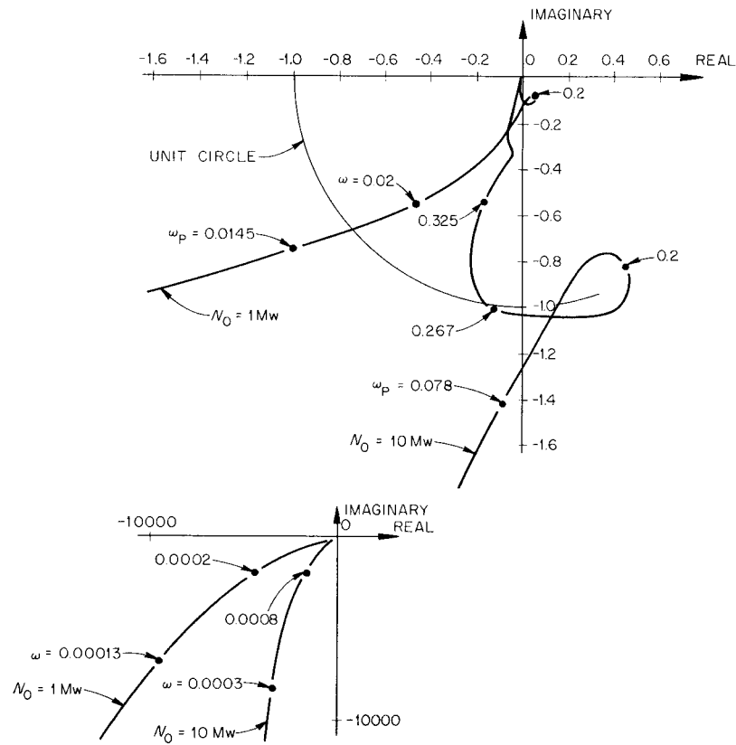
Fig. 12. Nyquist Diagrams for Complete Model N_0 = 1 and 10 Mw.
