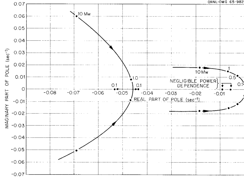
Fig. 13. Major Poles for the MSRE.
