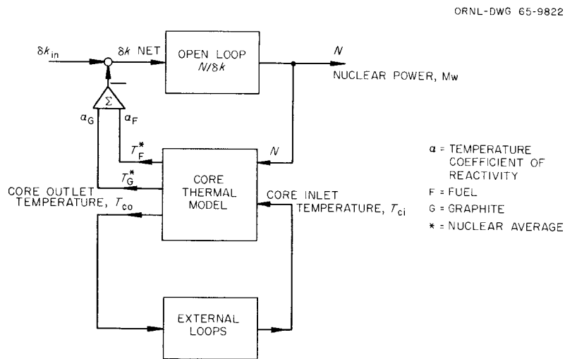
Fig. 14. MSRE as Closed-Loop Control System.
