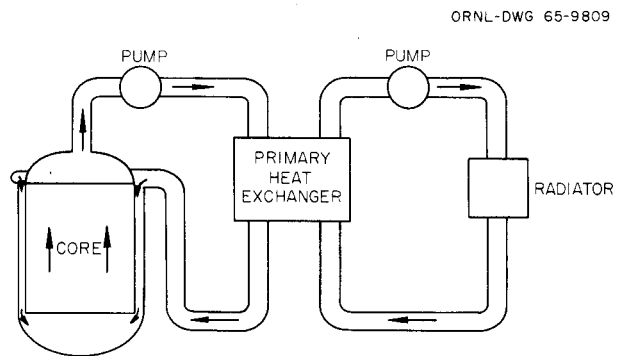
Fig. 1. MSRE Basic Flow Diagram.
