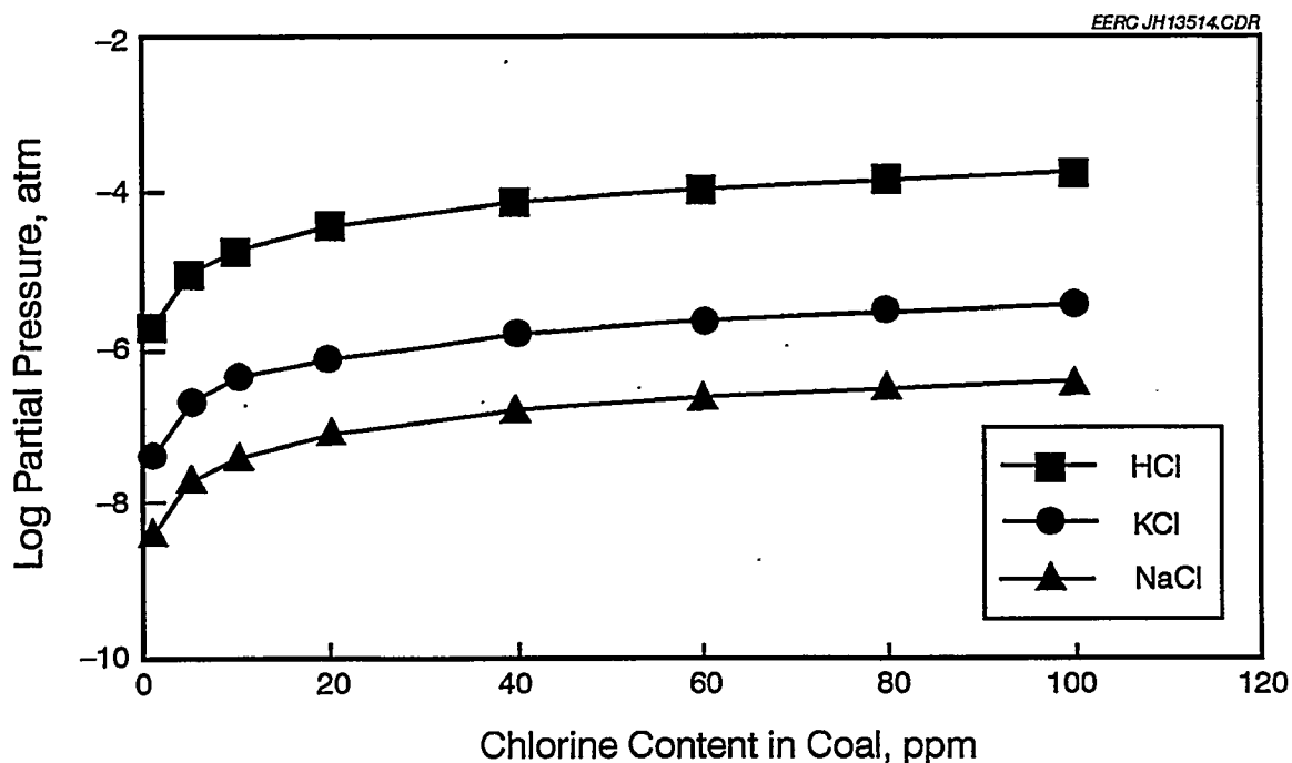
Figure 8. The calculated concentrations of major vapor-phase chloride species in the fluid bed of the Piñon Pine system as a function of the chlorine content of the coal.
