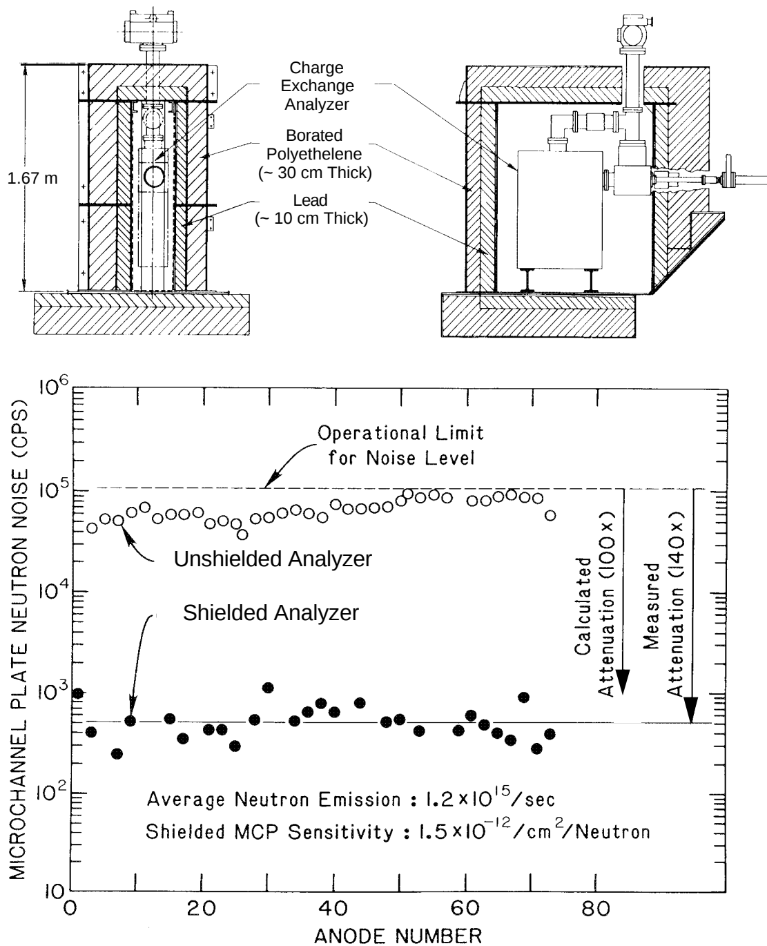
Fig.11 Schematic of the radiation shield for the TFTR E||B spectrometer (top) and comparison of the background neutron and gamma noise levels obtained for the shielded and unshielded analyzers (bottom).
