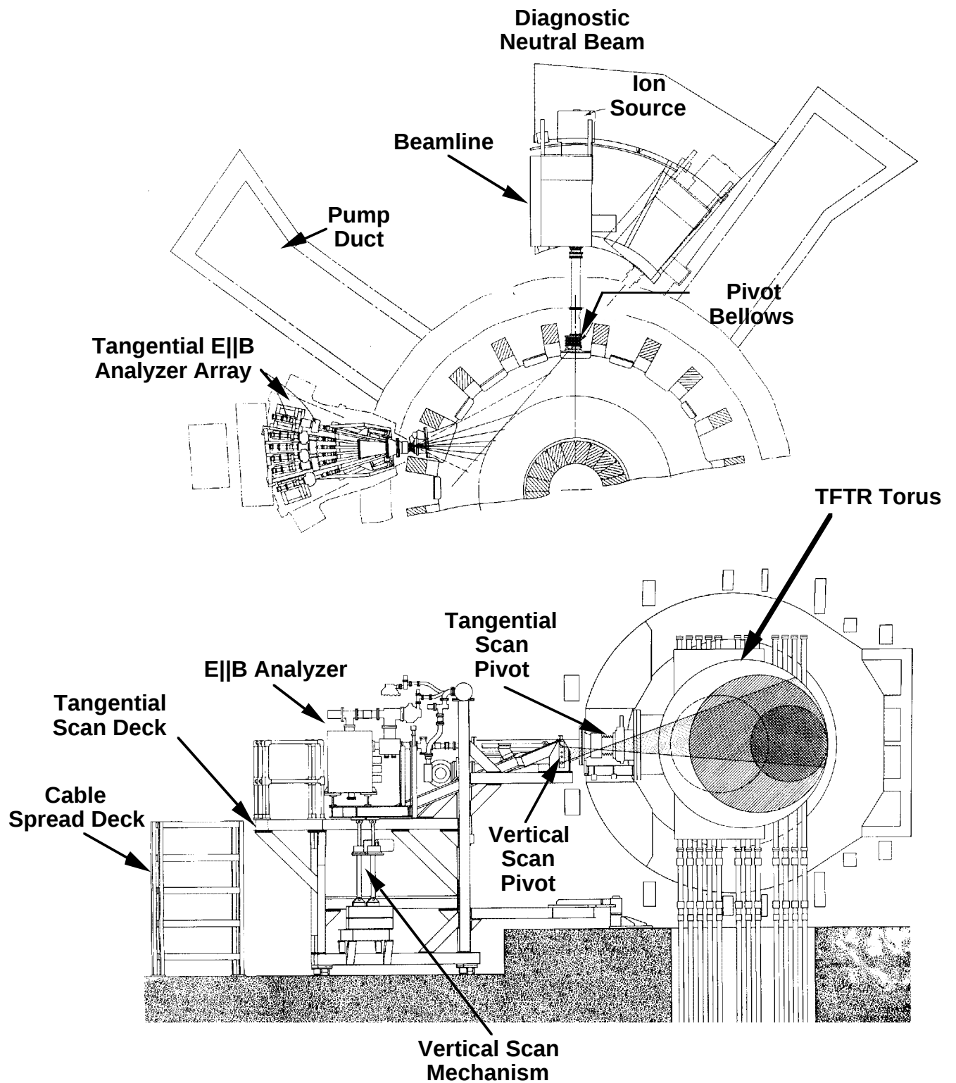
Fig. 14 Layout of the tangential charge exchange array on TFTR in plan (top) and elevation (bottom) views.
