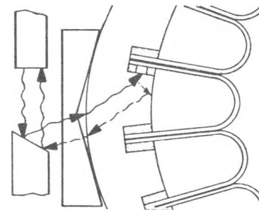
Bad Bond (On One Side of Joint): Signal Shear Wave at Unbonded Braze Echos Back to Transducer
