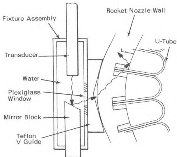
Good Bond: Signal Through Bonded Section Continues On
