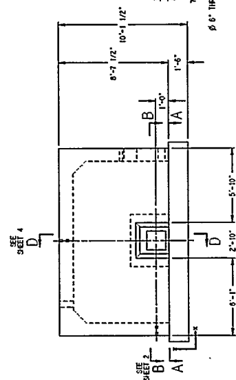
WEST ELEVATION SCALE 1/2"=1'-0"
