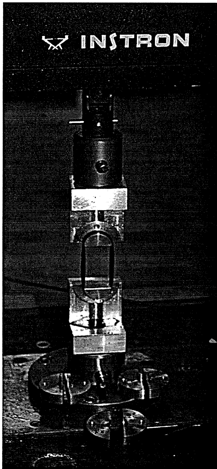
Figure 3. Insert mount and split-spool, interchangeable fixtures for O-ring tensile testing. Insert and split spools fabricated according to Sandia drawings.
