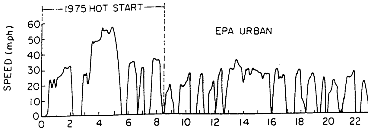
Figure 3.4. Urban Driving Cycle
