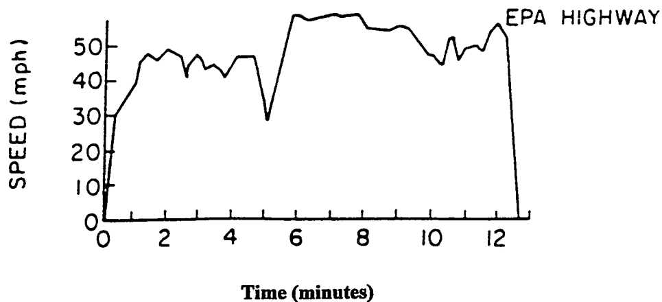
Figure 3.5. Highway Driving Cycle
