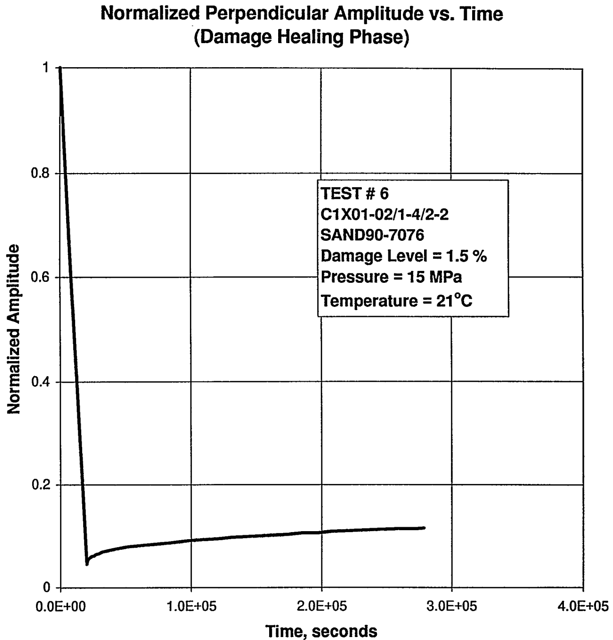
Figure E-103. Normalized Perpendicular Amplitude as a Function of Time During the Hydrostatic Loading to Recover Damage in Specimen C1X01-02/1-4/2-2.
