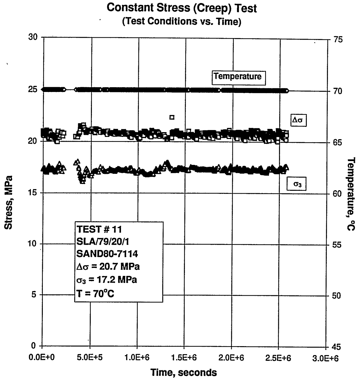
Figure B-63. Test Conditions Versus Time for a Creep Test: Specimen SLA/79/20/1; Stage 1 of 1.
