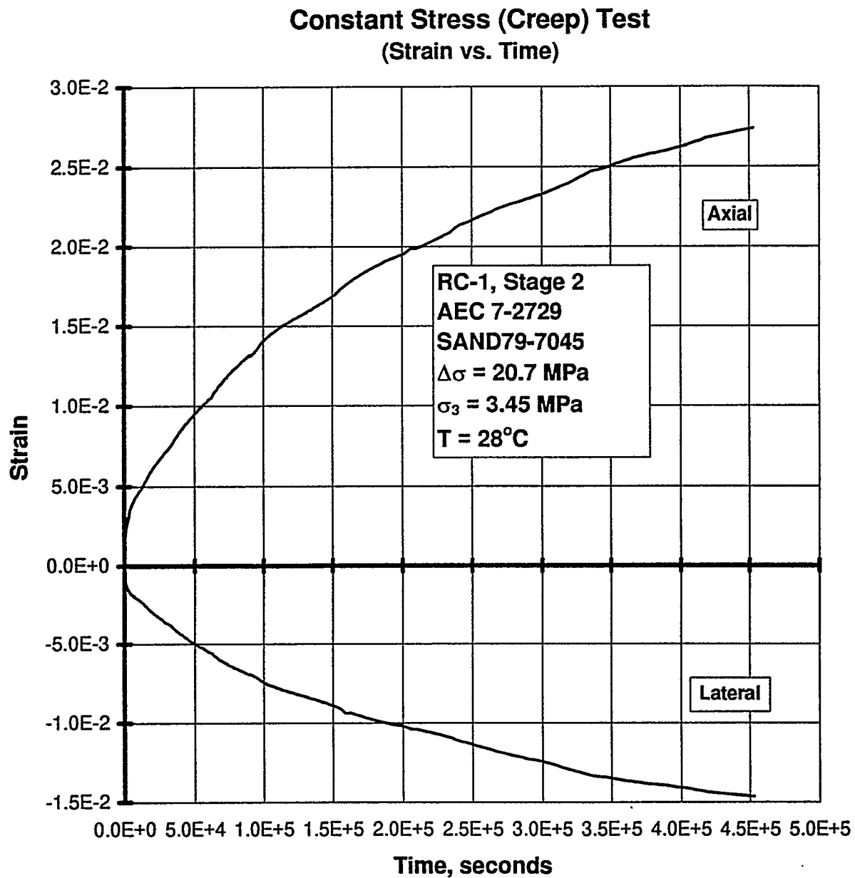
Figure B-150. Axial Strain and Lateral Strain Versus Time for a Creep Test: Specimen AEC7-2729; Stage 2 of 3.
