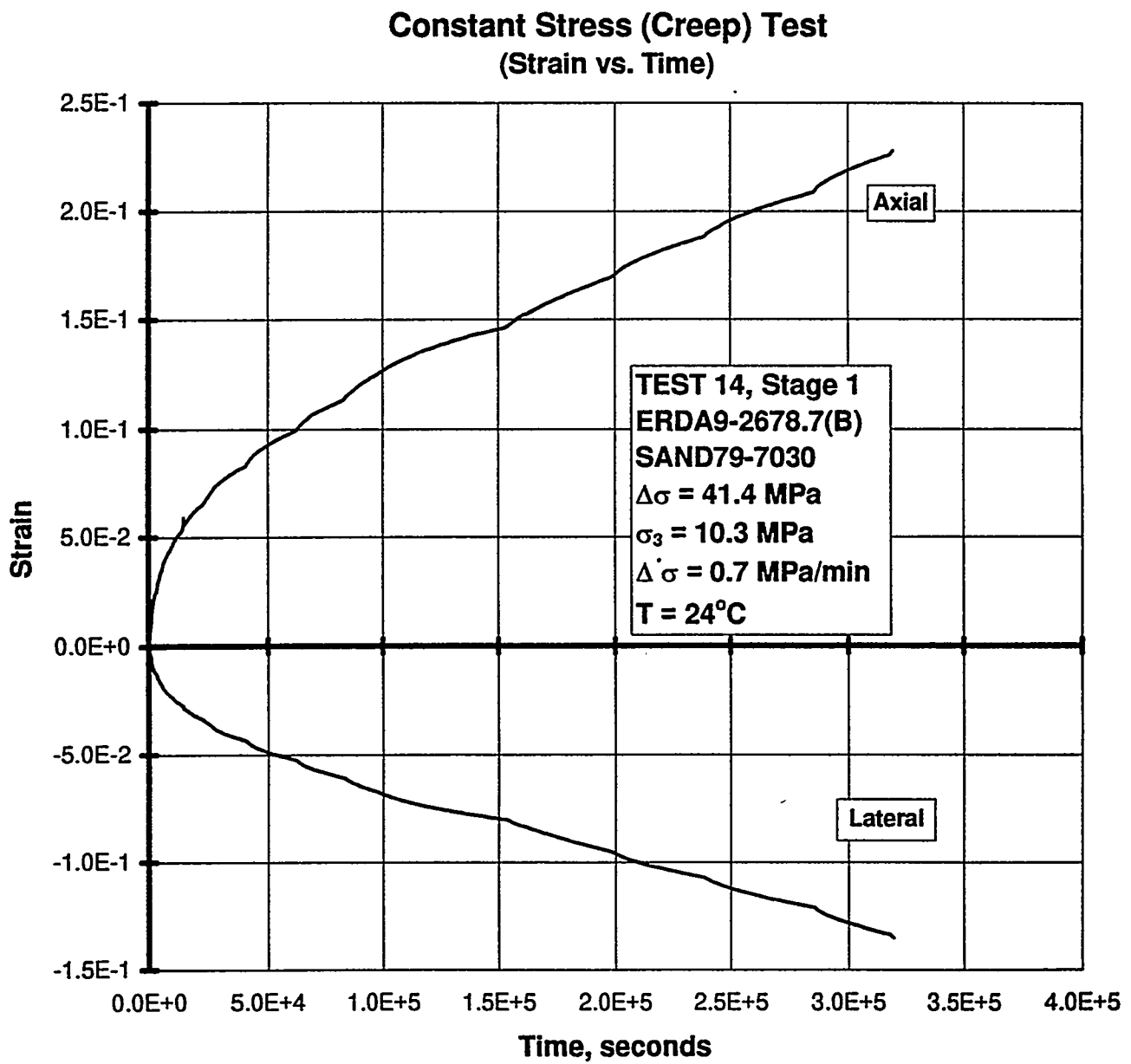
Figure B-142. Axial Strain and Lateral Strain Versus Time for a Creep Test: Specimen ERDA9-2678.7 (B); Stage 1 of 1.
