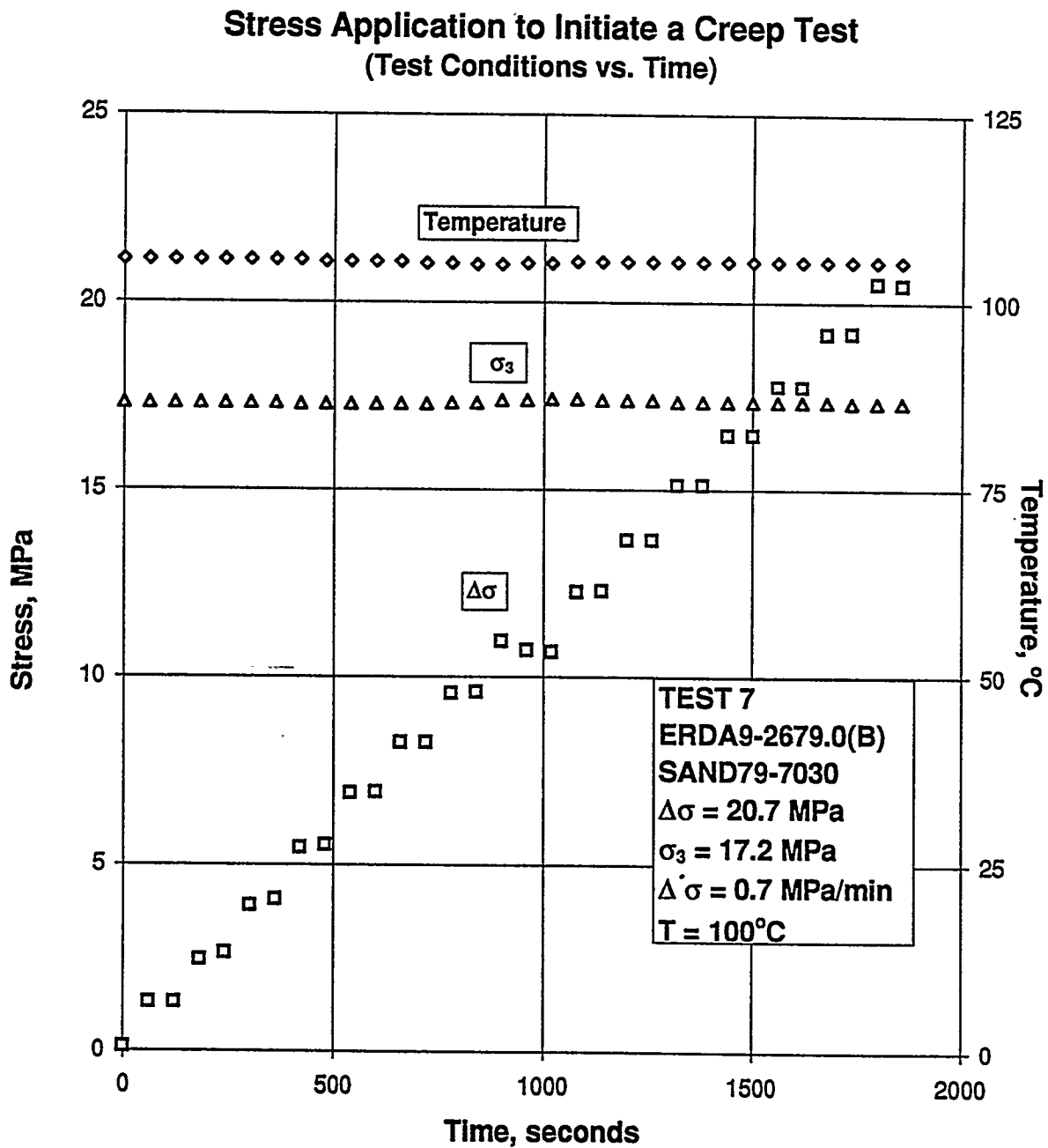
Figure B-97. Test Conditions Versus Time for Stress Application to Initiate a Creep Test: Specimen ERDA9-2679.0 (B); Stage 1 of 1.
