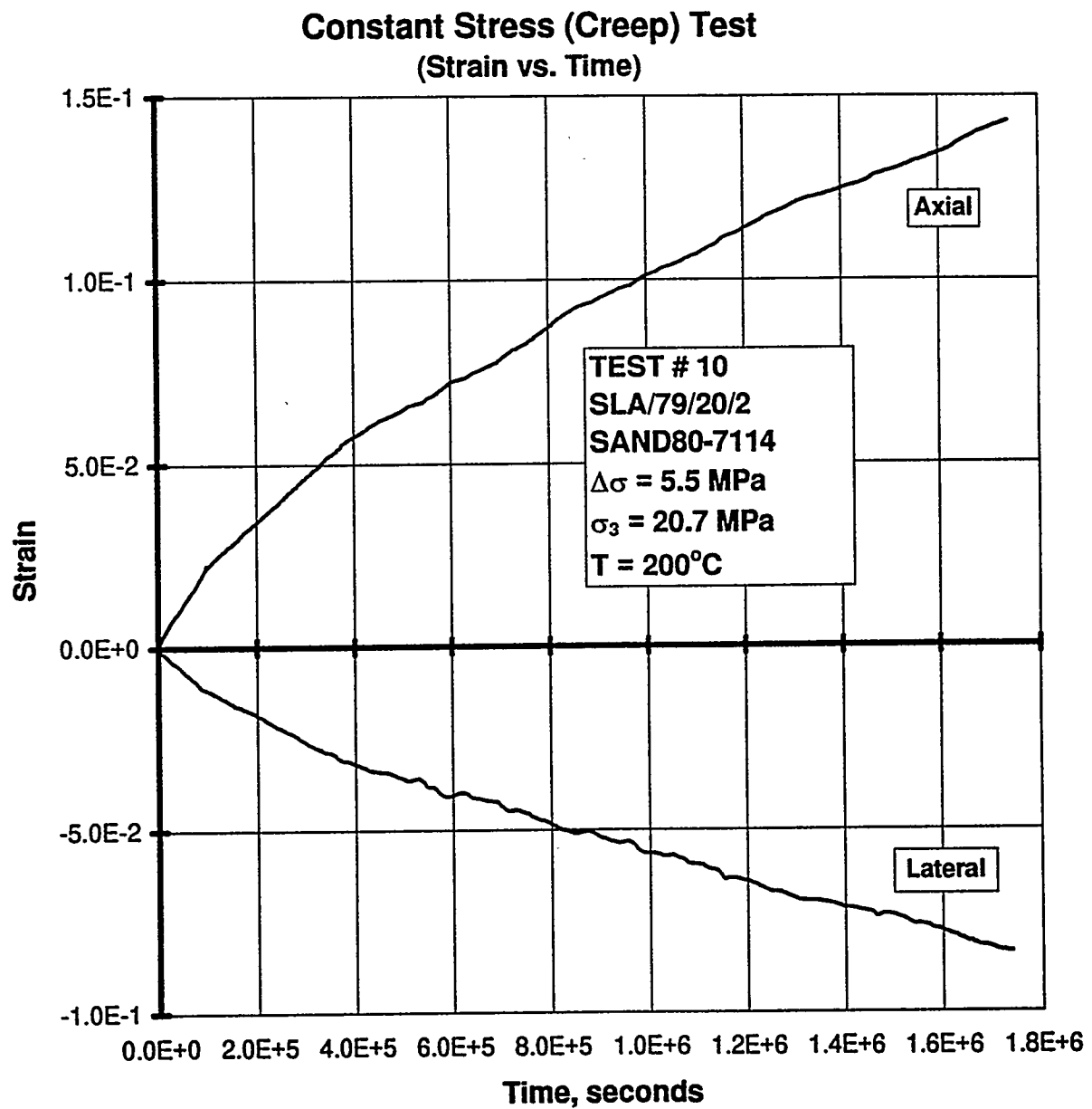
Figure B-60. Axial Strain and Lateral Strain Versus Time for a Creep Test: Specimen SLA/79/20/2; Stage 1 of 1.
