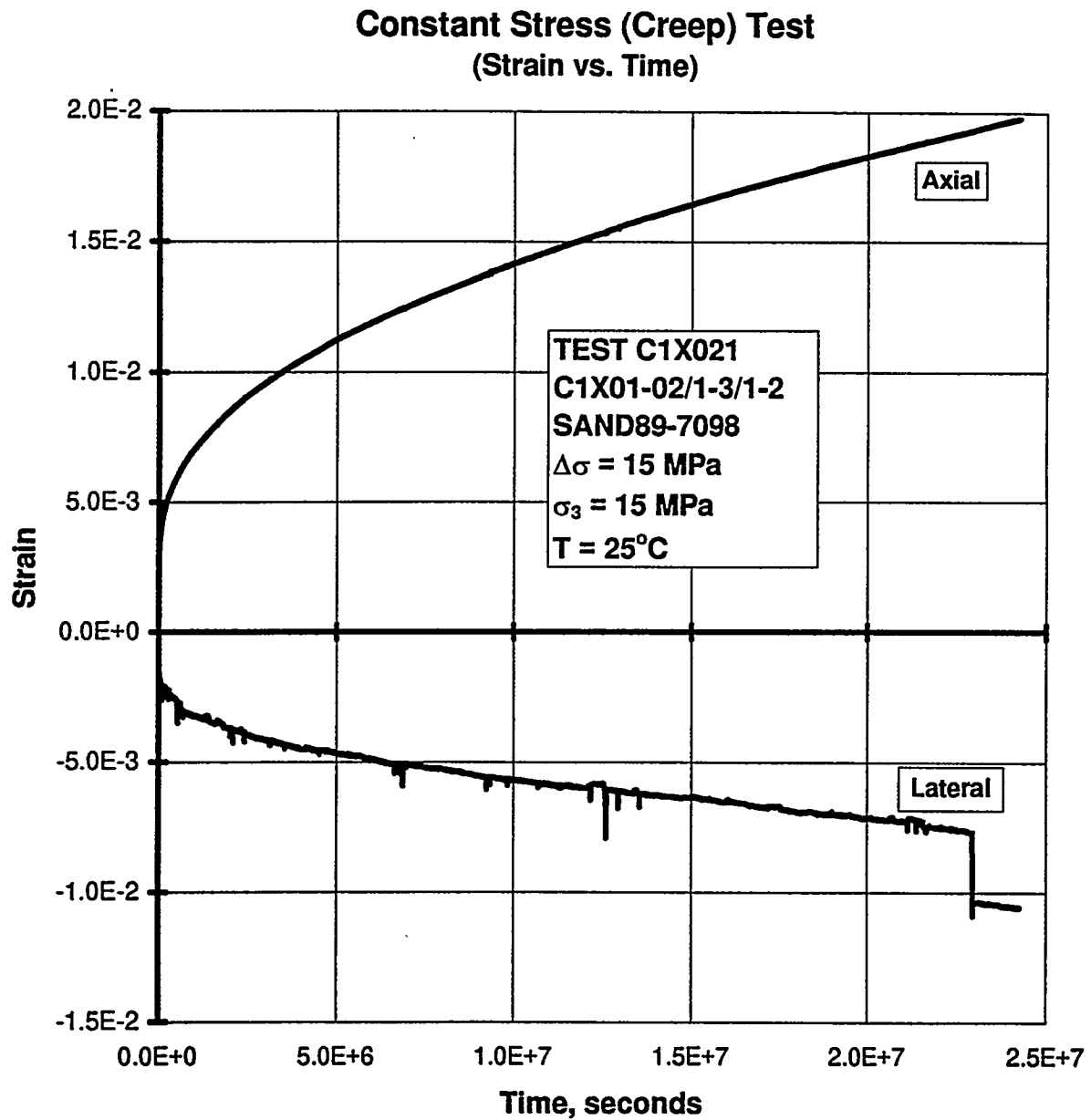
Figure C-36. Axial Strain and Lateral Strain Versus Time for a Creep Test: Specimen C1X01-02/1-3/1-2; Stage 1 of 1.
