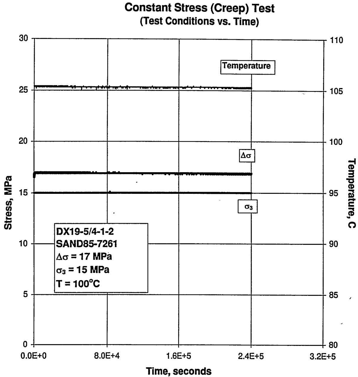
Figure C-81. Test Conditions Versus Time for a Creep Test: Specimen DX19-5/4-1-2; Stage 1 of 1.
