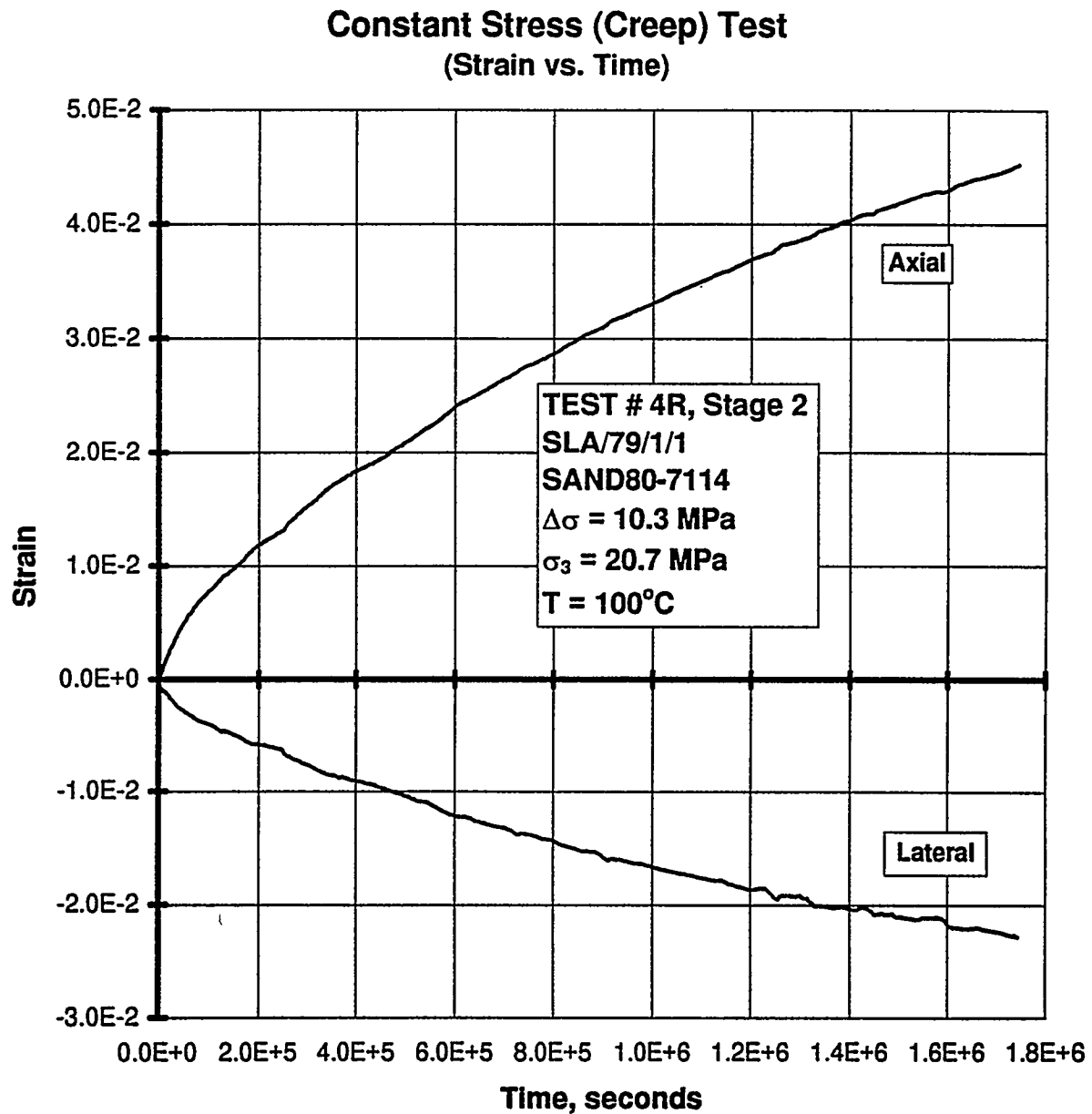
Figure B-36. Axial Strain and Lateral Strain Versus Time for a Creep Test: Specimen SLA/79/1/1; Stage 2 of 2.
