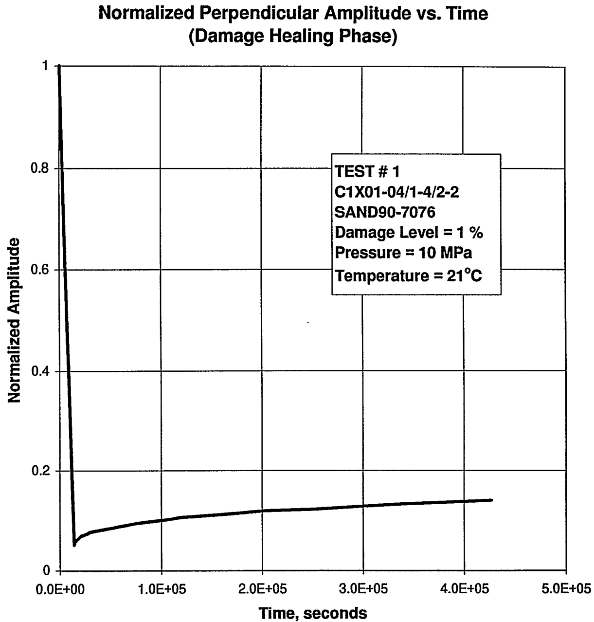
Figure E-43. Normalized Perpendicular Amplitude as a Function of Time During the Hydrostatic Loading to Recover Damage in Specimen C1X01-04/1-4/2-2.
