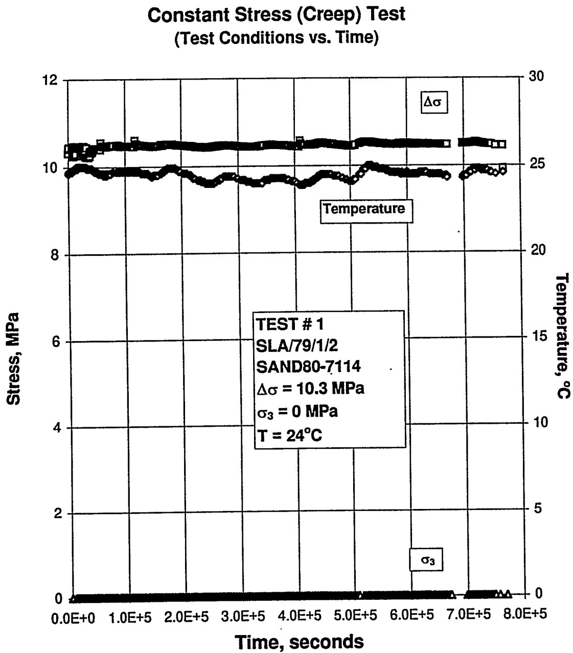
Figure B-9. Test Conditions Versus Time for a Creep Test: Specimen SLA/79/1/2; Stage 1 of 1.
