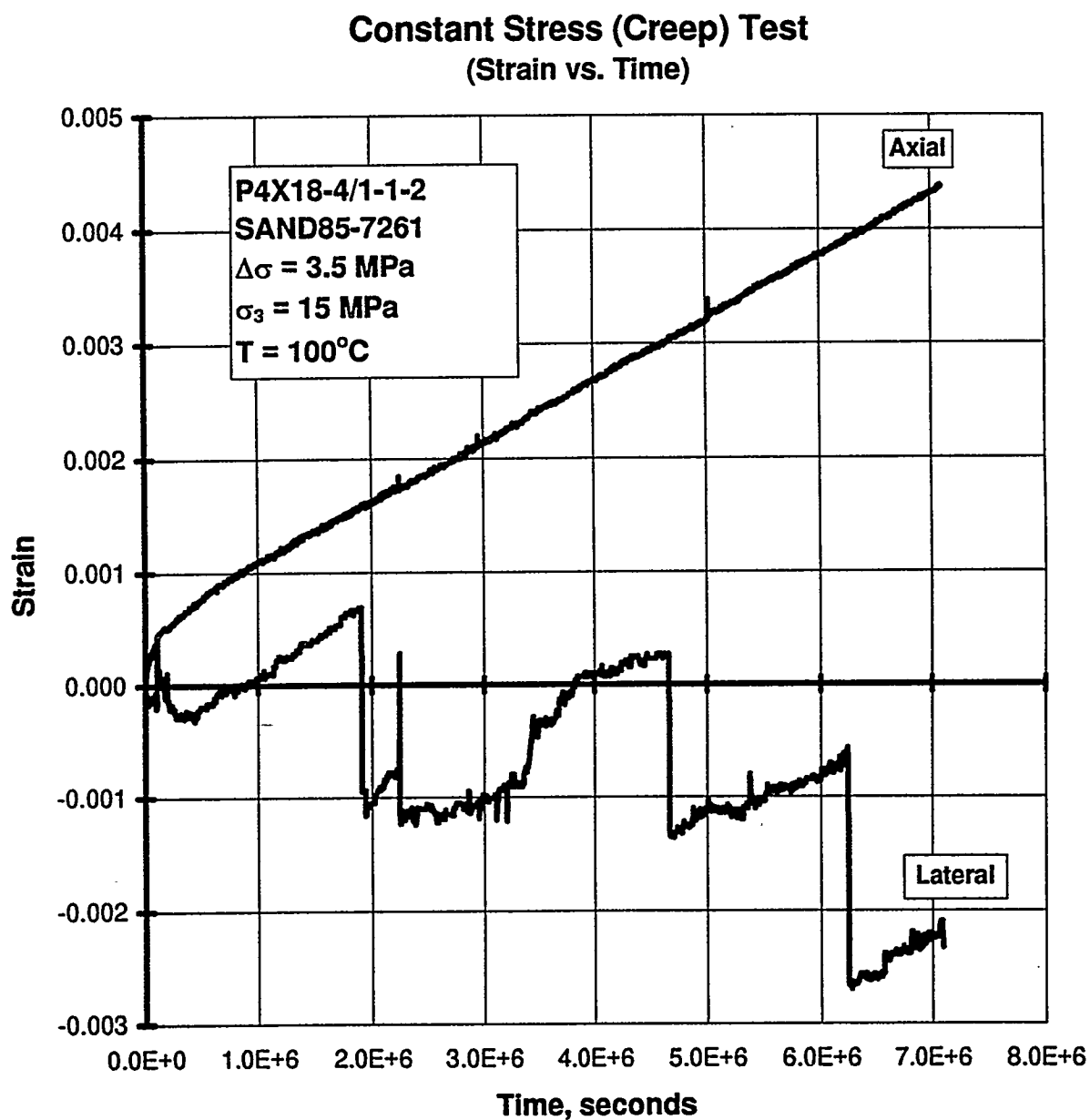
Figure C-48. Axial Strain and Lateral Strain Versus Time for a Creep Test: Specimen P4X18-4/1-1-2; Stage 1 of 1 (Argillaceous Salt).
