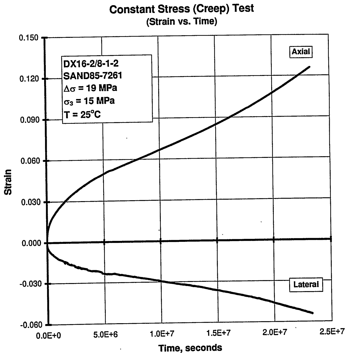
Figure C-66. Axial Strain and Lateral Strain Versus Time for a Creep Test: Specimen DX16-2/8-1-2; Stage 1 of 1.
