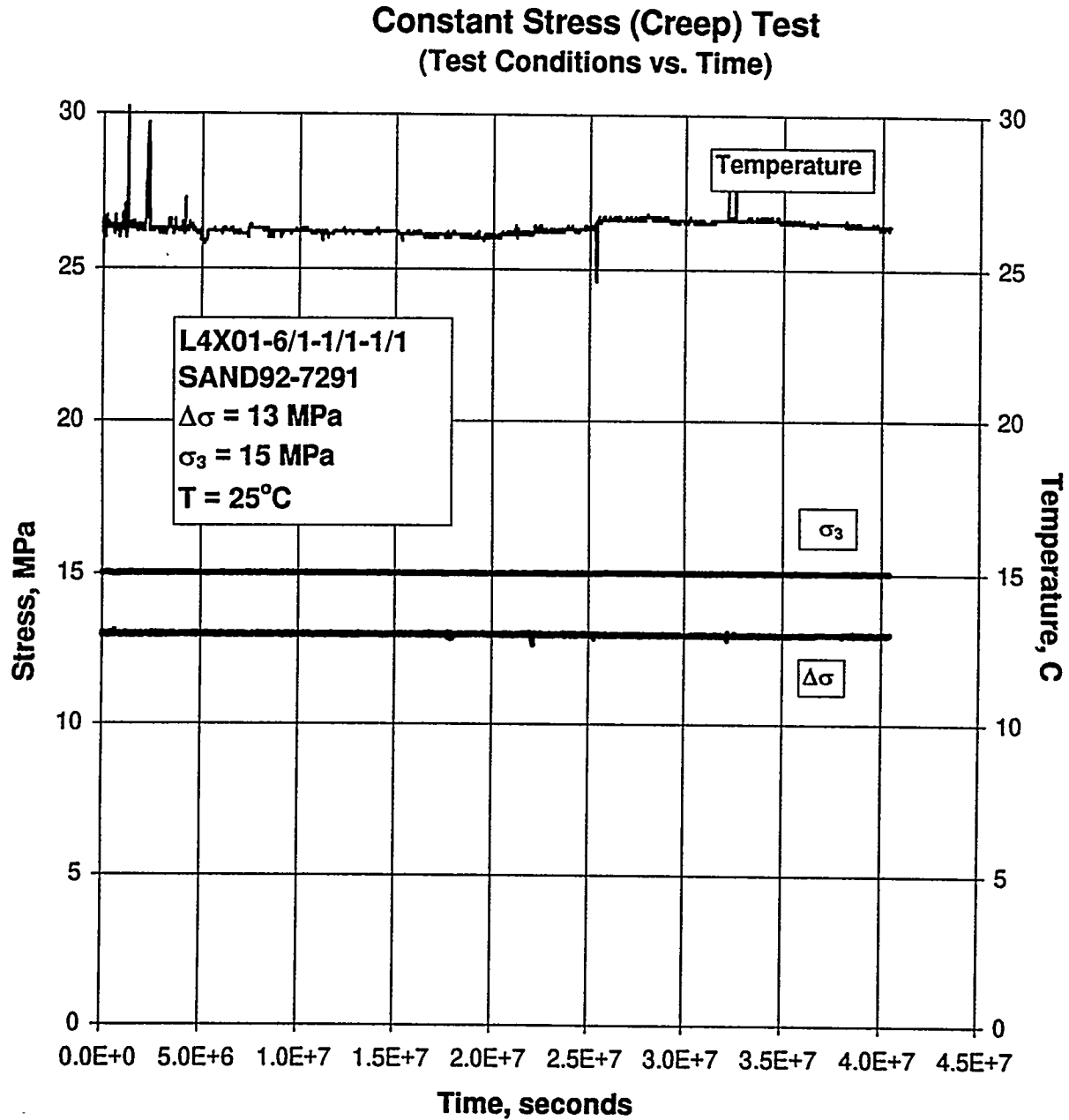
Figure C-19. Test Conditions Versus Time for a Creep Test: Specimen L4X01-6/1-1/1-1/1; Stage 1 of 1 (Argillaceous Salt).
