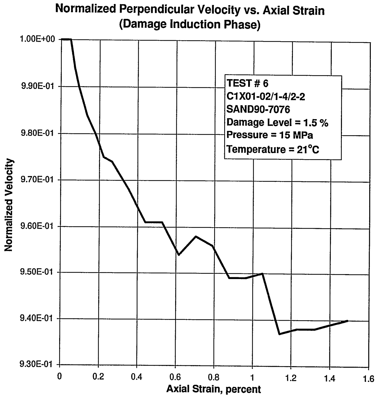
Figure E-99. Normalized Perpendicular Velocity as a Function of Axial Strain During the Quasi-Static Loading to Induce Damage in Specimen C1X01-02/1-4/2-2.
