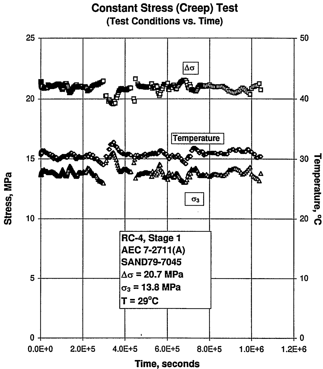
Figure B-177. Test Conditions Versus Time for a Creep Test: Specimen AEC7-2711 (A); Stage 1 of 2.
