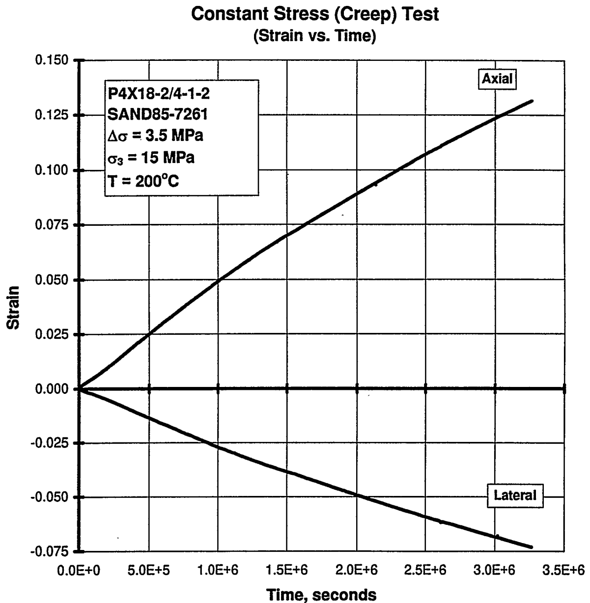
Figure C-54. Axial Strain and Lateral Strain Versus Time for a Creep Test: Specimen P4X18-2/4-1-2; Stage 1 of 1 (Argillaceous Salt. Anomalous Test Result. Possible Moisture Effects).
