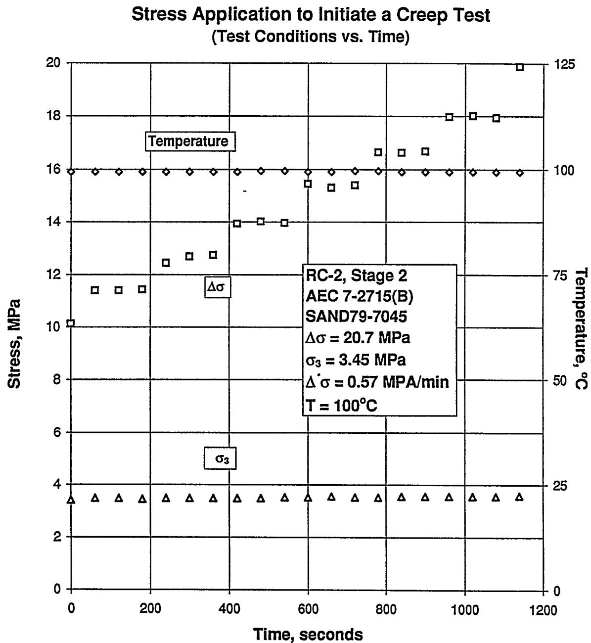
Figure B-159. Test Conditions Versus Time for Stress Application to Initiate a Creep Test: Specimen AEC7-2715 (B); Stage 2 of 2.
