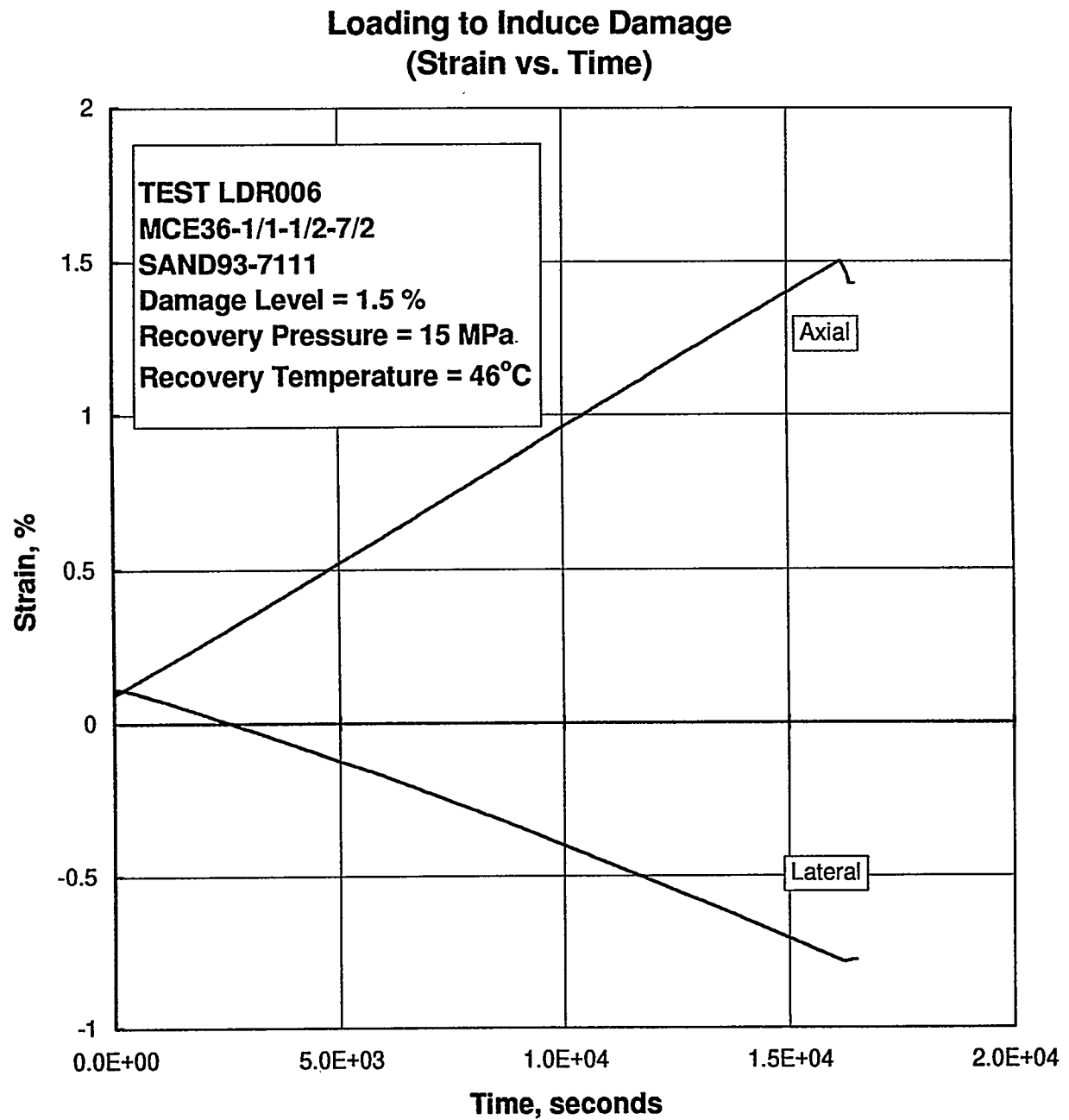
Figure E-30. Axial and Lateral Strain as a Function of Time During the Quasi-Static Loading to Induce Damage in Specimen MCE36-1/1-1/2-7/2.
