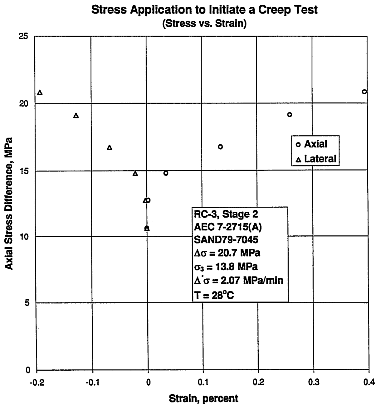
Figure B-168. Axial Stress Difference Versus Axial and Lateral Strain for Stress Application to Initiate a Creep Test: Specimen AEC7-2715 (A); Stage 2 of 3.
