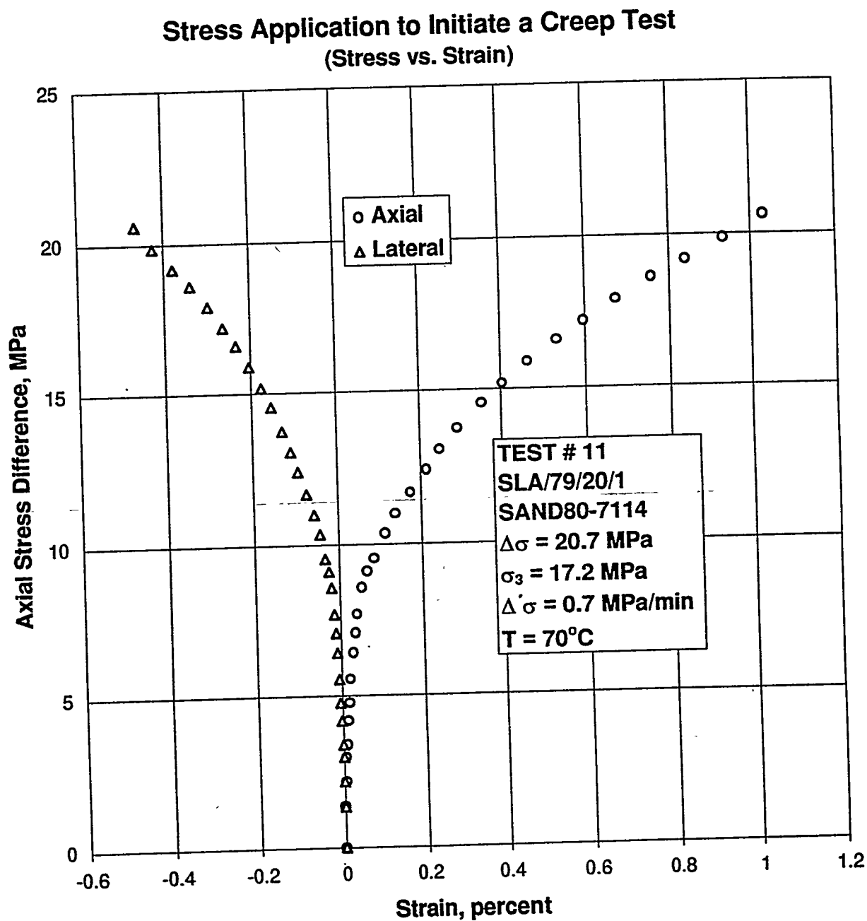
Figure B-62. Axial Stress Difference Versus Axial and Lateral Strain for Stress Application to Initiate a Creep Test: Specimen SLA/79/20/1; Stage 1 of 1.
