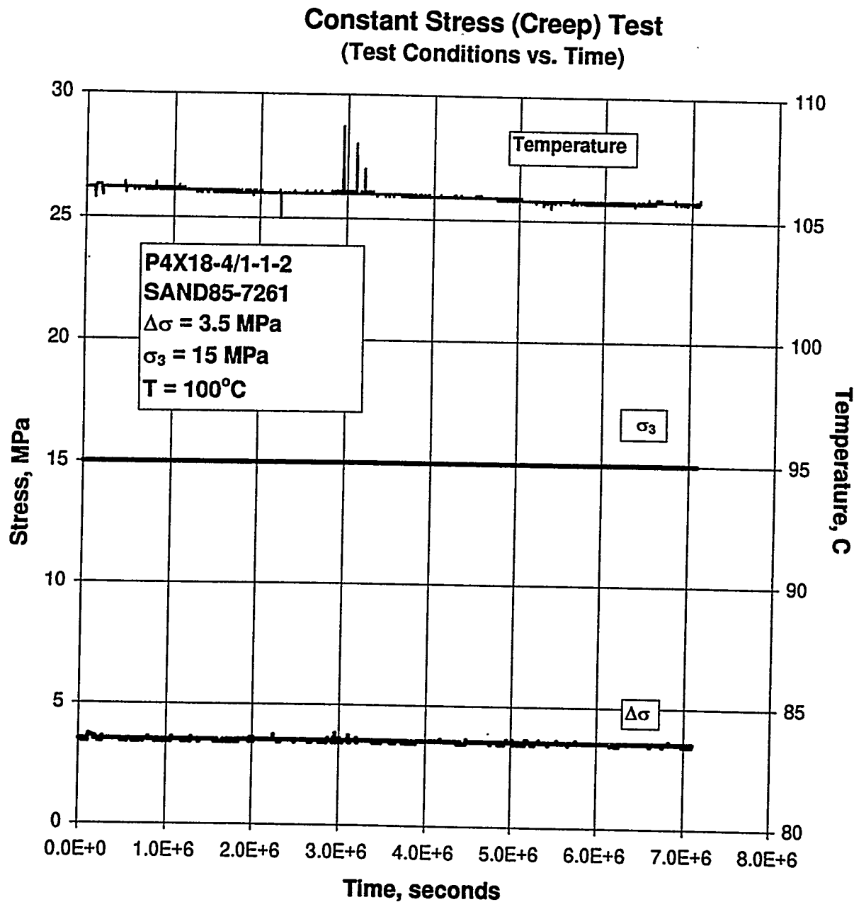
Figure C-47. Test Conditions Versus Time for a Creep Test: Specimen P4X18-4/1-1-2; Stage 1 of 1 (Argillaceous Salt).
