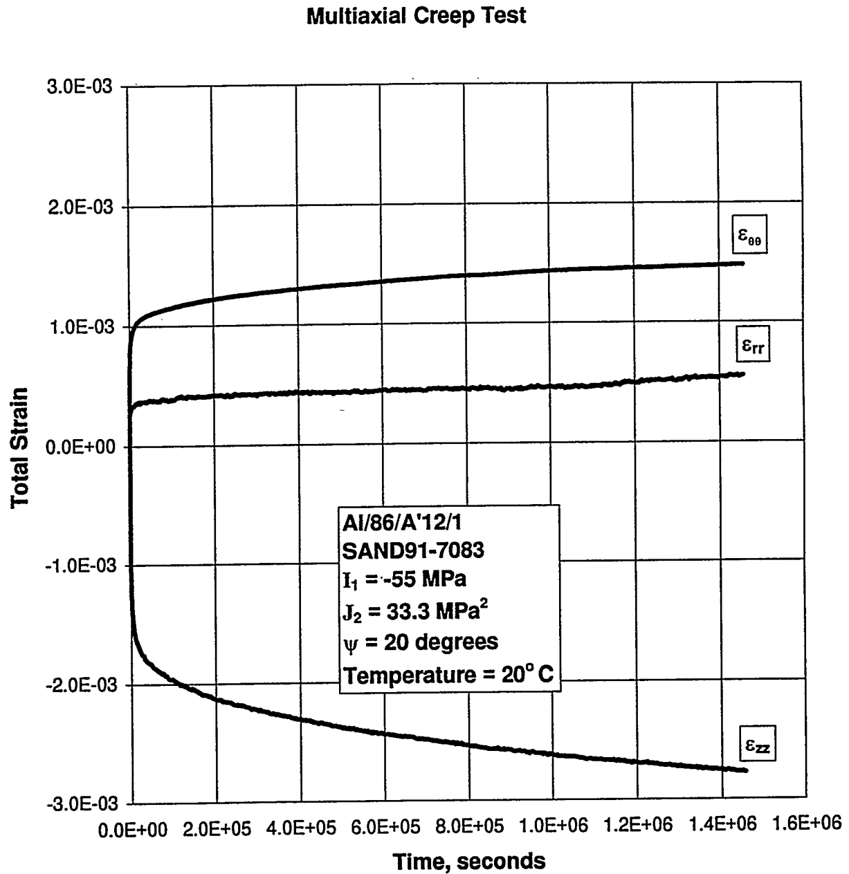
Figure D-10. Principal Strains Versus Time for a Multiaxial Creep Test: Specimen AI/86/A'12/1.
