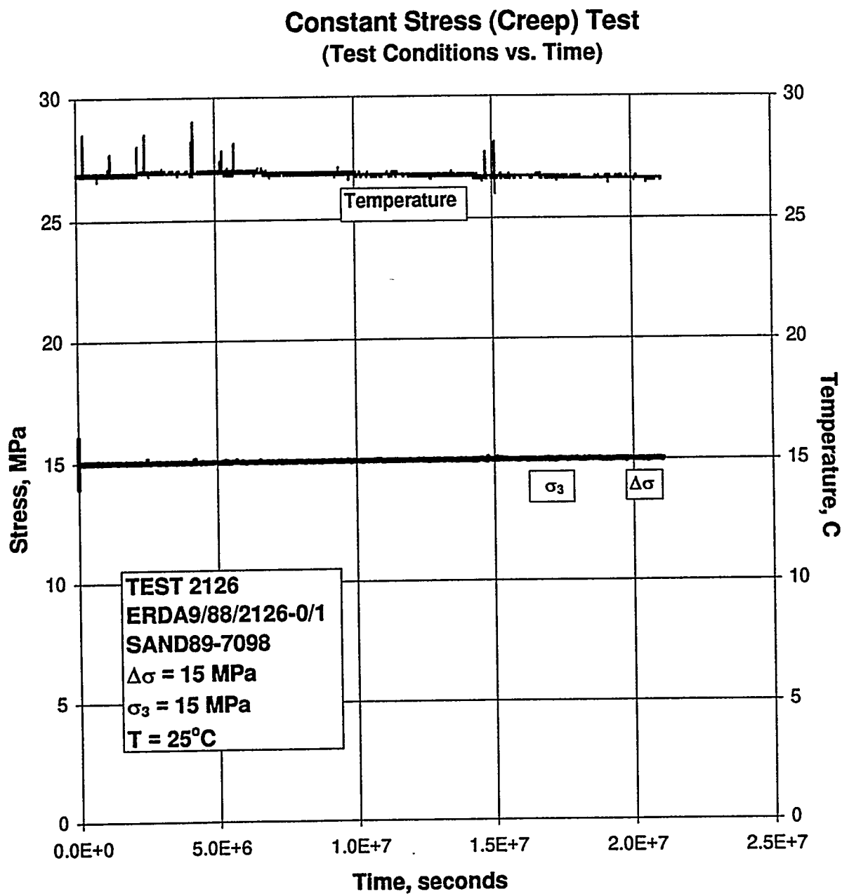
Figure B-5. Test Conditions Versus Time for a Creep Test: Specimen ERDA9/88/2126-0/1; Stage 1 of 1.
