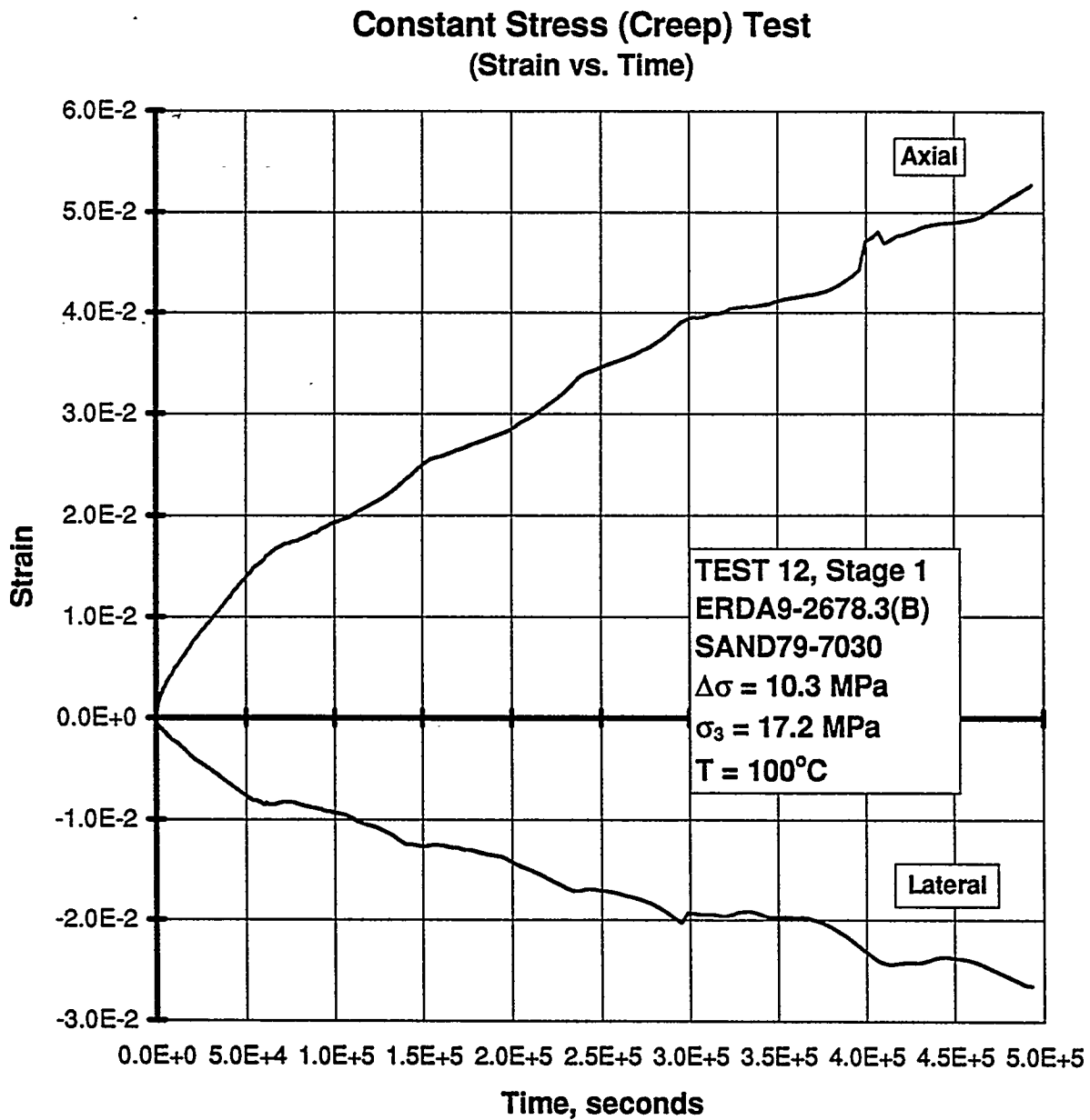
Figure B-130. Axial Strain and Lateral Strain Versus Time for a Creep Test: Specimen ERDA9-2678.3 (B); Stage 1 of 2.
