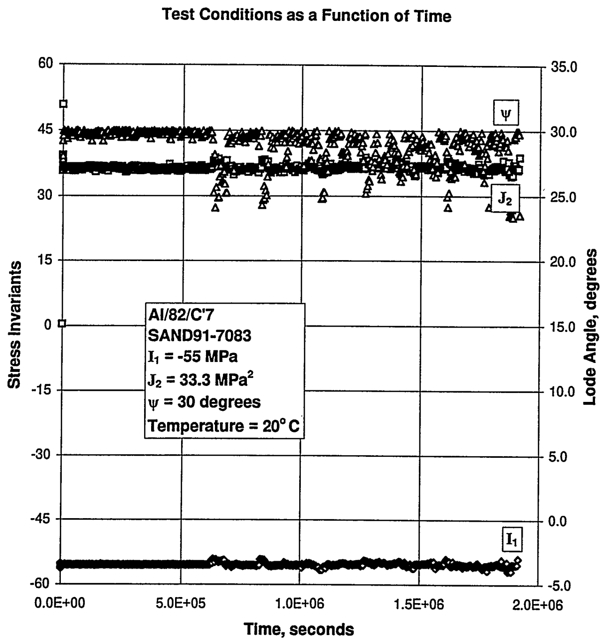
Figure D-11. Test Conditions Versus Time for a Multiaxial Creep Test: Specimen AI/82/C'7.
