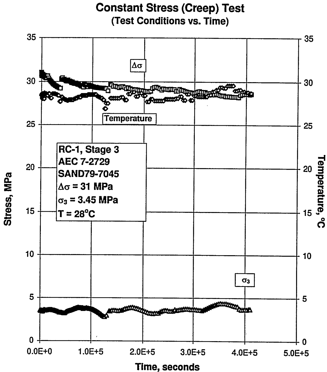
Figure B-153. Test Conditions Versus Time for a Creep Test: Specimen AEC7-2729; Stage 3 of 3.
