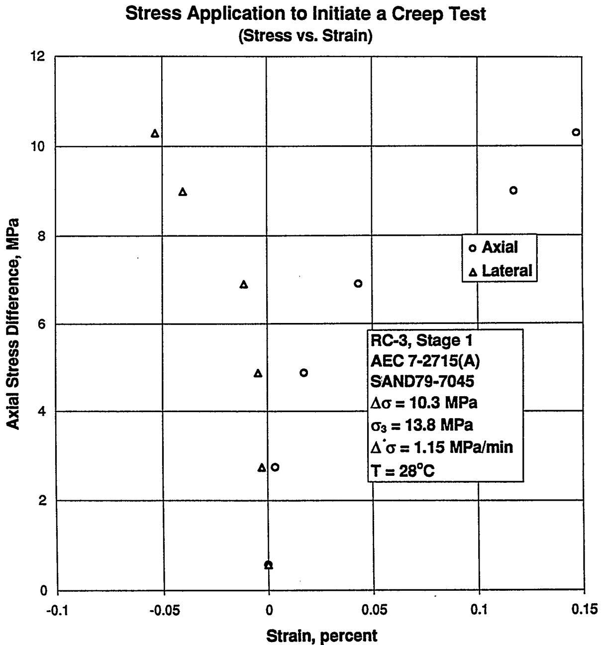
Figure B-164. Axial Stress Difference Versus Axial and Lateral Strain for Stress Application to Initiate a Creep Test: Specimen AEC7-2715 (A); Stage 1 of 3.
