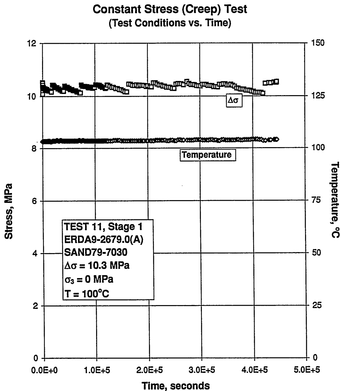
Figure B-123. Test Conditions Versus Time for a Creep Test: Specimen ERDA9-2679.0 (A); Stage 1 of 2.
