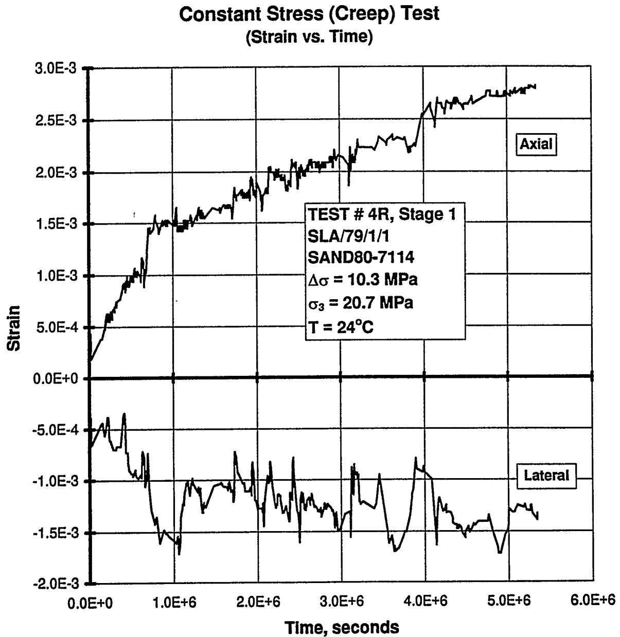
Figure B-33. Axial Strain and Lateral Strain Versus Time for a Creep Test: Specimen SLA/79/1/1; Stage 1 of 2.
