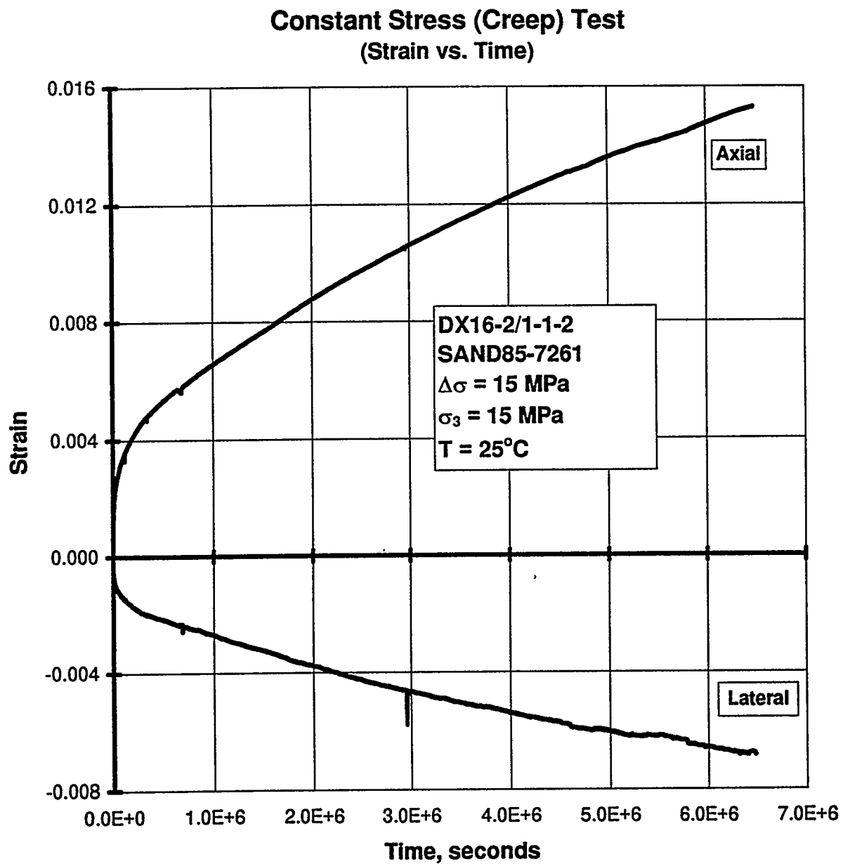
Figure C-62. Axial Strain and Lateral Strain Versus Time for a Creep Test: Specimen DX16-2/1-1-2; Stage 1 of 1.
