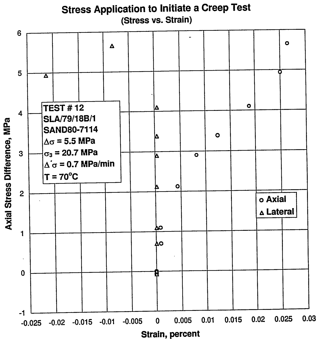
Figure B-66. Axial Stress Difference Versus Axial and Lateral Strain for Stress Application to Initiate a Creep Test: Specimen SLA/79/18B/1; Stage 1 of 1.
