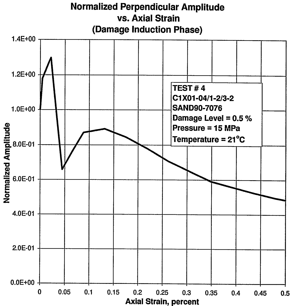
Figure E-73. Normalized Perpendicular Amplitude as a Function of Axial Strain During the Quasi-Static Loading to Induce Damage in Specimen C1X01-04/1-2/3-2.
