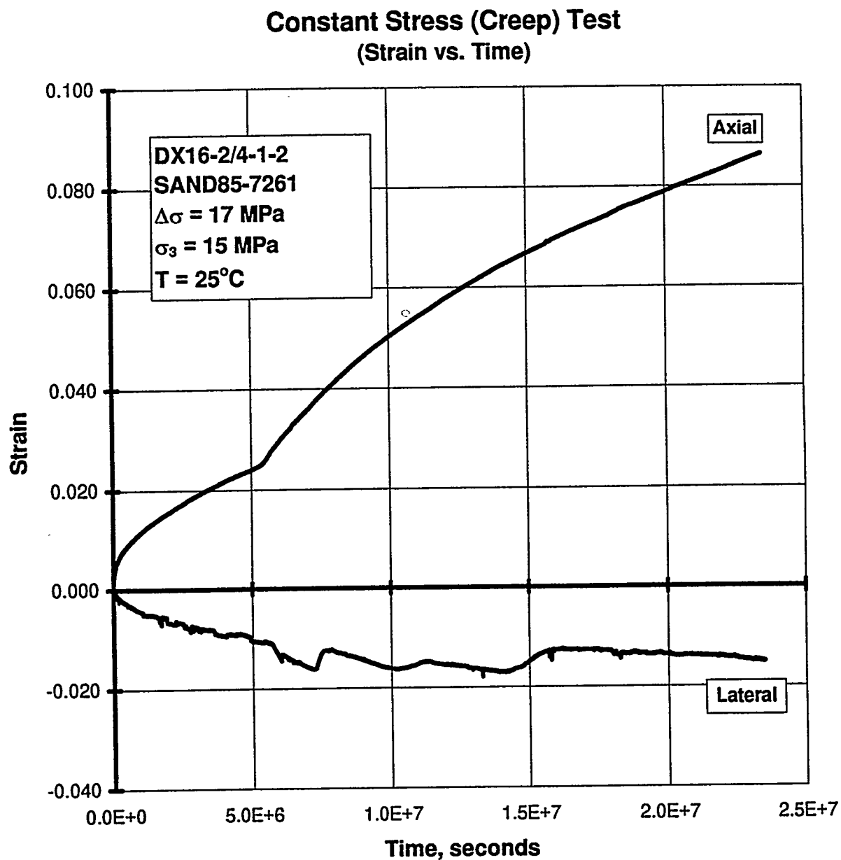
Figure C-64. Axial Strain and Lateral Strain Versus Time for a Creep Test: Specimen DX16-2/4-1-2; Stage 1 of 1 (Anomalous Test Result. Possible Machine Malfunction).
