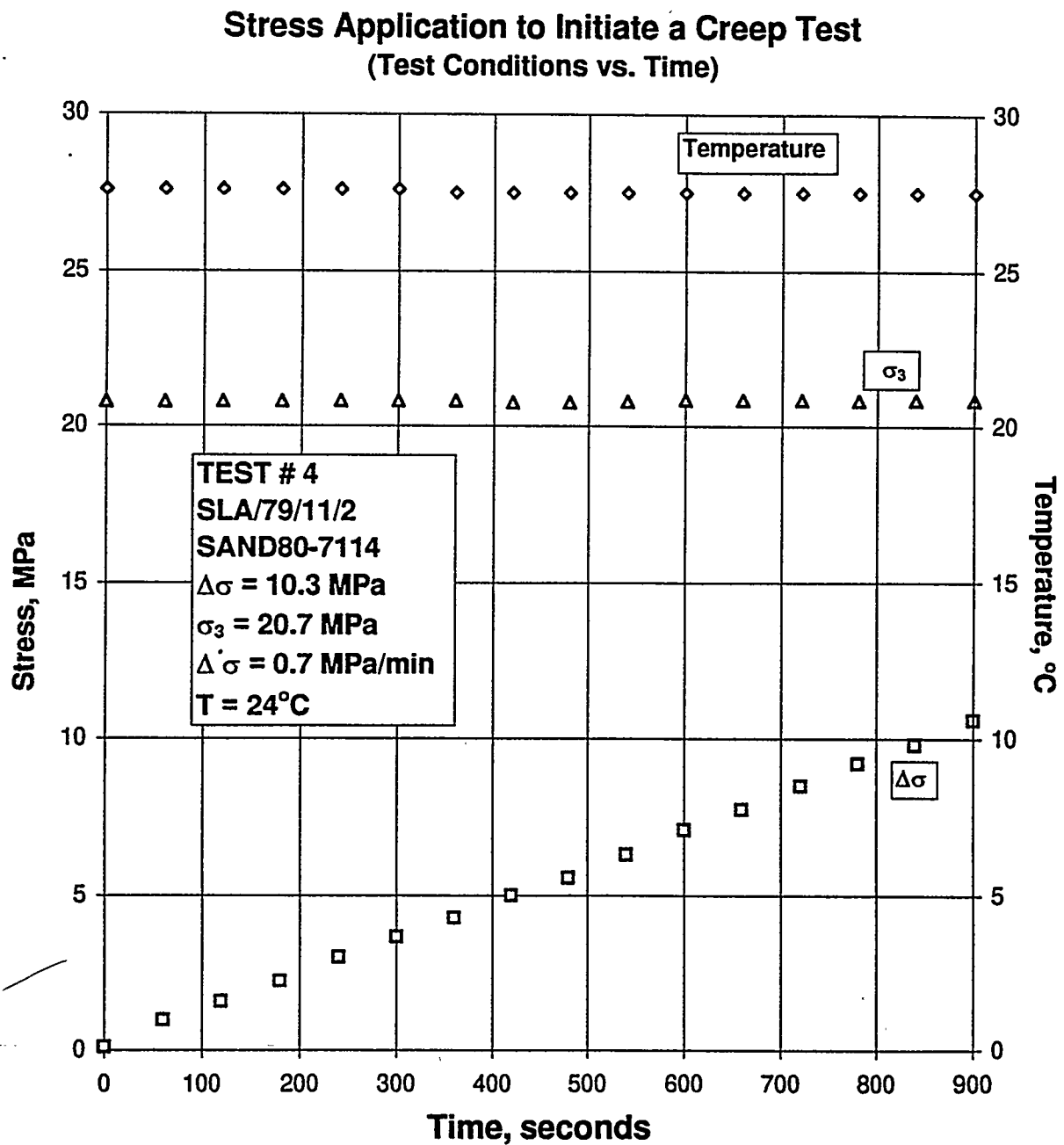
Figure B-26. Test Conditions Versus Time for Stress Application to Initiate a Creep Test: Specimen SLA/79/11/2; Stage 1 of 1.
