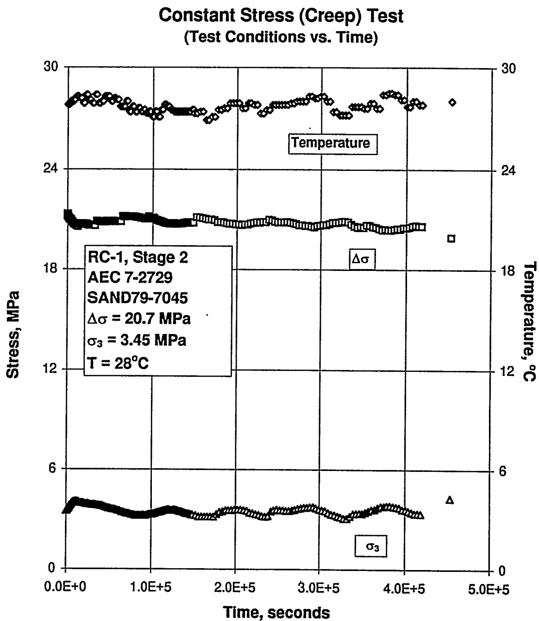
Figure B-149. Test Conditions Versus Time for a Creep Test: Specimen AEC7-2729; Stage 2 of 3.
