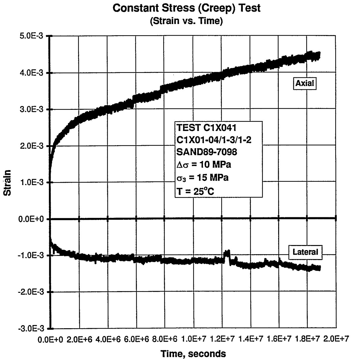
Figure C-32. Axial Strain and Lateral Strain Versus Time for a Creep Test: Specimen C1X01-04/1-3/1-2; Stage 1 of 1.
