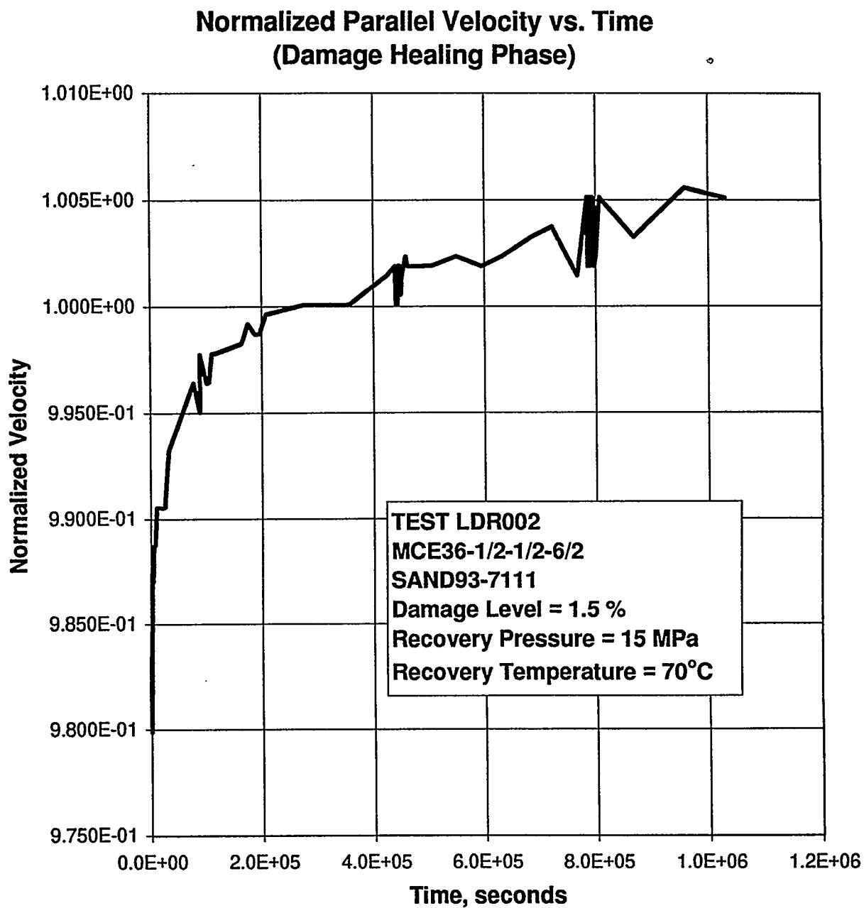
Figure E-16. Normalized Parallel Velocity as a Function of Time During the Hydrostatic Loading to Recover Damage in Specimen MCE36-1/2-1/2-6/2.
