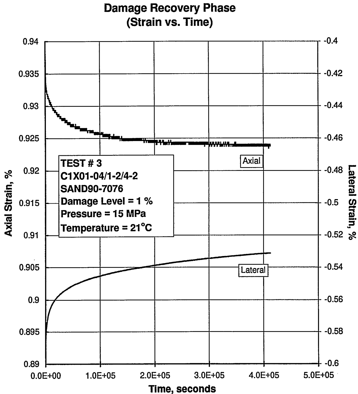
Figure E-66. Axial and Lateral Strain as a Function of Time During the Hydrostatic Loading to Recover Damage in Specimen C1X01-04/1-2/4-2.
