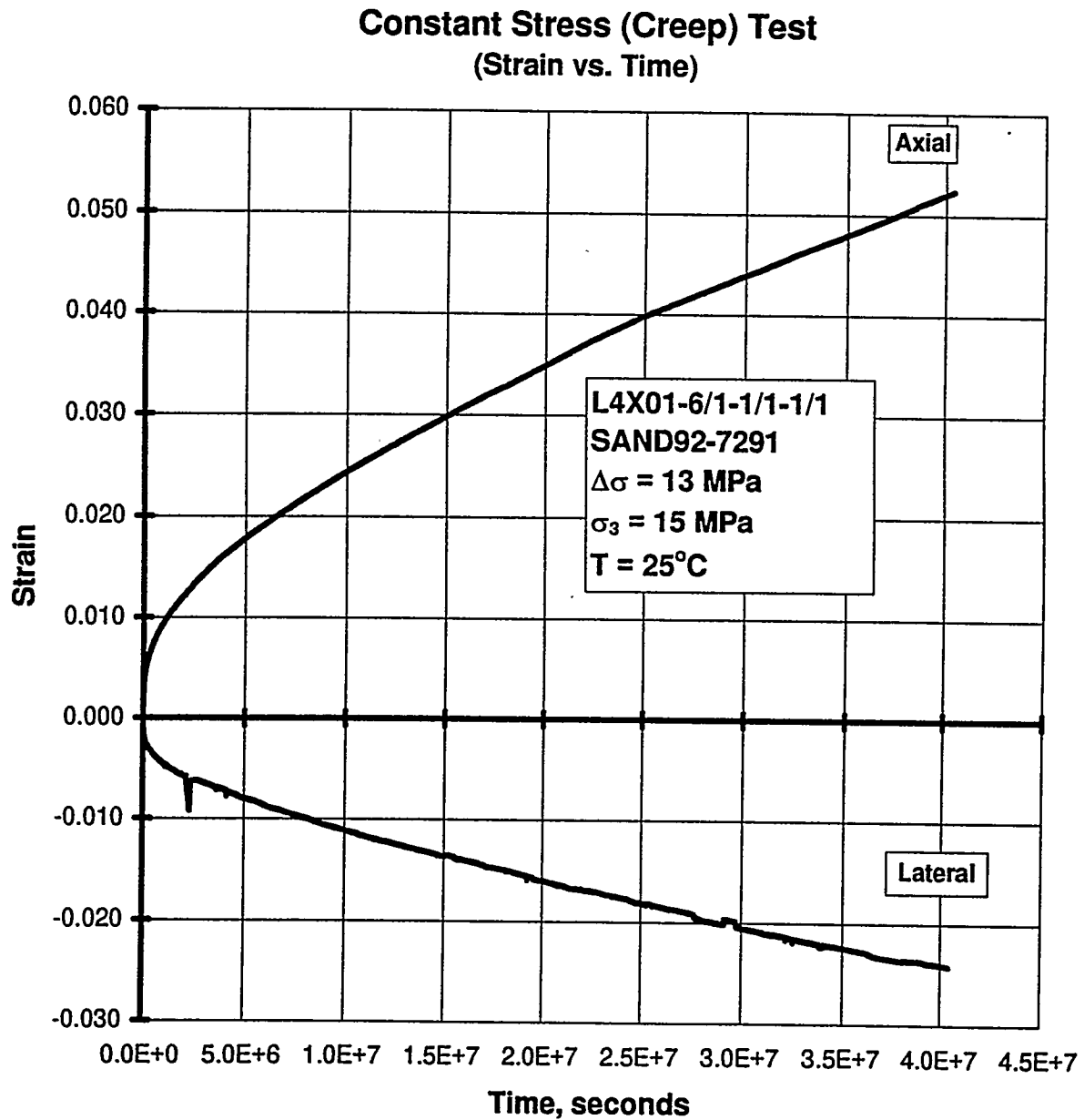
Figure C-20. Axial Strain and Lateral Strain Versus Time for a Creep Test: Specimen L4X01-6/1-1/1-1/1; Stage 1 of 1 (Argillaceous Salt).
