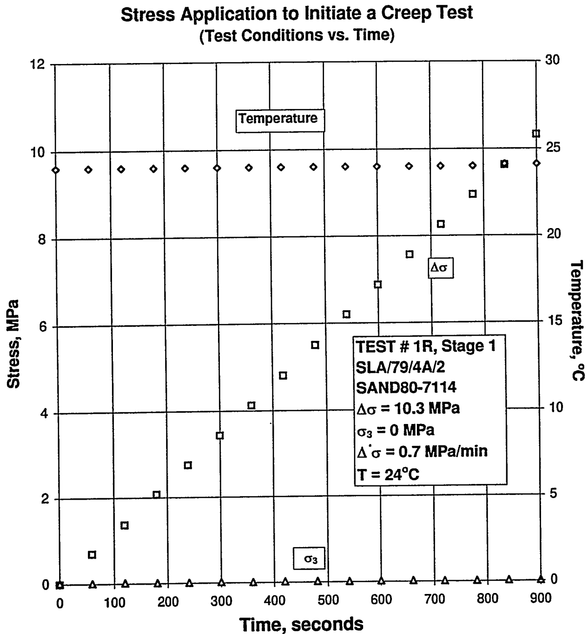
Figure B-11. Test Conditions Versus Time for Stress Application to Initiate a Creep Test: Specimen SLA/79/4A/2; Stage 1 of 2.
