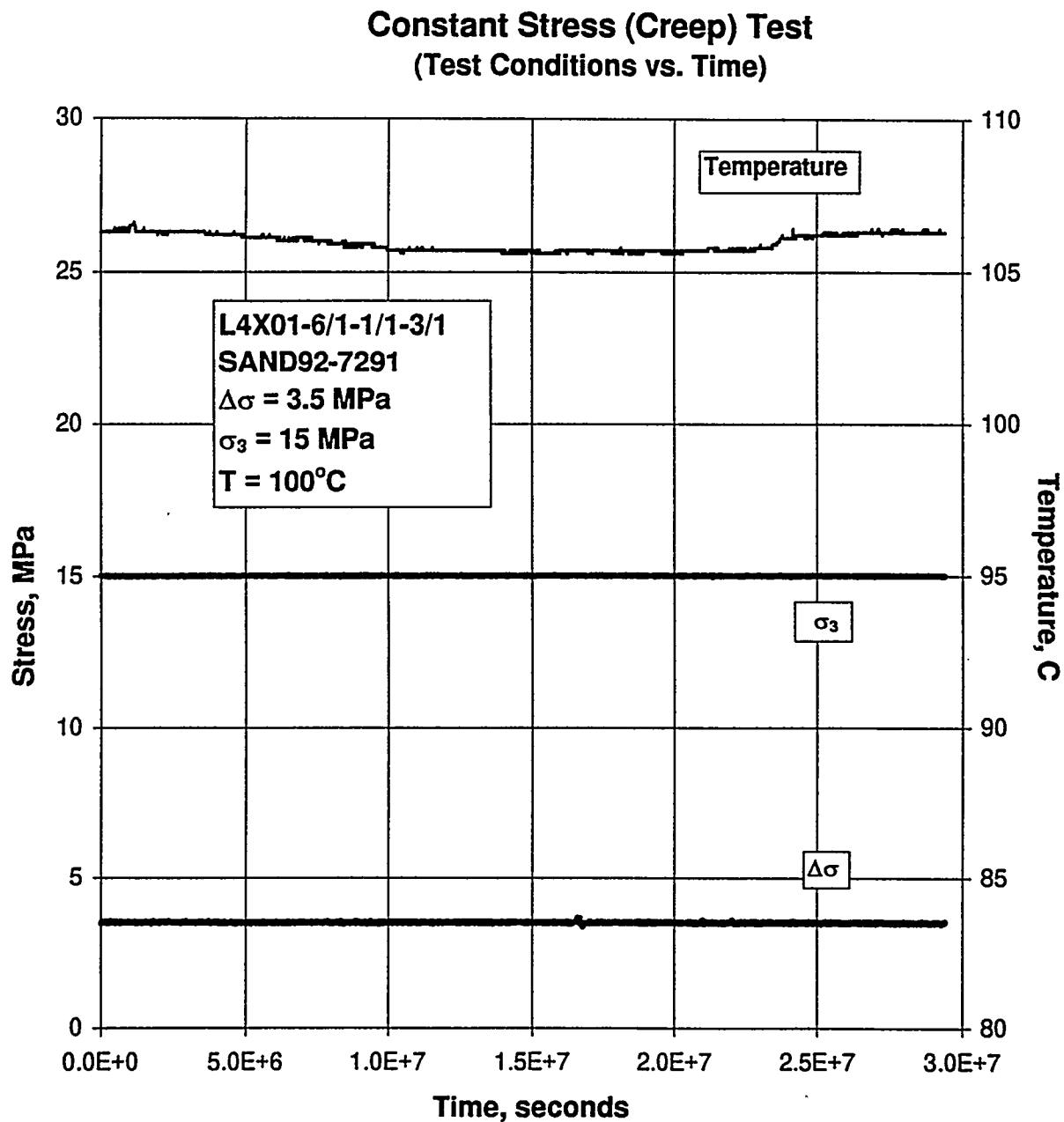
Figure C-25. Test Conditions Versus Time for a Creep Test: Specimen L4X01-6/1-1/1-3/1; Stage 1 of 1 (Argillaceous Salt).
