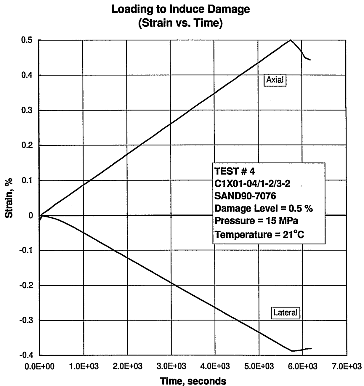
Figure E-72. Axial and Lateral Strain as a Function of Time During the Quasi-Static Loading to Induce Damage in Specimen C1X01-04/1-2/3-2.
