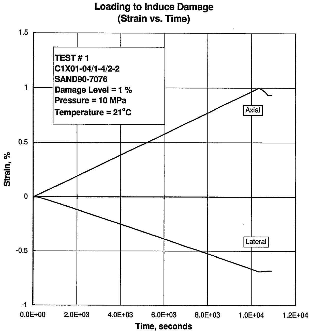
Figure E-36. Axial and Lateral Strain as a Function of Time During the Quasi-Static Loading to Induce Damage in Specimen C1X01-04/1-4/2-2.
