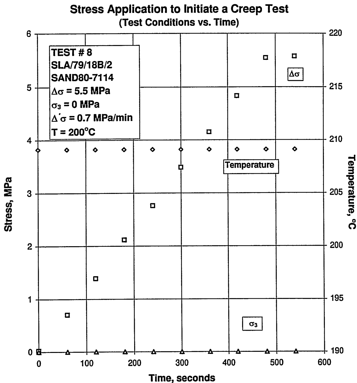
Figure B-49. Test Conditions Versus Time for Stress Application to Initiate a Creep Test: Specimen SLA/79/18B/2; Stage 1 of 1.
