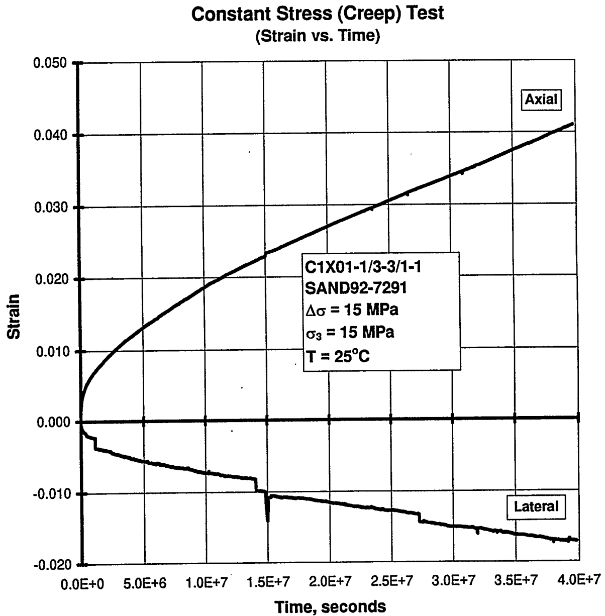
Figure C-4. Axial Strain and Lateral Strain Versus Time for a Creep Test: Specimen C1X01-1/3-3/1-1; Stage 1 of 1.
