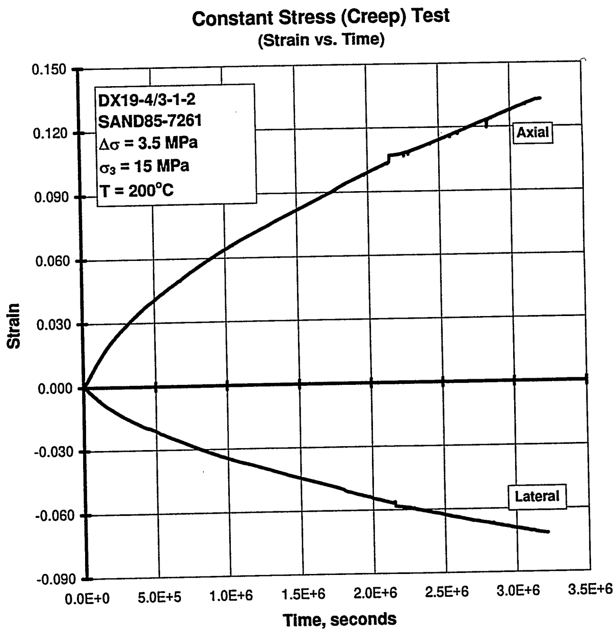
Figure C-88. Axial Strain and Lateral Strain Versus Time for a Creep Test: Specimen DX19-4/3-1-2; Stage 1 of 1.
