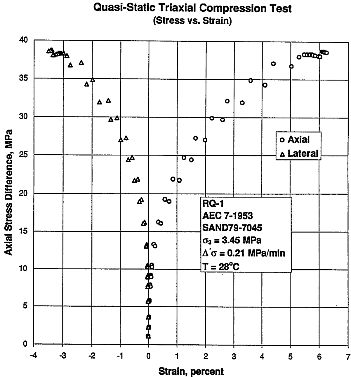
Figure A-2. Axial Stress Difference Versus Axial and Lateral Strain for a Quasi-Static Triaxial Compression Test: Specimen AEC7-1953.
