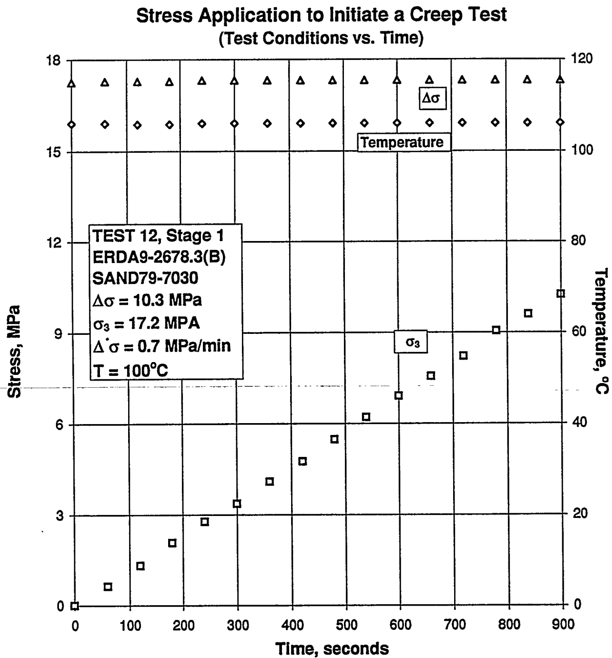
Figure B-127. Test Conditions Versus Time for Stress Application to Initiate a Creep Test: Specimen ERDA9-2678.3 (B); Stage 1 of 2.
