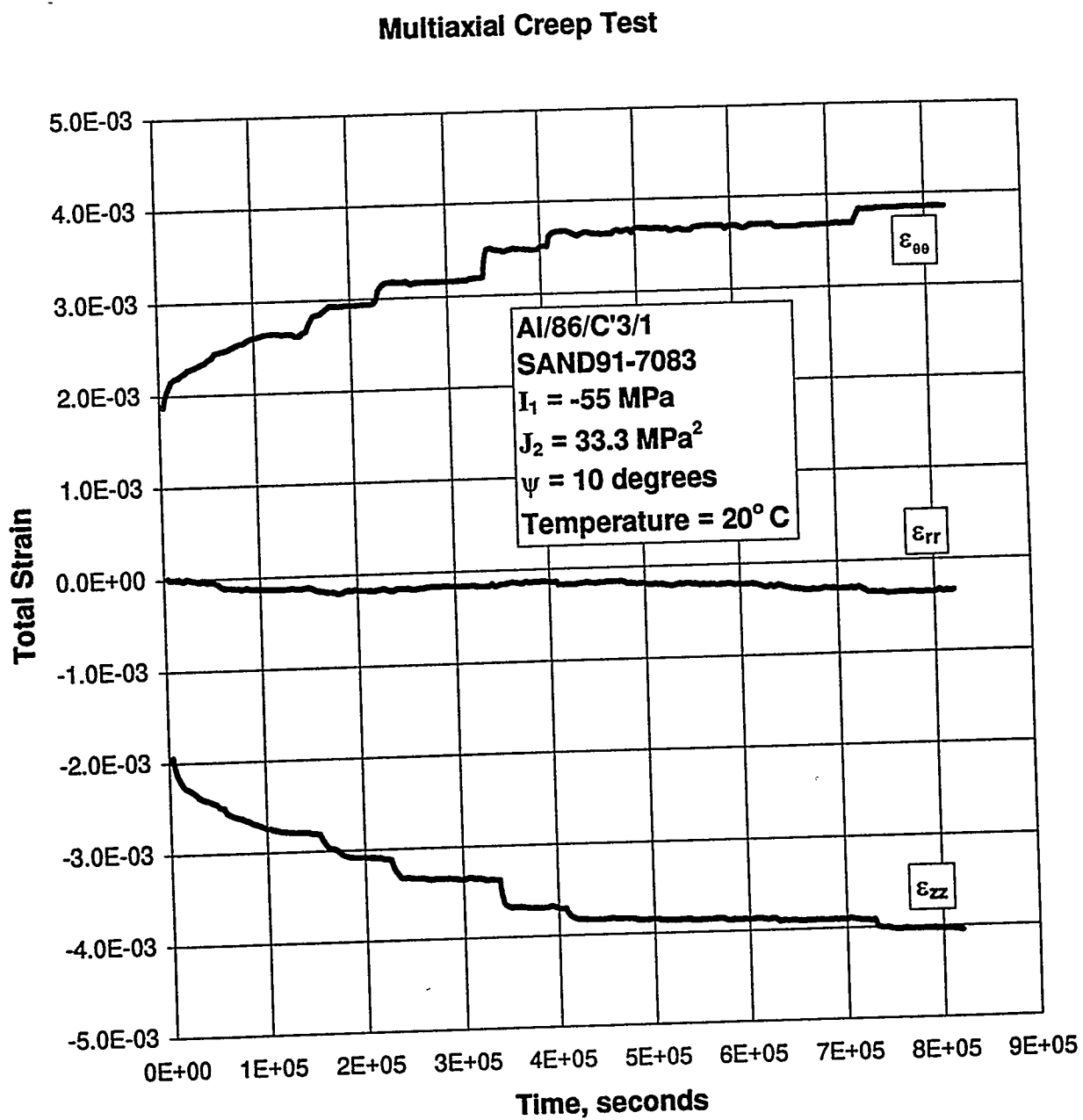
Figure D-4. Principal Strains Versus Time for a Multiaxial Creep Test: Specimen AI/86/C'3/1.
