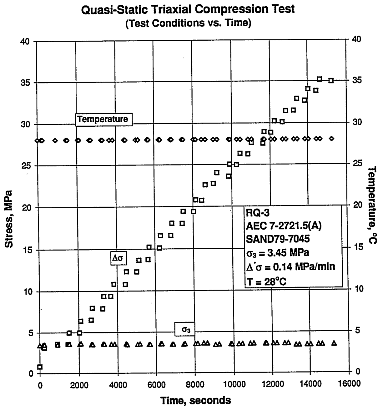
Figure A-5. Test Conditions Versus Time for a Quasi-Static Triaxial Compression Test: Specimen AEC7-2721.5 (A).
