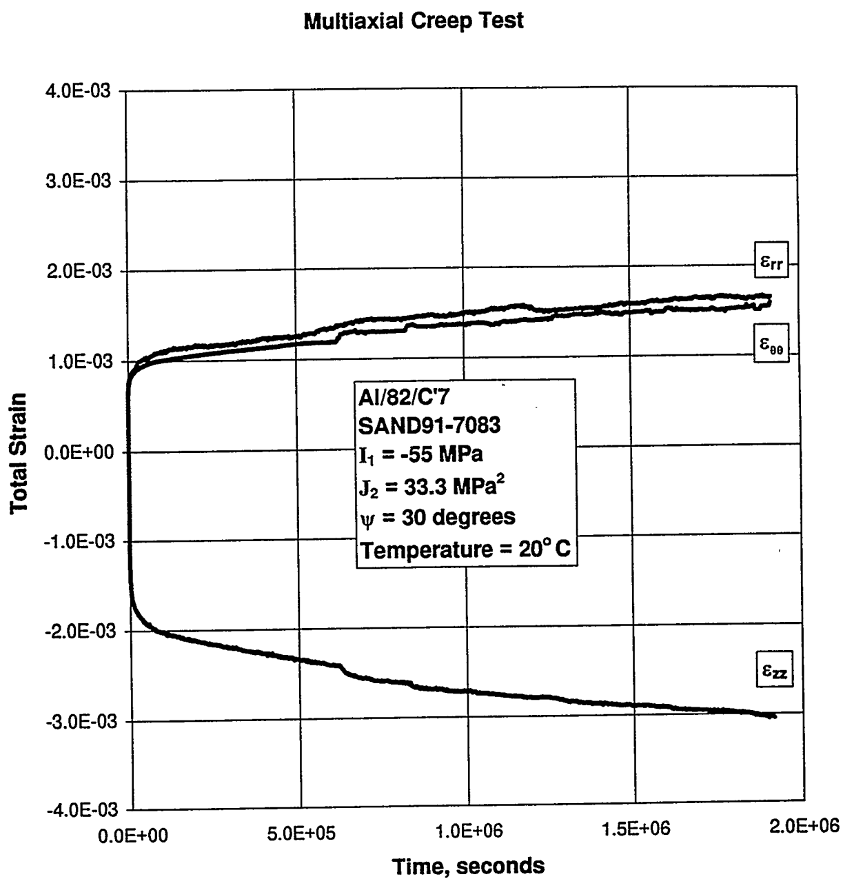
Figure D-12. Principal Strains Versus Time for a Multiaxial Creep Test: Specimen AI/82/C'7.
