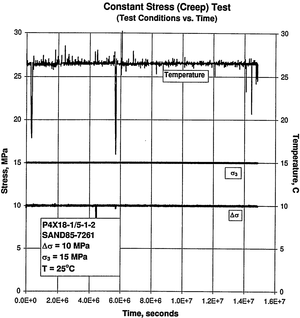
Figure C-39. Test Conditions Versus Time for a Creep Test: Specimen P4X18-1/5-1-2; Stage 1 of 1 (Argillaceous Salt).
