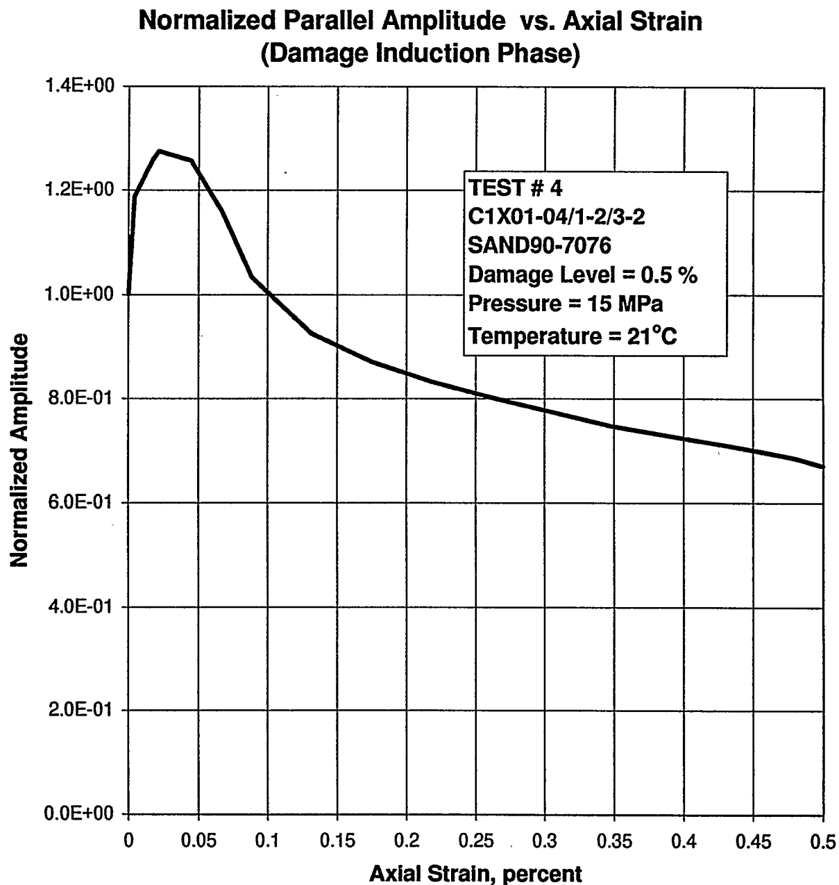
Figure E-74. Normalized Parallel Amplitude as a Function of Axial Strain During the Quasi-Static Loading to Induce Damage in Specimen C1X01-04/1-2/3-2.
