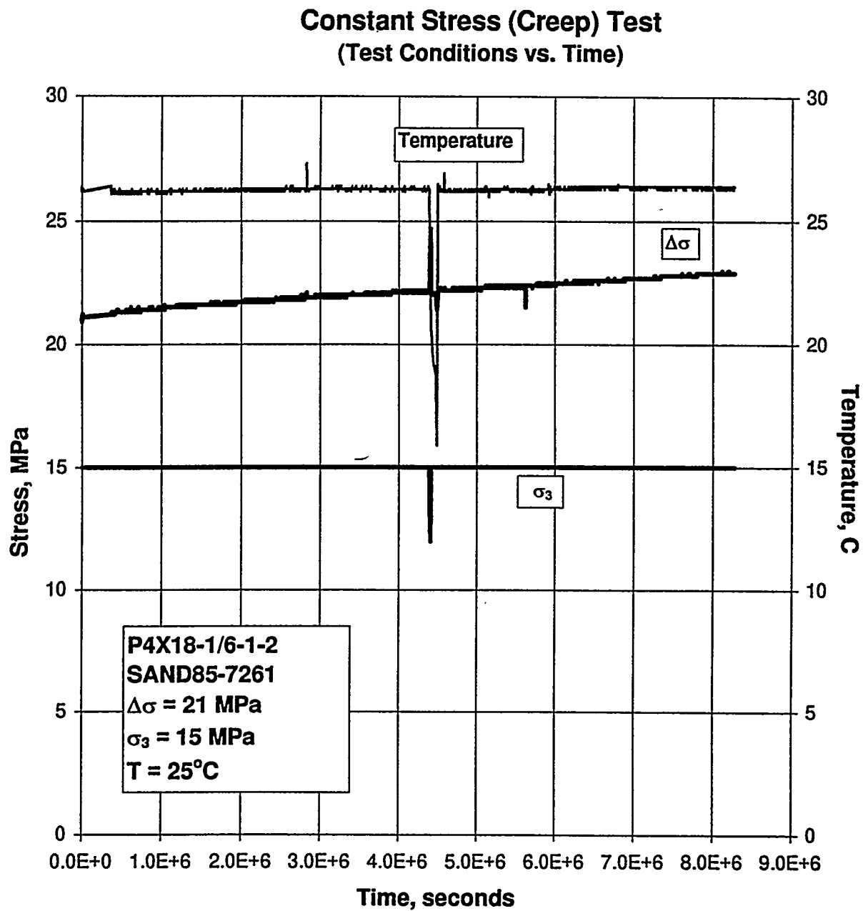
Figure C-45. Test Conditions Versus Time for a Creep Test: Specimen P4X18-1/6-1-2; Stage 1 of 1 (Argillaceous Salt).
