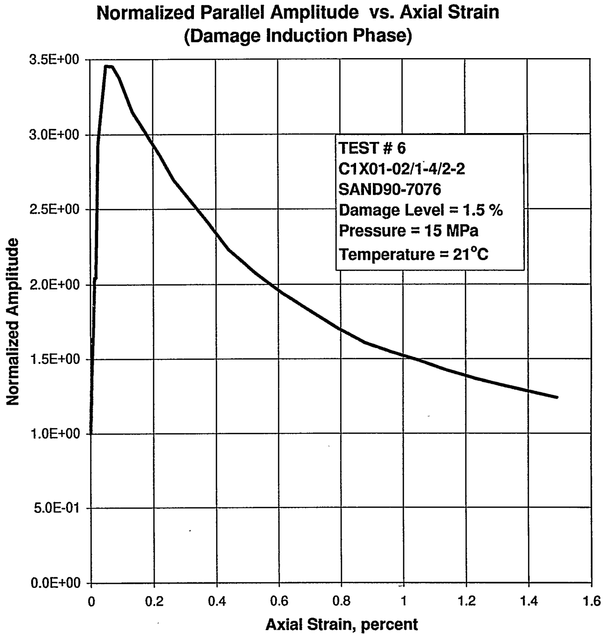
Figure E-98. Normalized Parallel Amplitude as a Function of Axial Strain During the Quasi-Static Loading to Induce Damage in Specimen C1X01-02/1-4/2-2.
