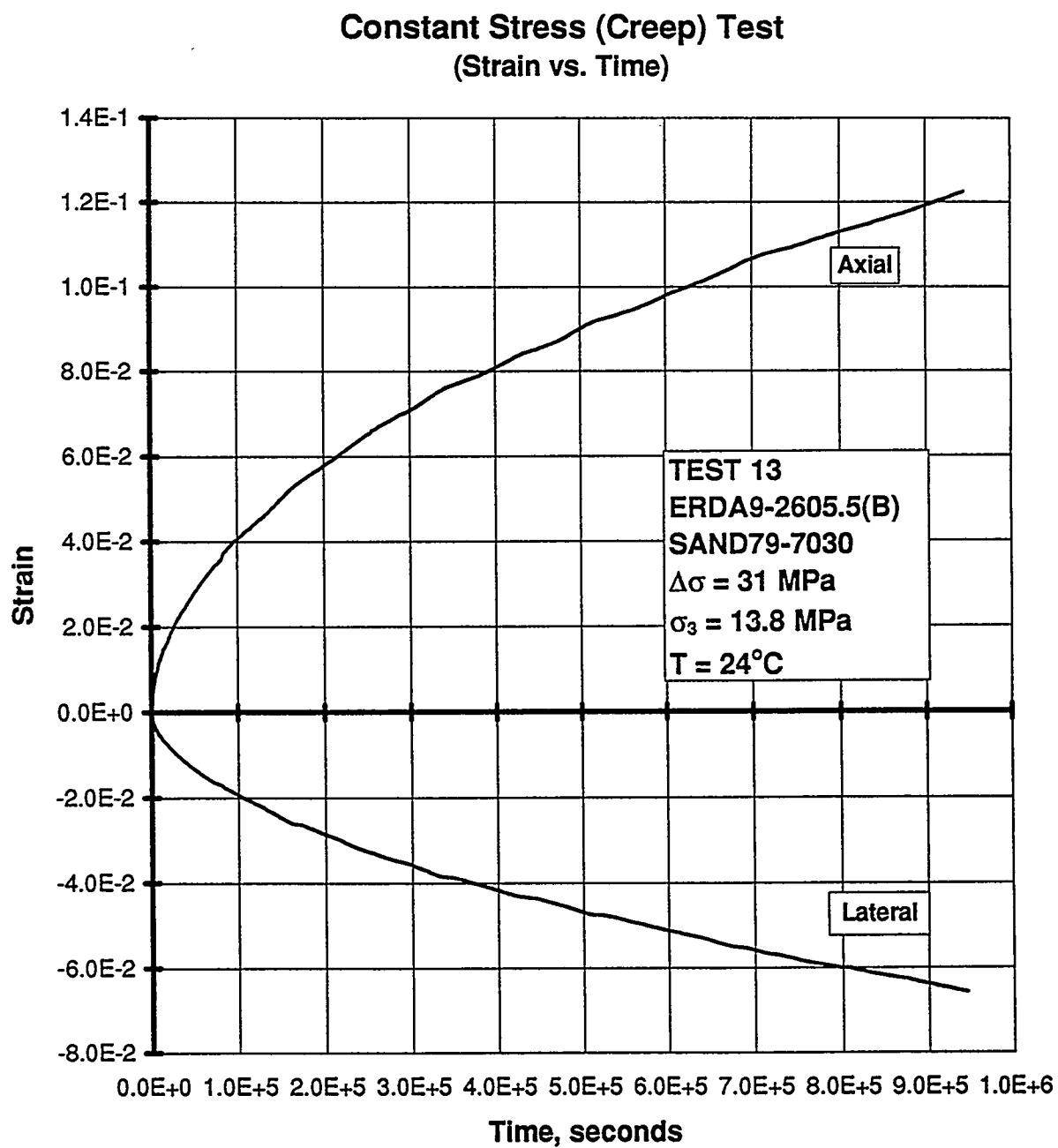
Figure B-138. Axial Strain and Lateral Strain Versus Time for a Creep Test: Specimen ERDA9-2605.5 (B); Stage 1 of 1.
