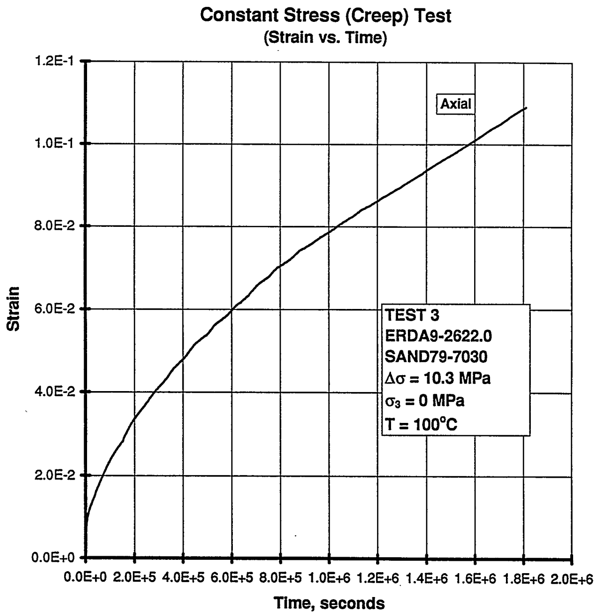
Figure B-84. Axial Strain and Lateral Strain Versus Time for a Creep Test: Specimen ERDA9-2622.0; Stage 1 of 1.
