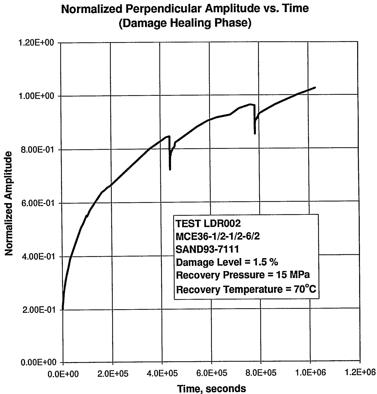
Figure E-14. Normalized Perpendicular Amplitude as a Function of Time During the Hydrostatic Loading to Recover Damage in Specimen MCE36-1/2-1/2-6/2.
