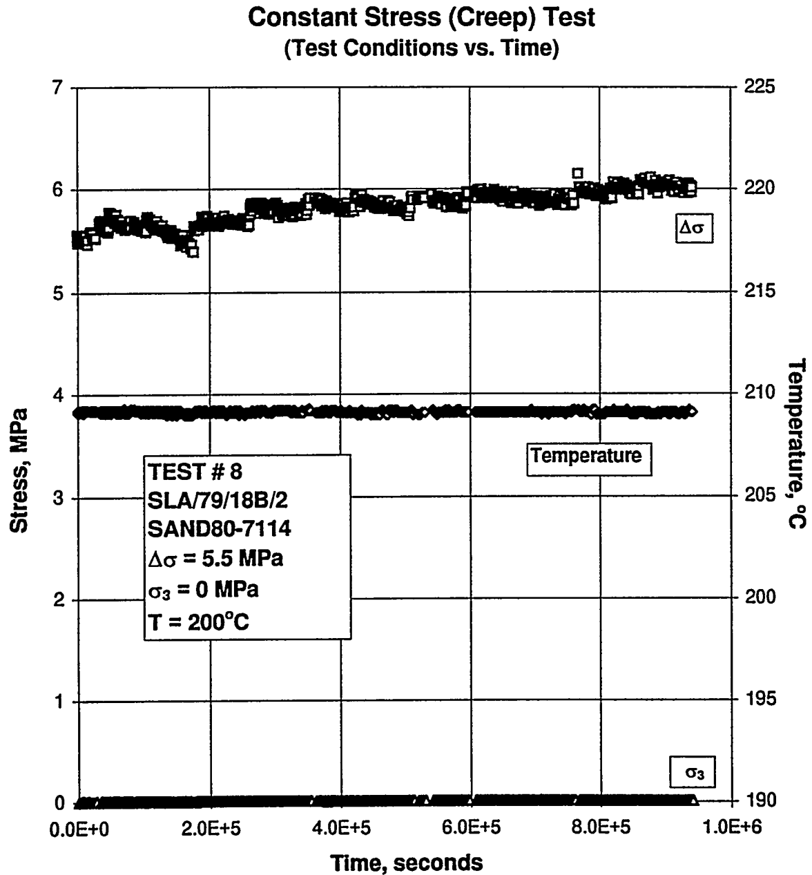
Figure B-51. Test Conditions Versus Time for a Creep Test: Specimen SLA/79/18B/2; Stage 1 of 1.
