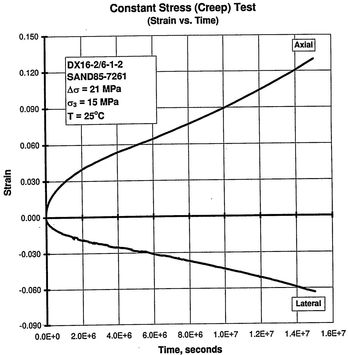
Figure C-70. Axial Strain and Lateral Strain Versus Time for a Creep Test: Specimen DX16-2/6-1-2; Stage 1 of 1 (Possible Jacket Leak Near End of Test).
