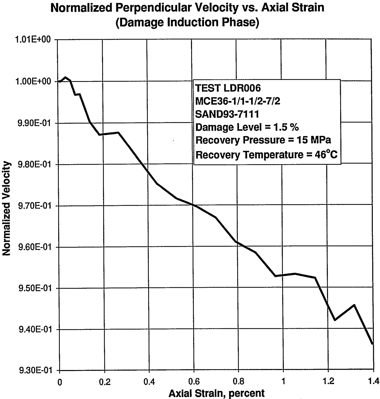
Figure E-33. Normalized Perpendicular Velocity as a Function of Axial Strain During the Quasi-Static Loading to Induce Damage in Specimen MCE36-1/1-1/2-7/2.
