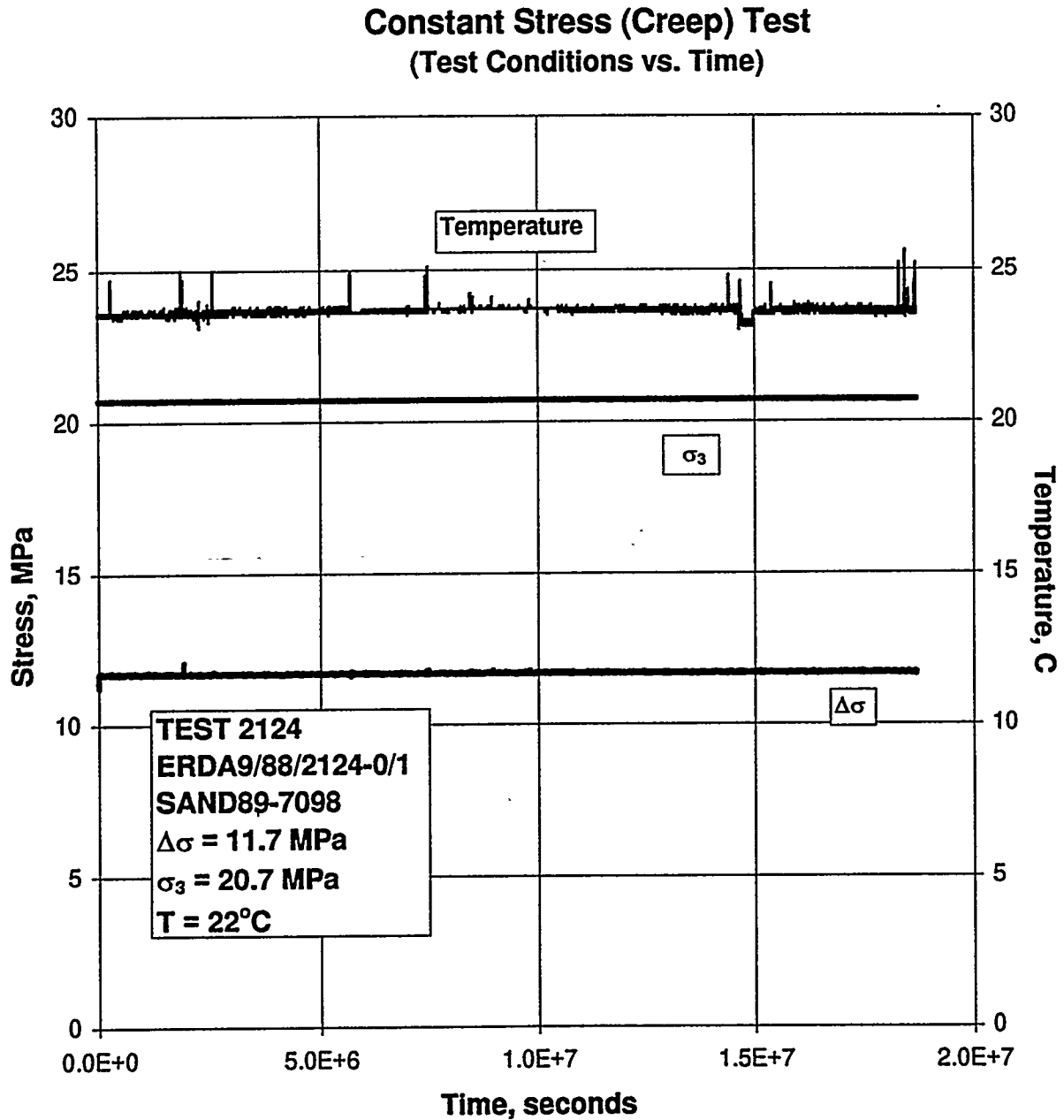
Figure B-3. Test Conditions Versus Time for a Creep Test: Specimen ERDA9/88/2124-0/1; Stage 1 of 1.
