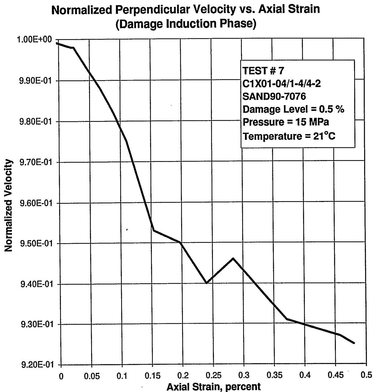
Figure E-111. Normalized Perpendicular Velocity as a Function of Axial Strain During the Quasi-Static Loading to Induce Damage in Specimen C1X01-04/1-4/4-2.
