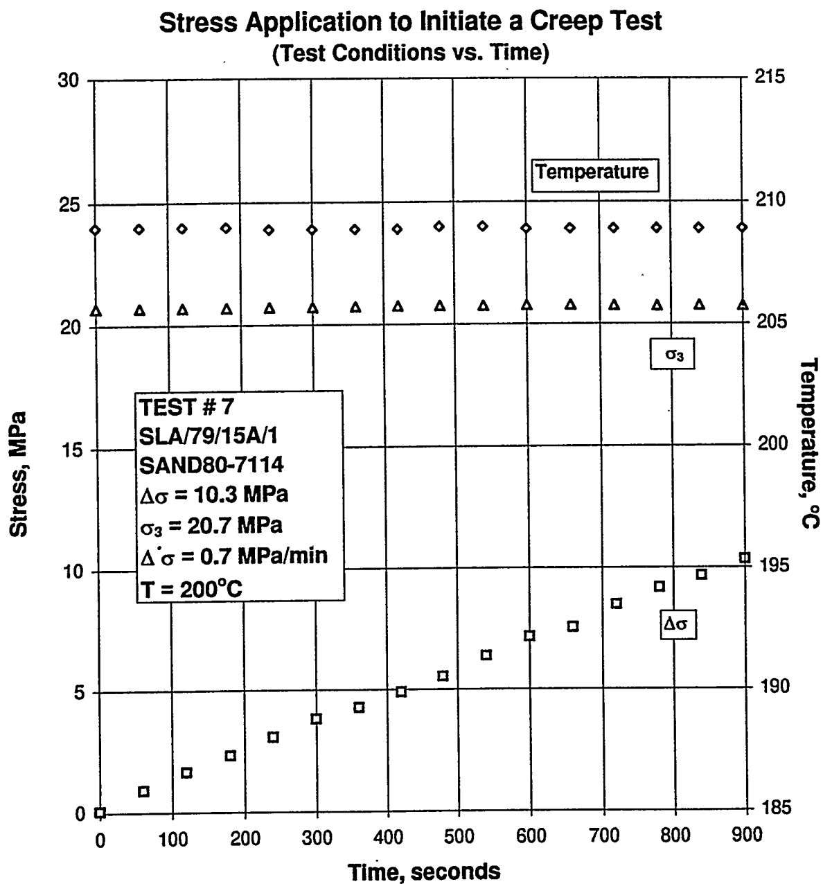
Figure B-45. Test Conditions Versus Time for Stress Application to Initiate a Creep Test: Specimen SLA/79/15A/1; Stage 1 of 1.
