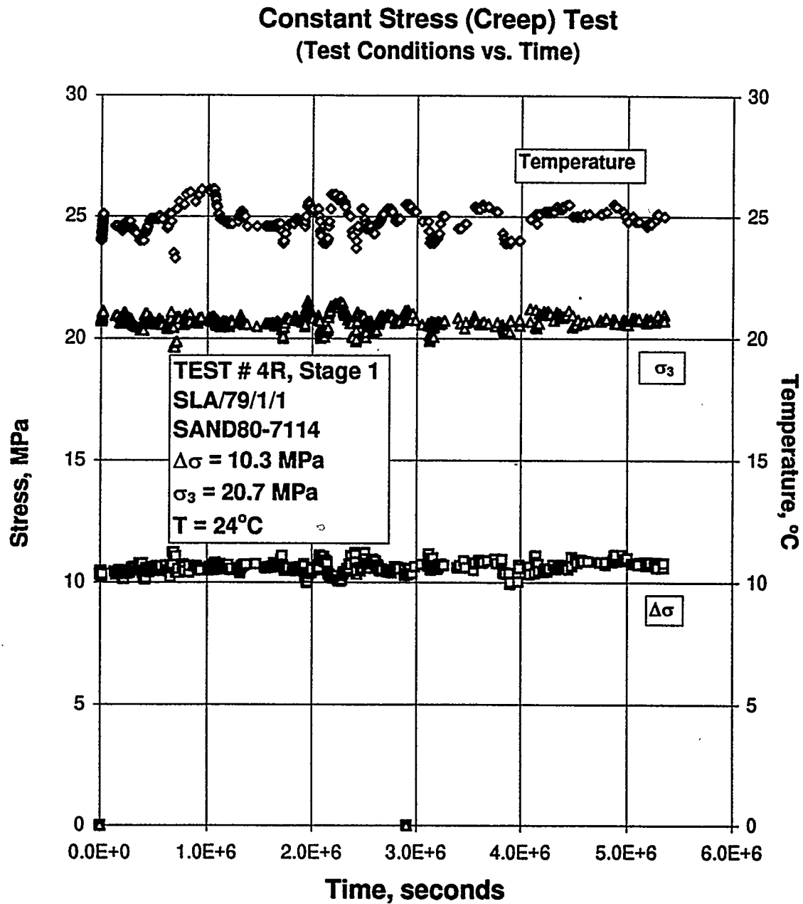
Figure B-32. Test Conditions Versus Time for a Creep Test: Specimen SLA/79/1/1; Stage 1 of 2.
