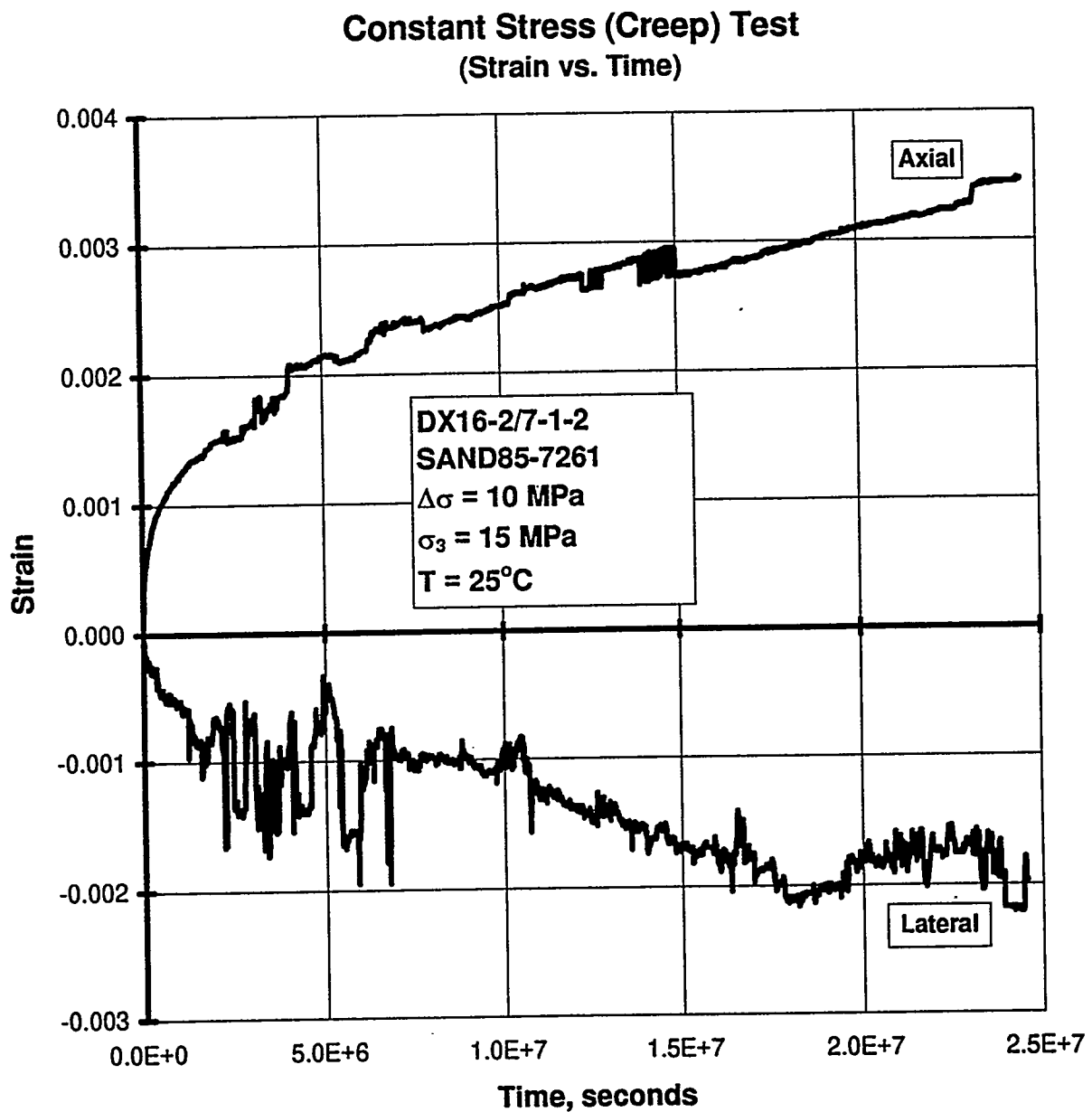
Figure C-56. Axial Strain and Lateral Strain Versus Time for a Creep Test: Specimen DX16-2/7-1-2; Stage 1 of 1.
