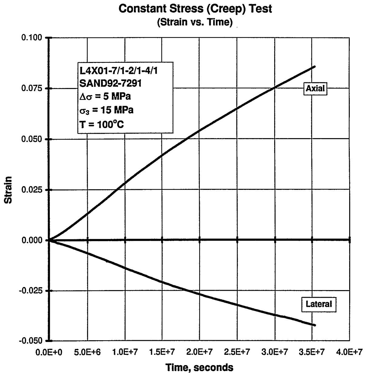
Figure C-30. Axial Strain and Lateral Strain Versus Time for a Creep Test: Specimen L4X01-7/1-2/1-4/1; Stage 1 of 1 (Argillaceous Salt).
