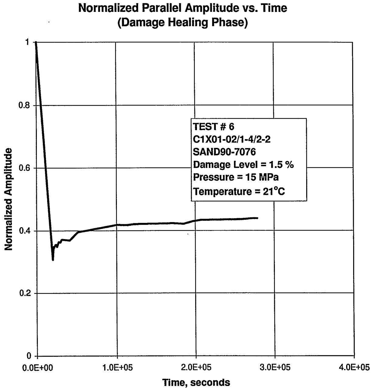
Figure E-104. Normalized Parallel Amplitude as a Function of Time During the Hydrostatic Loading to Recover Damage in Specimen C1X01-02/1-4/2-2.
