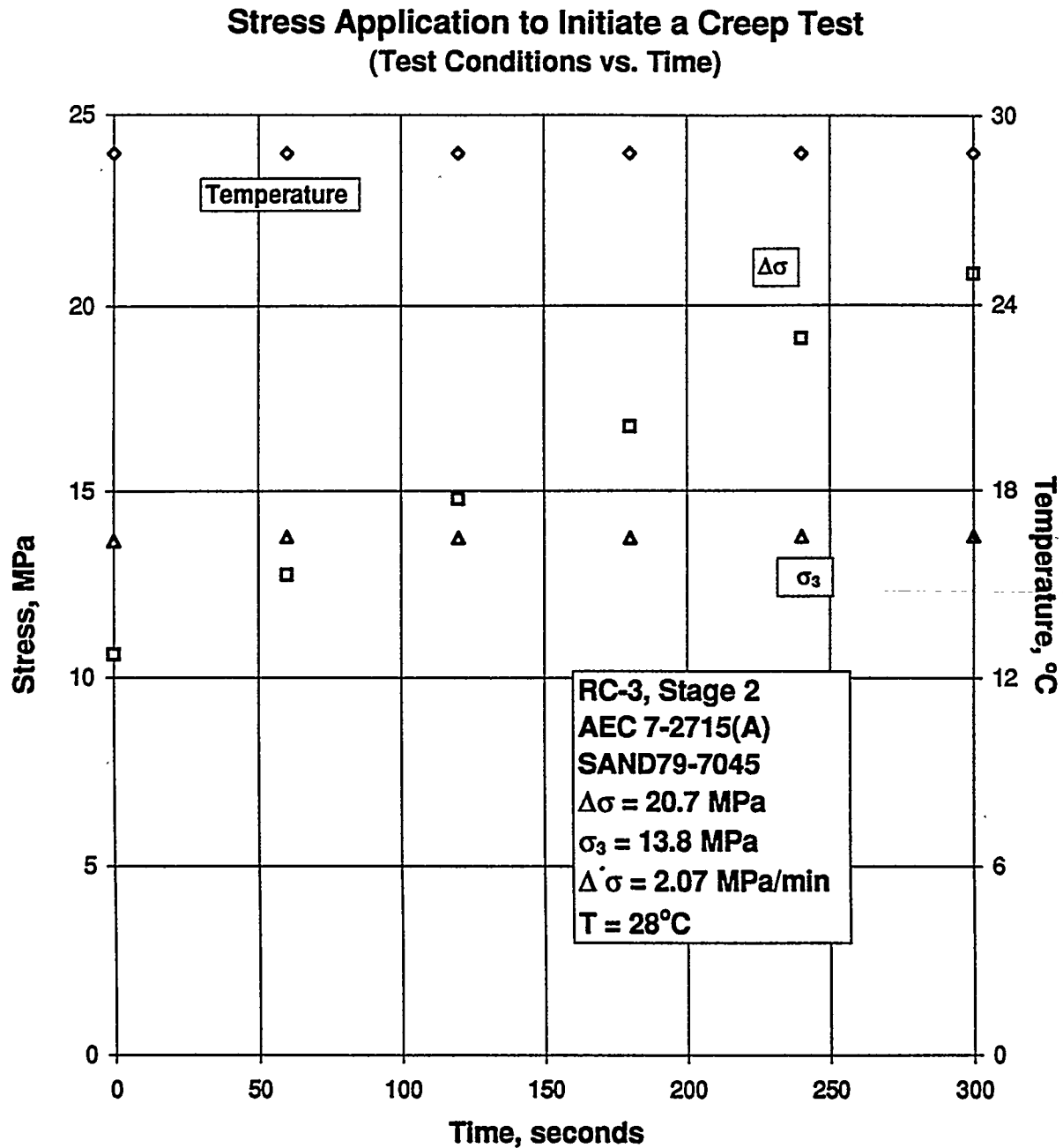
Figure B-167. Test Conditions Versus Time for Stress Application to Initiate a Creep Test: Specimen AEC7-2715 (A); Stage 2 of 3.
