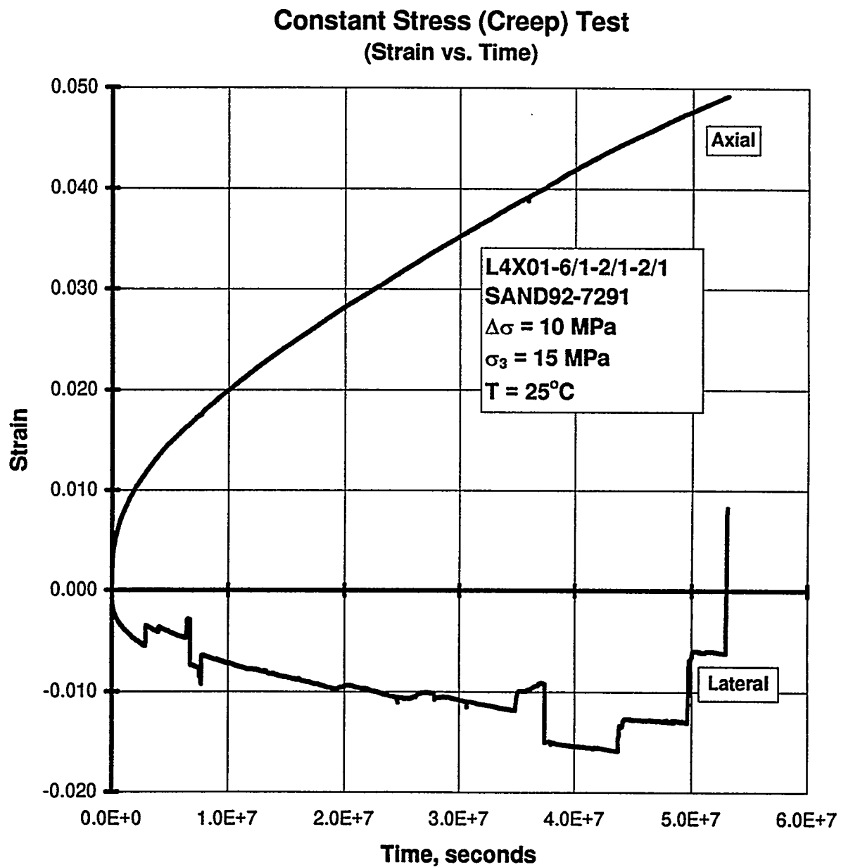
Figure C-16. Axial Strain and Lateral Strain Versus Time for a Creep Test: Specimen L4X01-6/1-2/1-2/1; Stage 1 of 1 (Argillaceous Salt).
