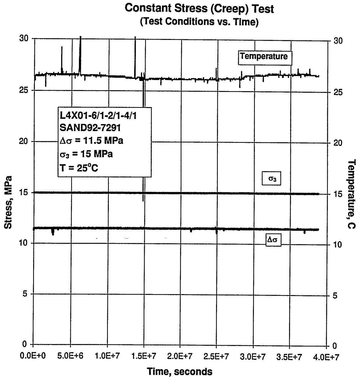
Figure C-17. Test Conditions Versus Time for a Creep Test: Specimen L4X01-6/1-2/1-4/1; Stage 1 of 1 (Argillaceous Salt).
