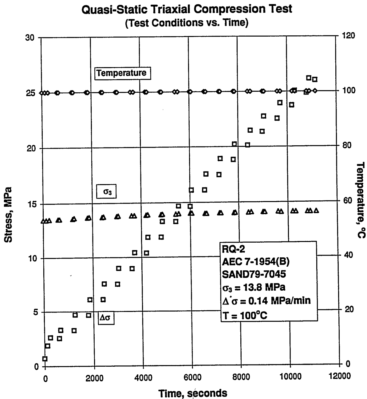
Figure A-3. Test Conditions Versus Time for a Quasi-Static Triaxial Compression Test: Specimen AEC7-1954 (B).
