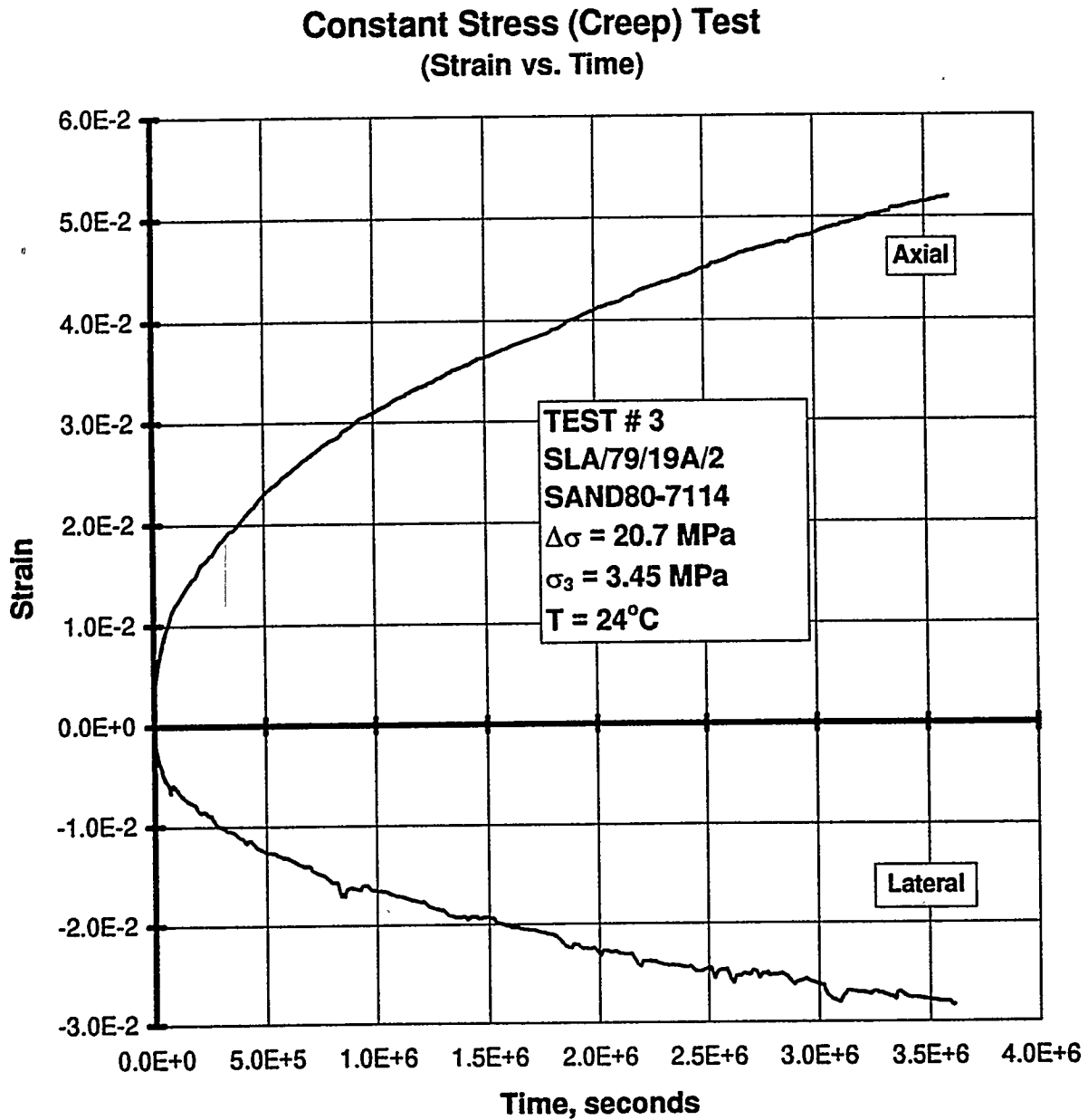
Figure B-25. Axial Strain and Lateral Strain Versus Time for a Creep Test: Specimen SLA/79/19A/2; Stage 1 of 1.
