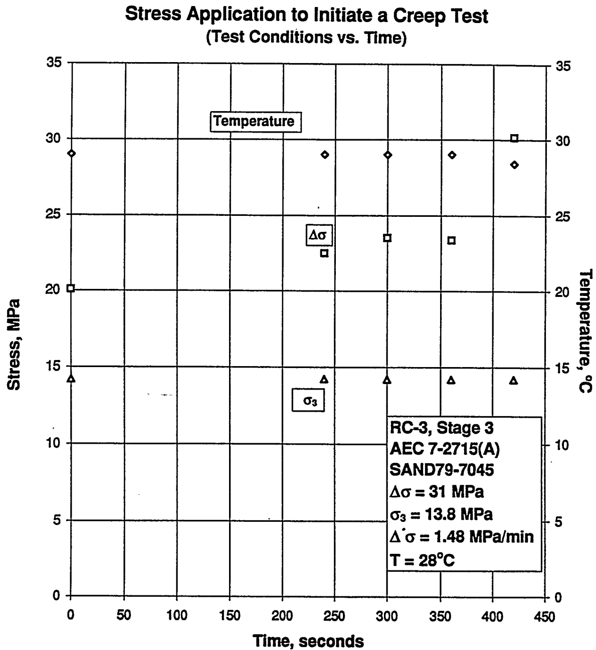
Figure B-171. Test Conditions Versus Time for Stress Application to Initiate a Creep Test: Specimen AEC7-2715 (A); Stage 3 of 3.
