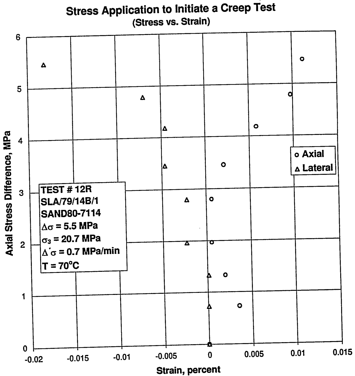
Figure B-70. Axial Stress Difference Versus Axial and Lateral Strain for Stress Application to Initiate a Creep Test: Specimen SLA/79/14B/1; Stage 1 of 1.
