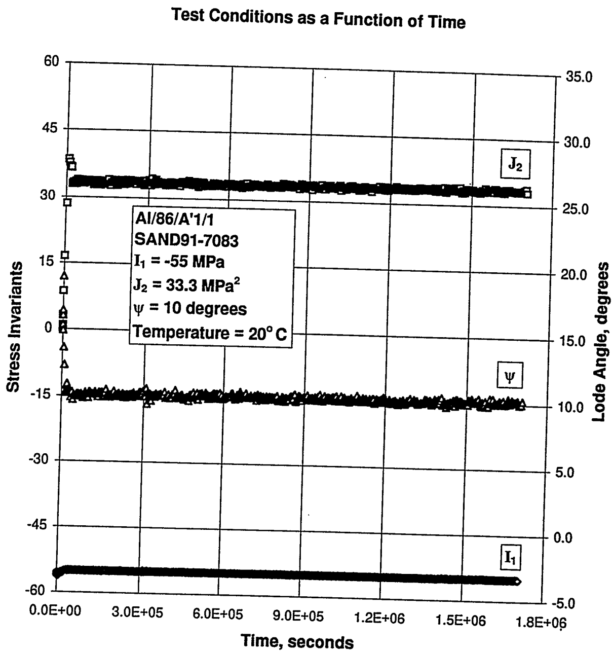
Figure D-5. Test Conditions Versus Time for a Multiaxial Creep Test: Specimen AI/86/A'1/1.
