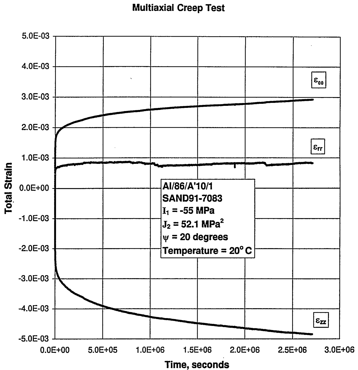
Figure D-14. Principal Strains Versus Time for a Multiaxial Creep Test: Specimen AI/86/A'10/1.
