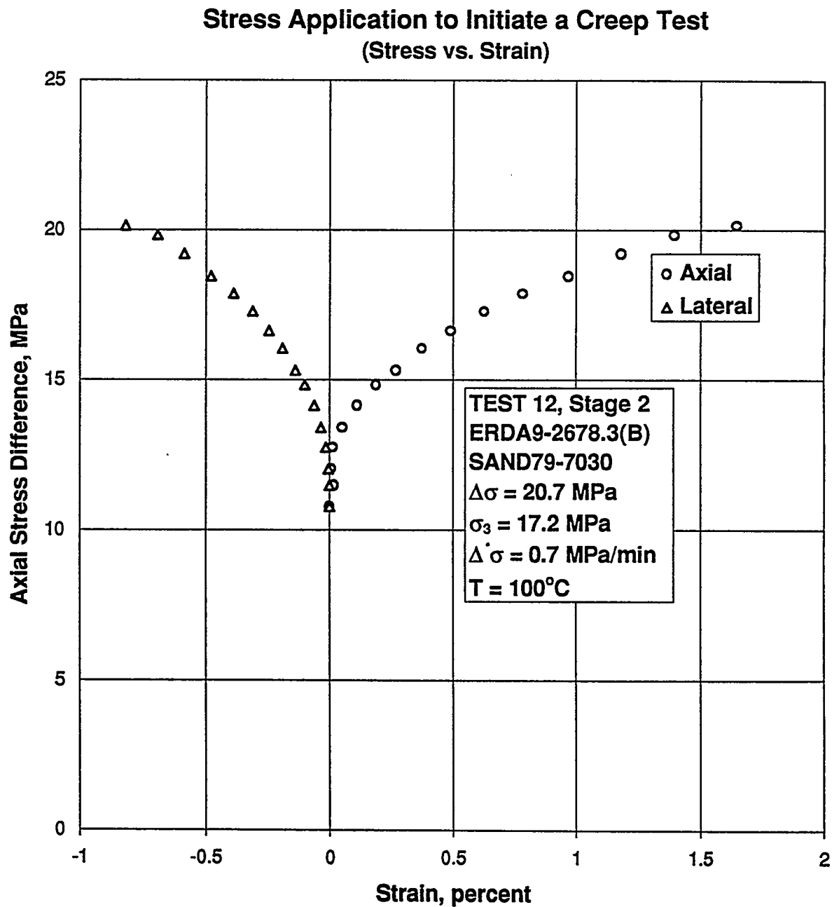
Figure B-132. Axial Stress Difference Versus Axial and Lateral Strain for Stress Application to Initiate a Creep Test: Specimen ERDA9-2678.3 (B); Stage 2 of 2.
