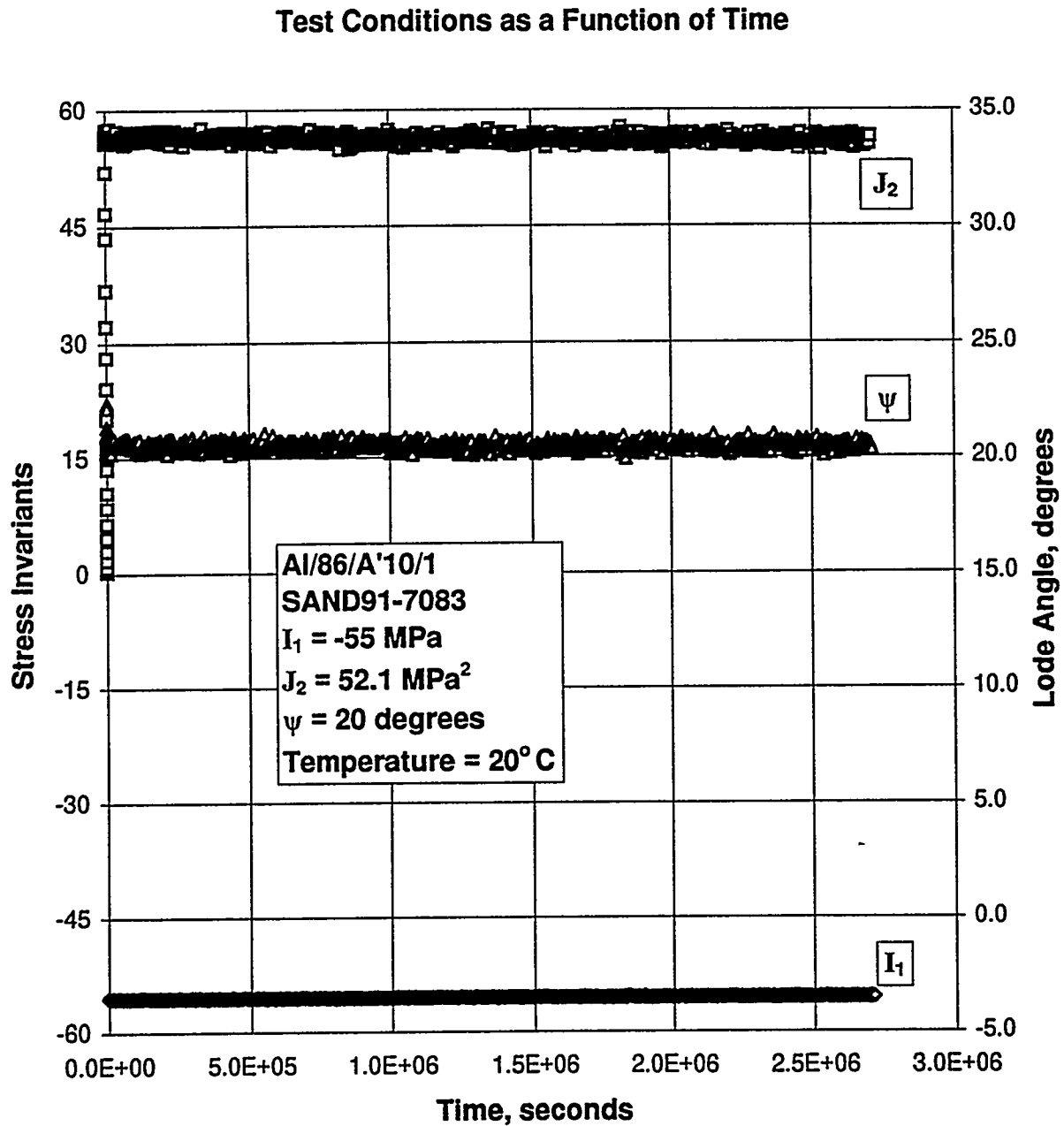
Figure D-13. Test Conditions Versus Time for a Multiaxial Creep Test: Specimen AI/86/A'10/1.
