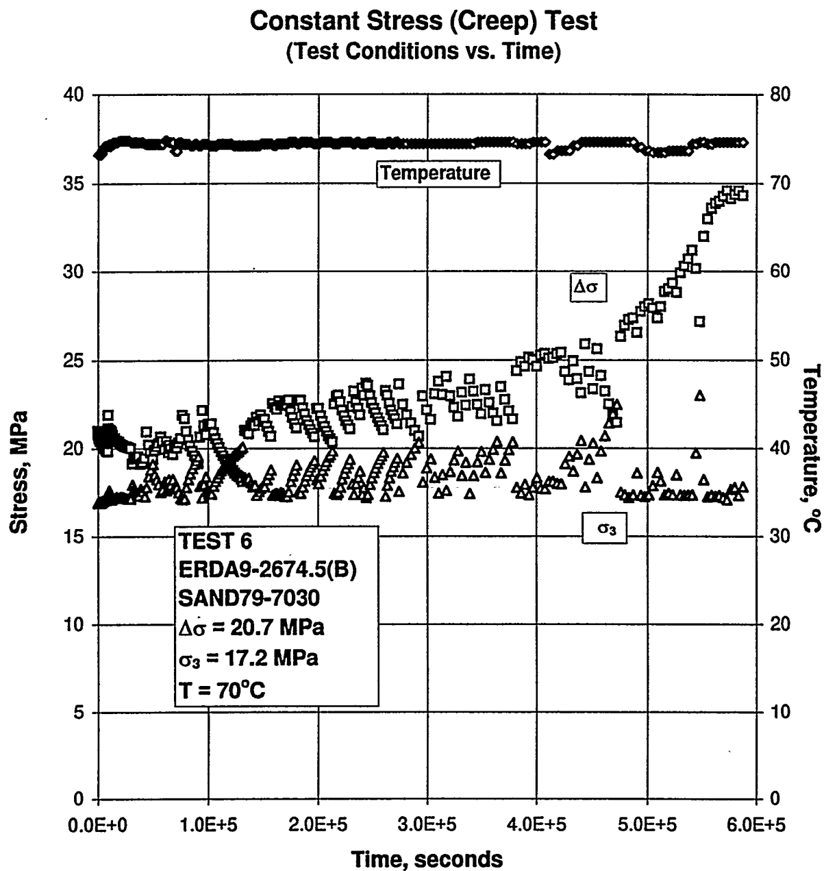
Figure B-95. Test Conditions Versus Time for a Creep Test: Specimen ERDA9-2674.5 (B); Stage 1 of 1 (Specimen Contacted Vessel Wall at 150 Hours).
