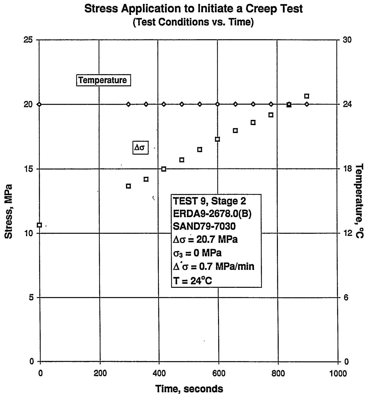
Figure B-109. Test Conditions Versus Time for Stress Application to Initiate a Creep Test: Specimen ERDA9-2678.0 (B); Stage 2 of 2.
