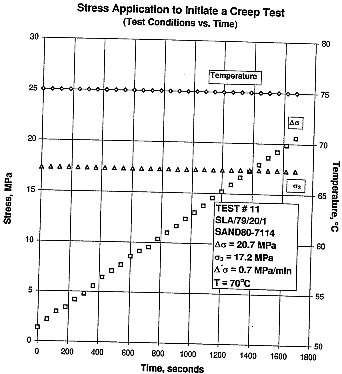
Figure B-61. Test Conditions Versus Time for Stress Application to Initiate a Creep Test: Specimen SLA/79/20/1; Stage 1 of 1.
