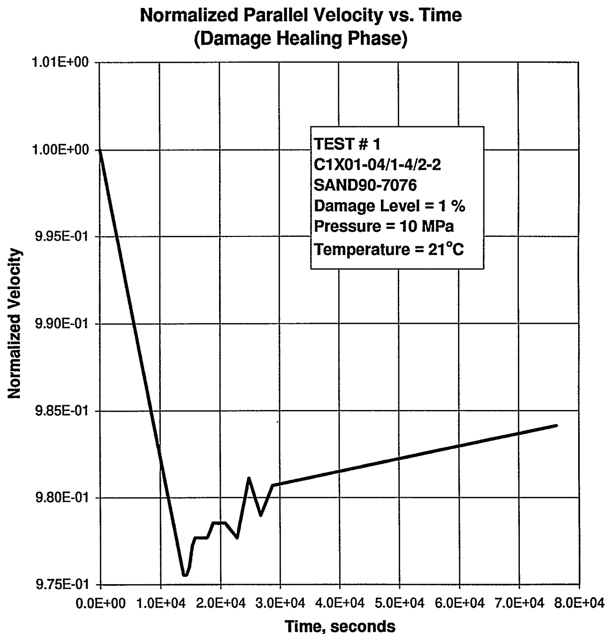
Figure E-46. Normalized Parallel Velocity as a Function of Time During the Hydrostatic Loading to Recover Damage in Specimen C1X01-04/1-4/2-2.
