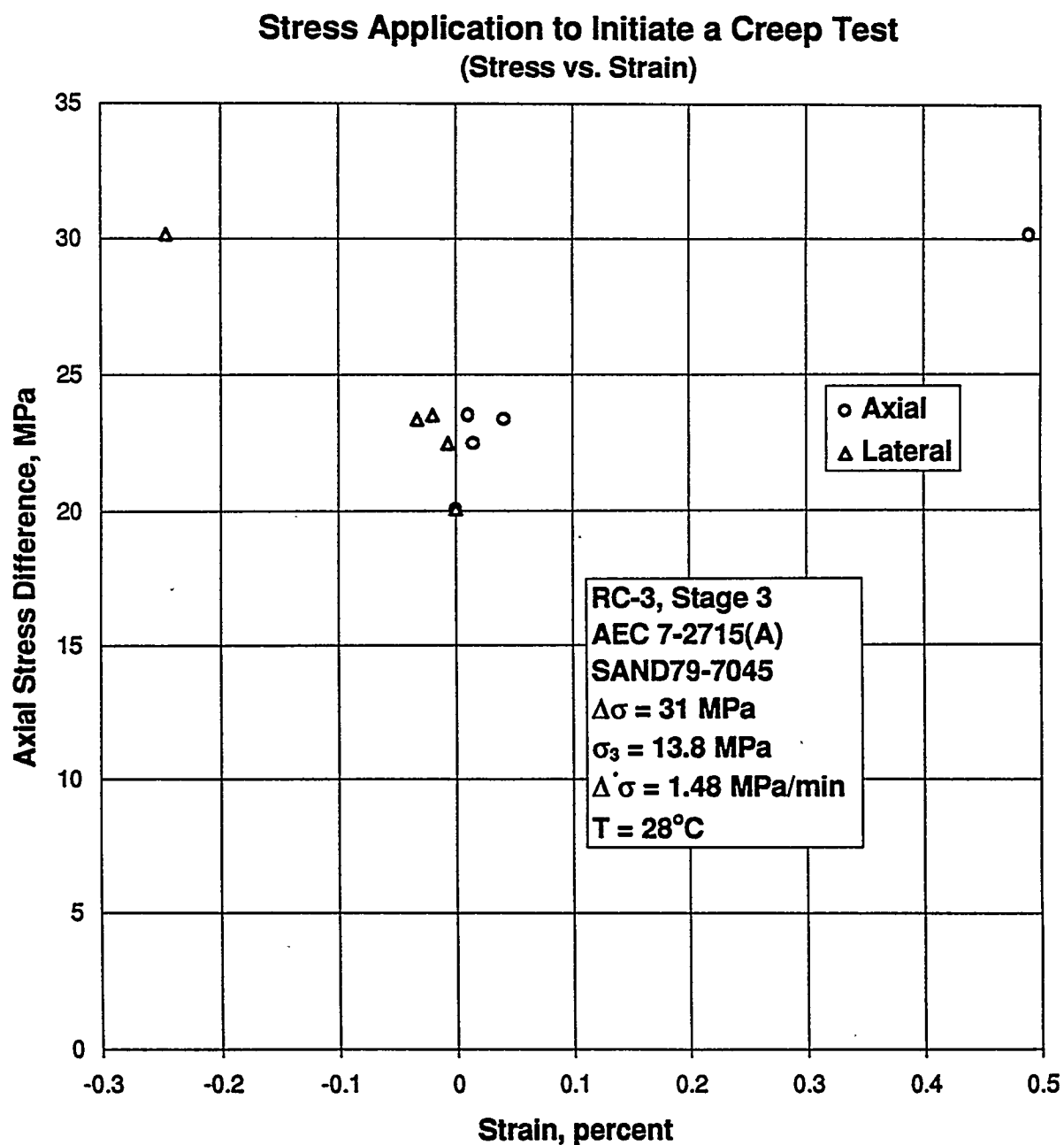
Figure B-172. Axial Stress Difference Versus Axial and Lateral Strain for Stress Application to Initiate a Creep Test: Specimen AEC7-2715 (A); Stage 3 of 3.
