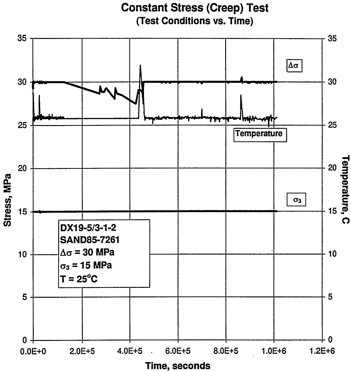
Figure C-75. Test Conditions Versus Time for a Creep Test: Specimen DX19-5/3-1-2; Stage 1 of 1.
