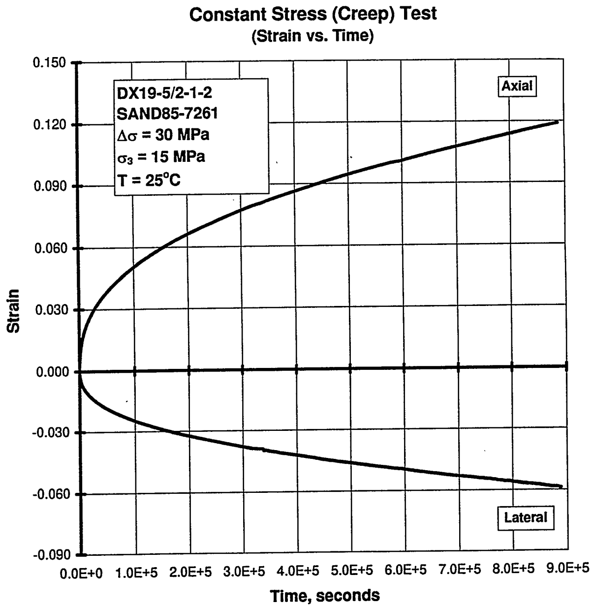
Figure C-74. Axial Strain and Lateral Strain Versus Time for a Creep Test: Specimen DX19-5/2-1-2; Stage 1 of 1.
