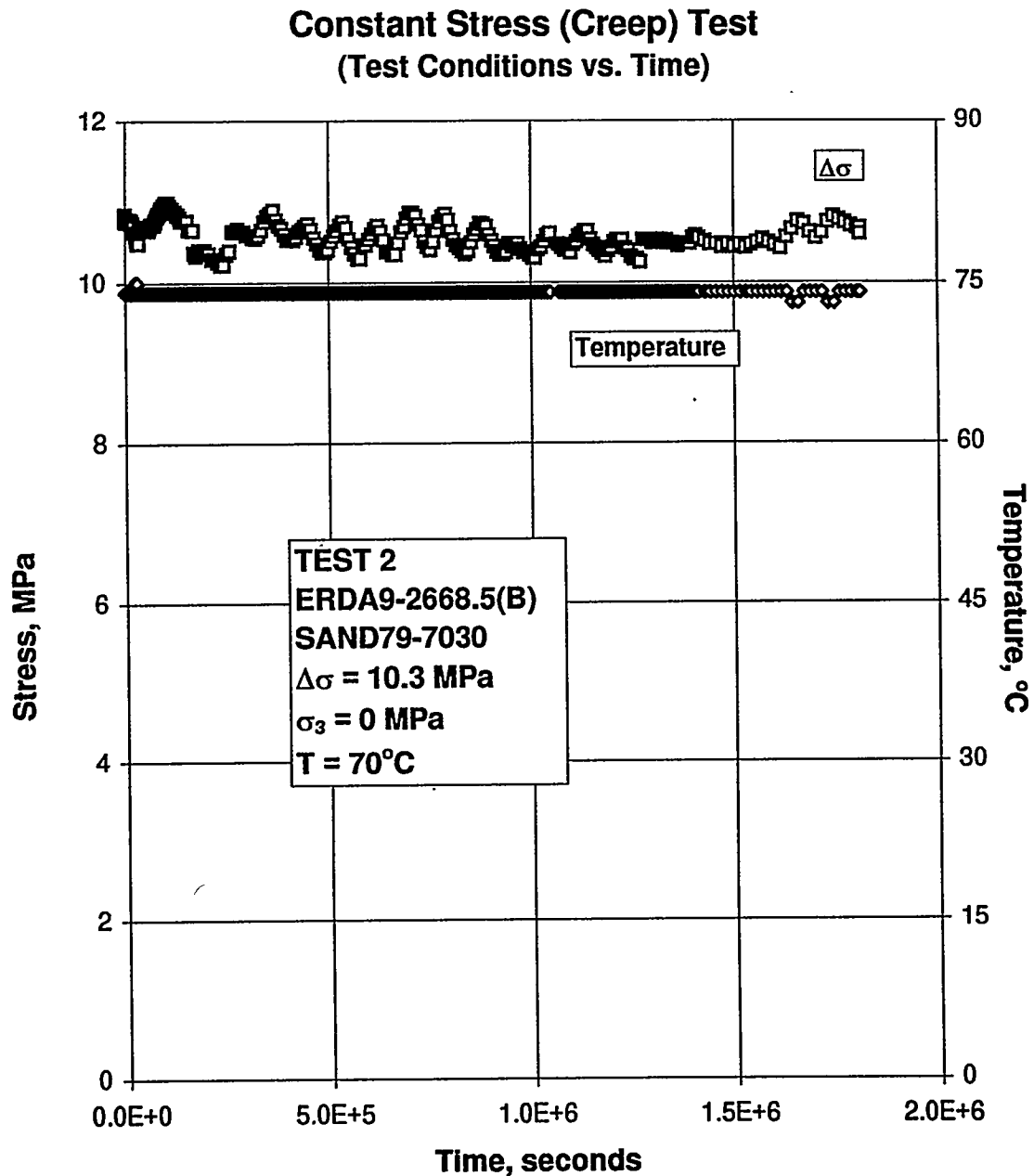
Figure B-79. Test Conditions Versus Time for a Creep Test: Specimen ERDA9-2668.5 (B); Stage 1 of 1.
