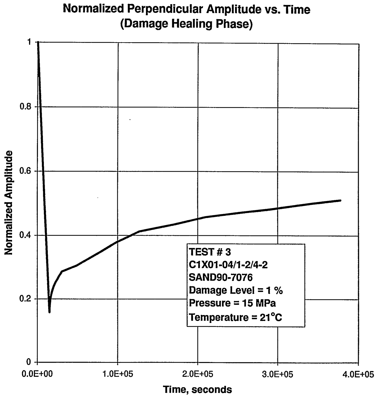
Figure E-67. Normalized Perpendicular Amplitude as a Function of Time During the Hydrostatic Loading to Recover Damage in Specimen C1X01-04/1-2/4-2.
