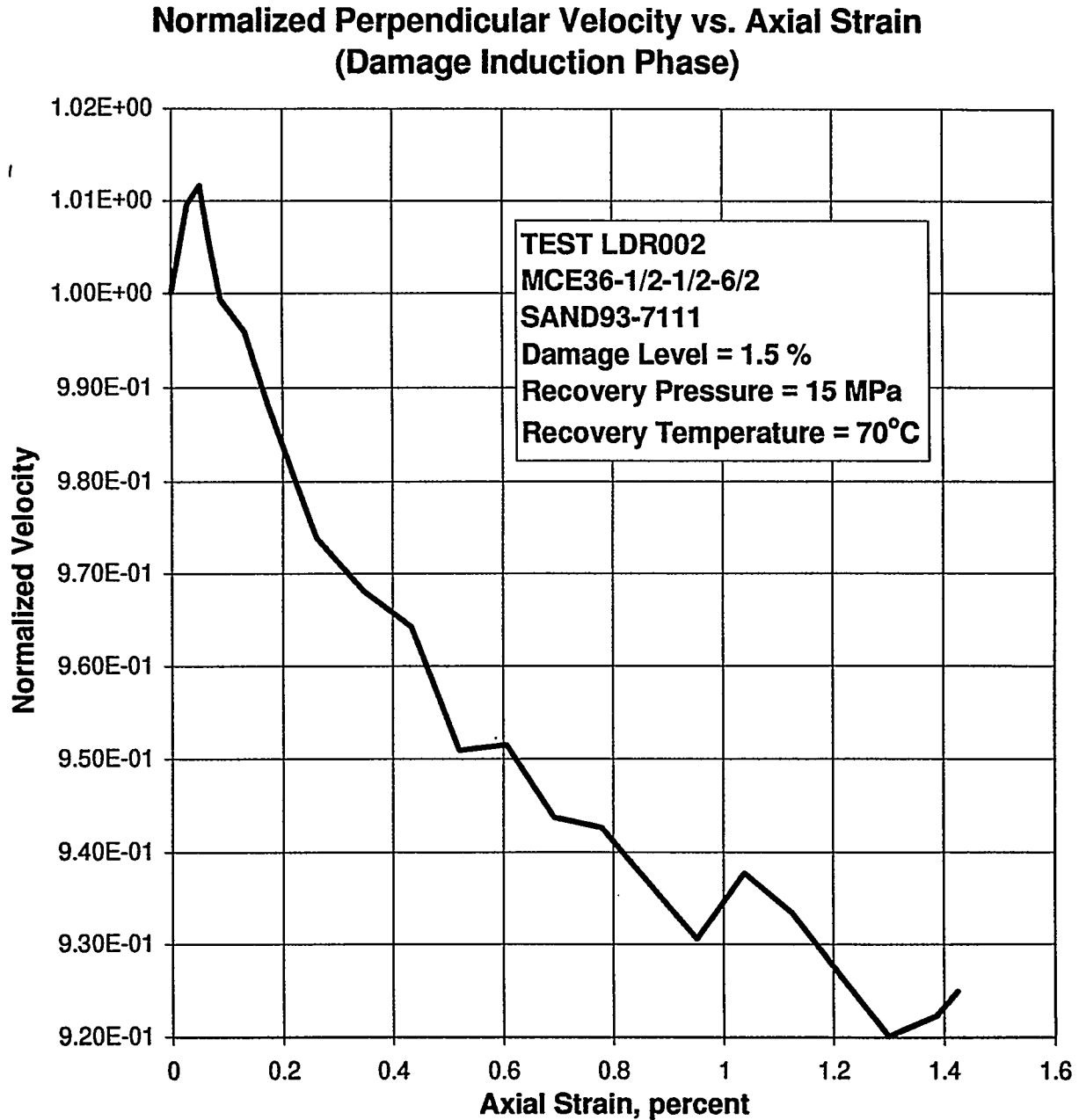
Figure E-10. Normalized Perpendicular Velocity as a Function of Axial Strain During the Quasi-Static Loading to Induce Damage in Specimen MCE36-1/2-1/2-6/2.
