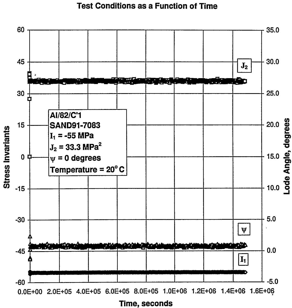
Figure D-1. Test Conditions Versus Time for a Multiaxial Creep Test: Specimen AI/82/C'1.
