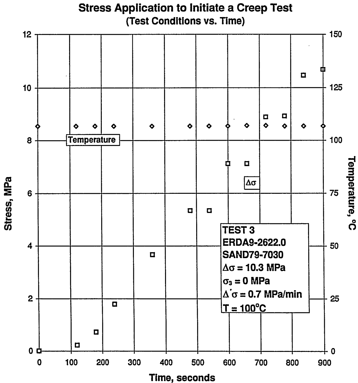
Figure B-81. Test Conditions Versus Time for Stress Application to Initiate a Creep Test: Specimen ERDA9-2622.0; Stage 1 of 1.
