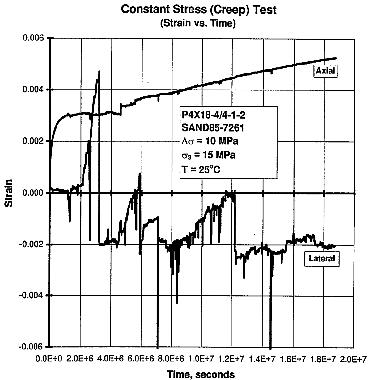
Figure C-38. Axial Strain and Lateral Strain Versus Time for a Creep Test: Specimen P4X18-4/4-1-2; Stage 1 of 1 (Argillaceous Salt).
