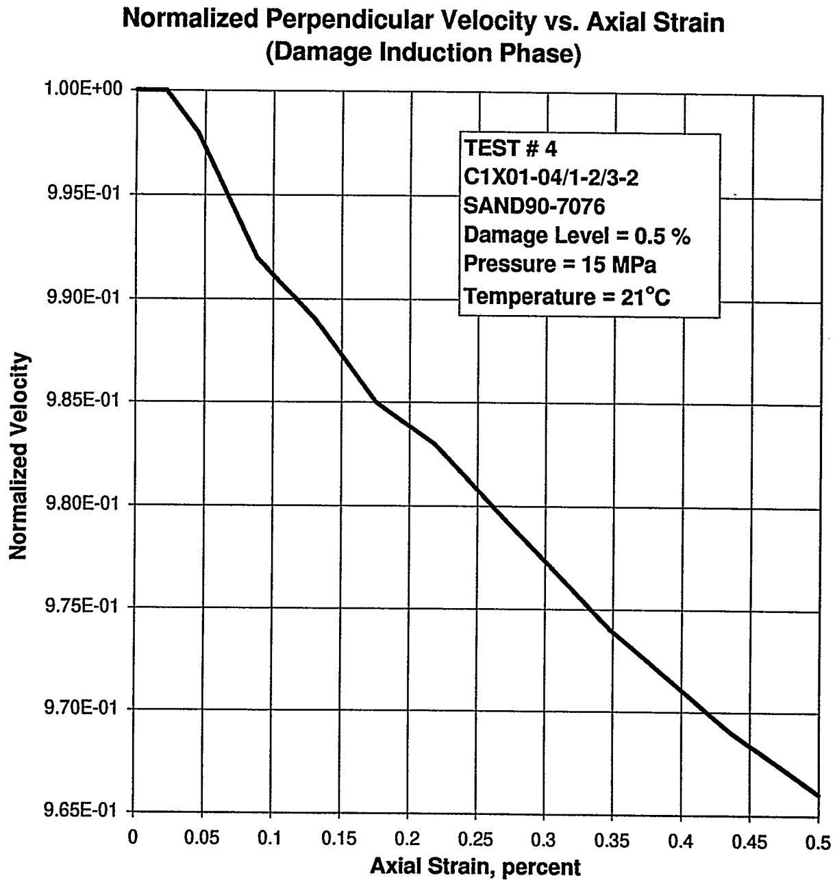
Figure E-75. Normalized Perpendicular Velocity as a Function of Axial Strain During the Quasi-Static Loading to Induce Damage in Specimen C1X01-04/1-2/3-2.
