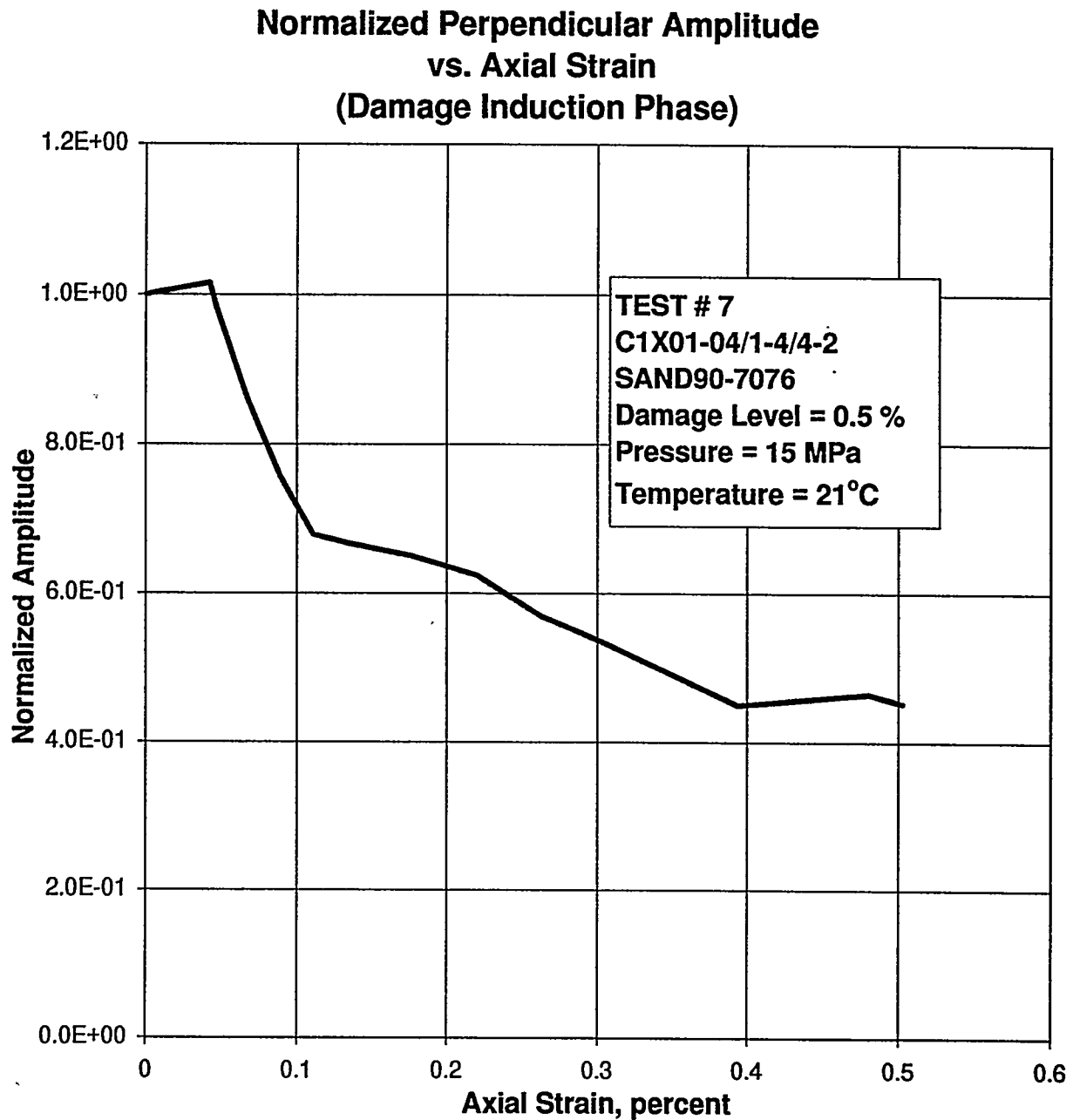
Figure E-109. Normalized Perpendicular Amplitude as a Function of Axial Strain During the Quasi-Static Loading to Induce Damage in Specimen C1X01-04/1-4/4-2.
