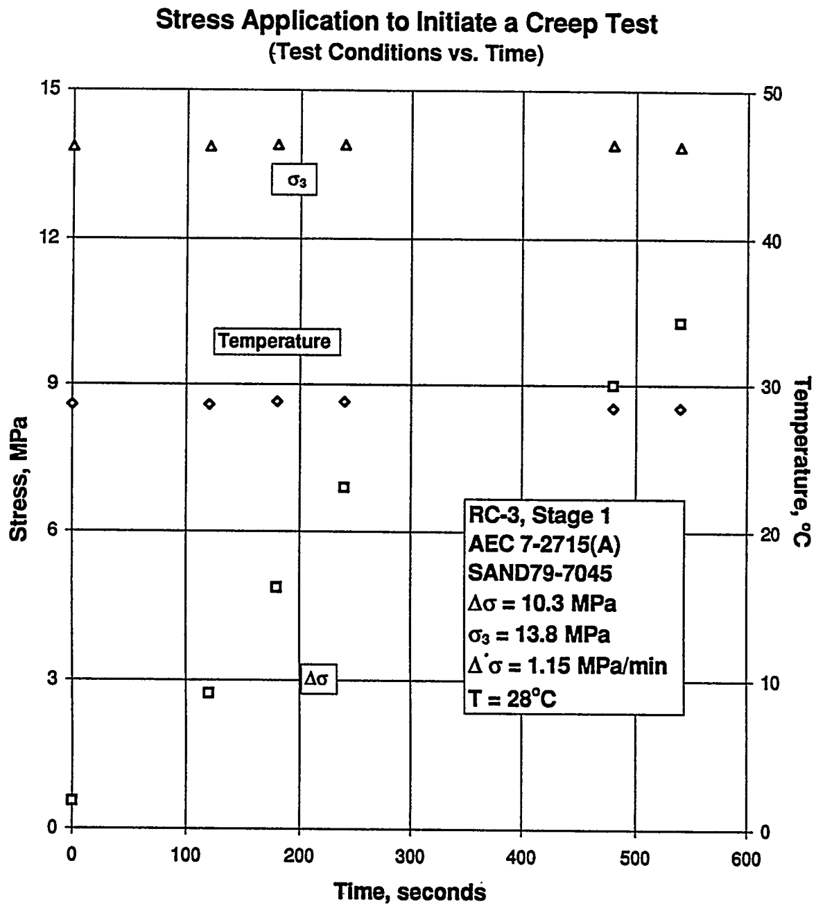
Figure B-163. Test Conditions Versus Time for Stress Application to Initiate a Creep Test: Specimen AEC7-2715 (A); Stage 1 of 3.
