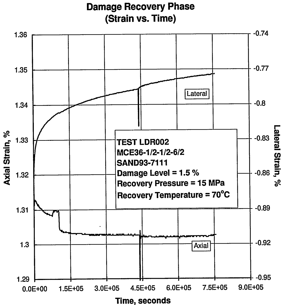
Figure E-13. Axial and Lateral Strain as a Function of Time During the Hydrostatic Loading to Recover Damage in Specimen MCE36-1/2-1/2-6/2.
