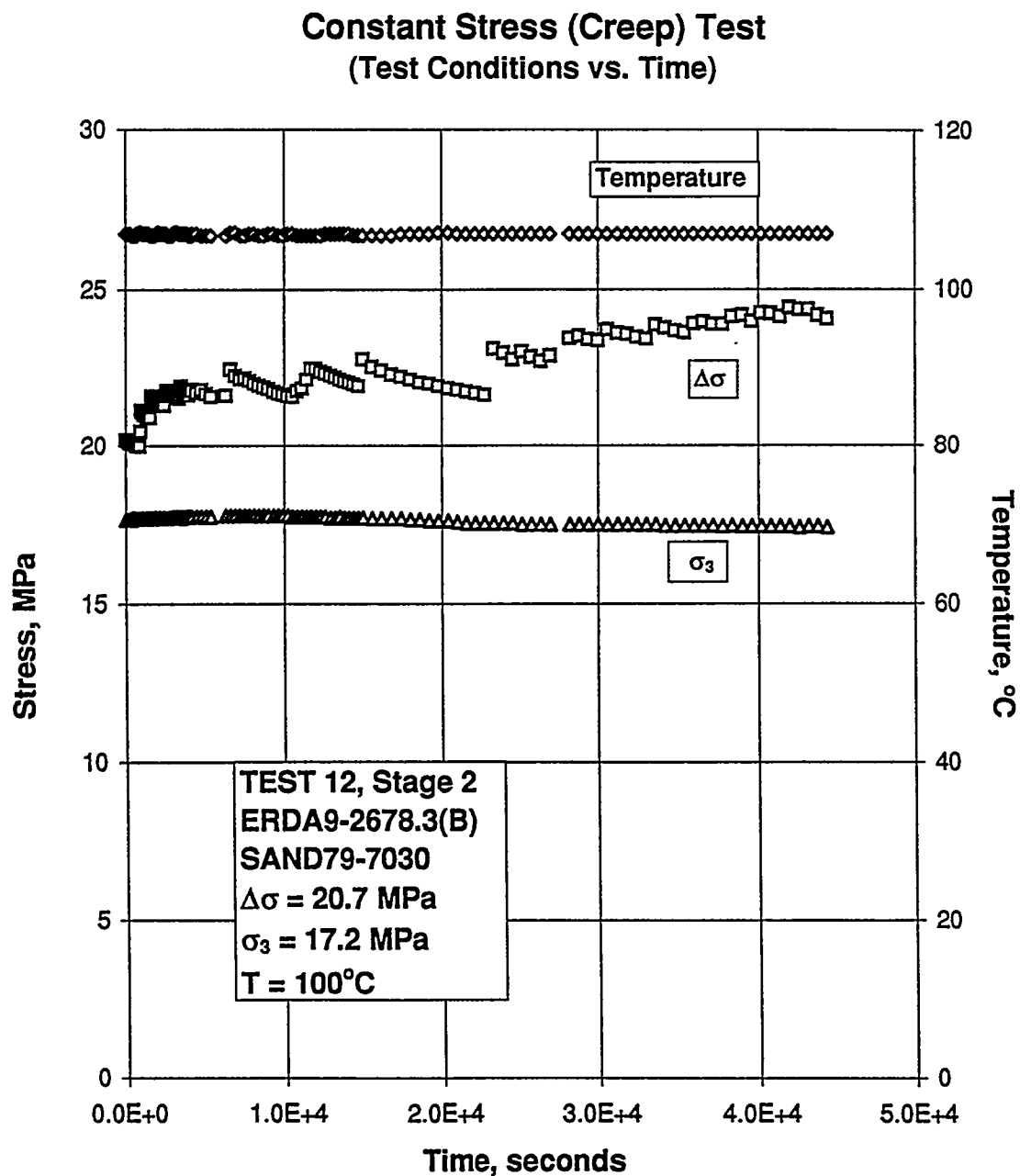
Figure B-133. Test Conditions Versus Time for a Creep Test: Specimen ERDA9-2678.3 (B); Stage 2 of 2.
