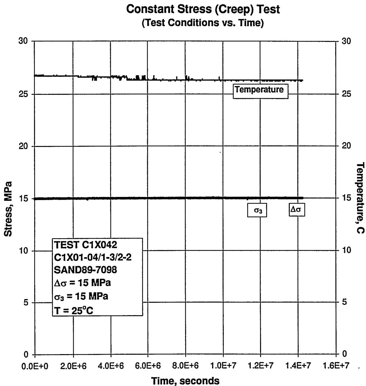
Figure C-33. Test Conditions Versus Time for a Creep Test: Specimen C1X01-04/1-3/2-2; Stage 1 of 1.
