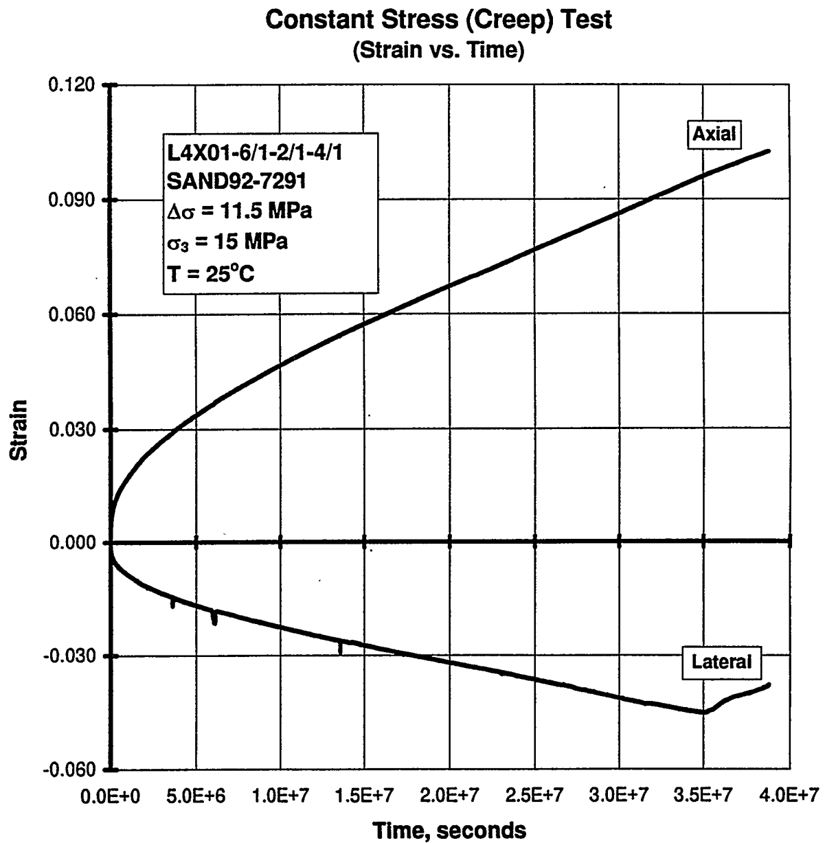
Figure C-18. Axial Strain and Lateral Strain Versus Time for a Creep Test: Specimen L4X01-6/1-2/1-4/1; Stage 1 of 1 (Argillaceous Salt).
