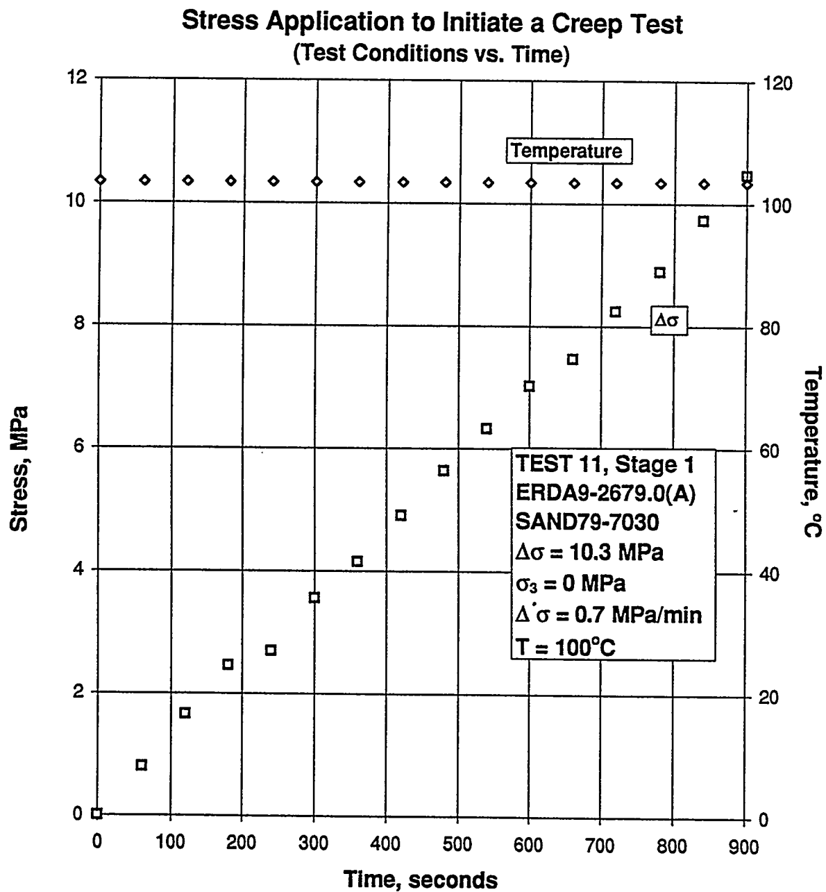
Figure B-121. Test Conditions Versus Time for Stress Application to Initiate a Creep Test: Specimen ERDA9-2679.0 (A); Stage 1 of 2.
