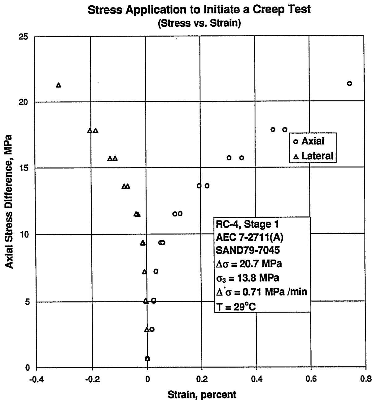
Figure B-176. Axial Stress Difference Versus Axial and Lateral Strain for Stress Application to Initiate a Creep Test: Specimen AEC7-2711 (A); Stage 1 of 2.
