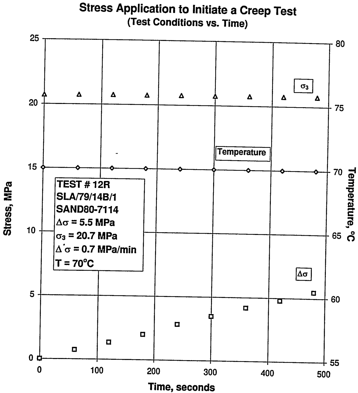
Figure B-69. Test Conditions Versus Time for Stress Application to Initiate a Creep Test: Specimen SLA/79/14B/1; Stage 1 of 1.
