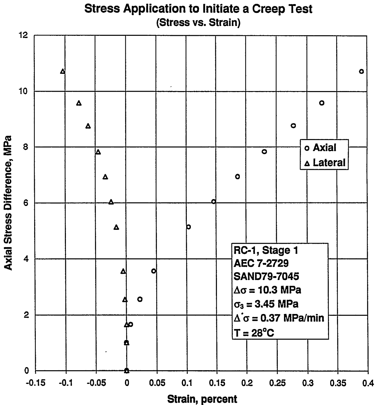
Figure B-144. Axial Stress Difference Versus Axial and Lateral Strain for Stress Application to Initiate a Creep Test: Specimen AEC7-2729; Stage 1 of 3.
