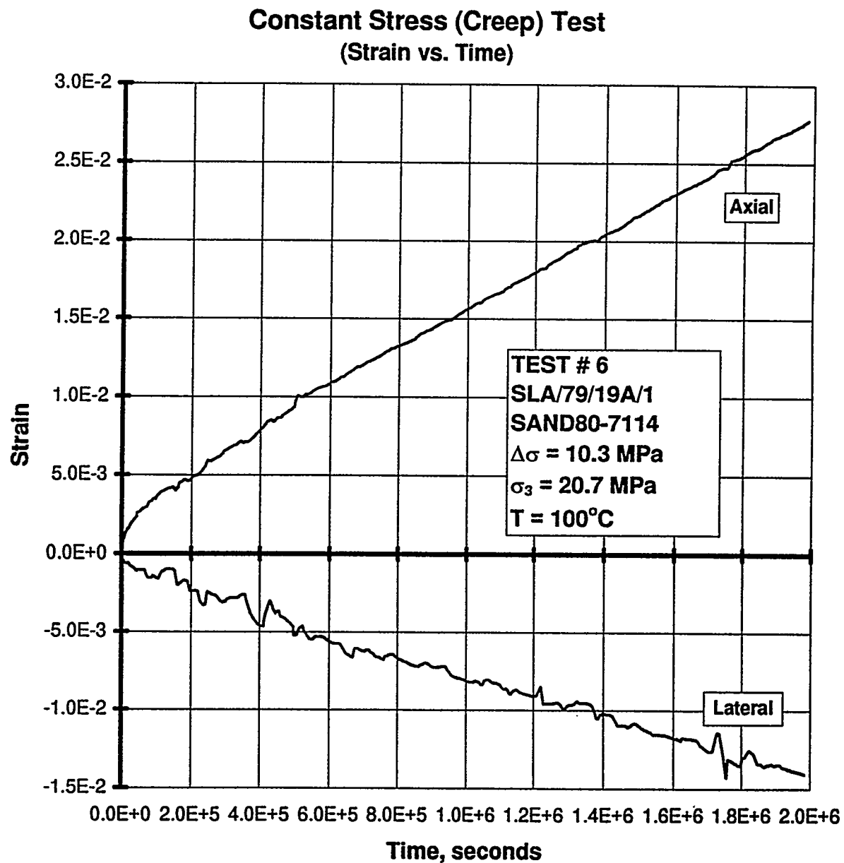
Figure B-44. Axial Strain and Lateral Strain Versus Time for a Creep Test: Specimen SLA/79/19A/1; Stage 1 of 1.
