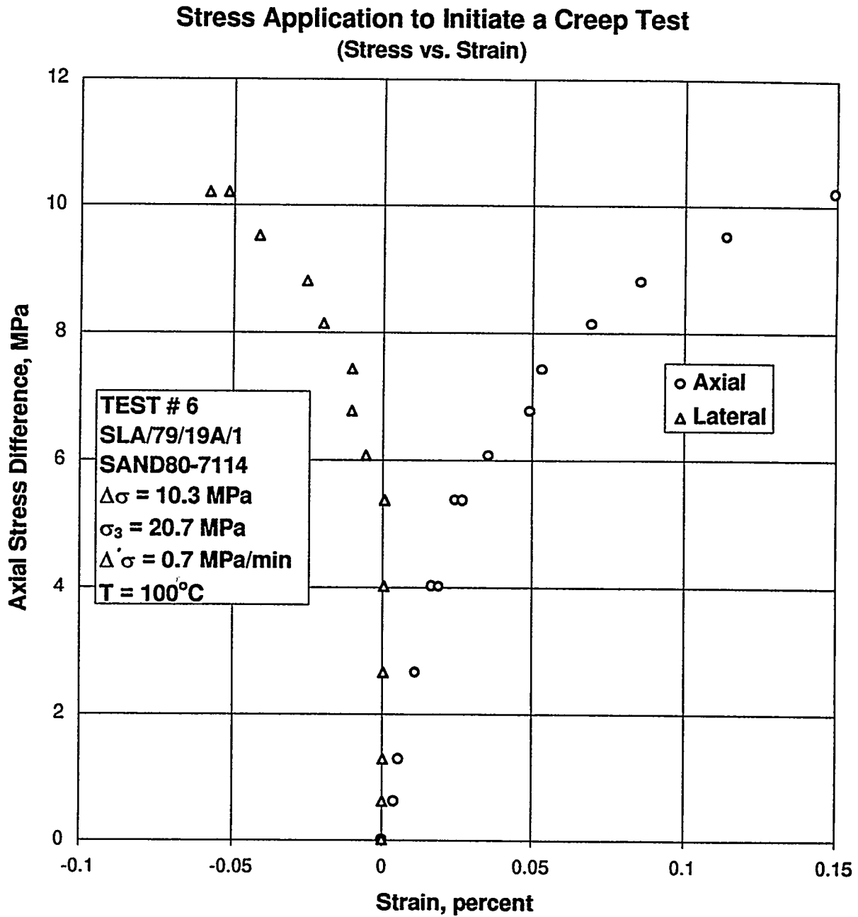
Figure B-42. Axial Stress Difference Versus Axial and Lateral Strain for Stress Application to Initiate a Creep Test: Specimen SLA/79/19A/1; Stage 1 of 1.
