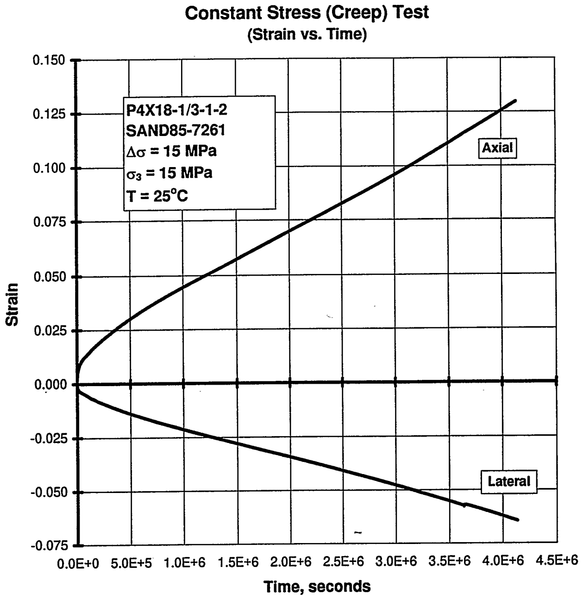
Figure C-42. Axial Strain and Lateral Strain Versus Time for a Creep Test: Specimen P4X18-1/3-1-2; Stage 1 of 1 (Argillaceous Salt. Anomalous Test Result. Localized Deformation Along Clay Seams).
