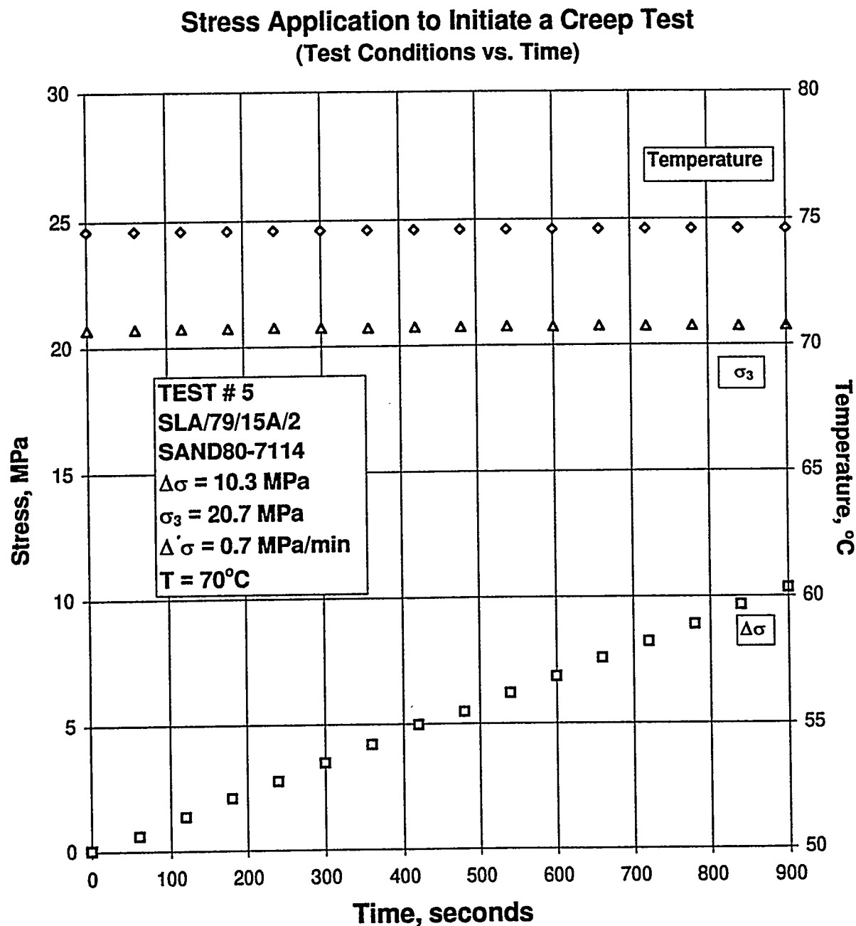
Figure B-37. Test Conditions Versus Time for Stress Application to Initiate a Creep Test: Specimen SLA/79/15A/2; Stage 1 of 1.
