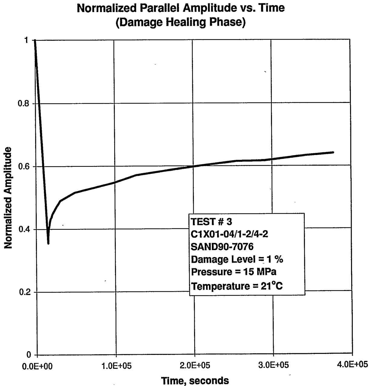
Figure E-68. Normalized Parallel Amplitude as a Function of Time During the Hydrostatic Loading to Recover Damage in Specimen C1X01-04/1-2/4-2.
