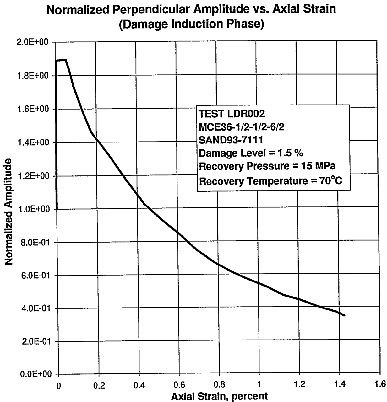
Figure E-9. Normalized Perpendicular Amplitude as a Function of Axial Strain During the Quasi-Static Loading to Induce Damage in Specimen MCE36-1/2-1/2-6/2.
