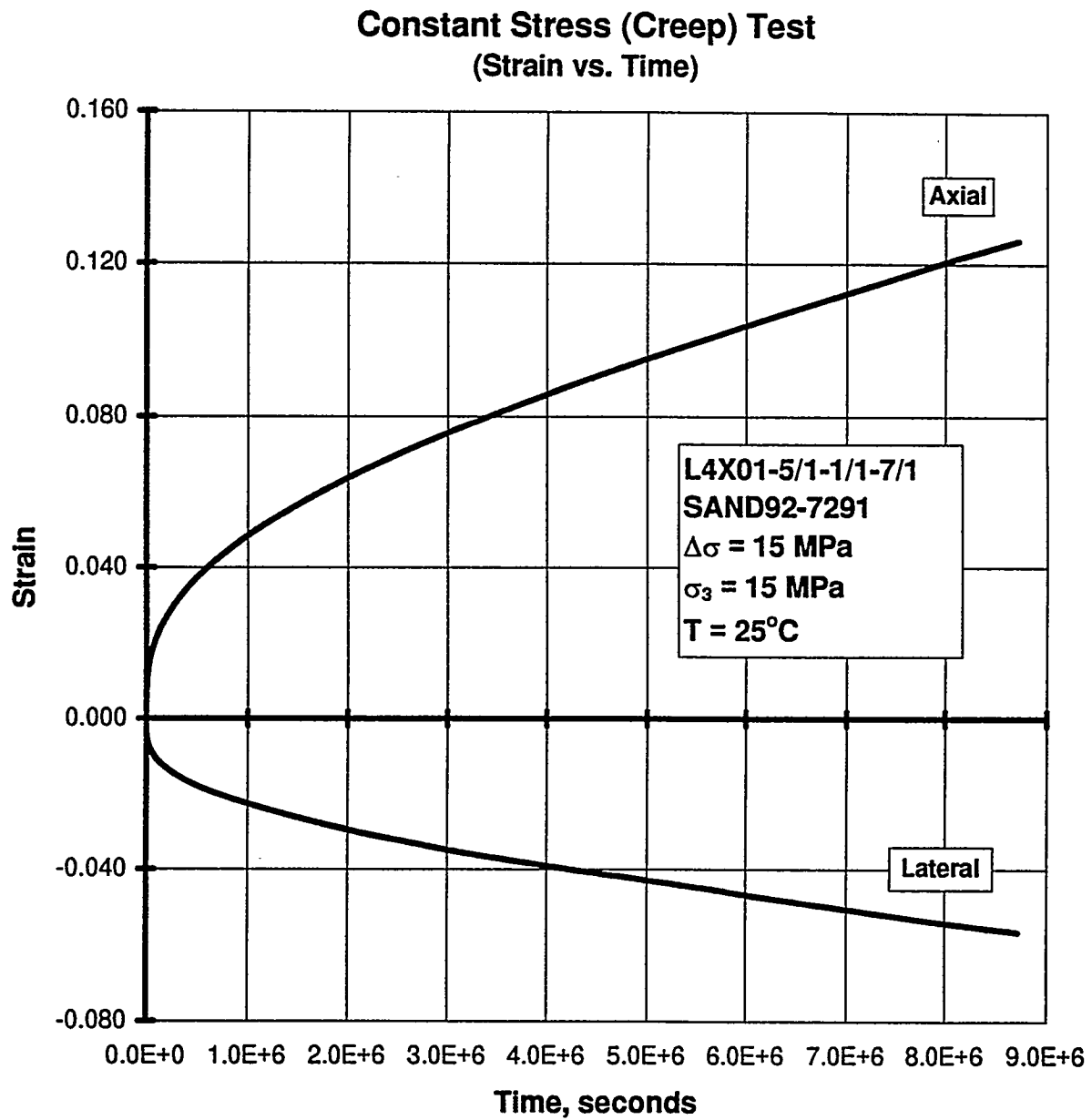
Figure C-24. Axial Strain and Lateral Strain Versus Time for a Creep Test: Specimen L4X01-5/1-1/1-7/1; Stage 1 of 1 (Argillaceous Salt).
