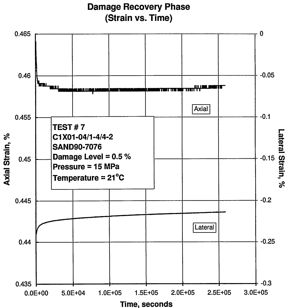
Figure E-114. Axial and Lateral Strain as a Function of Time During the Hydrostatic Loading to Recover Damage in Specimen C1X01-04/1-4/4-2.
