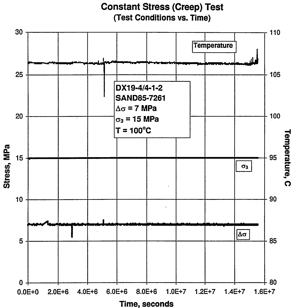
Figure C-79. Test Conditions Versus Time for a Creep Test: Specimen DX19-4/4-1-2; Stage 1 of 1.
