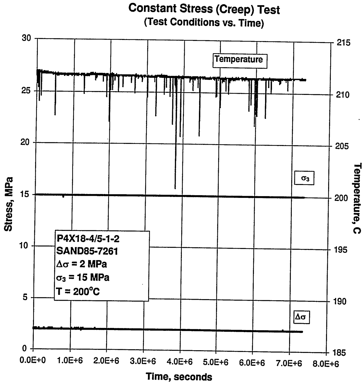
Figure C-51. Test Conditions Versus Time for a Creep Test: Specimen P4X18-4/5-1-2; Stage 1 of 1 (Argillaceous Salt).
