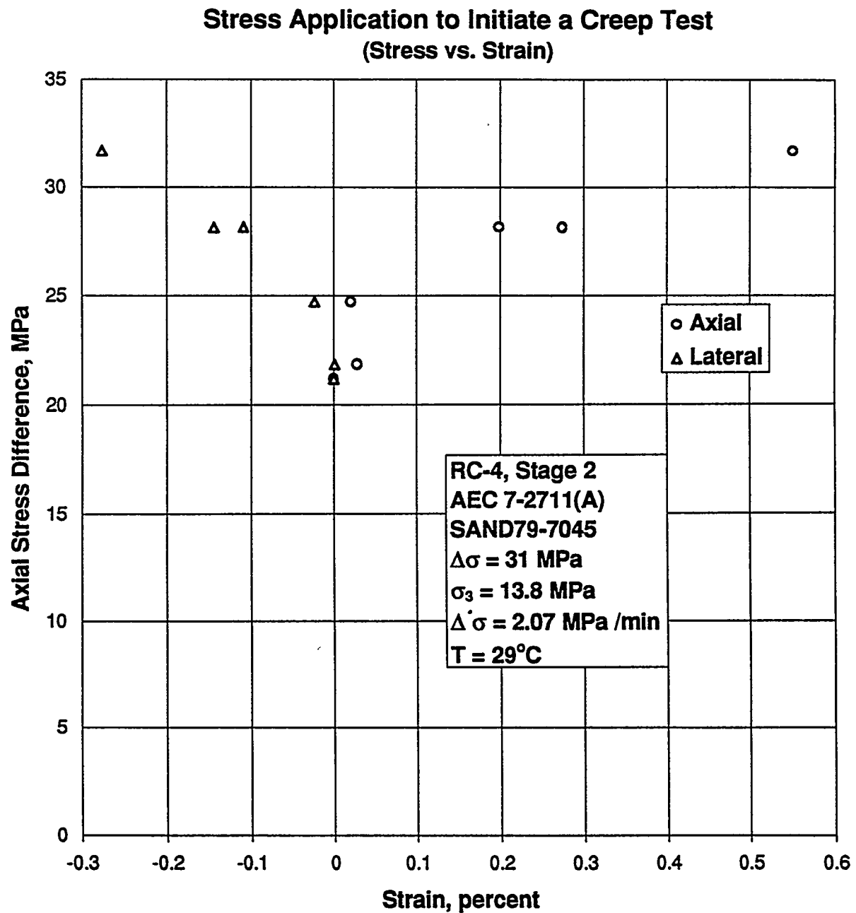
Figure B-180. Axial Stress Difference Versus Axial and Lateral Strain for Stress Application to Initiate a Creep Test: Specimen AEC7-2711 (A); Stage 2 of 2.
