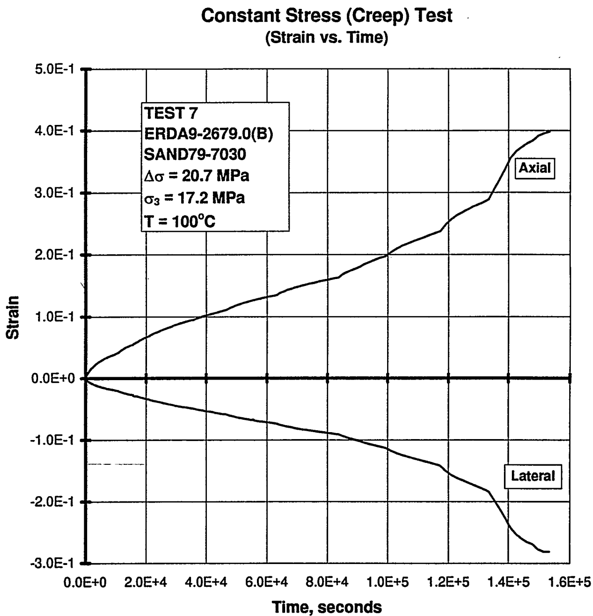
Figure B-100. Axial Strain and Lateral Strain Versus Time for a Creep Test: Specimen ERDA9-2679.0 (B); Stage 1 of 1 (Specimen Contacted Vessel Wall at End of Test).
