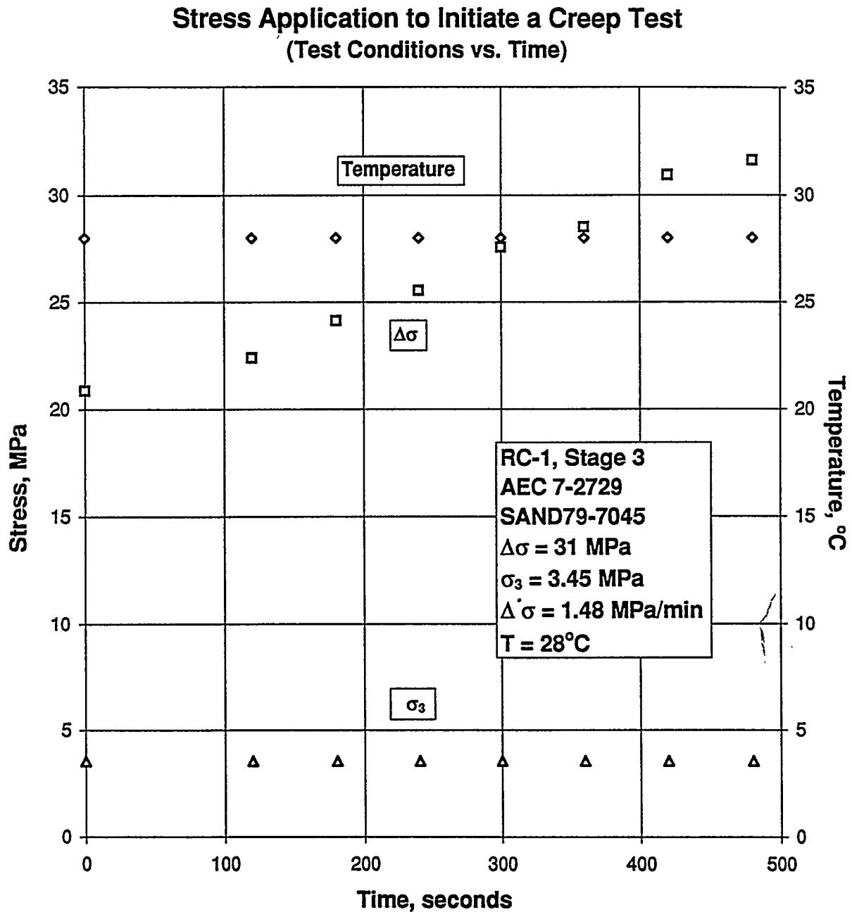
Figure B-151. Test Conditions Versus Time for Stress Application to Initiate a Creep Test: Specimen AEC7-2729; Stage 3 of 3.
