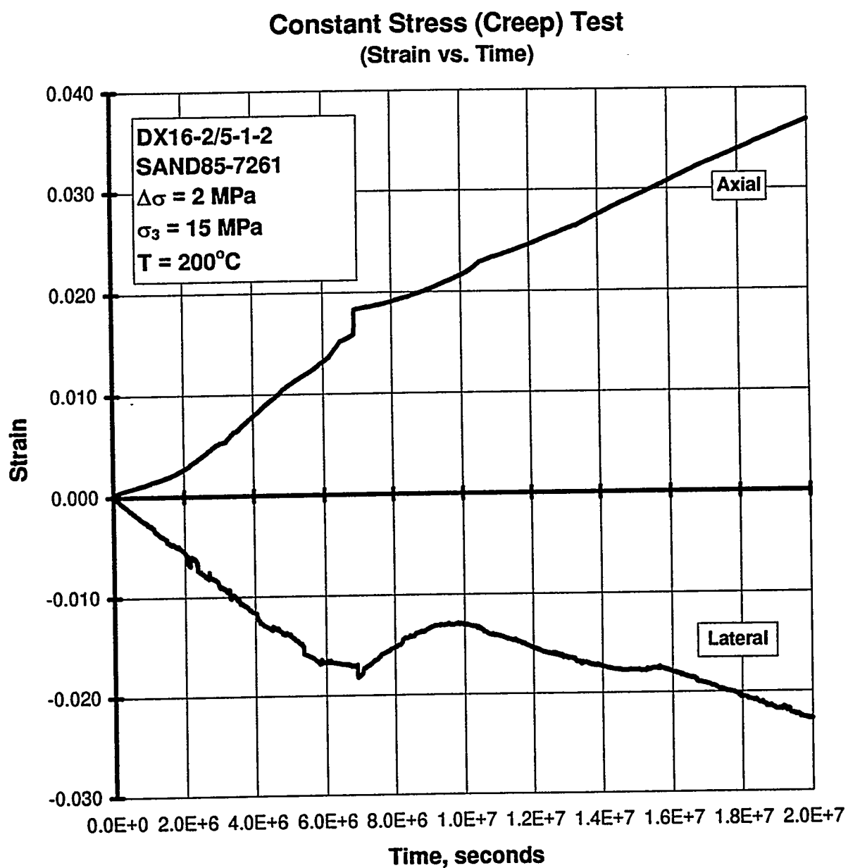
Figure C-86. Axial Strain and Lateral Strain Versus Time for a Creep Test: Specimen DX16-2/5-1-2; Stage 1 of 1 (Anomalous Test Result. Unknown Cause).
