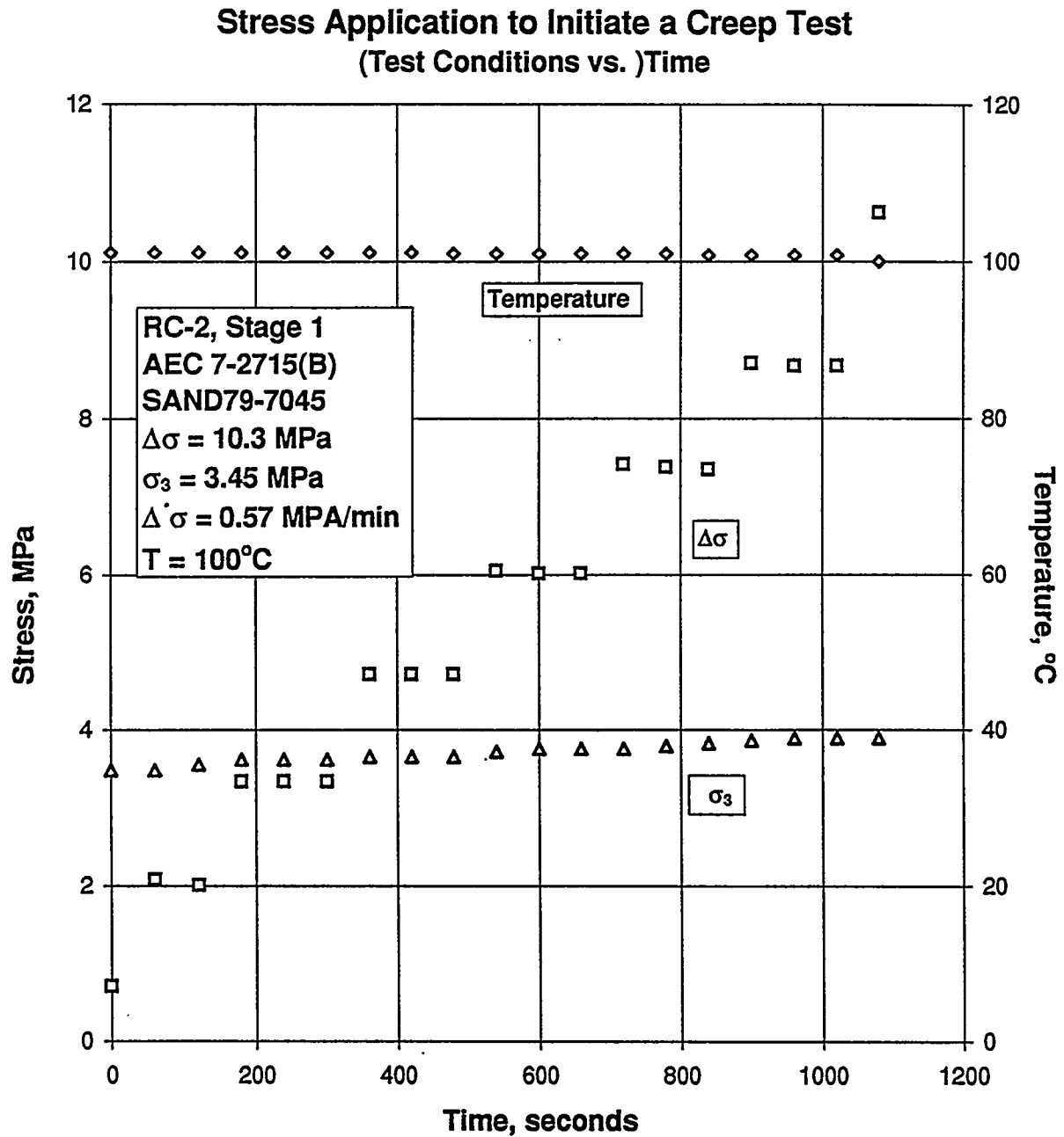
Figure B-155. Test Conditions Versus Time for Stress Application to Initiate a Creep Test: Specimen AEC7-2715 (B); Stage 1 of 2.
