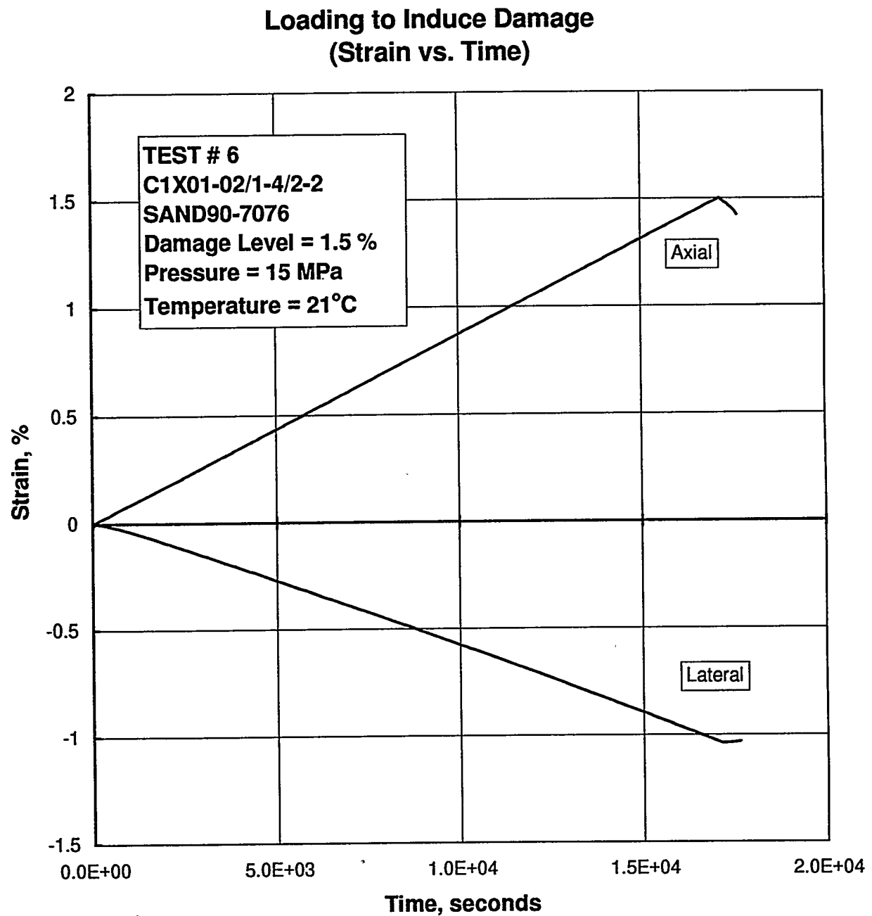
Figure E-96. Axial and Lateral Strain as a Function of Time During the Quasi-Static Loading to Induce Damage in Specimen C1X01-02/1-4/2-2.
