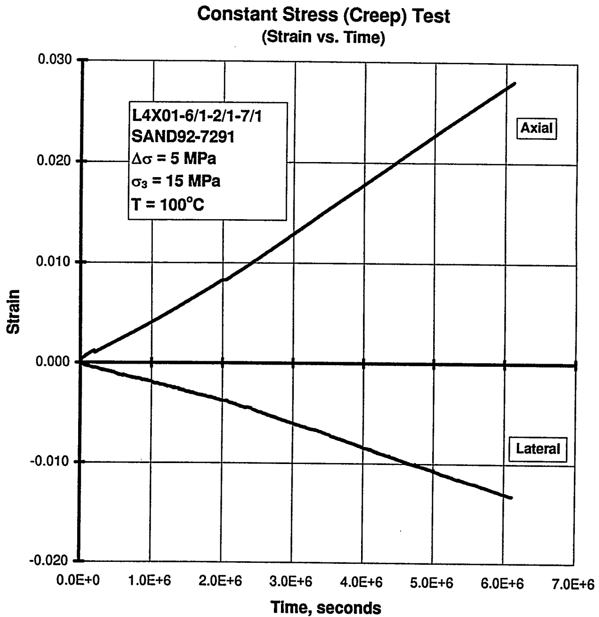
Figure C-28. Axial Strain and Lateral Strain Versus Time for a Creep Test: Specimen L4X01-6/1-2/1-7/1; Stage 1 of 1 (Argillaceous Salt).
