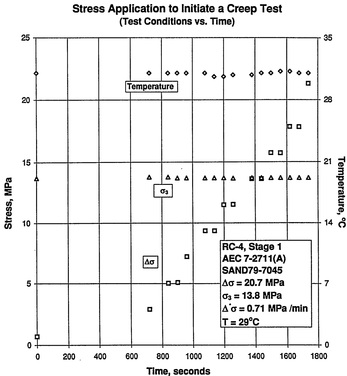
Figure B-175. Test Conditions Versus Time for Stress Application to Initiate a Creep Test: Specimen AEC7-2711 (A); Stage 1 of 2.
