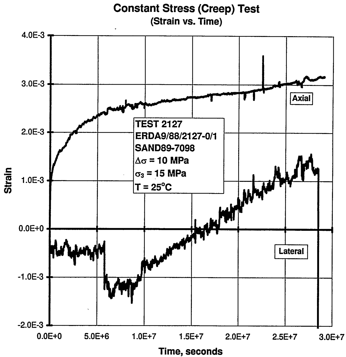
Figure B-2. Axial Strain and Lateral Strain Versus Time for a Creep Test: Specimen ERDA9/88/2127-0/1; Stage 1 of 1.
