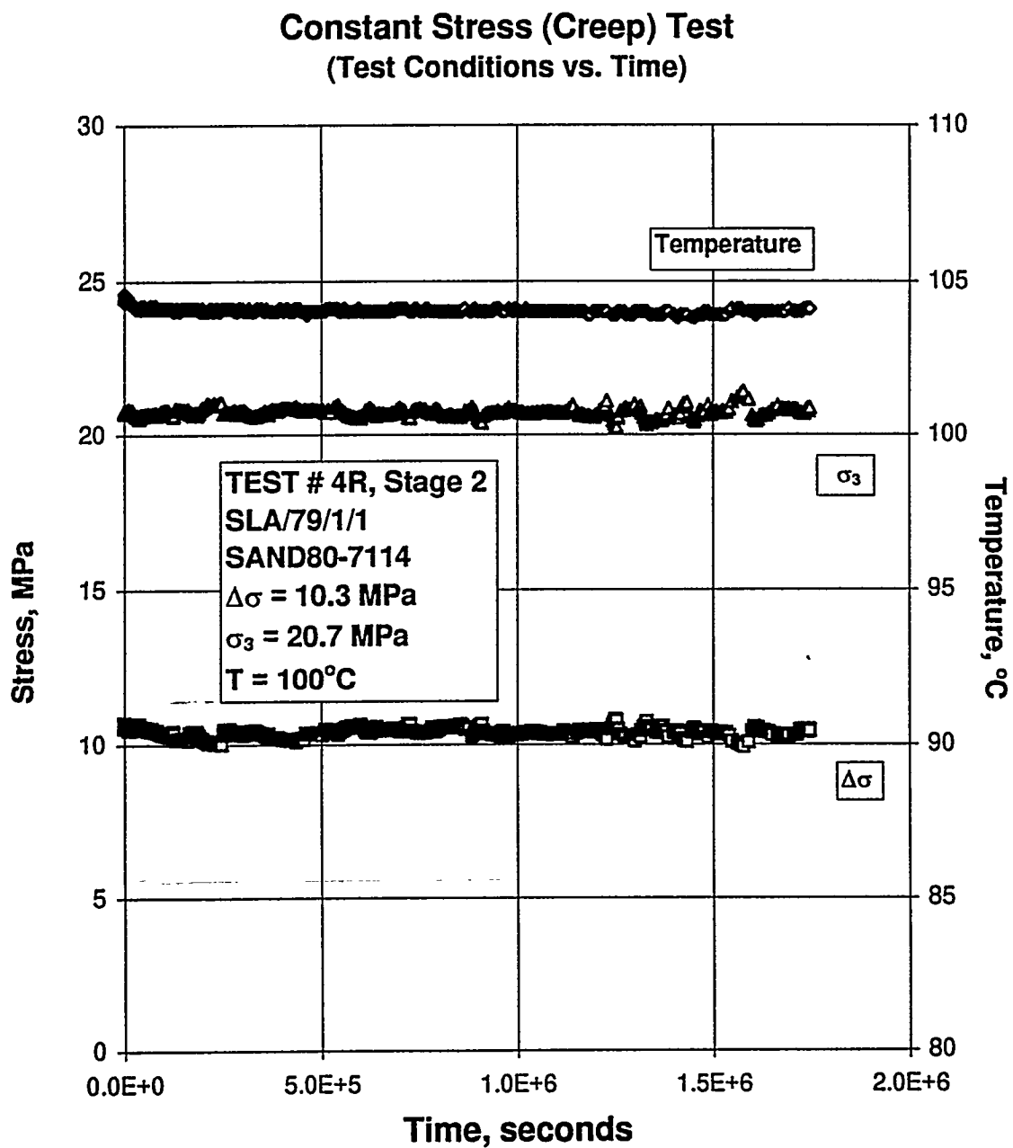
Figure B-35. Test Conditions Versus Time for a Creep Test: Specimen SLA/79/1/1; Stage 2 of 2.
