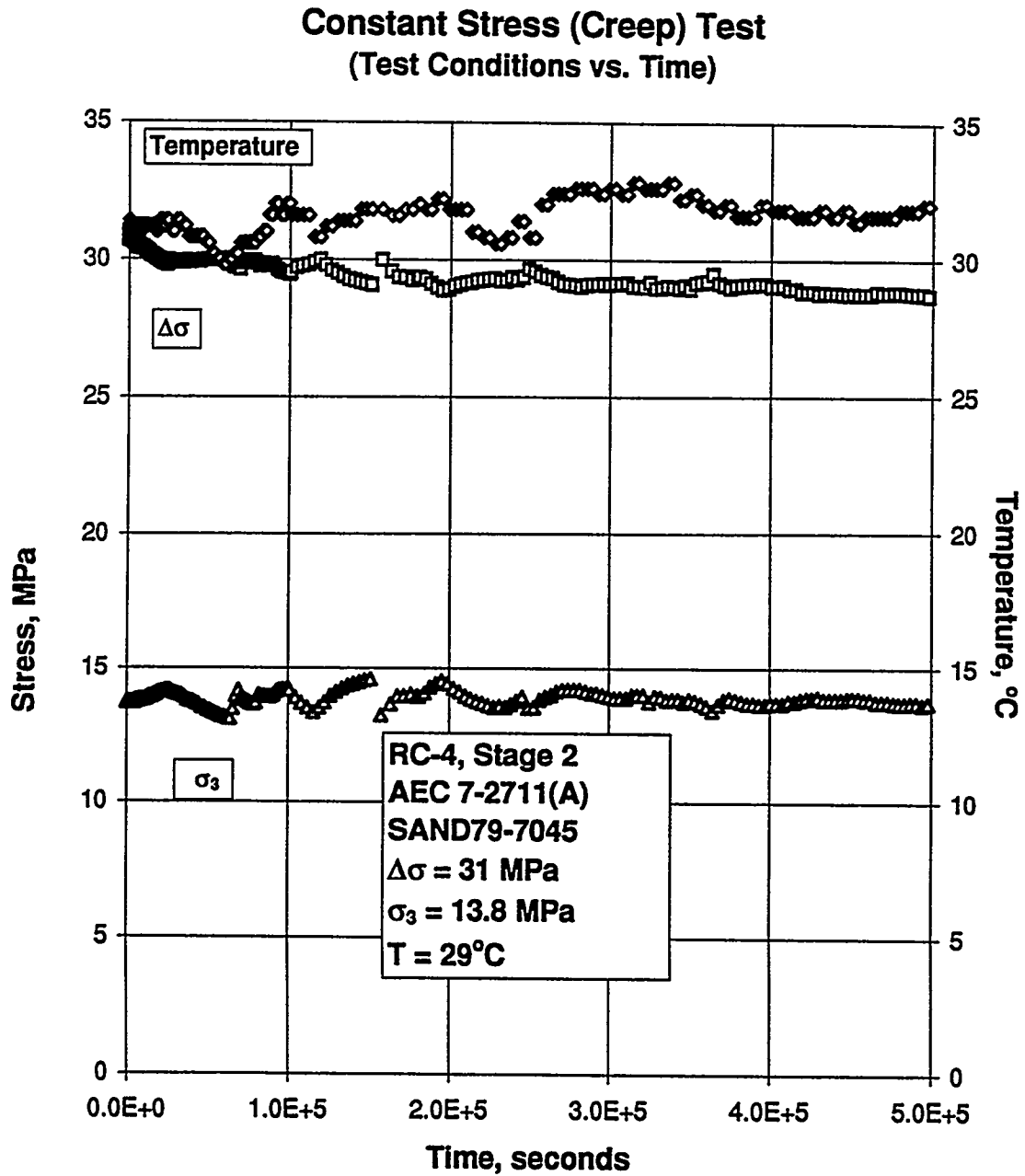
Figure B-181. Test Conditions Versus Time for a Creep Test: Specimen AEC7-2711 (A); Stage 2 of 2.
