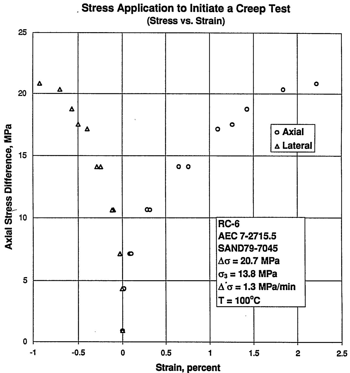
Figure B-192. Axial Stress Difference Versus Axial and Lateral Strain for Stress Application to Initiate a Creep Test: Specimen AEC7-2715.5; Stage 1 of 1.
