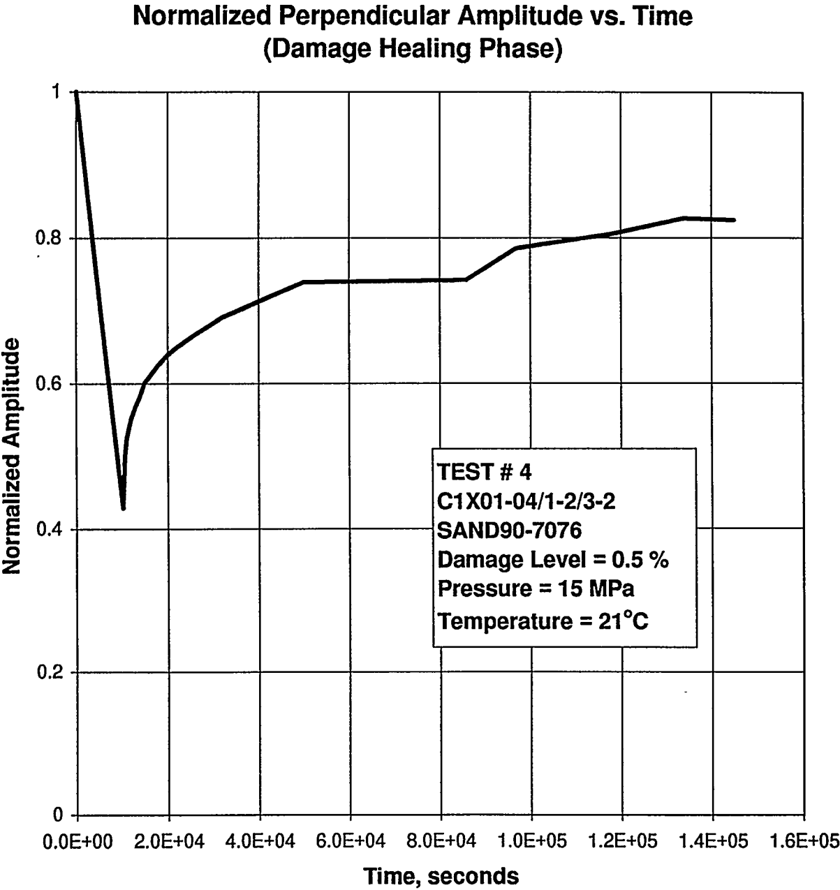
Figure E-79. Normalized Perpendicular Amplitude as a Function of Time During the Hydrostatic Loading to Recover Damage in Specimen C1X01-04/1-2/3-2.
