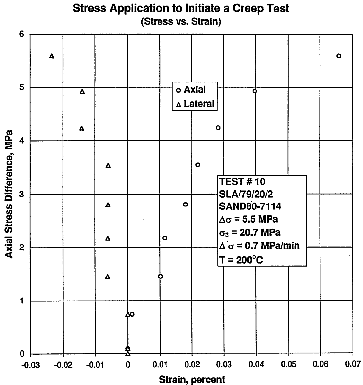
Figure B-58. Axial Stress Difference Versus Axial and Lateral Strain for Stress Application to Initiate a Creep Test: Specimen SLA/79/20/2; Stage 1 of 1.
