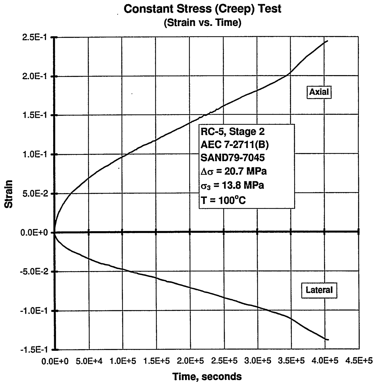
Figure B-190. Axial Strain and Lateral Strain Versus Time for a Creep Test: Specimen AEC7-2711 (B); Stage 2 of 2.
