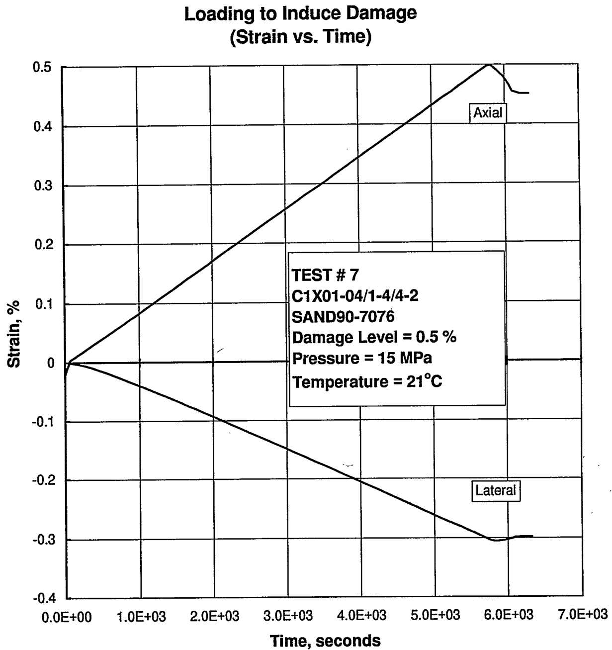
Figure E-108. Axial and Lateral Strain as a Function of Time During the Quasi-Static Loading to Induce Damage in Specimen C1X01-04/1-4/4-2.
