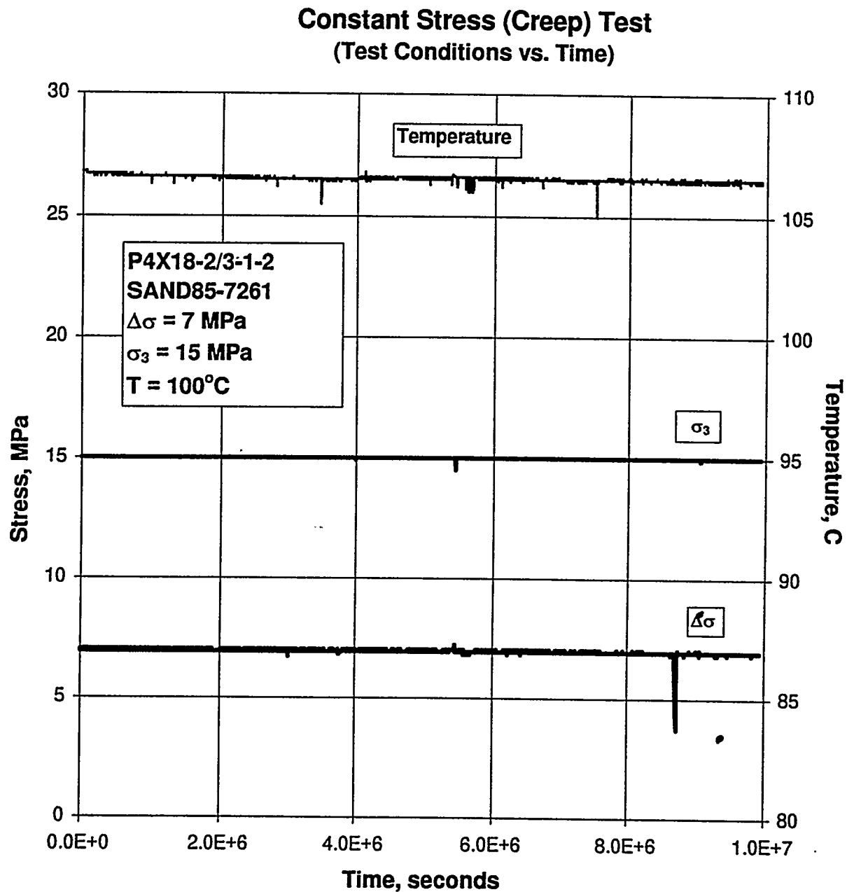
Figure C-49. Test Conditions Versus Time for a Creep Test: Specimen P4X18-2/3-1-2; Stage 1 of 1 (Argillaceous Salt).
