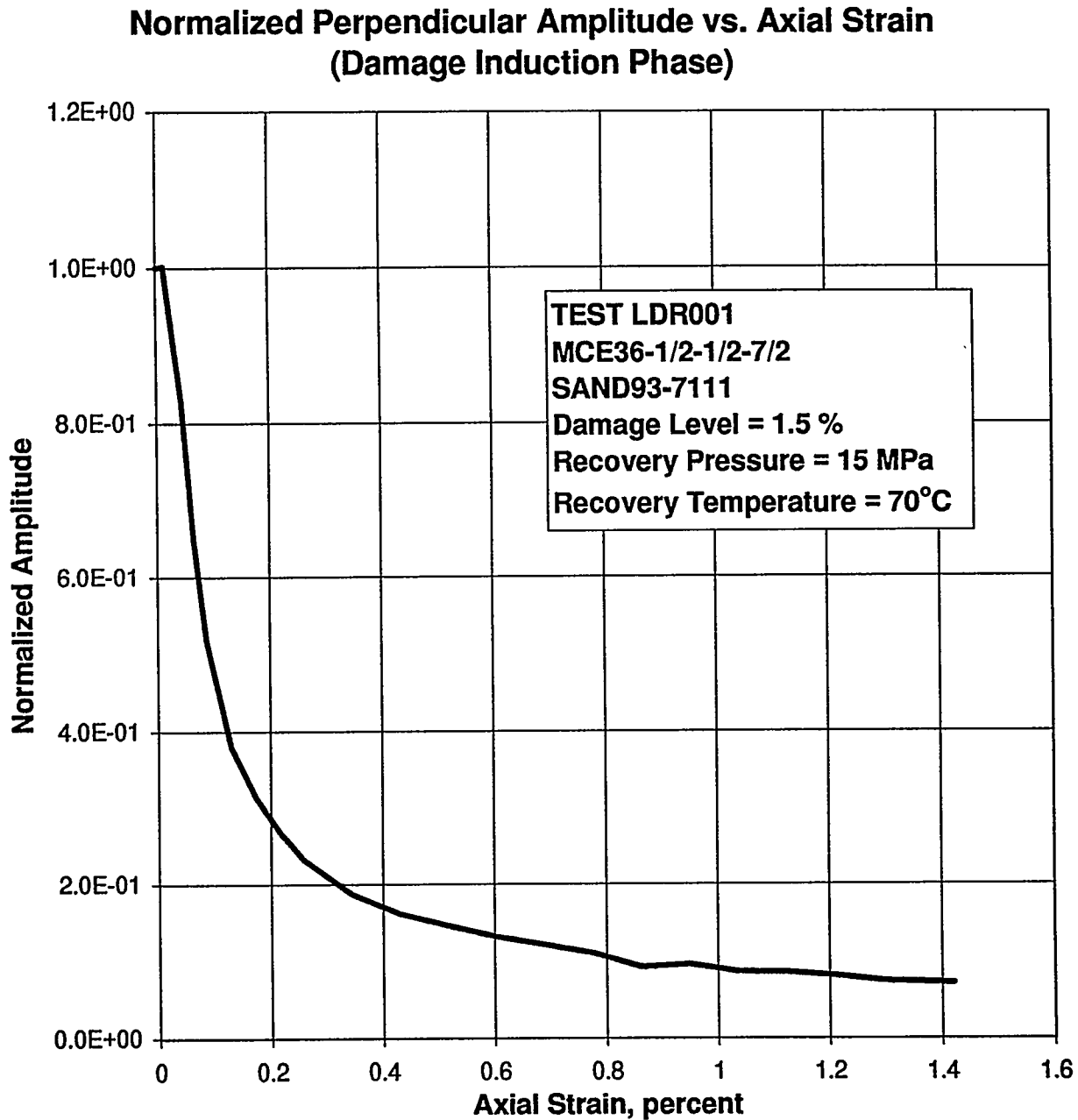
Figure E-3. Normalized Perpendicular Amplitude as a Function of Axial Strain During the Quasi-Static Loading to Induce Damage in Specimen MCE36-1/2-1/2-7/2.
