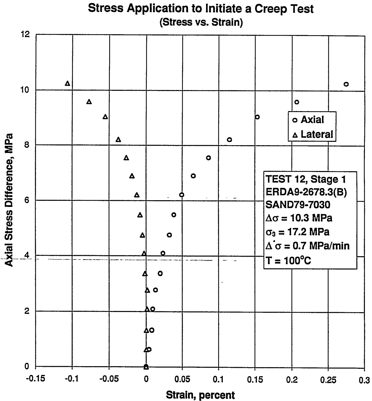
Figure B-128. Axial Stress Difference Versus Axial and Lateral Strain for Stress Application to Initiate a Creep Test: Specimen ERDA9-2678.3 (B); Stage 1 of 2.
