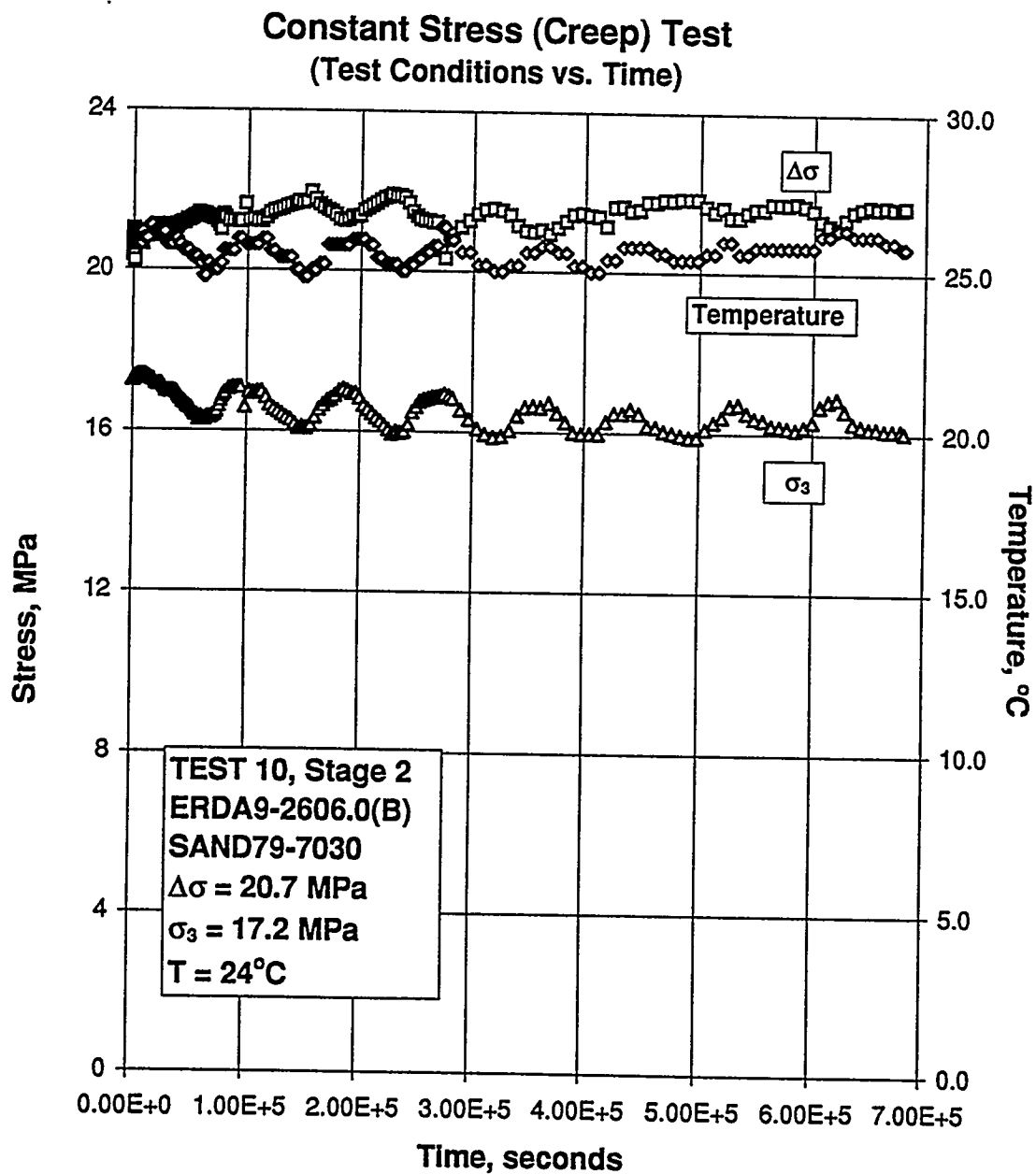
Figure B-119. Test Conditions Versus Time for a Creep Test: Specimen ERDA9-2606.0 (B); Stage 2 of 2.
