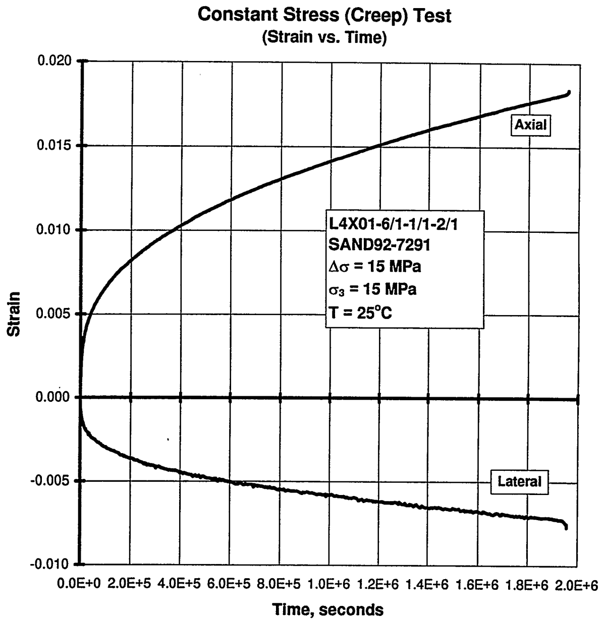
Figure C-22. Axial Strain and Lateral Strain Versus Time for a Creep Test: Specimen L4X01-6/1-1/1-2/1; Stage 1 of 1 (Argillaceous Salt).
