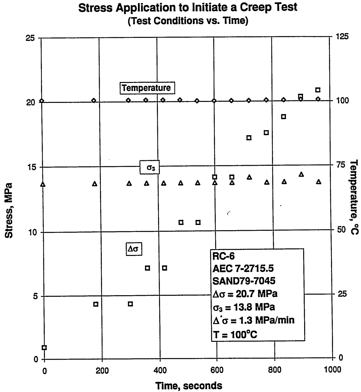
Figure B-191. Test Conditions Versus Time for Stress Application to Initiate a Creep Test: Specimen AEC7-2715.5; Stage 1 of 1.
