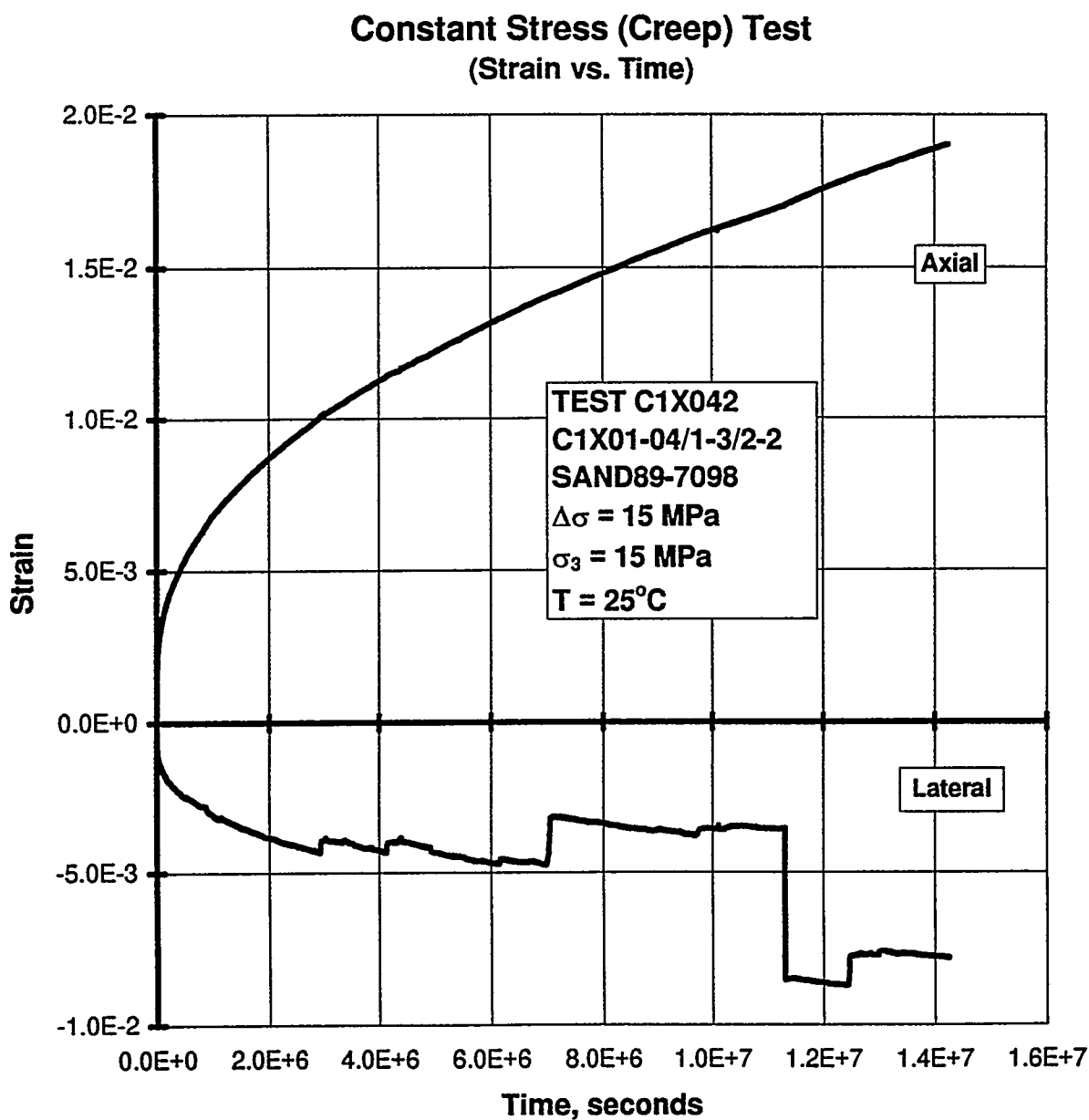
Figure C-34. Axial Strain and Lateral Strain Versus Time for a Creep Test: Specimen C1X01-04/1-3/2-2; Stage 1 of 1.
