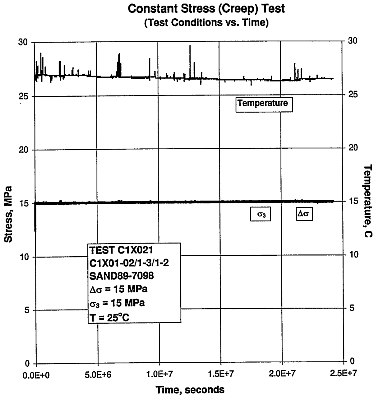
Figure C-35. Test Conditions Versus Time for a Creep Test: Specimen C1X01-02/1-3/1-2; Stage 1 of 1.
