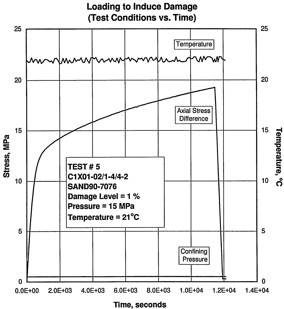
Figure E-83. Test Conditions as a Function of Time During the Quasi-Static Loading to Induce Damage in Specimen C1X01-02/1-4/4-2.
