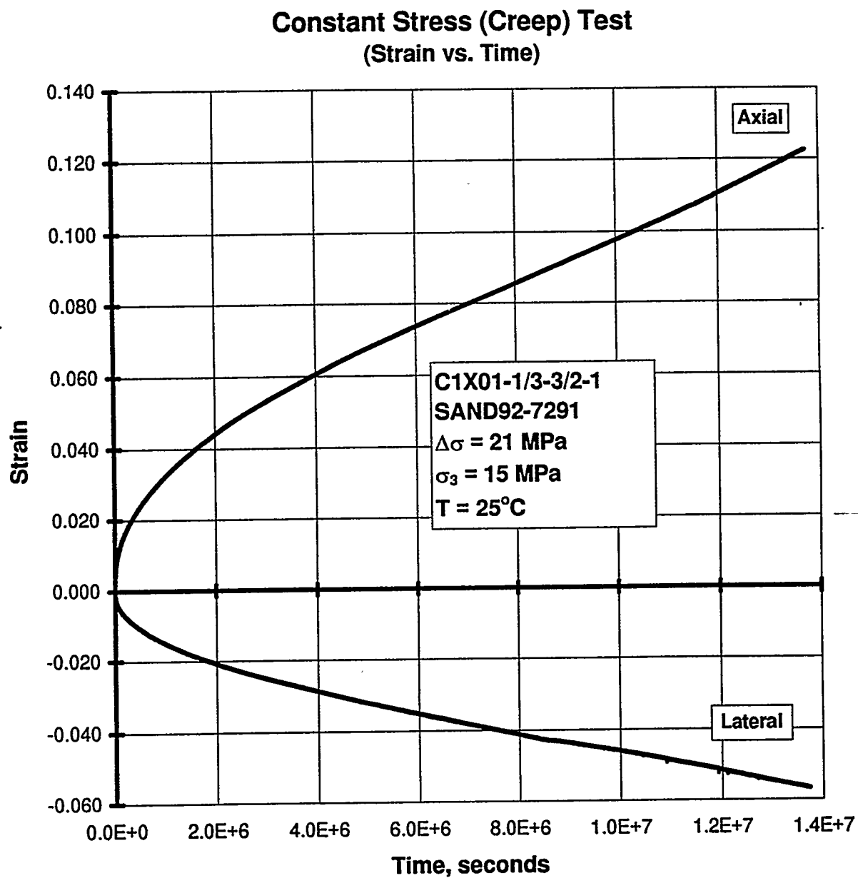
Figure C-8. Axial Strain and Lateral Strain Versus Time for a Creep Test: Specimen C1X01-1/3-3/2-1; Stage 1 of 1.
