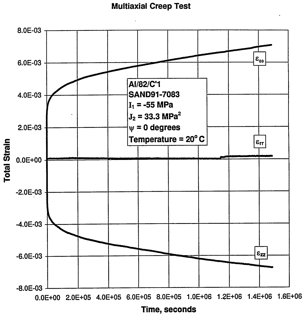
Figure D-2. Principal Strains Versus Time for a Multiaxial Creep Test: Specimen AI/82/C'1.
