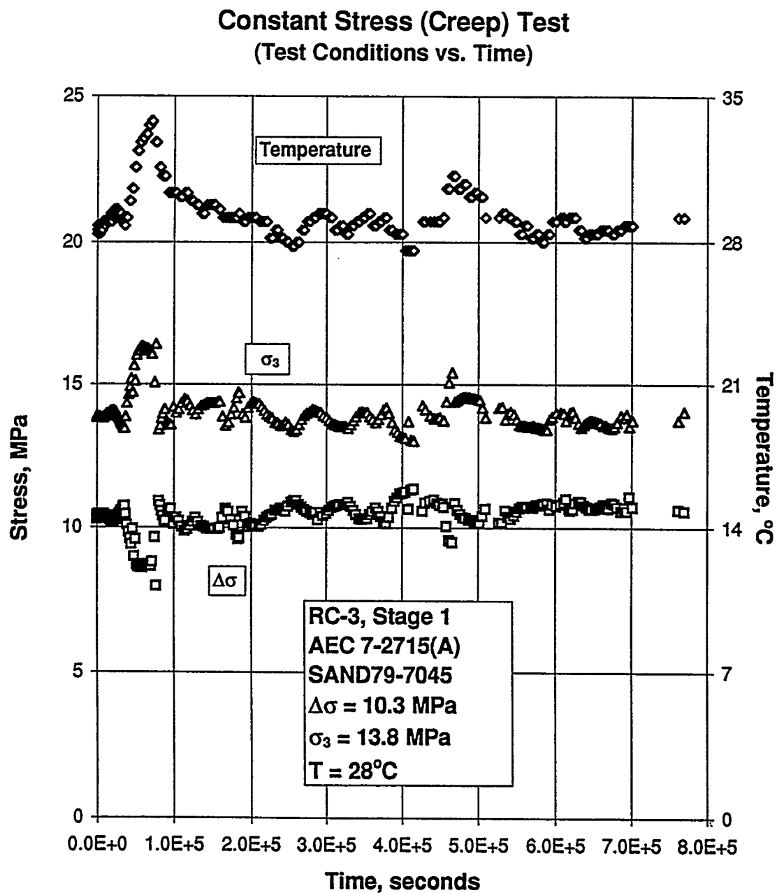
Figure B-165. Test Conditions Versus Time for a Creep Test: Specimen AEC7-2715 (A); Stage 1 of 3.
