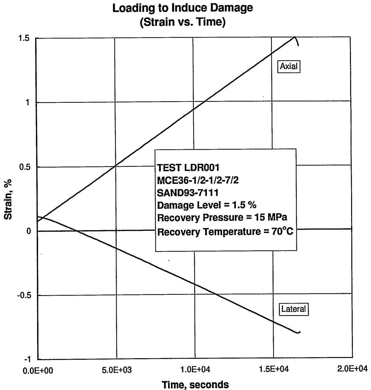
Figure E-2. Axial and Lateral Strain as a Function of Time During the Quasi-Static Loading to Induce Damage in Specimen MCE36-1/2-1/2-7/2.
