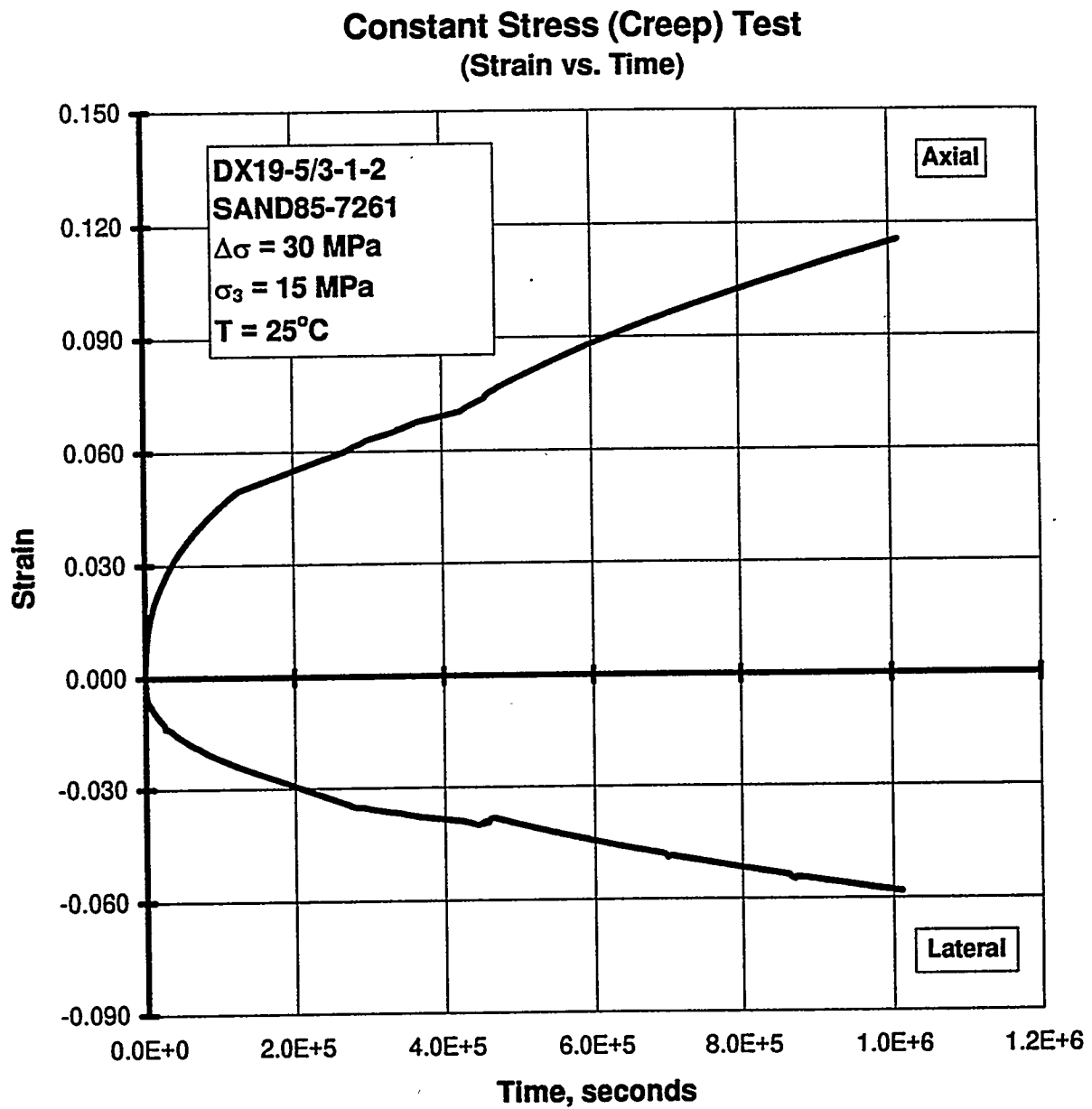
Figure C-76. Axial Strain and Lateral Strain Versus Time for a Creep Test: Specimen DX19-5/3-1-2; Stage 1 of 1.
