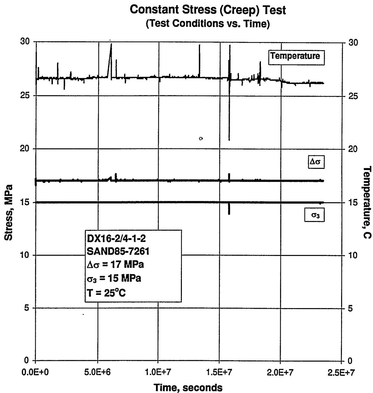
Figure C-63. Test Conditions Versus Time for a Creep Test: Specimen DX16-2/4-1-2; Stage 1 of 1.
