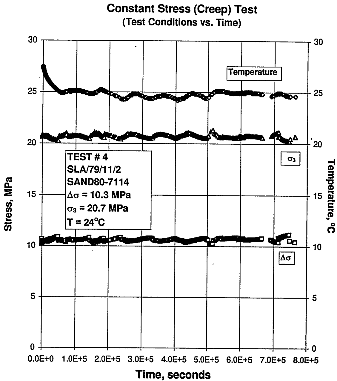
Figure B-28. Test Conditions Versus Time for a Creep Test: Specimen SLA/79/11/2; Stage 1 of 1.
