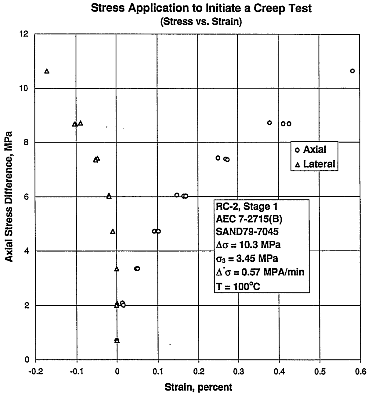
Figure B-156. Axial Stress Difference Versus Axial and Lateral Strain for Stress Application to Initiate a Creep Test: Specimen AEC7-2715 (B); Stage 1 of 2.
