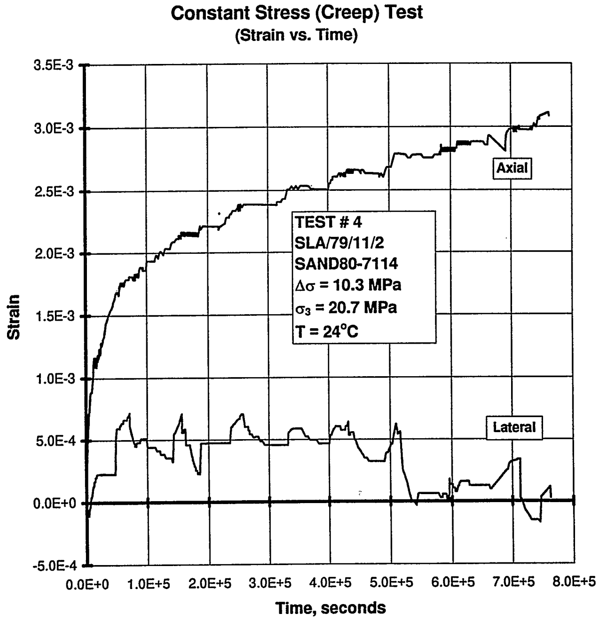
Figure B-29. Axial Strain and Lateral Strain Versus Time for a Creep Test: Specimen SLA/79/11/2; Stage 1 of 1 (Data Acquisition Failure at 9 Days. Data Before 9 Days is Valid. Poor Lateral Data Caused by Dilatometer Leak).
