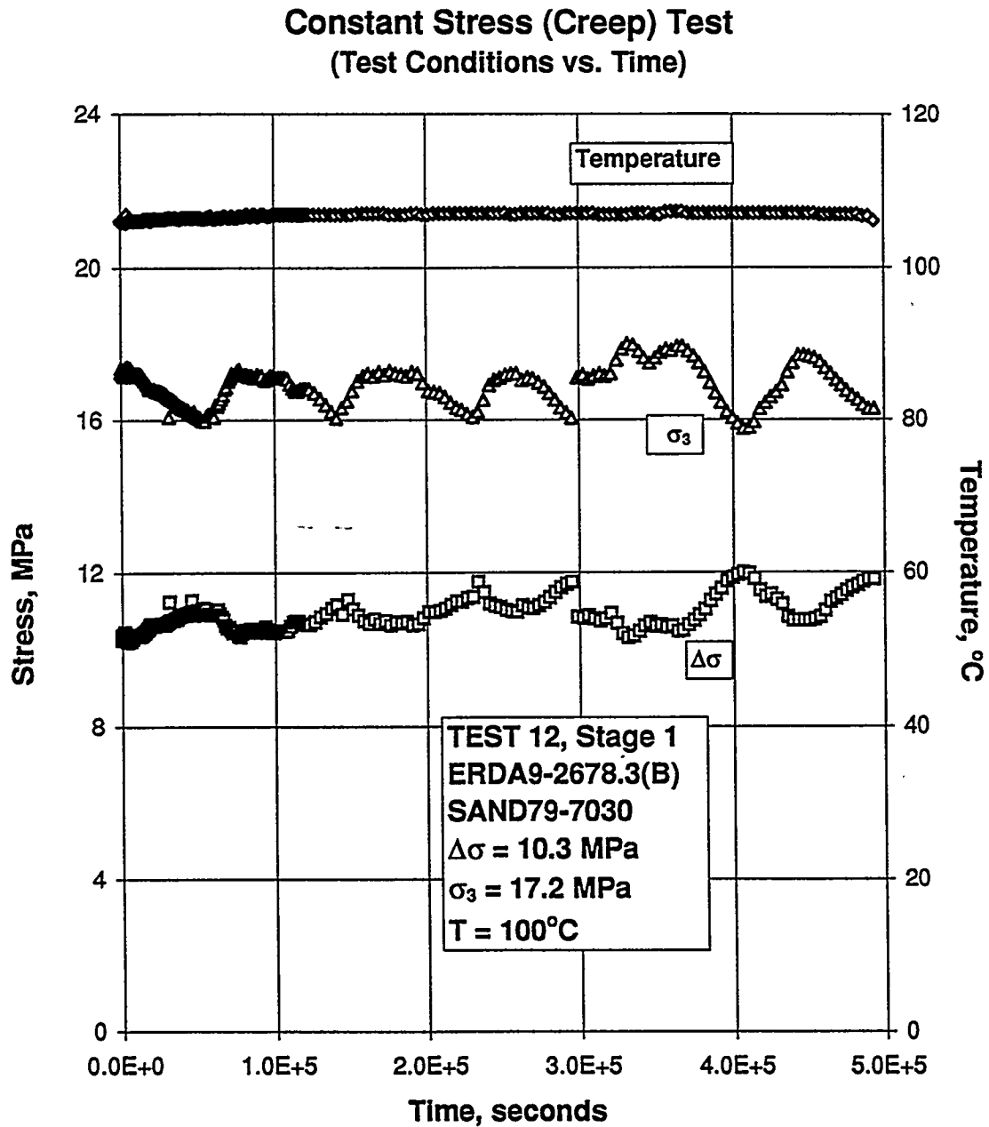
Figure B-129. Test Conditions Versus Time for a Creep Test: Specimen ERDA9-2678.3 (B); Stage 1 of 2.
