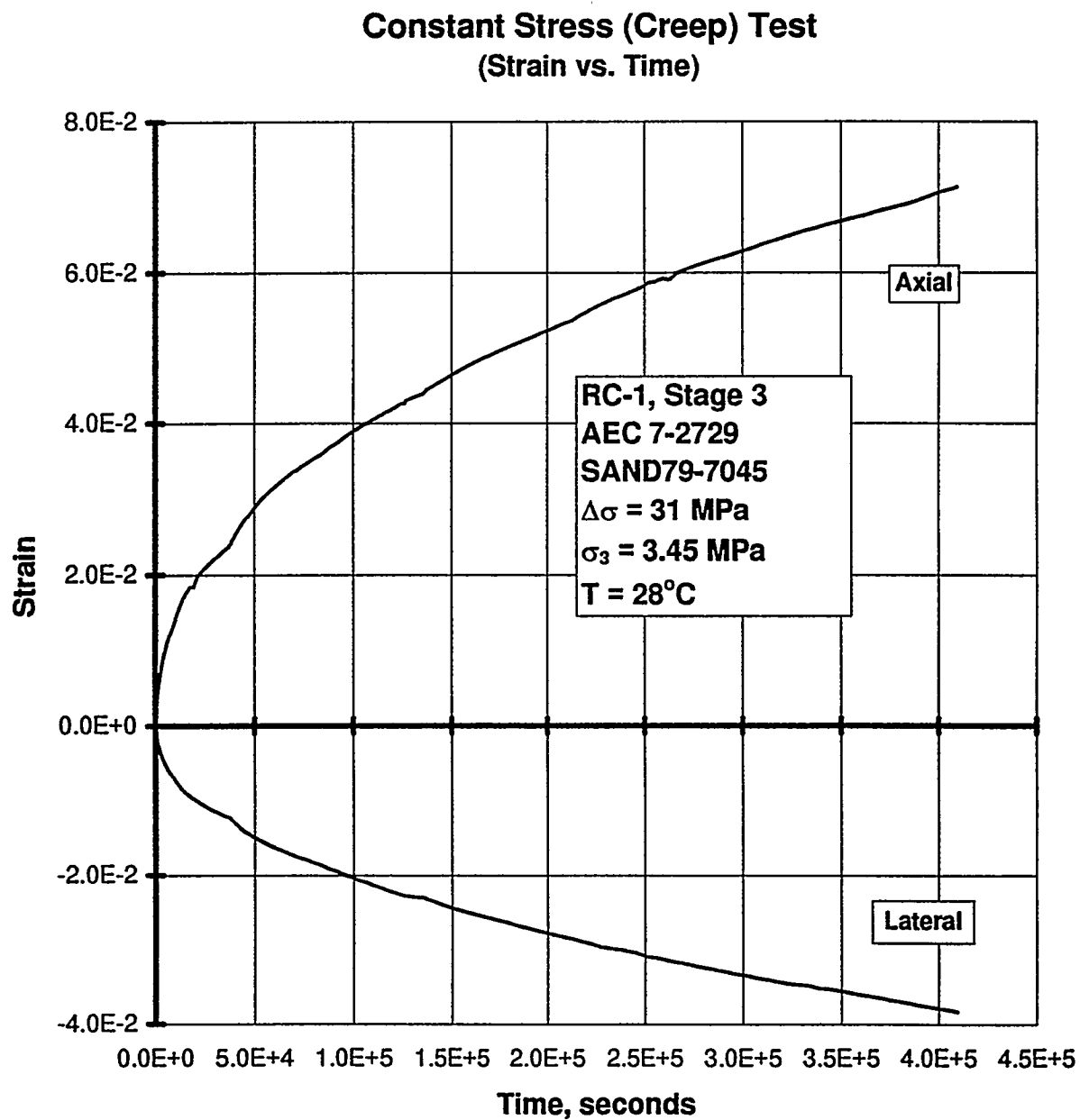
Figure B-154. Axial Strain and Lateral Strain Versus Time for a Creep Test: Specimen AEC7-2729; Stage 3 of 3.
