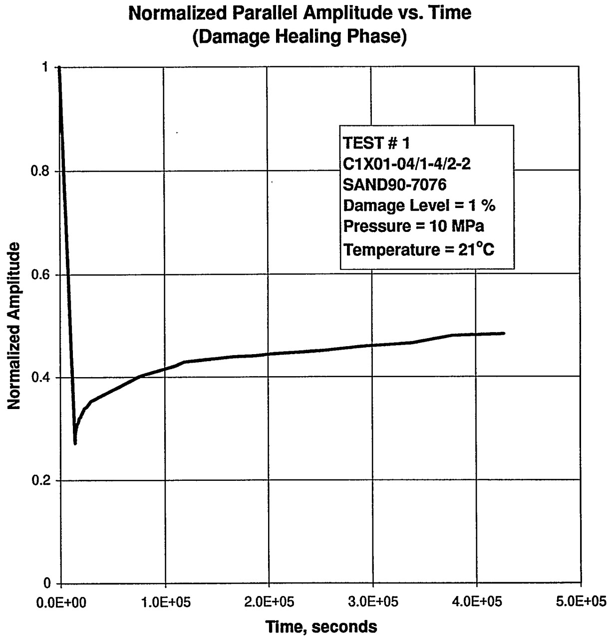
Figure E-44. Normalized Parallel Amplitude as a Function of Time During the Hydrostatic Loading to Recover Damage in Specimen C1X01-04/1-4/2-2.
