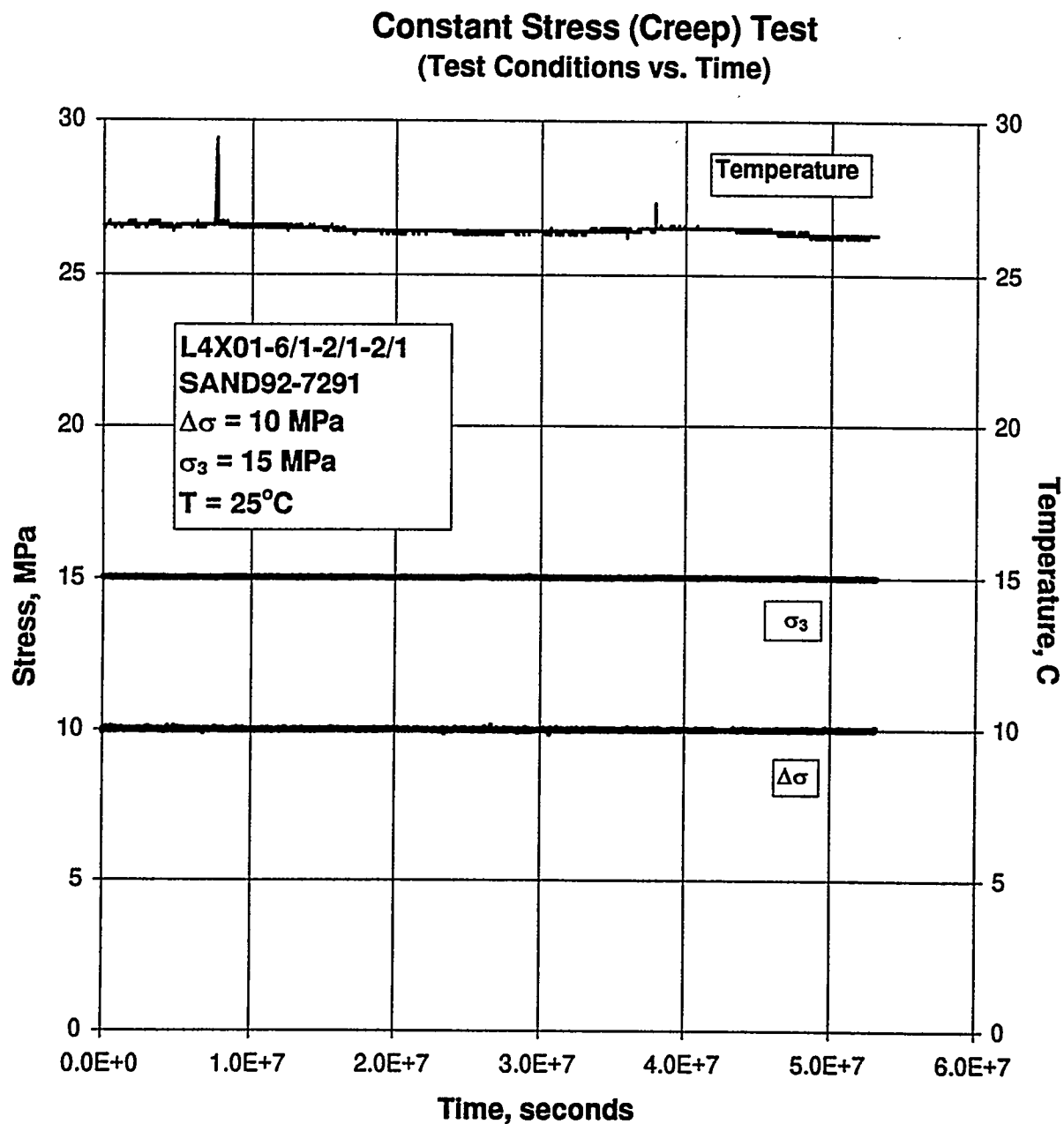
Figure C-15. Test Conditions Versus Time for a Creep Test: Specimen L4X01-6/1-2/1-2/1; Stage 1 of 1 (Argillaceous Salt).
