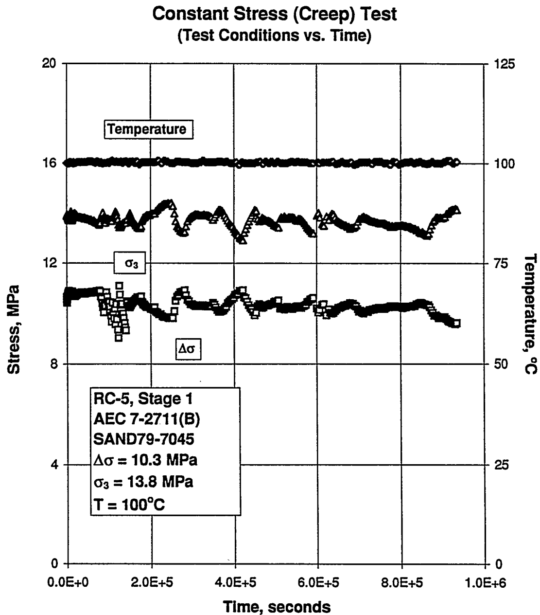
Figure B-185. Test Conditions Versus Time for a Creep Test: Specimen AEC7-2711 (B); Stage 1 of 2.
