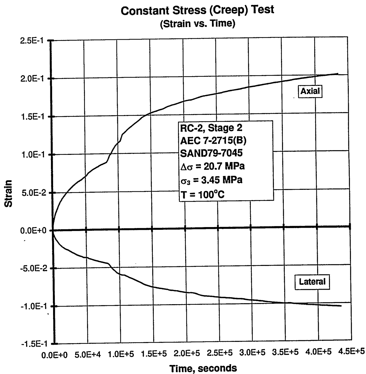
Figure B-162. Axial Strain and Lateral Strain Versus Time for a Creep Test: Specimen AEC7-2715 (B); Stage 2 of 2.
