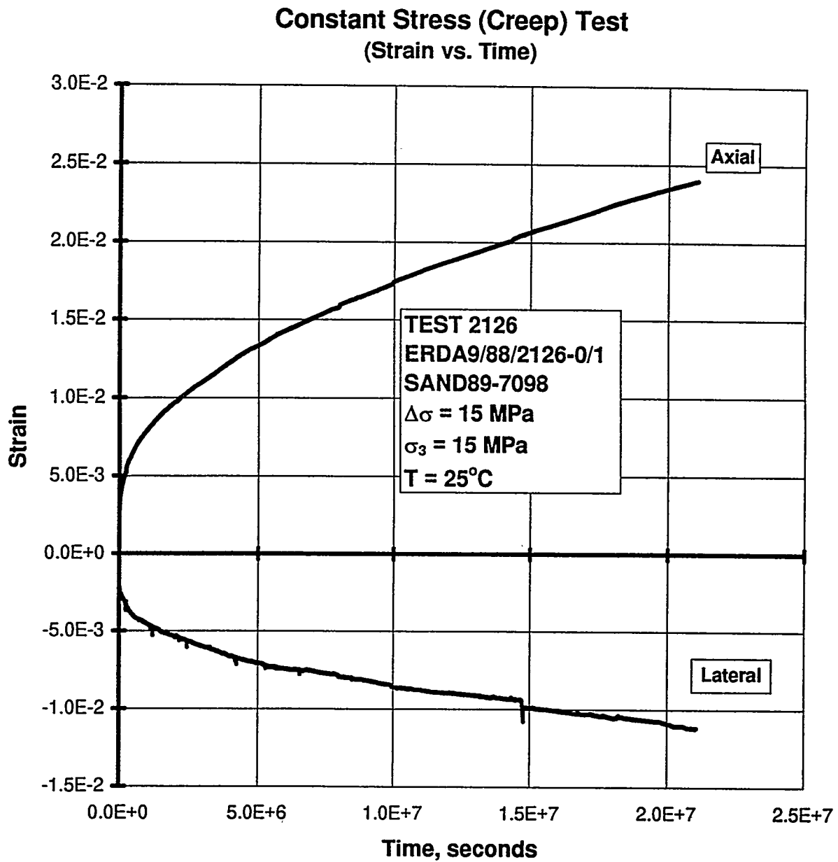
Figure B-6. Axial Strain and Lateral Strain Versus Time for a Creep Test: Specimen ERDA9/88/2126-0/1; Stage 1 of 1.
