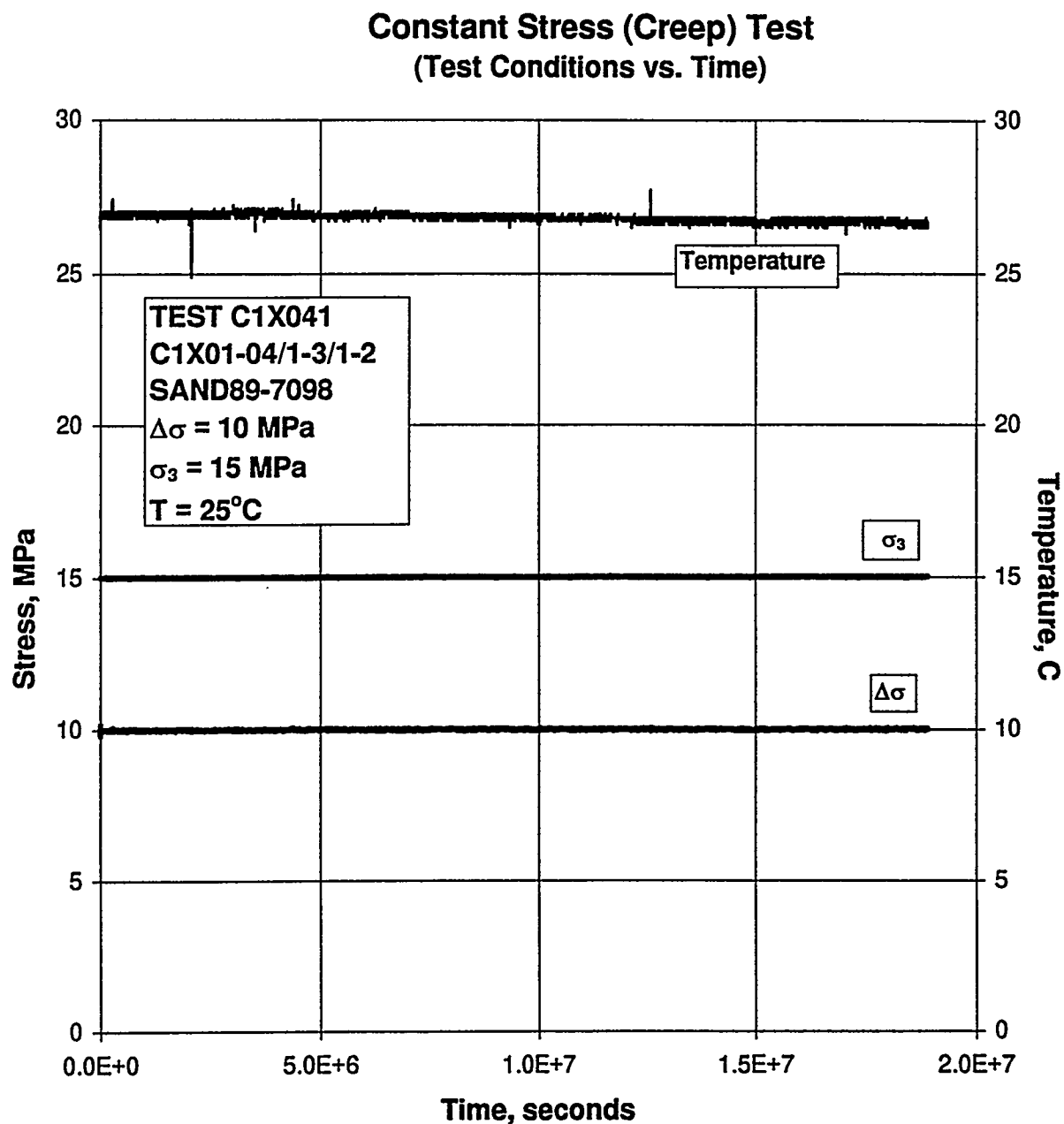
Figure C-31. Test Conditions Versus Time for a Creep Test: Specimen C1X01-04/1-3/1-2; Stage 1 of 1.
