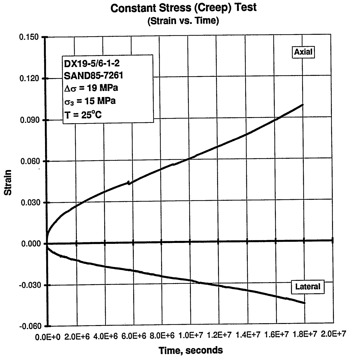
Figure C-68. Axial Strain and Lateral Strain Versus Time for a Creep Test: Specimen DX19-5/6-1-2; Stage 1 of 1.
