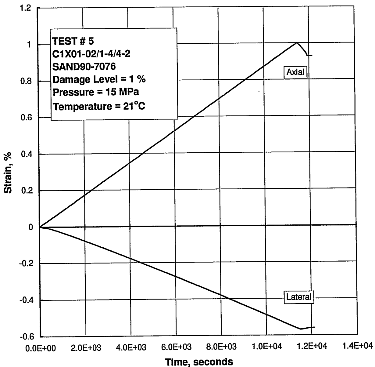
Figure E-84. Axial and Lateral Strain as a Function of Time During the Quasi-Static Loading to Induce Damage in Specimen C1X01-02/1-4/4-2.
