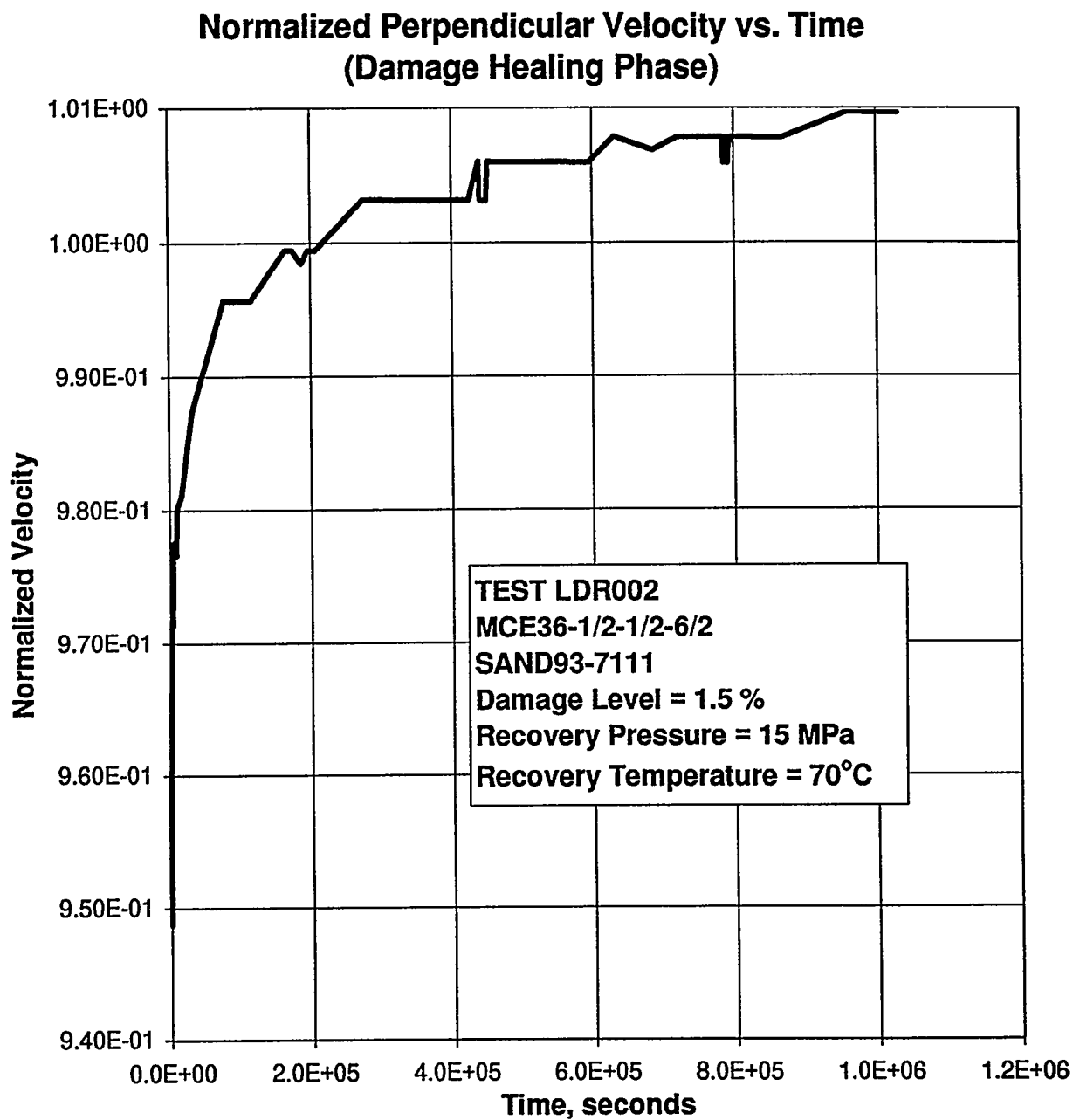
Figure E-15. Normalized Perpendicular Velocity as a Function of Time During the Hydrostatic Loading to Recover Damage in Specimen MCE36-1/2-1/2-6/2.
