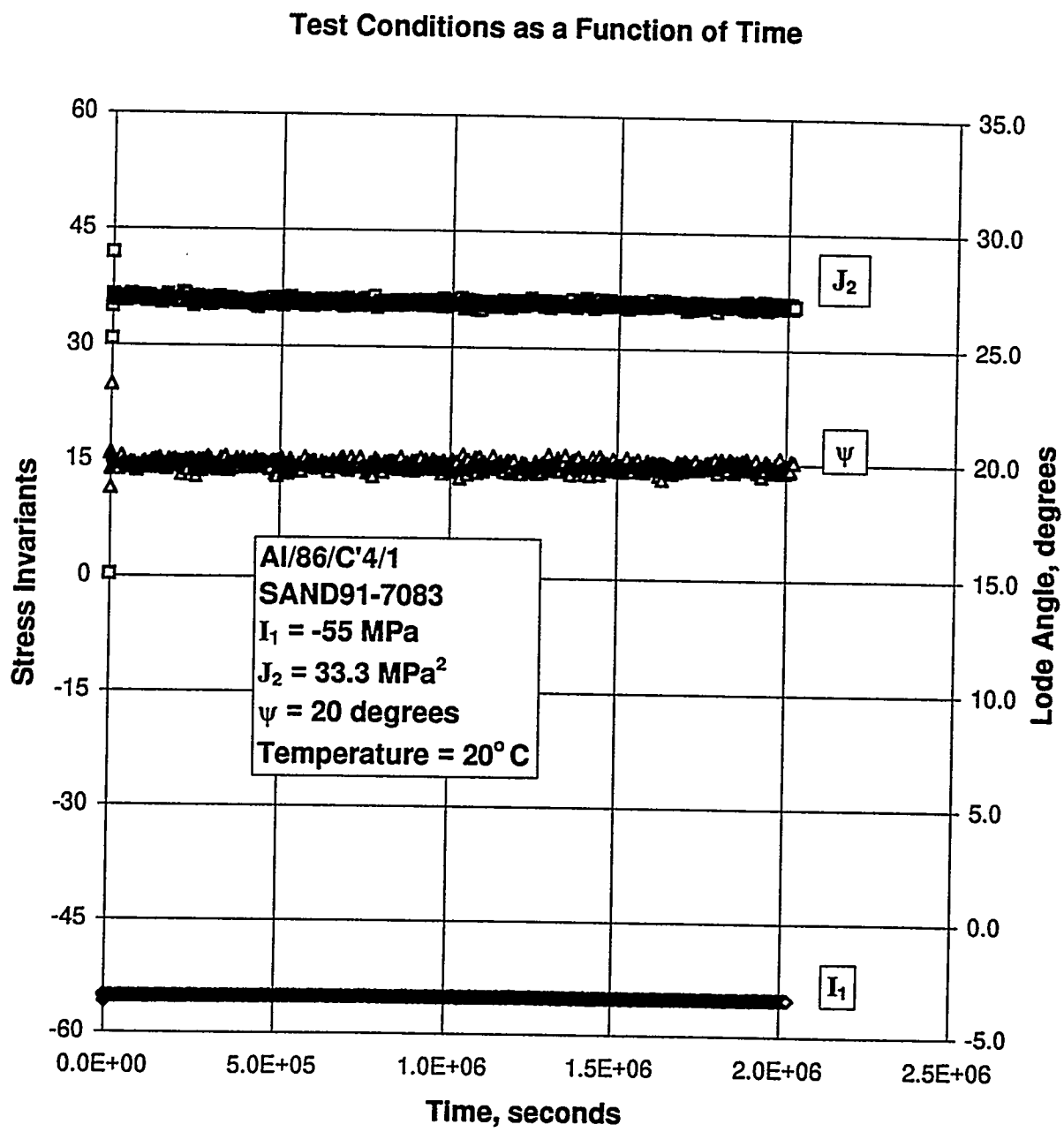
Figure D-7. Test Conditions Versus Time for a Multiaxial Creep Test: Specimen AI/86/C'4/1.
