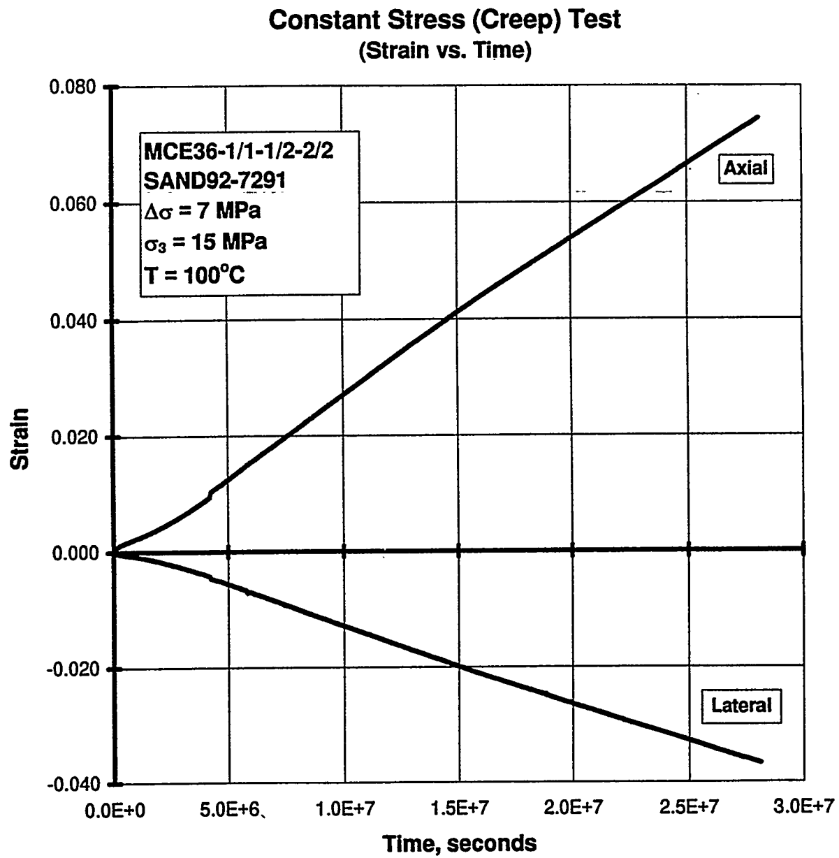
Figure C-14. Axial Strain and Lateral Strain Versus Time for a Creep Test: Specimen MCE36-1/1-1/2-2/2; Stage 1 of 1.
