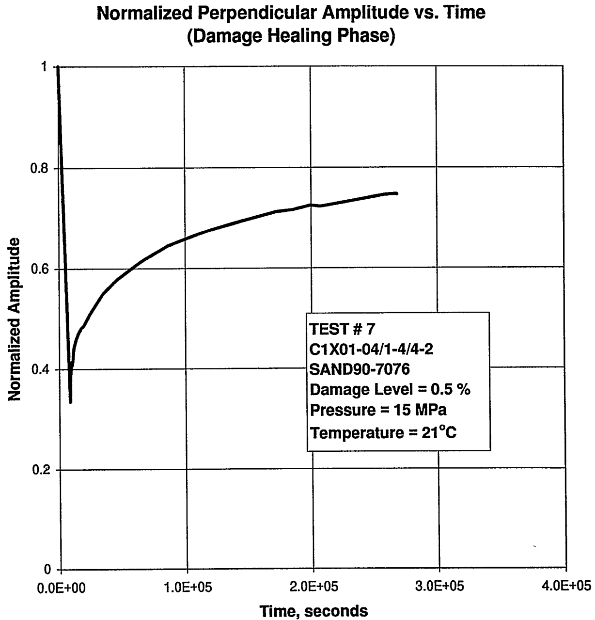
Figure E-115. Normalized Perpendicular Amplitude as a Function of Time During the Hydrostatic Loading to Recover Damage in Specimen C1X01-04/1-4/4-2.
