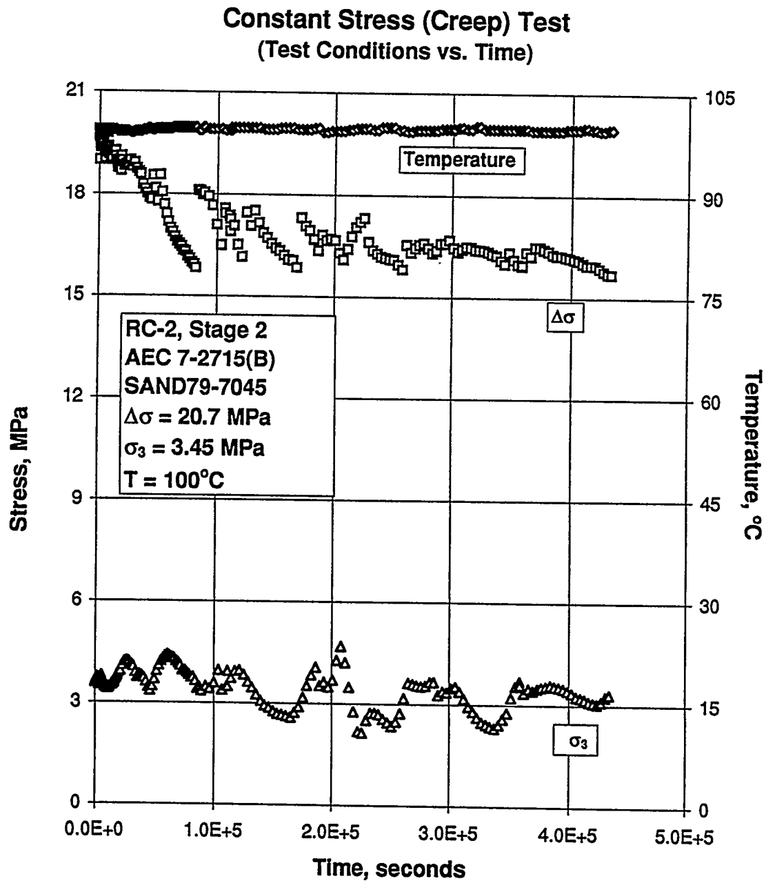
Figure B-161. Test Conditions Versus Time for a Creep Test: Specimen AEC7-2715 (B); Stage 2 of 2.
