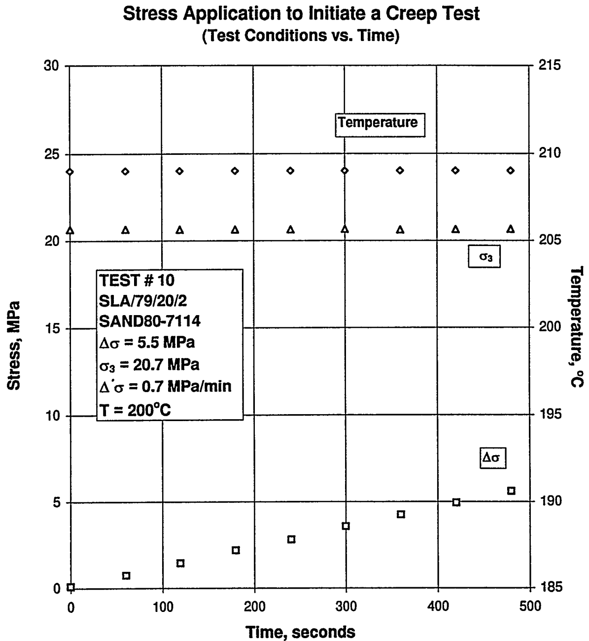
Figure B-57. Test Conditions Versus Time for Stress Application to Initiate a Creep Test: Specimen SLA/79/20/2; Stage 1 of 1.
