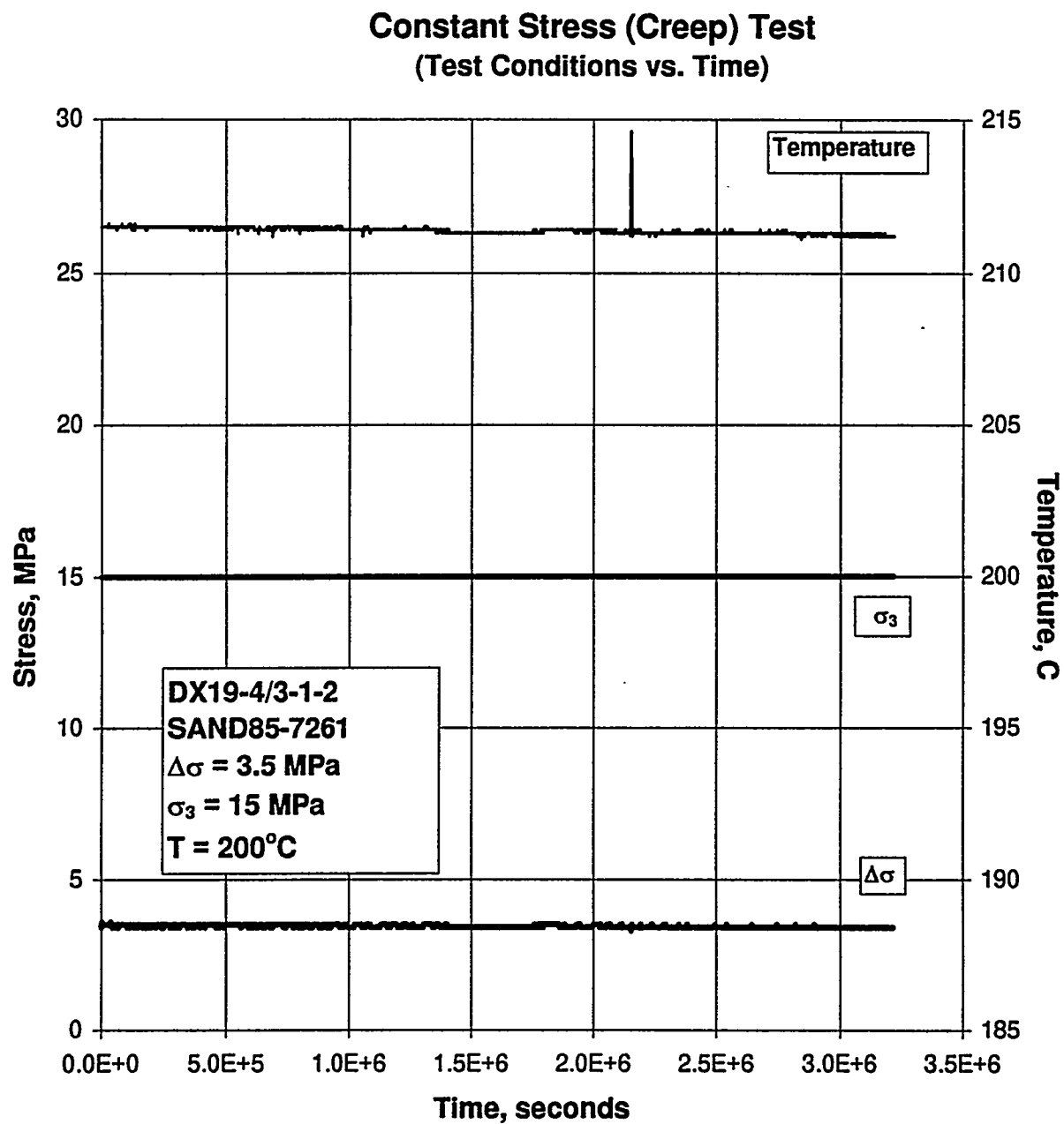
Figure C-87. Test Conditions Versus Time for a Creep Test: Specimen DX19-4/3-1-2; Stage 1 of 1.
