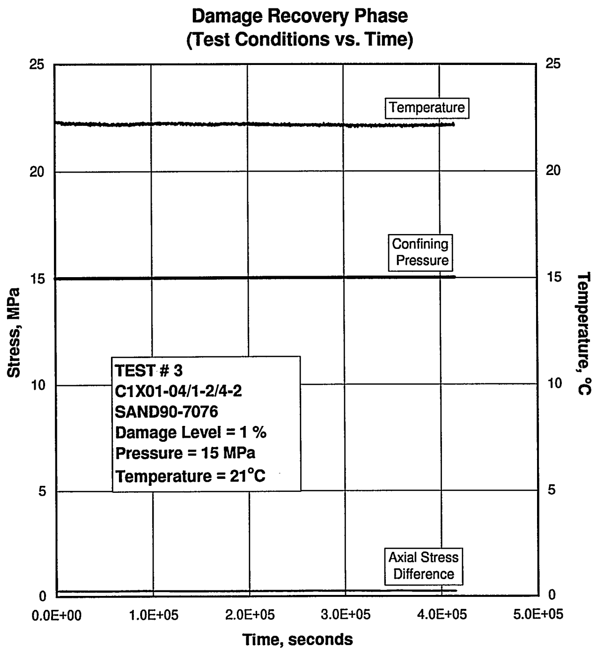
Figure E-65. Test Conditions as a Function of Time During the Hydrostatic Loading to Recover Damage in Specimen C1X01-04/1-2/4-2.
