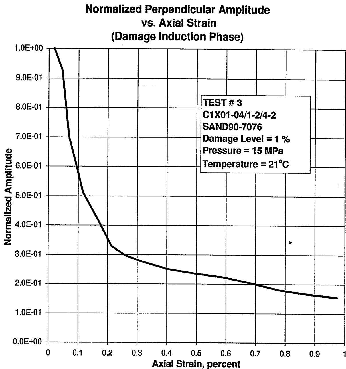
Figure E-61. Normalized Perpendicular Amplitude as a Function of Axial Strain During the Quasi-Static Loading to Induce Damage in Specimen C1X01-04/1-2/4-2.
