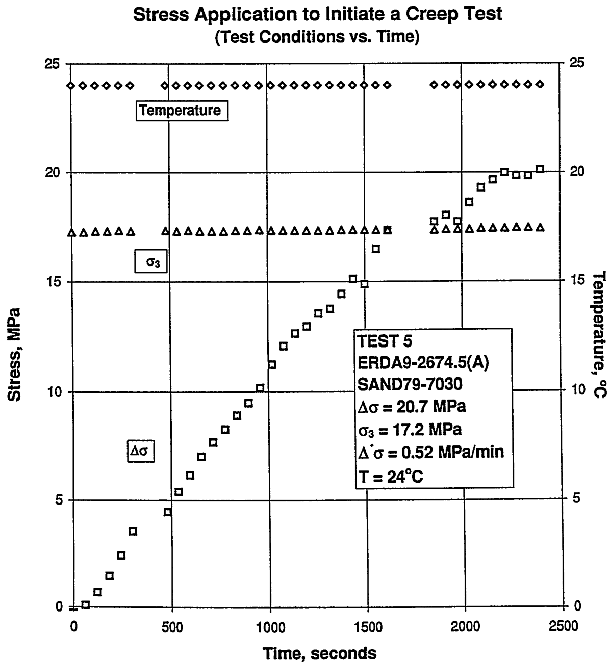
Figure B-89. Test Conditions Versus Time for Stress Application to Initiate a Creep Test: Specimen ERDA9-2674.5 (A); Stage 1 of 1.
