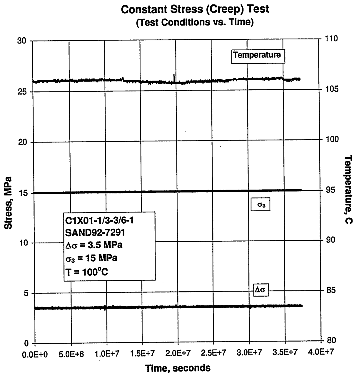
Figure C-10. Axial Strain and Lateral Strain Versus Time for a Creep Test: Specimen C1X01-1/3-3/6-1; Stage 1 of 1.
