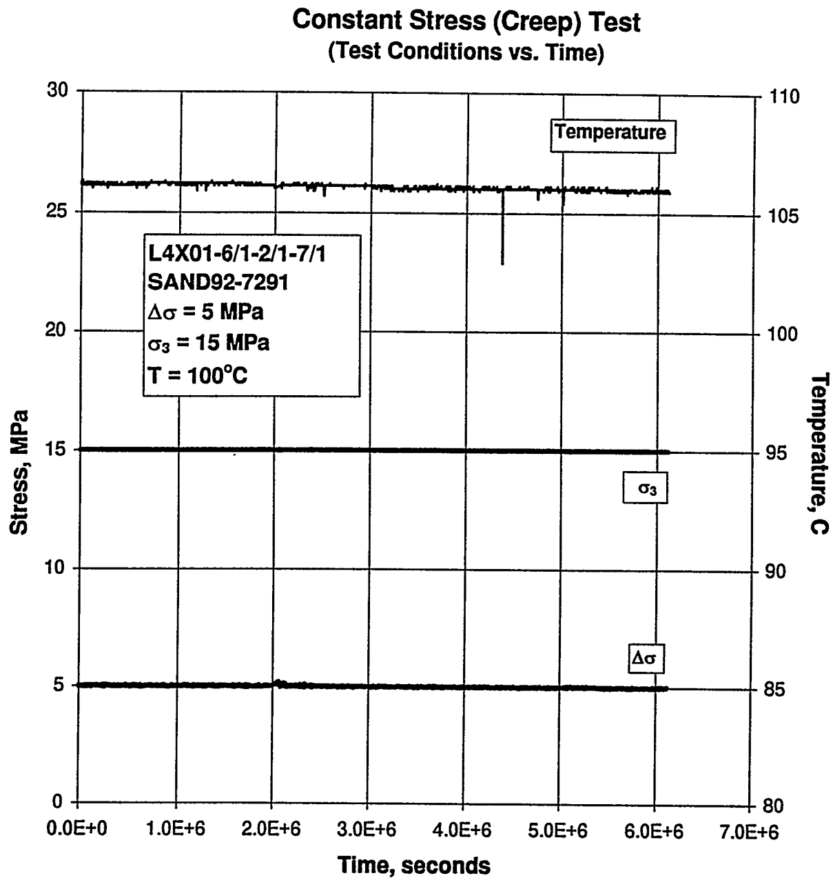
Figure C-27. Test Conditions Versus Time for a Creep Test: Specimen L4X01-6/1-2/1-7/1; Stage 1 of 1 (Argillaceous Salt).
