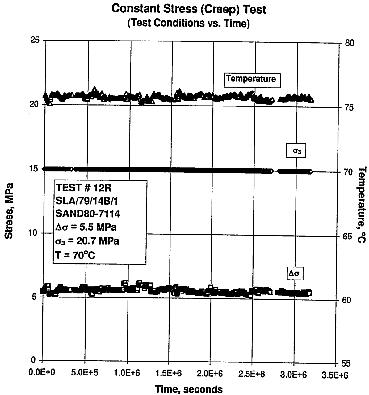
Figure B-71. Test Conditions Versus Time for a Creep Test: Specimen SLA/79/14B/1; Stage 1 of 1.
