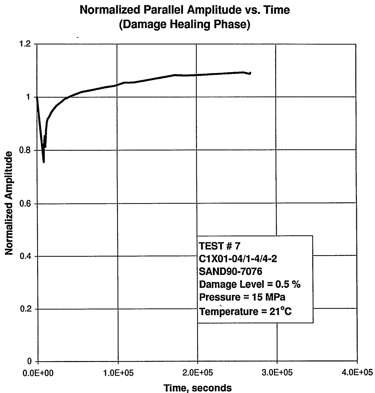
Figure E-116. Normalized Parallel Amplitude as a Function of Time During the Hydrostatic Loading to Recover Damage in Specimen C1X01-04/1-4/4-2.
