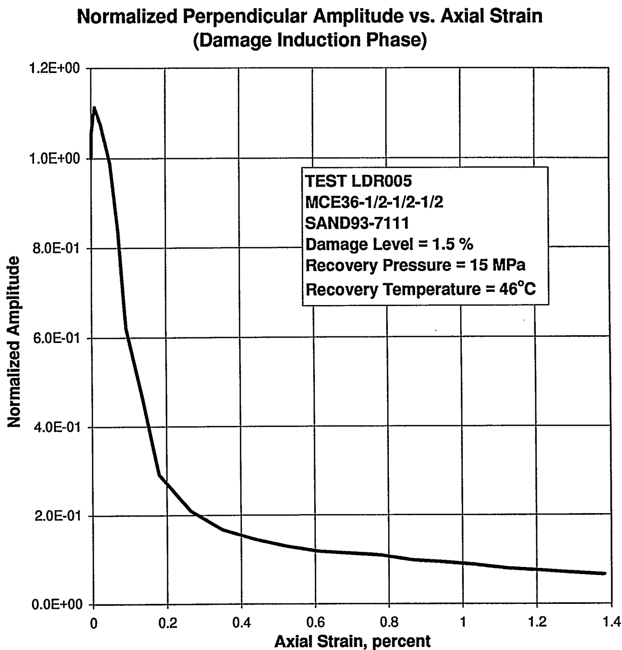
Figure E-19. Normalized Perpendicular Amplitude as a Function of Axial Strain During the Quasi-Static Loading to Induce Damage in Specimen MCE36-1/2-1/2-1/2.
