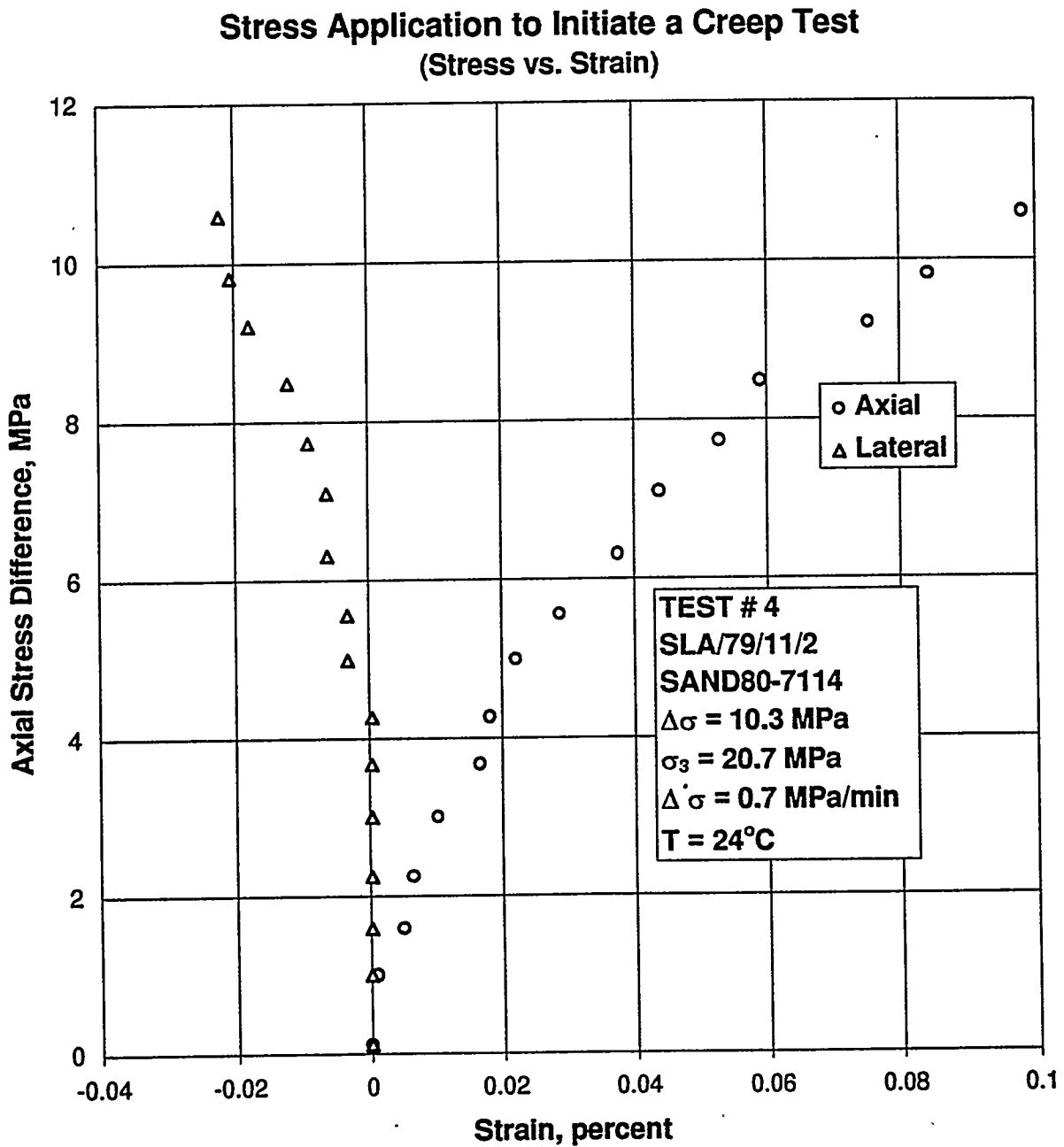
Figure B-27. Axial Stress Difference Versus Axial and Lateral Strain for Stress Application to Initiate a Creep Test: Specimen SLA/79/11/2; Stage 1 of 1.
