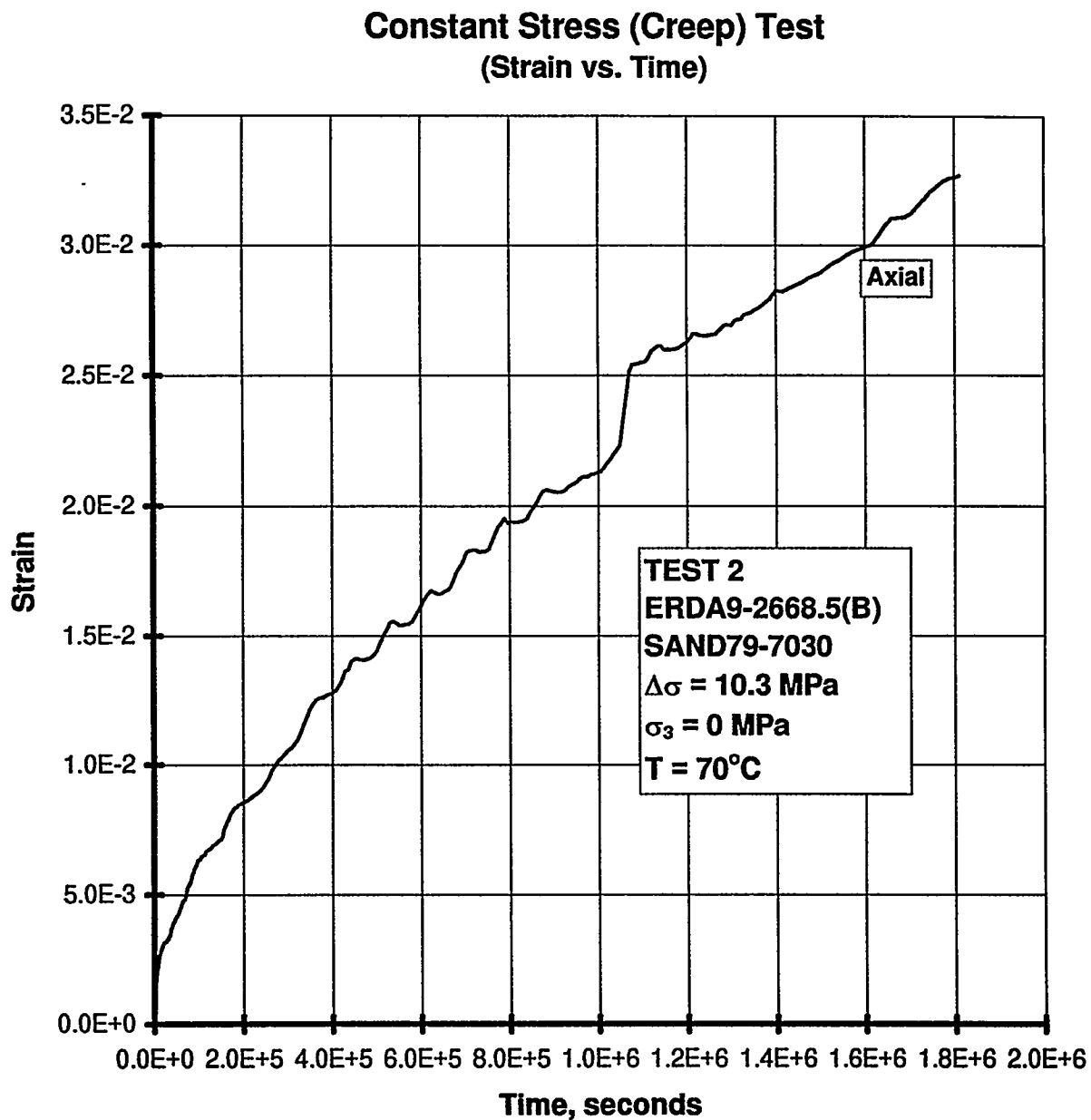
Figure B-80. Axial Strain and Lateral Strain Versus Time for a Creep Test: Specimen ERDA9-2668.5 (B); Stage 1 of 1.
