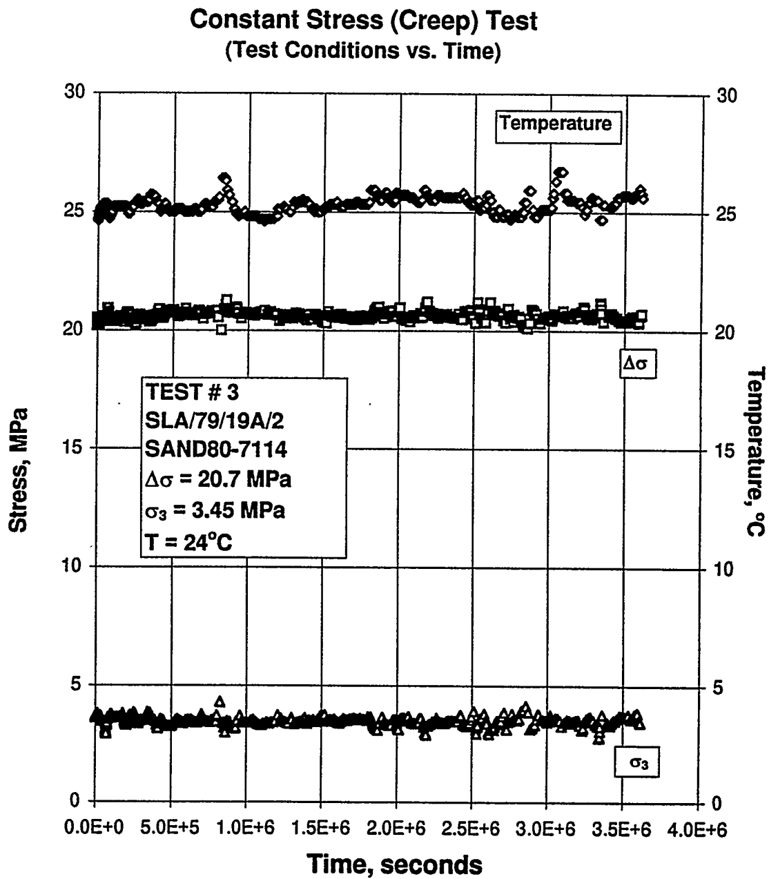
Figure B-24. Test Conditions Versus Time for a Creep Test: Specimen SLA/79/19A/2; Stage 1 of 1.
