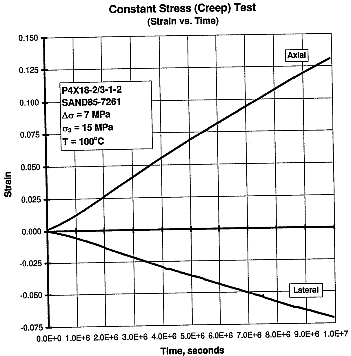
Figure C-50. Axial Strain and Lateral Strain Versus Time for a Creep Test: Specimen P4X18-2/3-1-2; Stage 1 of 1 (Argillaceous Salt. Anomalous Test Result. Possible Moisture Effects).
