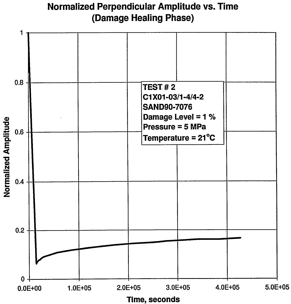
Figure E-55. Normalized Perpendicular Amplitude as a Function of Time During the Hydrostatic Loading to Recover Damage in Specimen C1X01-03/1-4/4-2.
