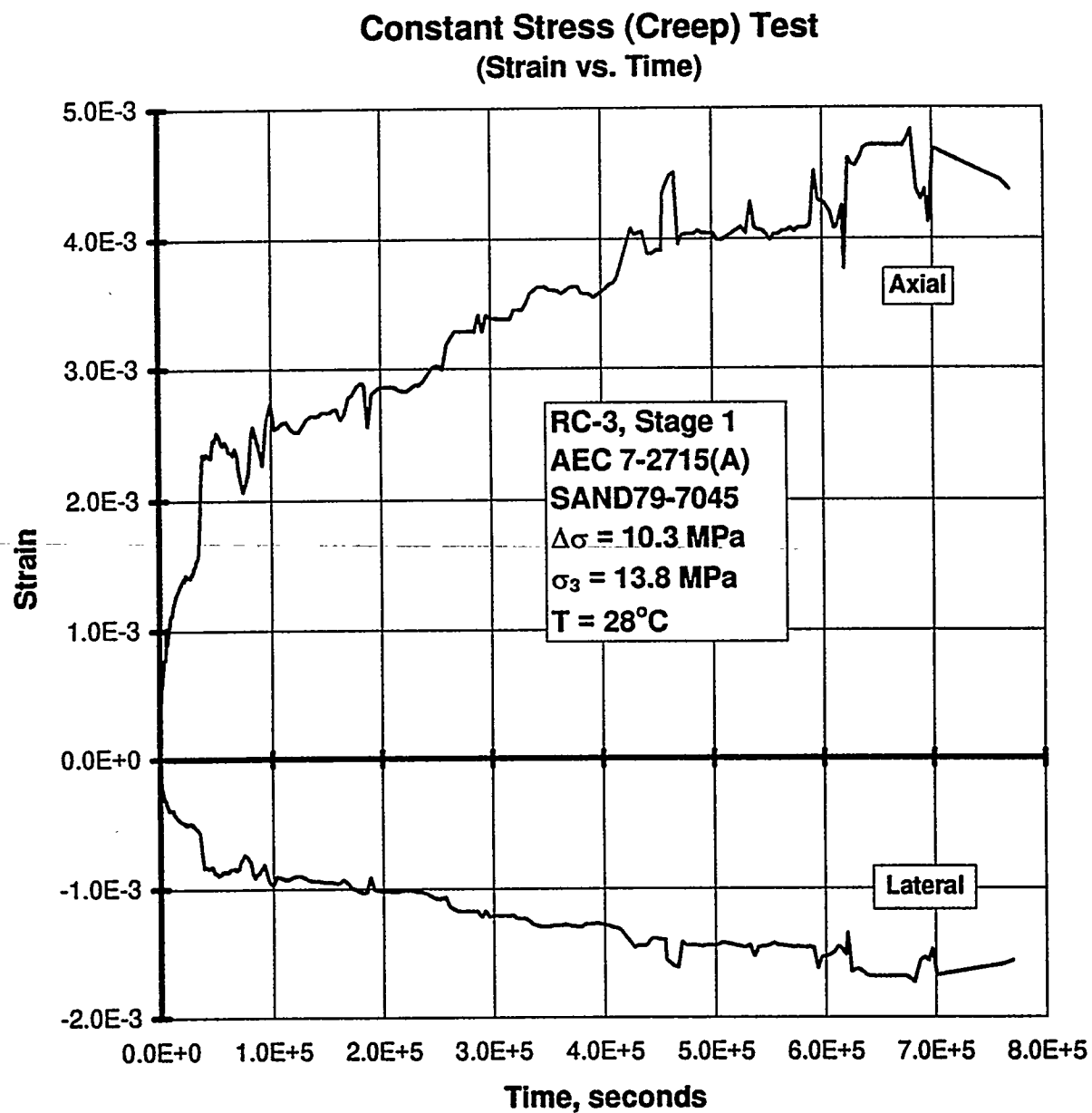
Figure B-166. Axial Strain and Lateral Strain Versus Time for a Creep Test: Specimen AEC7-2715 (A); Stage 1 of 3.
