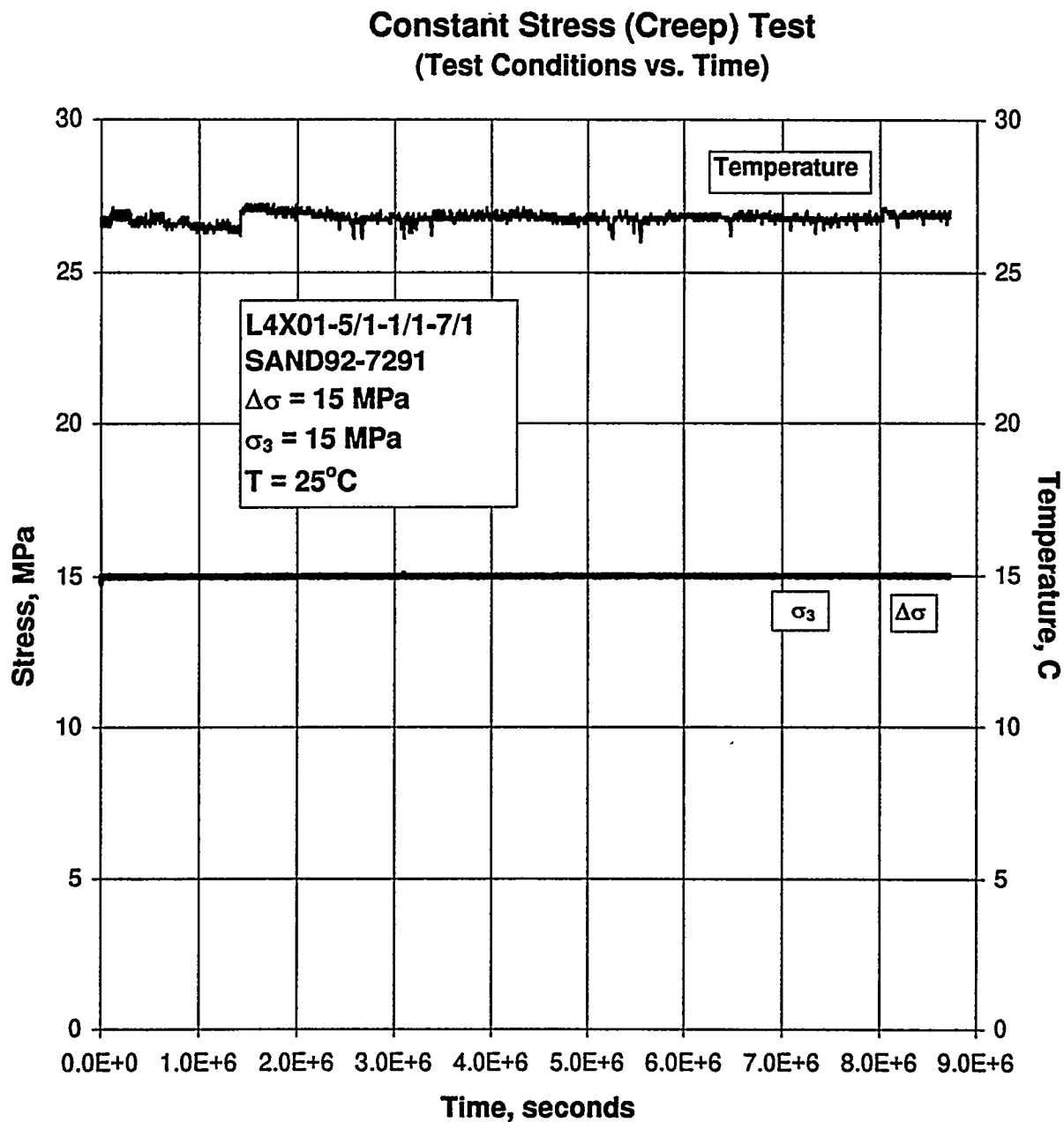
Figure C-23. Test Conditions Versus Time for a Creep Test: Specimen L4X01-5/1-1/1-7/1; Stage 1 of 1 (Argillaceous Salt).
