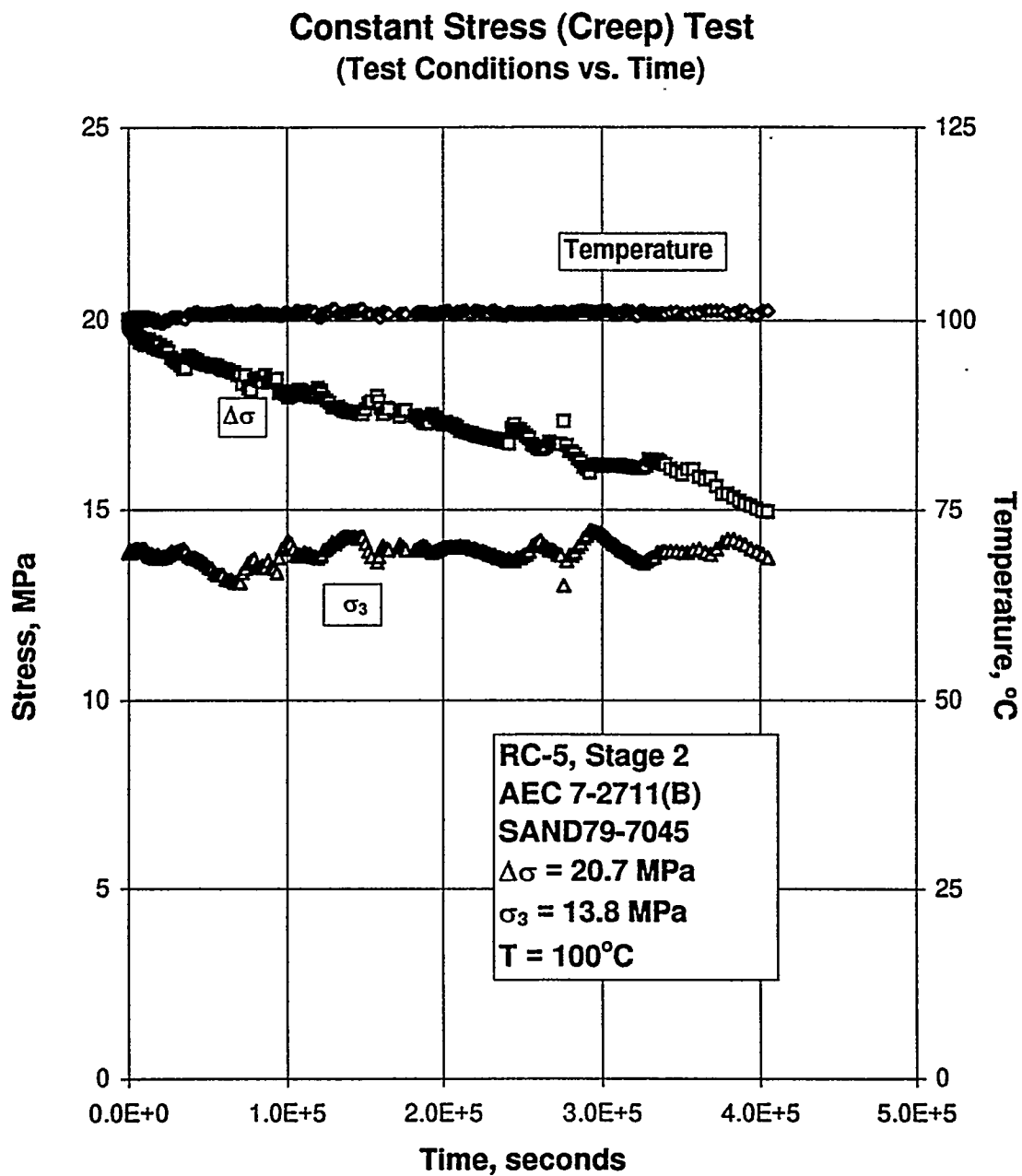
Figure B-189. Test Conditions Versus Time for a Creep Test: Specimen AEC7-2711 (B); Stage 2 of 2.
