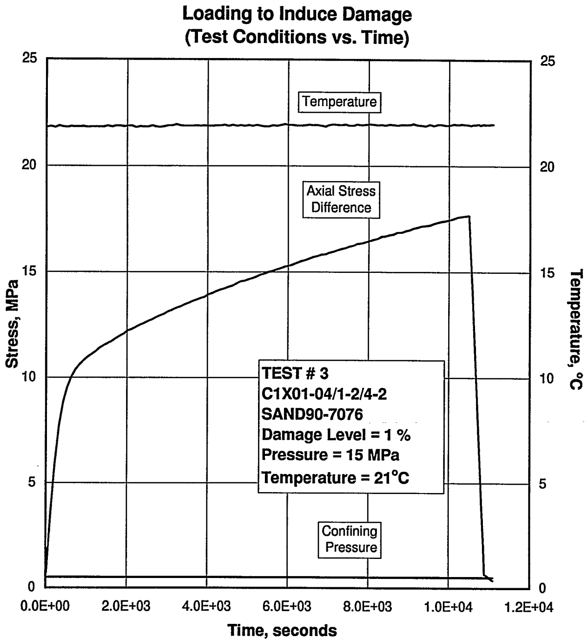
Figure E-59. Test Conditions as a Function of Time During the Quasi-Static Loading to Induce Damage in Specimen C1X01-04/1-2/4-2.
