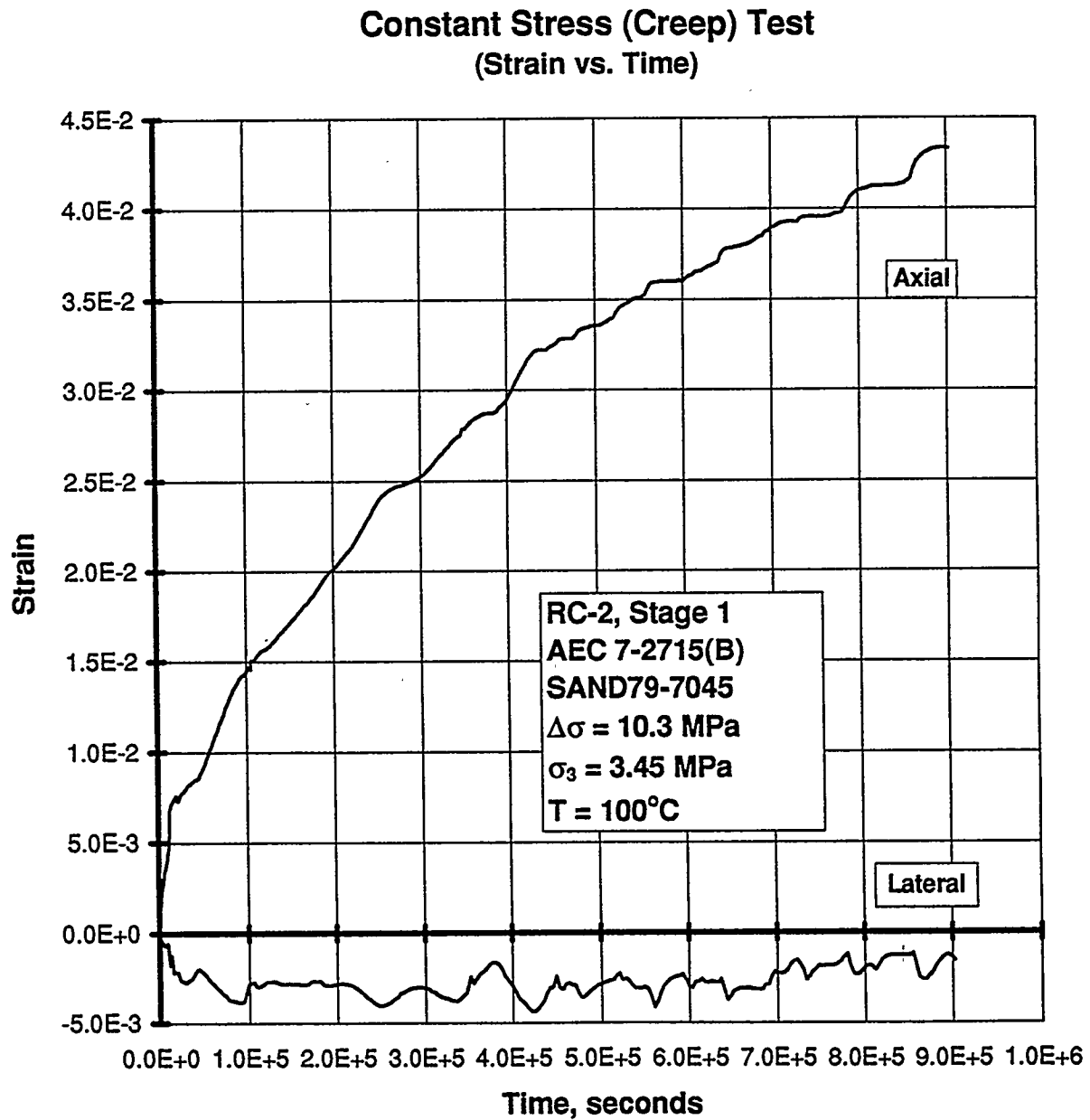
Figure B-158. Axial Strain and Lateral Strain Versus Time for a Creep Test: Specimen AEC7-2715 (B); Stage 1 of 2.
