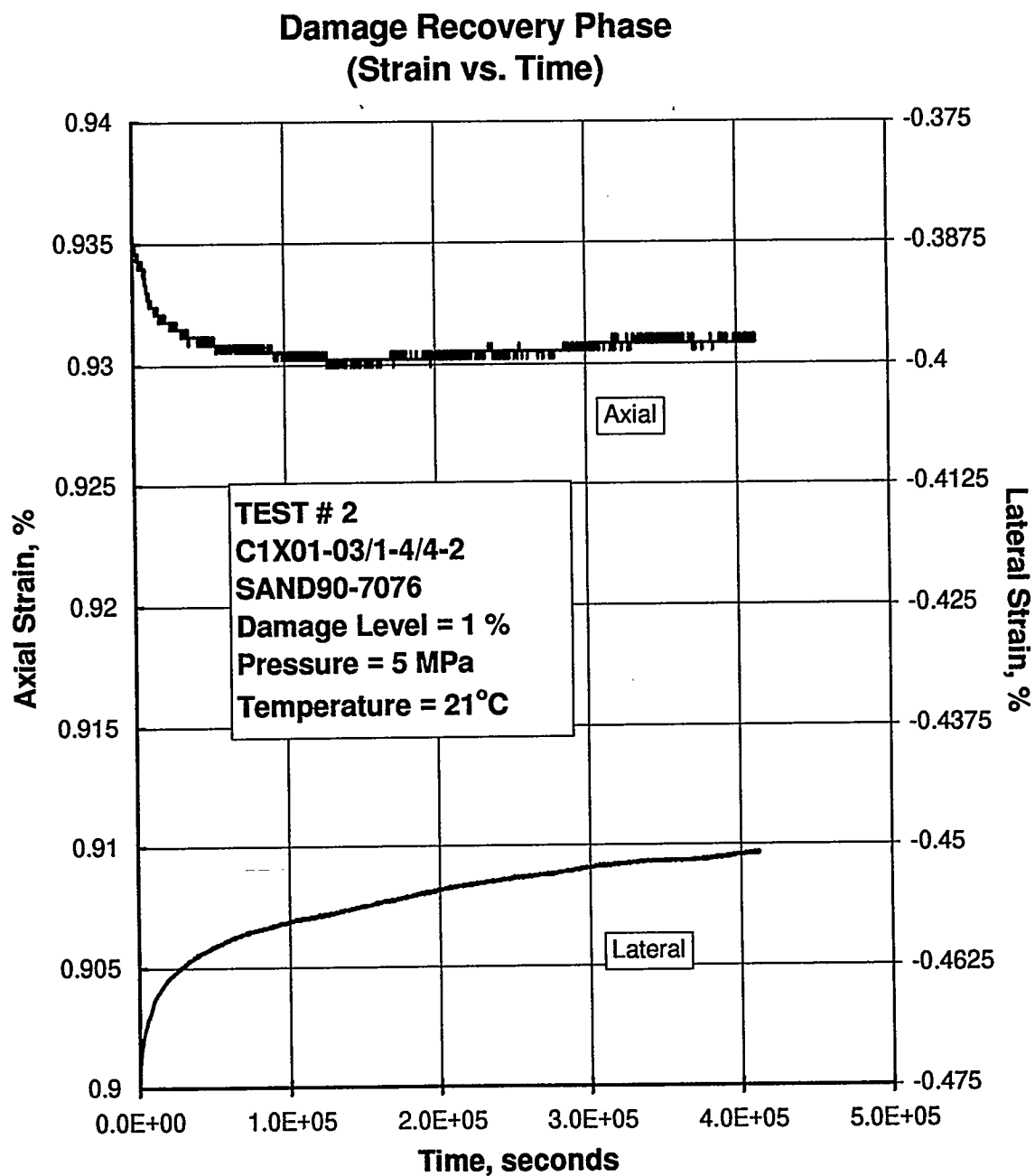
Figure E-54. Axial and Lateral Strain as a Function of Time During the Hydrostatic Loading to Recover Damage in Specimen C1X01-03/1-4/4-2.
