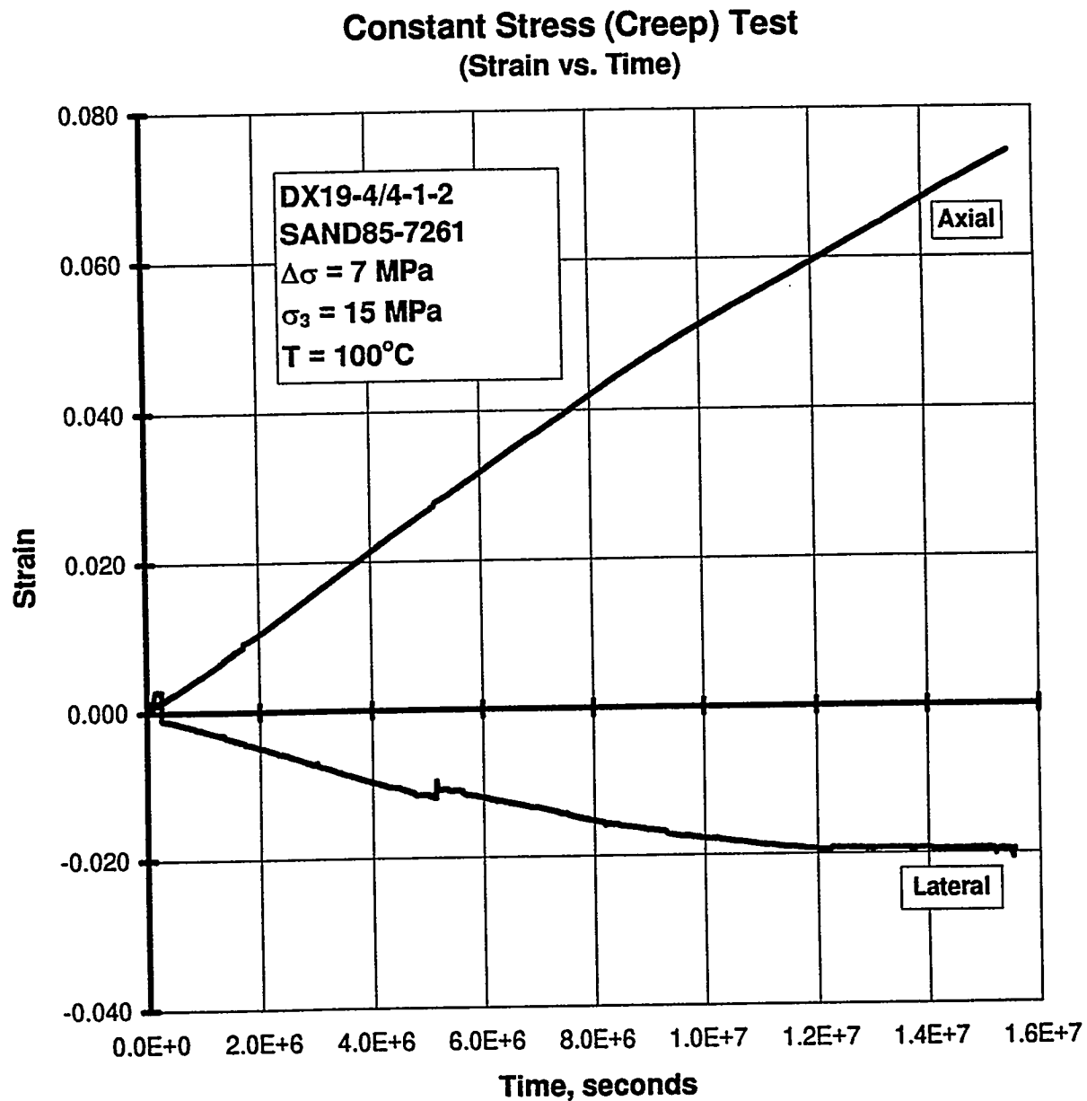
Figure C-80. Axial Strain and Lateral Strain Versus Time for a Creep Test: Specimen DX19-4/4-1-2; Stage 1 of 1 (Anomalous Test Result. Unknown Cause).
