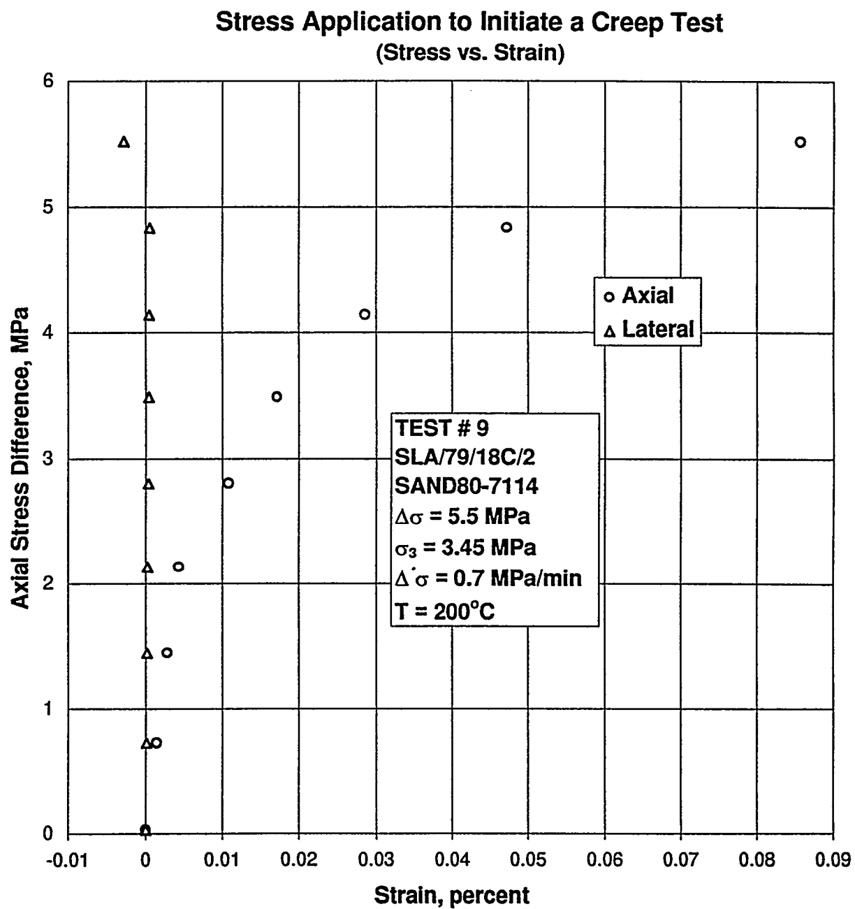
Figure B-54. Axial Stress Difference Versus Axial and Lateral Strain for Stress Application to Initiate a Creep Test: Specimen SLA/79/18C/2; Stage 1 of 1.
