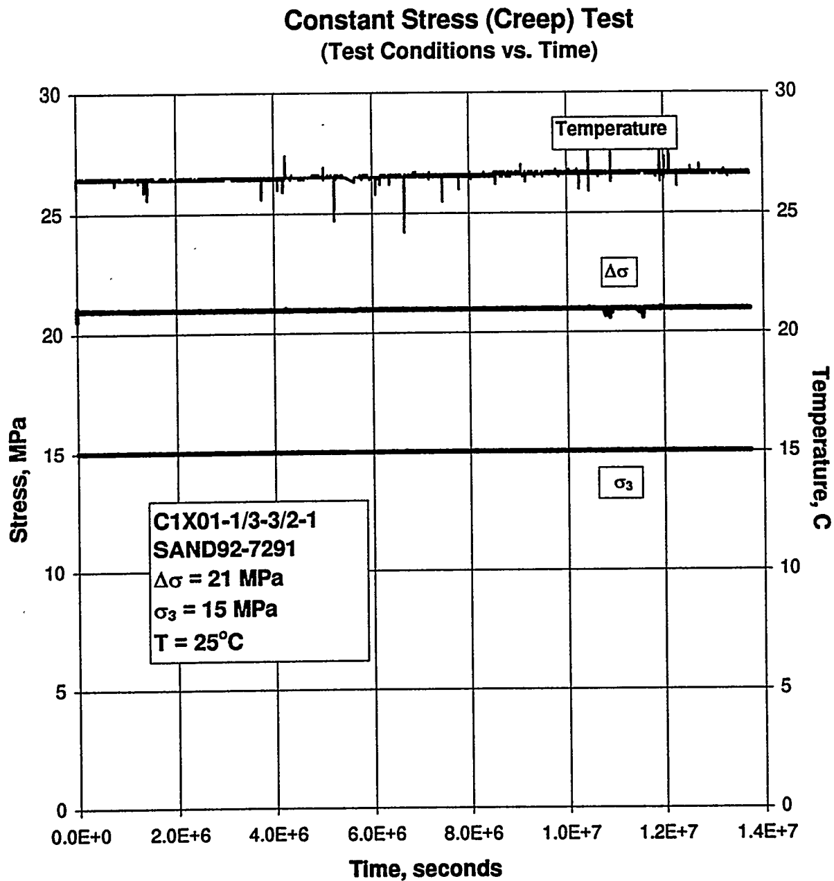
Figure C-7. Test Conditions Versus Time for a Creep Test: Specimen C1X01-1/3-3/2-1; Stage 1 of 1.
