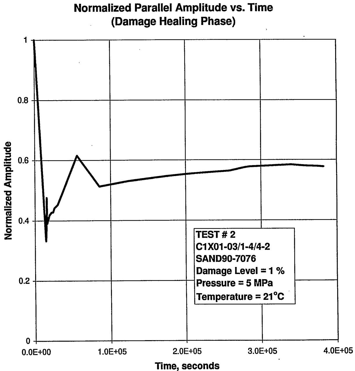
Figure E-56. Normalized Parallel Amplitude as a Function of Time During the Hydrostatic Loading to Recover Damage in Specimen C1X01-03/1-4/4-2.
