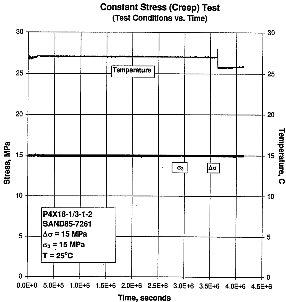
Figure C-41. Test Conditions Versus Time for a Creep Test: Specimen P4X18-1/3-1-2; Stage 1 of 1 (Argillaceous Salt).
