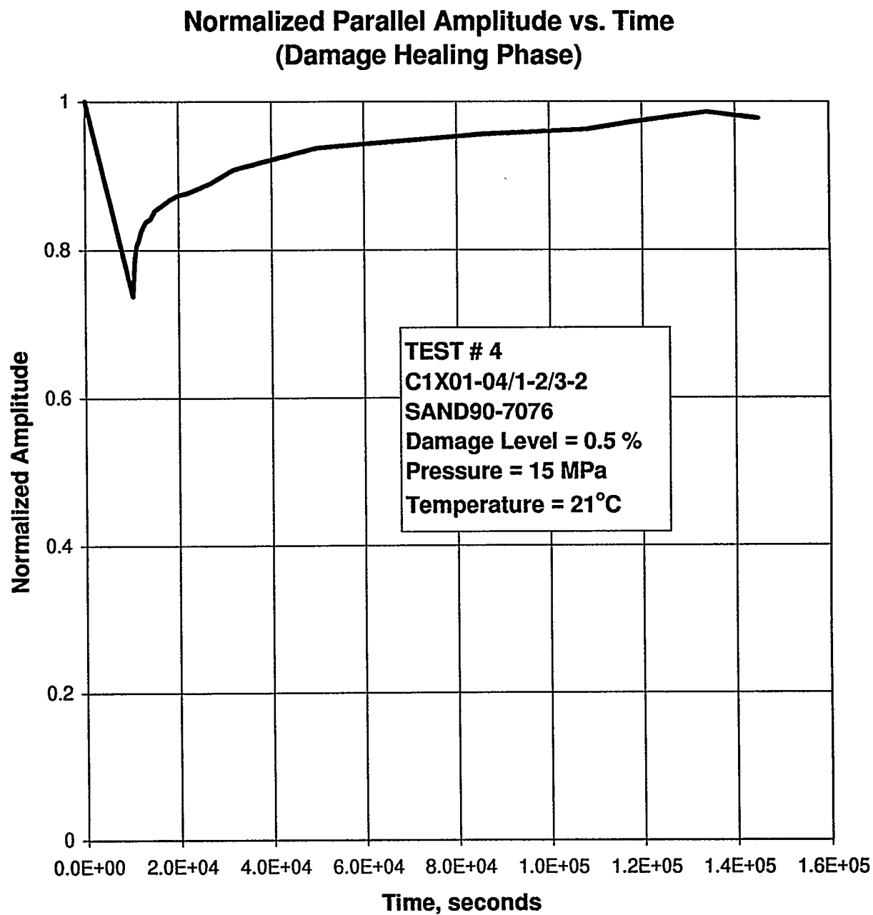
Figure E-80. Normalized Parallel Amplitude as a Function of Time During the Hydrostatic Loading to Recover Damage in Specimen C1X01-04/1-2/3-2.
