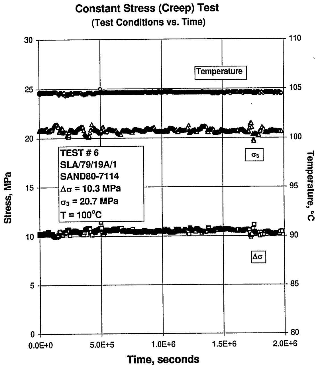
Figure B-43. Test Conditions Versus Time for a Creep Test: Specimen SLA/79/19A/1; Stage 1 of 1.
