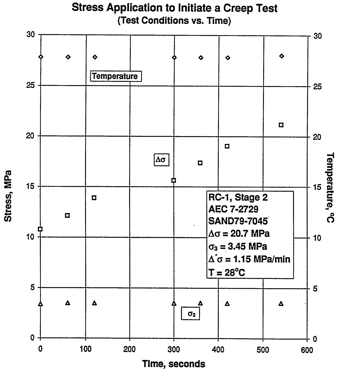
Figure B-147. Test Conditions Versus Time for Stress Application to Initiate a Creep Test: Specimen AEC7-2729; Stage 2 of 3.
