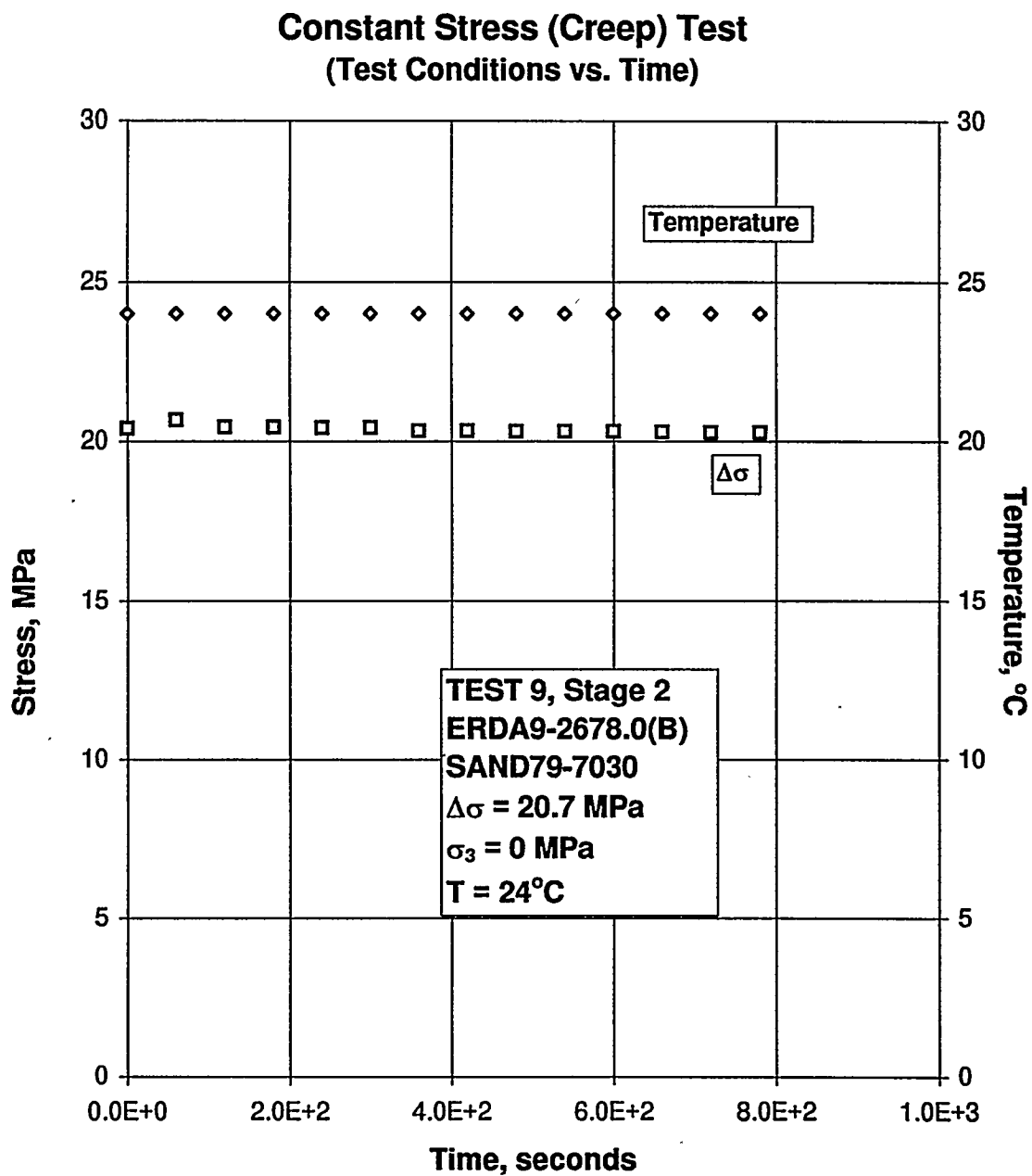
Figure B-111. Test Conditions Versus Time for a Creep Test: Specimen ERDA9-2678.0 (B); Stage 2 of 2 (Specimen Rupture Terminated Test).
