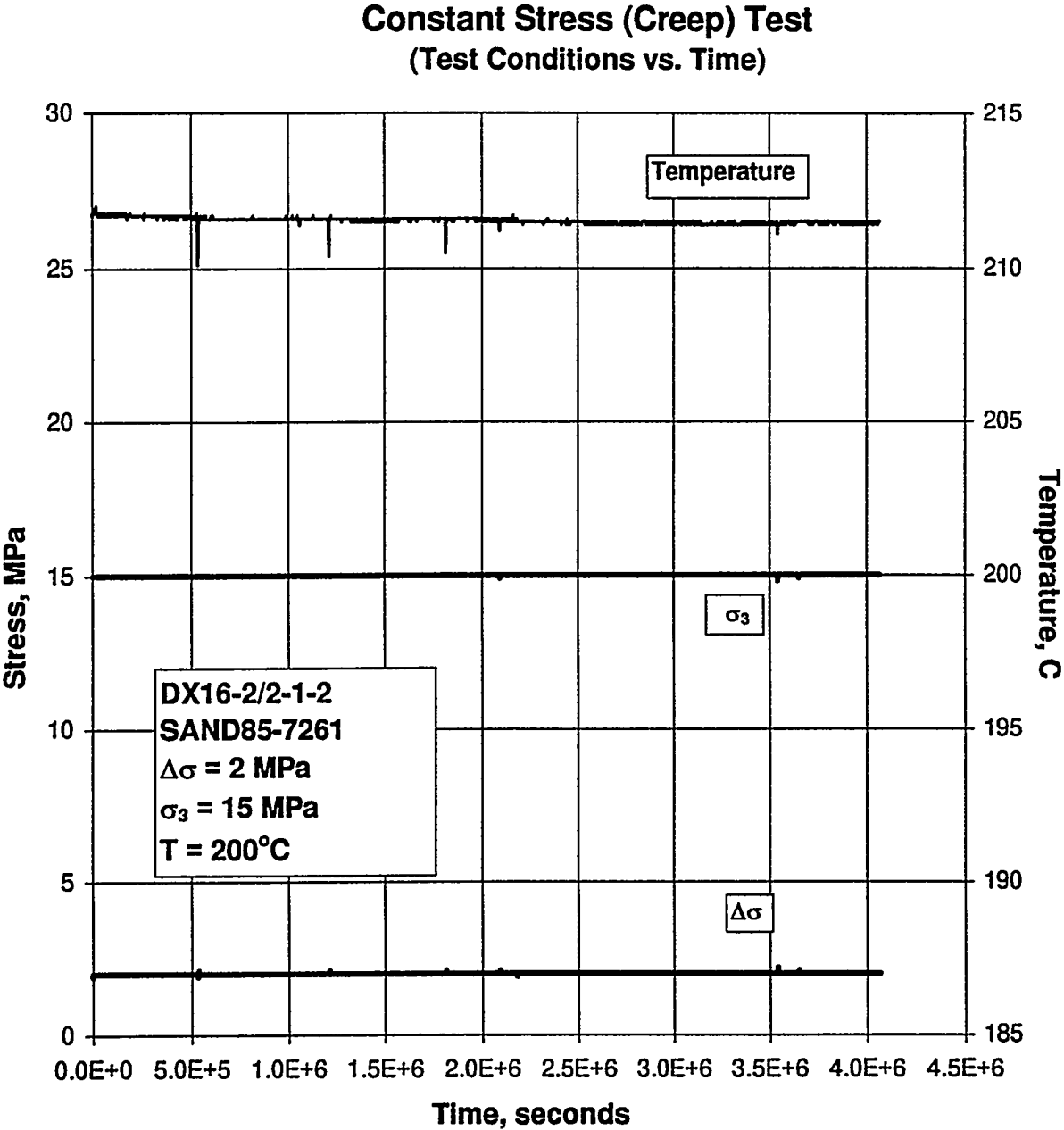
Figure C-83. Test Conditions Versus Time for a Creep Test: Specimen DX16-2/2-1-2; Stage 1 of 1.
