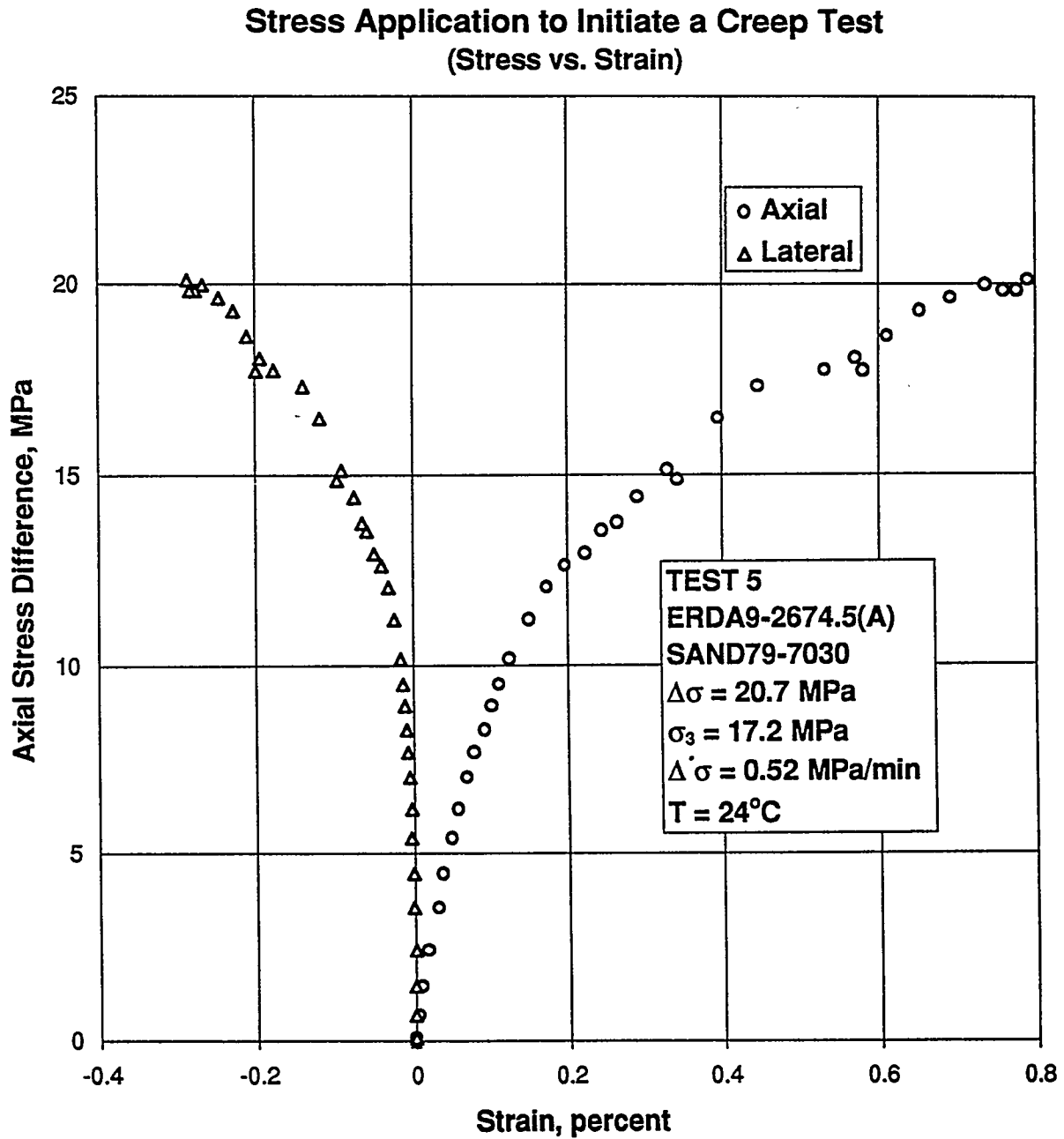
Figure B-90. Axial Stress Difference Versus Axial and Lateral Strain for Stress Application to Initiate a Creep Test: Specimen ERDA9-2674.5 (A); Stage 1 of 1.
