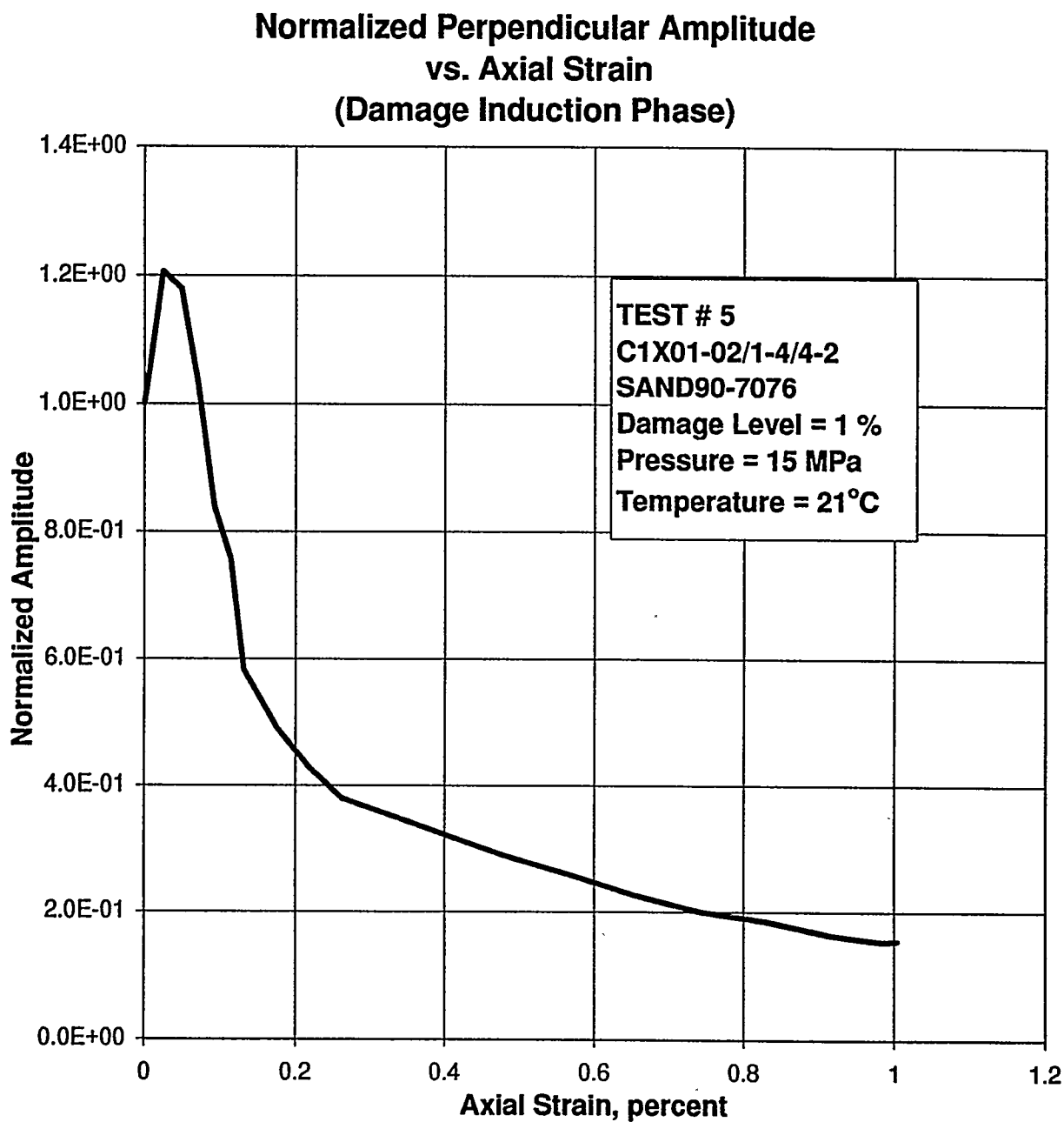
Figure E-85. Normalized Perpendicular Amplitude as a Function of Axial Strain During the Quasi-Static Loading to Induce Damage in Specimen C1X01-02/1-4/4-2.
