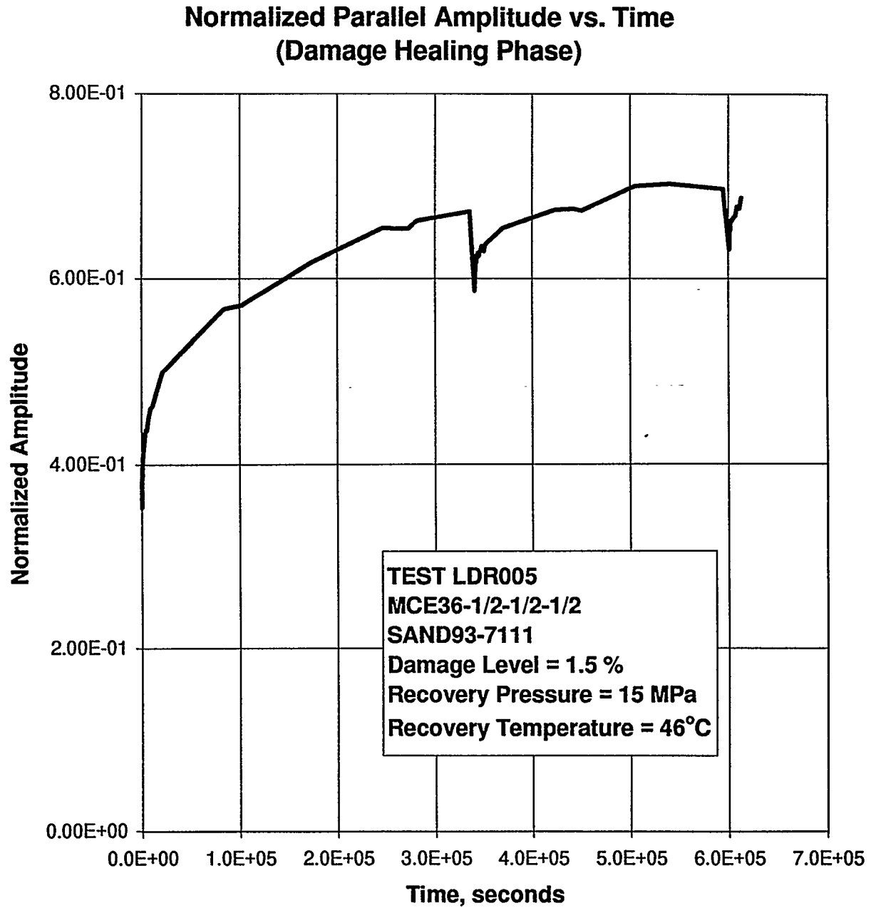
Figure E-26. Normalized Parallel Amplitude as a Function of Time During the Hydrostatic Loading to Recover Damage in Specimen MCE36-1/2-1/2-1/2.
