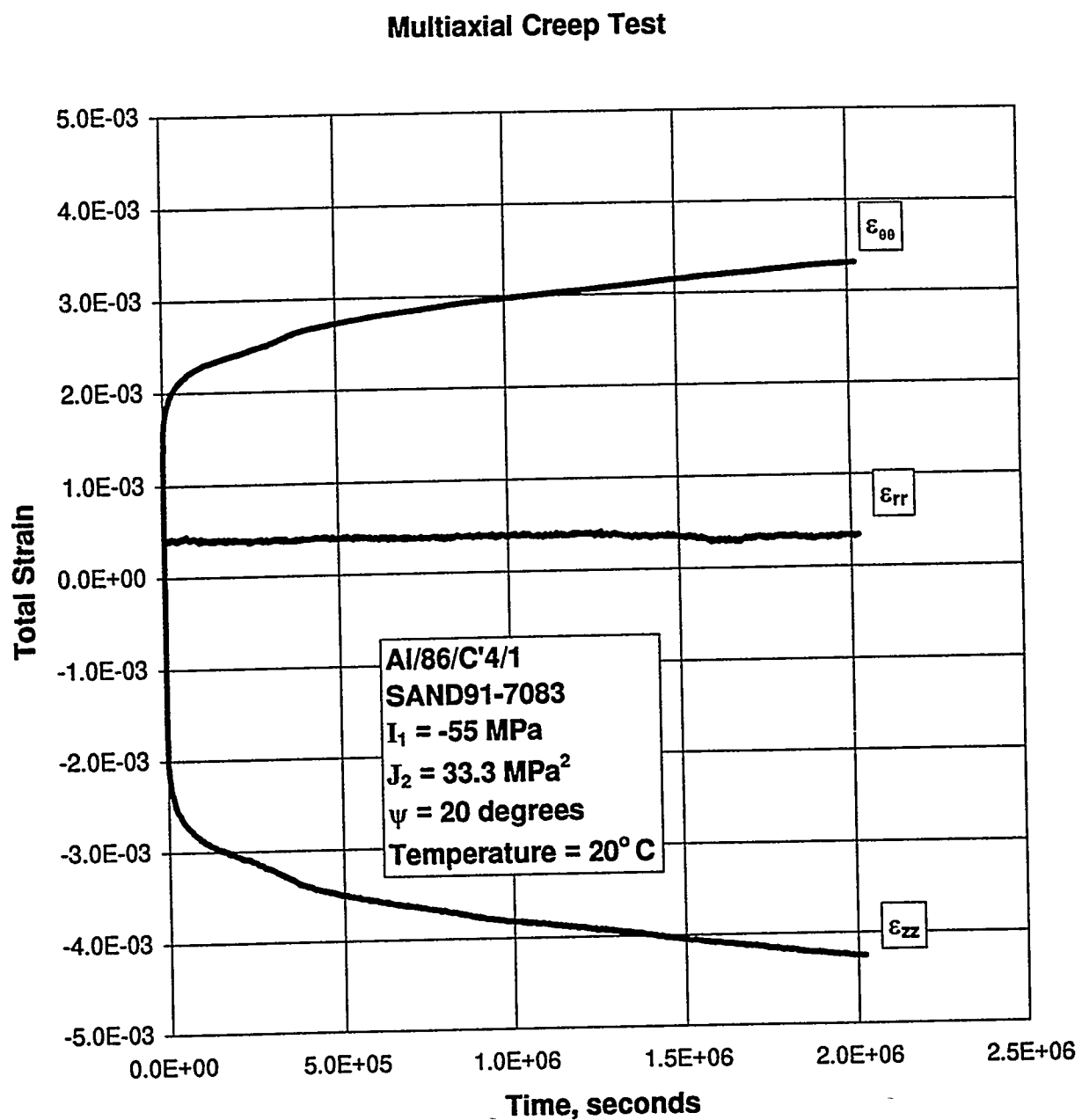
Figure D-8. Principal Strains Versus Time for a Multiaxial Creep Test: Specimen AI/86/C'4/1.
