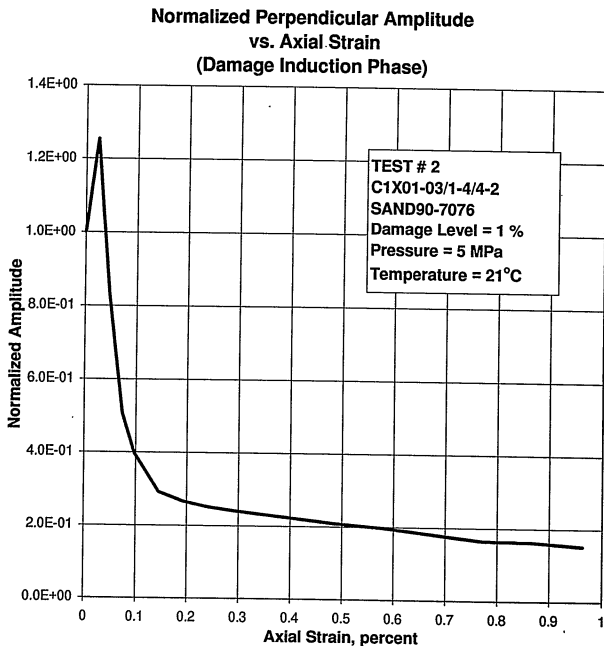
Figure E-49. Normalized Perpendicular Amplitude as a Function of Axial Strain During the Quasi-Static Loading to Induce Damage in Specimen C1X01-03/1-4/4-2.
