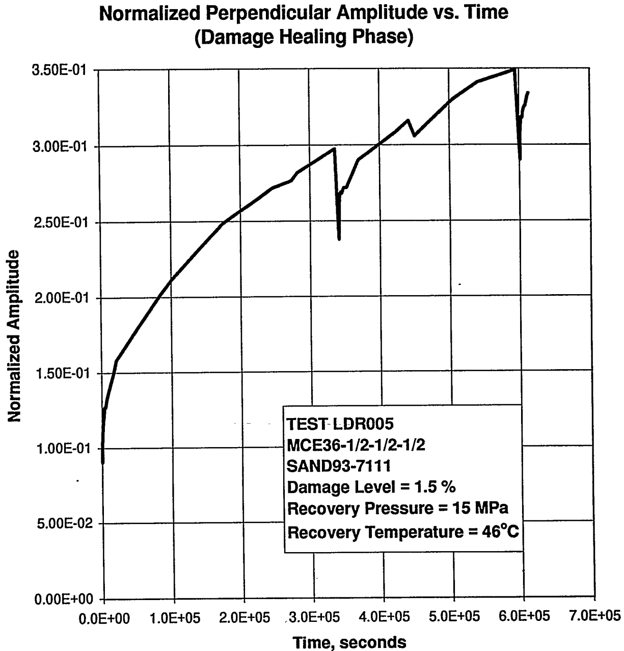
Figure E-25. Normalized Perpendicular Amplitude as a Function of Time During the Hydrostatic Loading to Recover Damage in Specimen MCE36-1/2-1/2-1/2.
