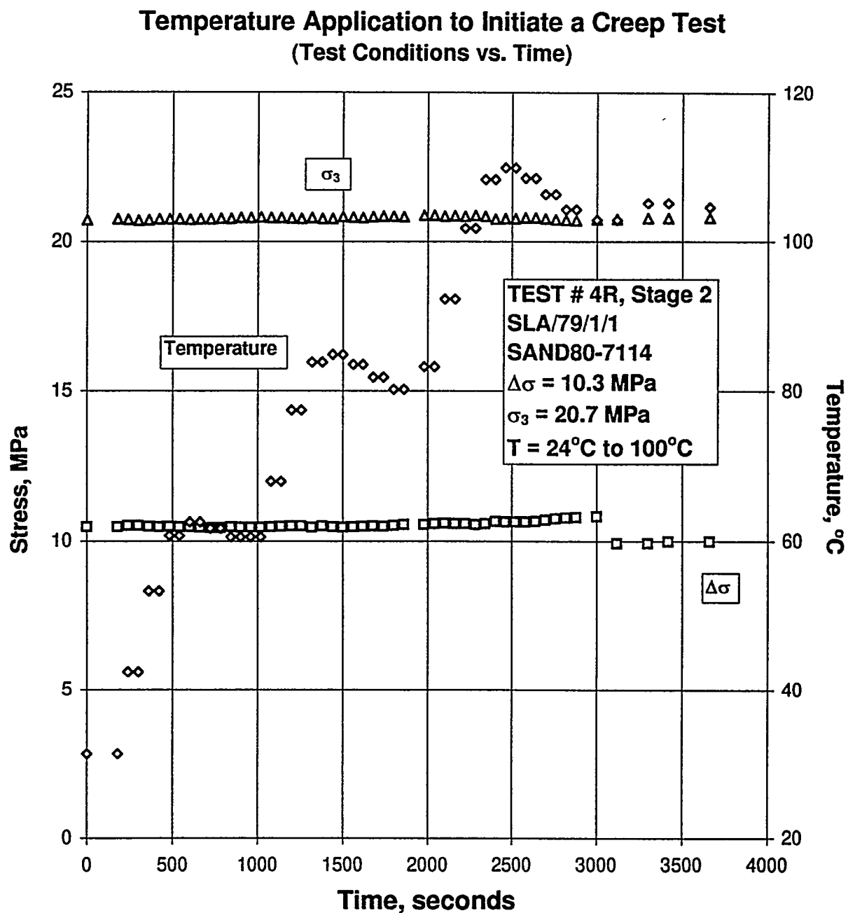
Figure B-34. Test Conditions Versus Time for Temperature Application to Initiate a Creep Test: Specimen SLA/79/1/1; Stage 2 of 2.
