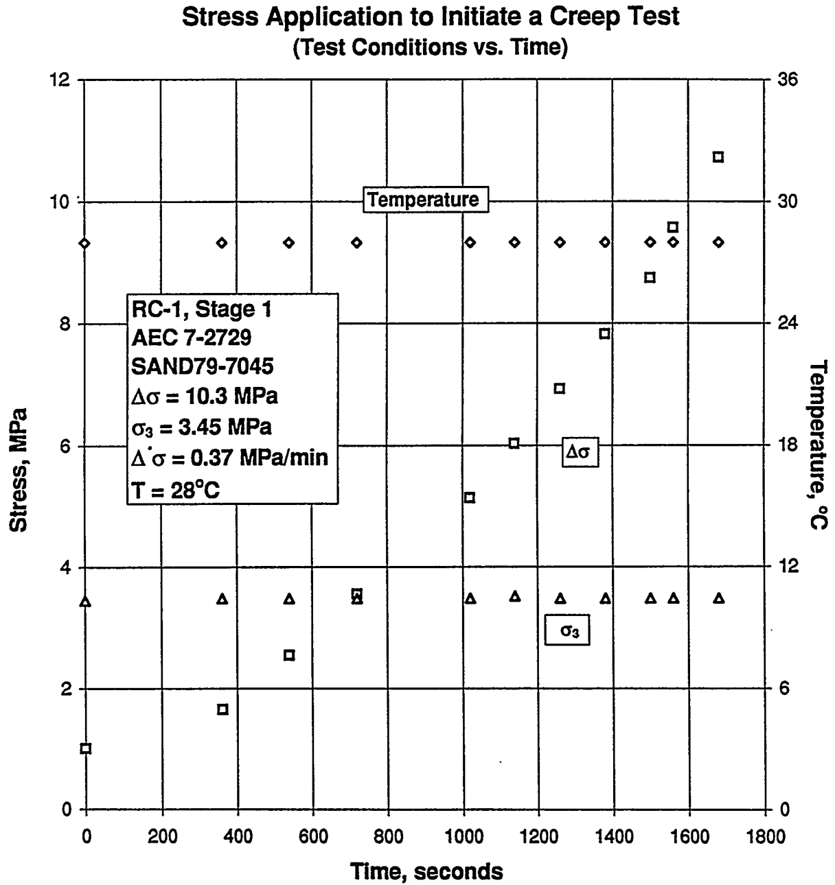
Figure B-143. Test Conditions Versus Time for Stress Application to Initiate a Creep Test: Specimen AEC7-2729; Stage 1 of 3.
