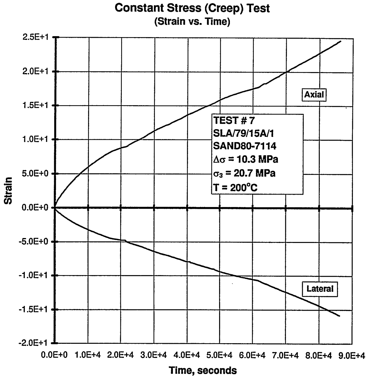
Figure B-48. Axial Strain and Lateral Strain Versus Time for a Creep Test: Specimen SLA/79/15A/1; Stage 1 of 1.
