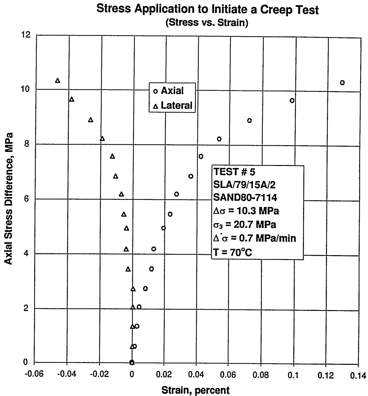
Figure B-38. Axial Stress Difference Versus Axial and Lateral Strain for Stress Application to Initiate a Creep Test: Specimen SLA/79/15A/2; Stage 1 of 1.
