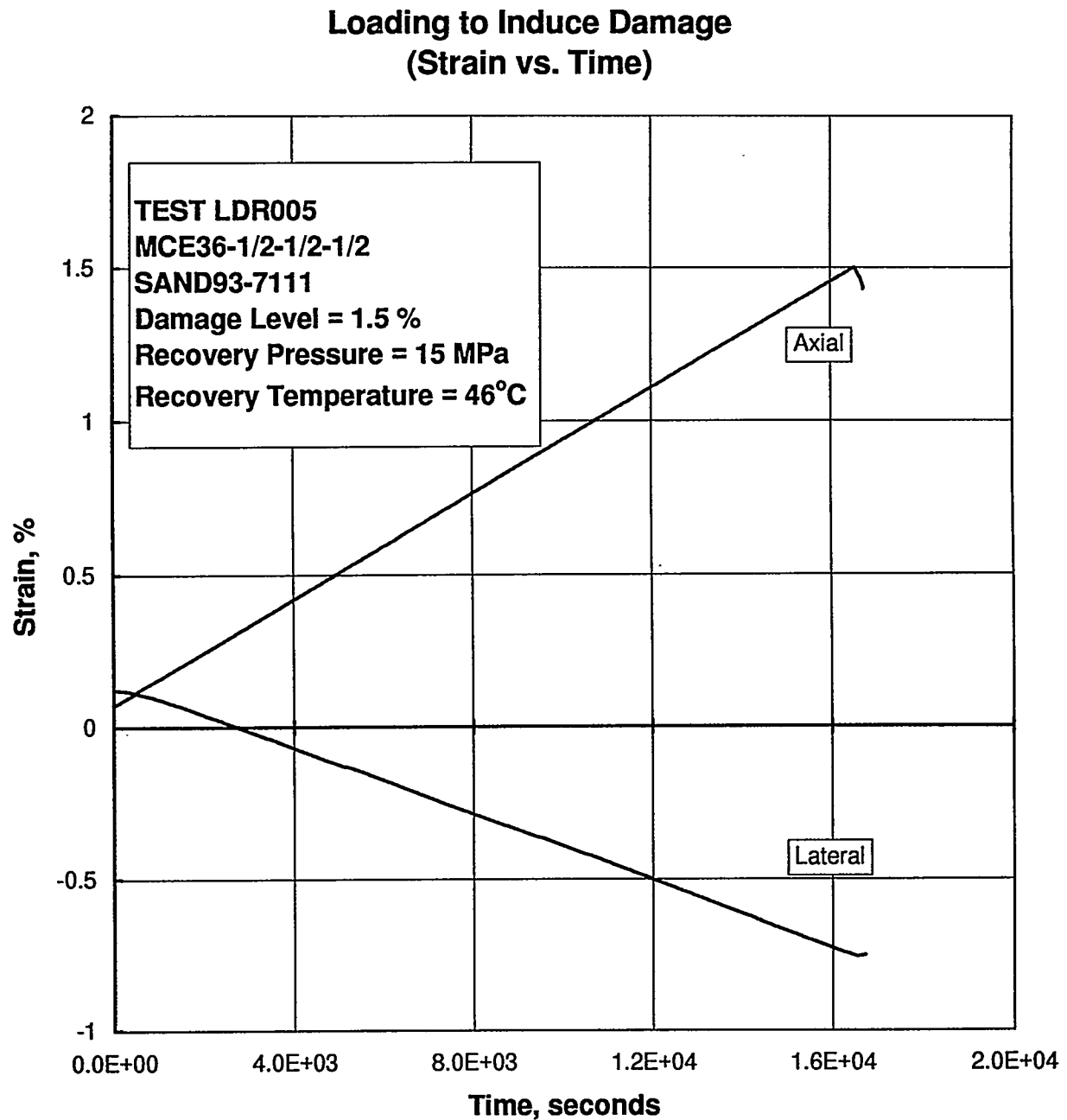
Figure E-18. Axial and Lateral Strain as a Function of Time During the Quasi-Static Loading to Induce Damage in Specimen MCE36-1/2-1/2-1/2.
