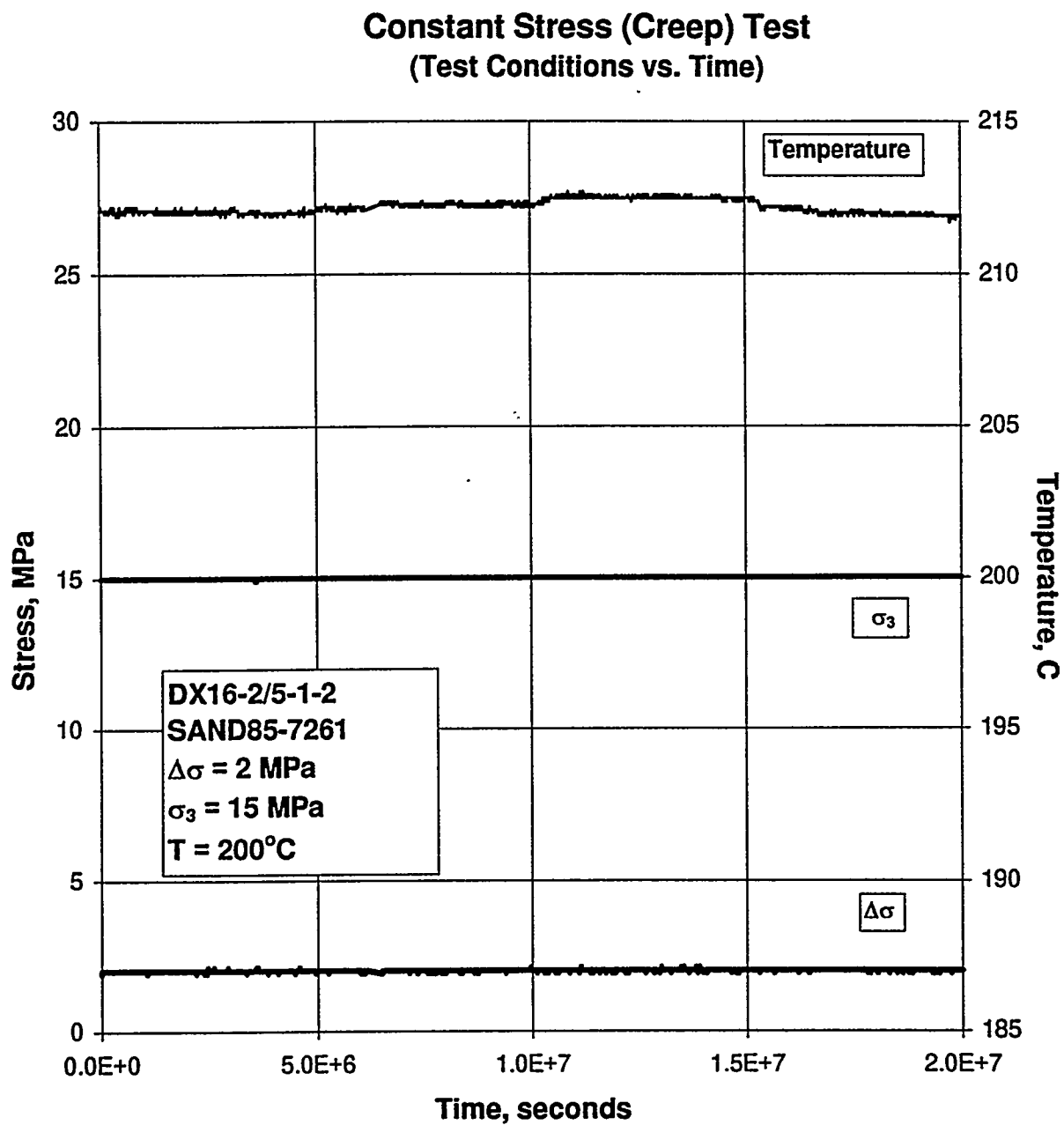
Figure C-85. Test Conditions Versus Time for a Creep Test: Specimen DX16-2/5-1-2; Stage 1 of 1.
