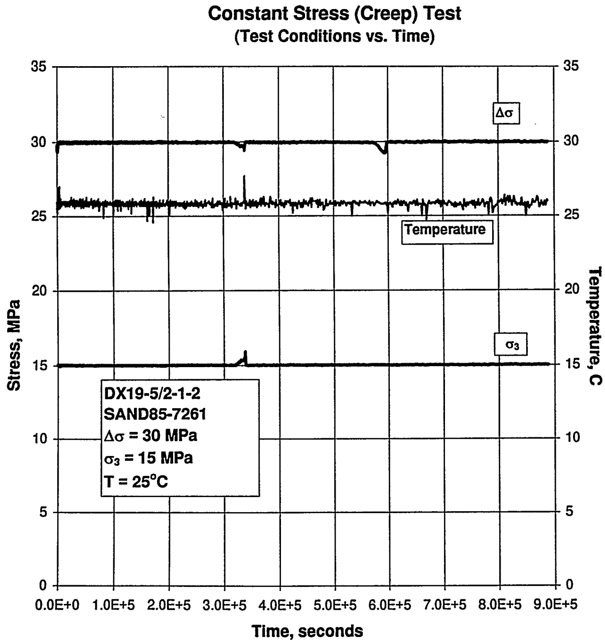
Figure C-73. Test Conditions Versus Time for a Creep Test: Specimen DX19-5/2-1-2; Stage 1 of 1.
