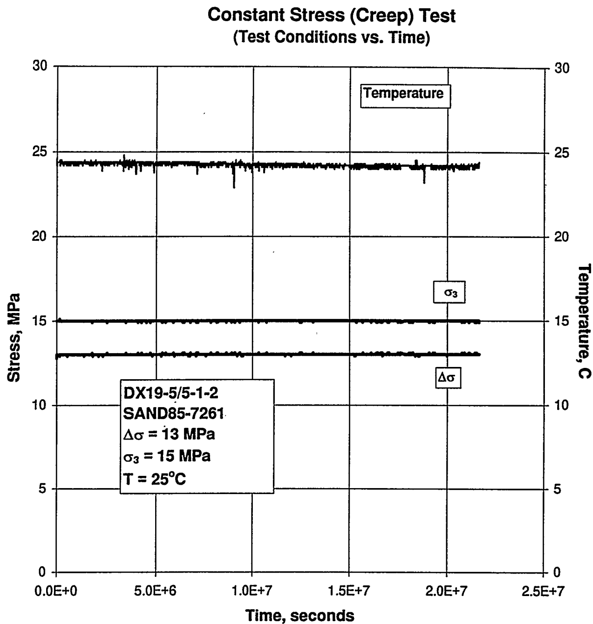
Figure C-59. Test Conditions Versus Time for a Creep Test: Specimen DX19-5/5-1-2; Stage 1 of 1.
