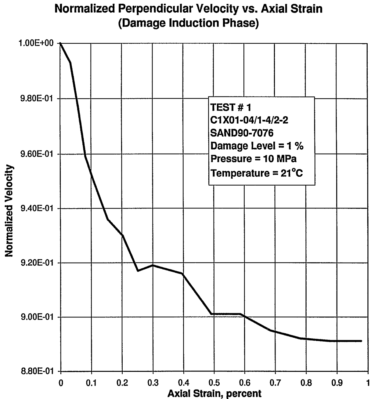
Figure E-39. Normalized Perpendicular Velocity as a Function of Axial Strain During the Quasi-Static Loading to Induce Damage in Specimen C1X01-04/1-4/2-2.
