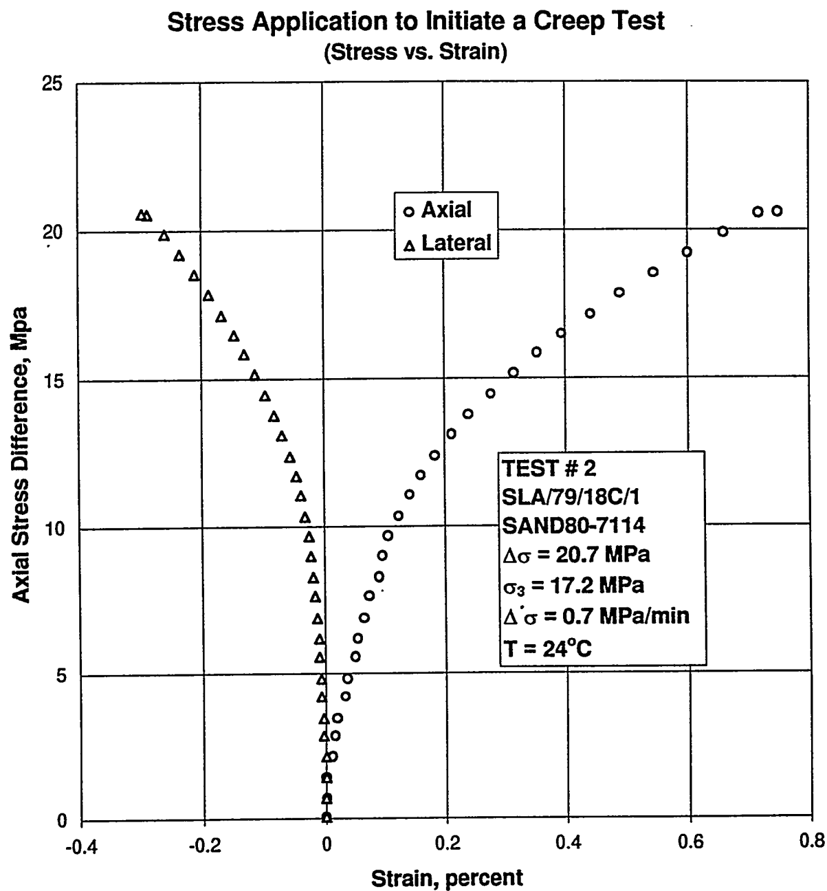
Figure B-19. Axial Stress Difference Versus Axial and Lateral Strain for Stress Application to Initiate a Creep Test: Specimen SLA/79/18C/1; Stage 1 of 1.
