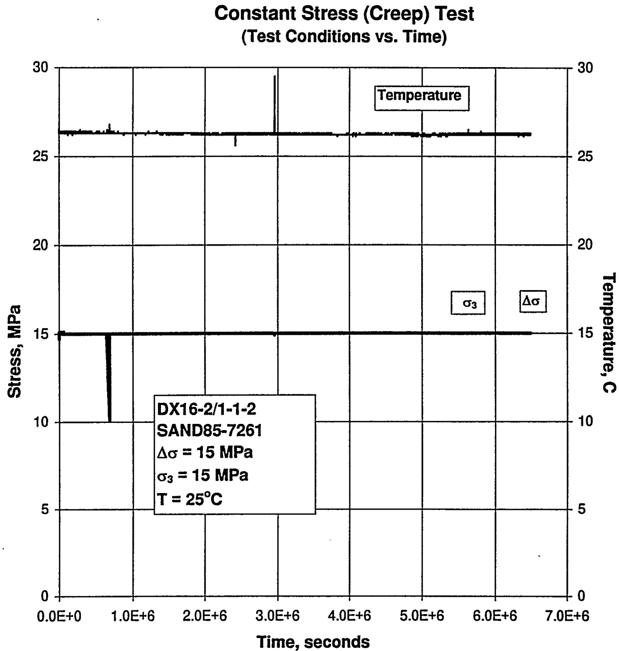
Figure C-61. Test Conditions Versus Time for a Creep Test: Specimen DX16-2/1-1-2; Stage 1 of 1.
