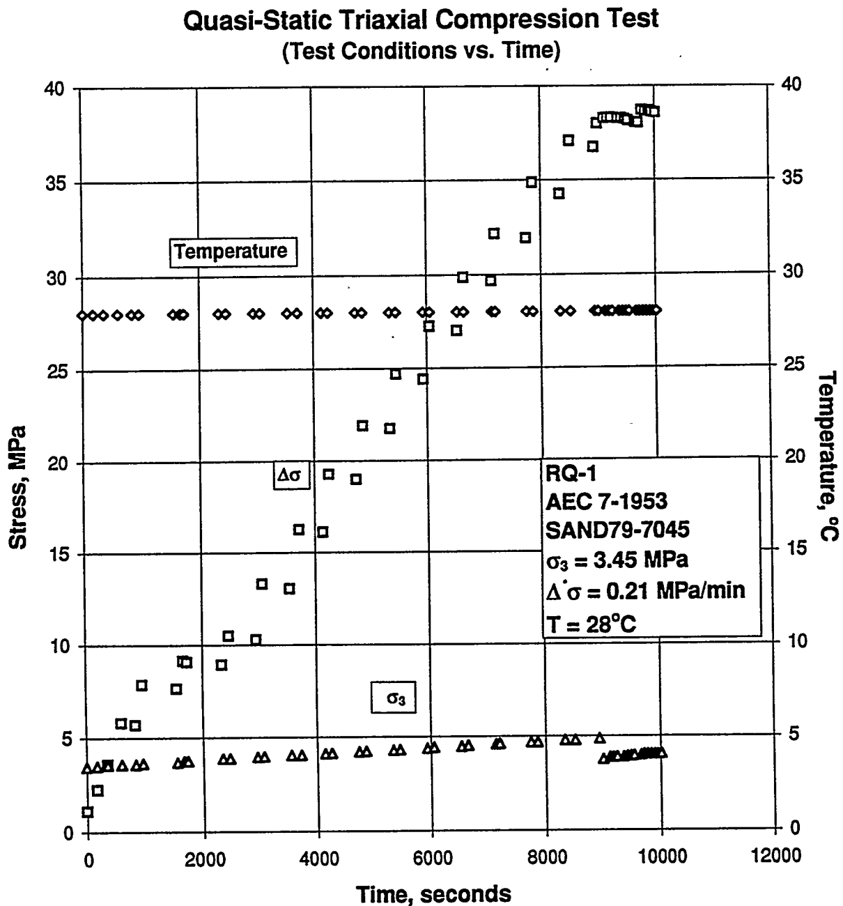
Figure A-1. Test Conditions Versus Time for a Quasi-Static Triaxial Compression Test: Specimen AEC7-1953.
