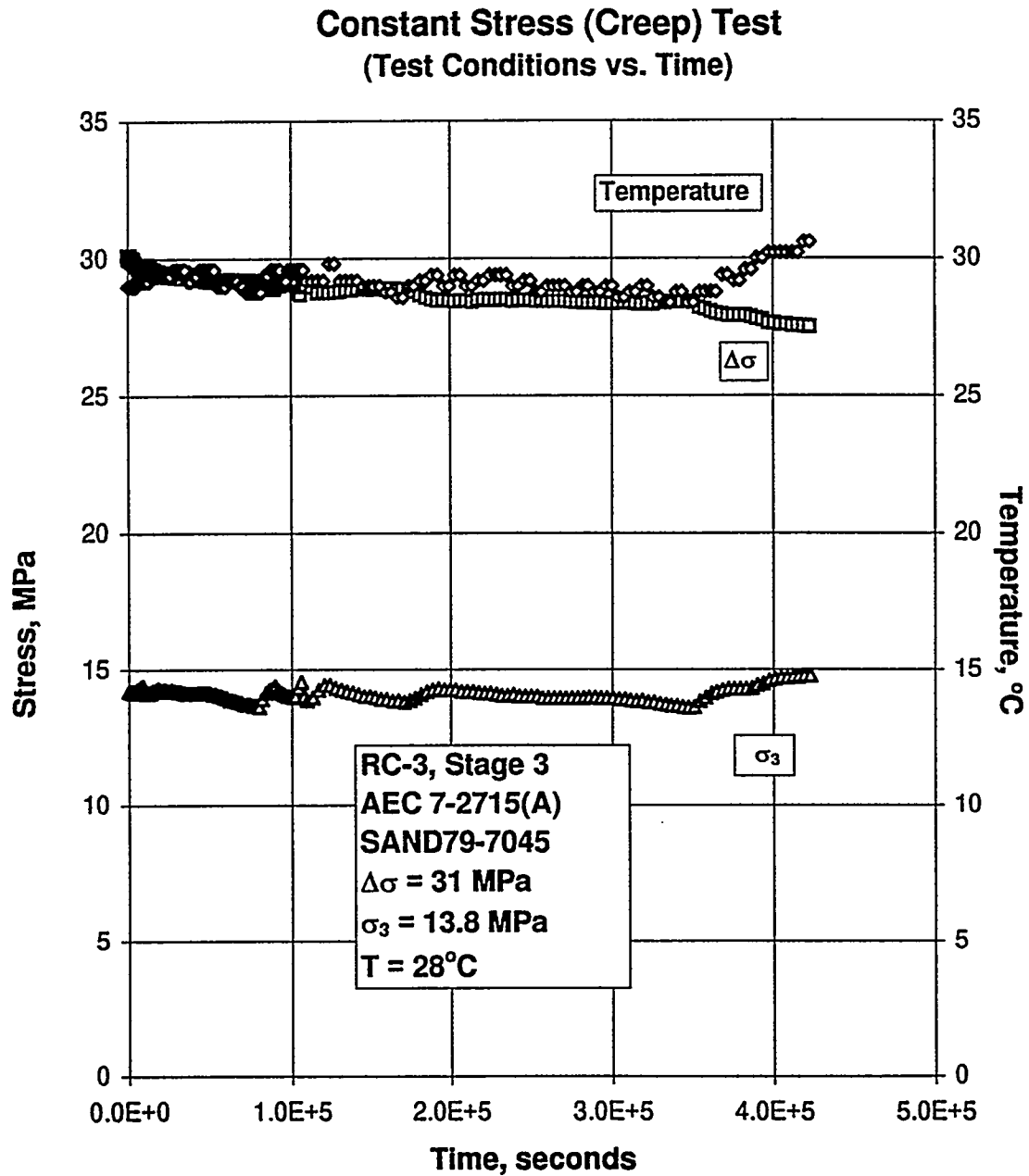
Figure B-173. Test Conditions Versus Time for a Creep Test: Specimen AEC7-2715 (A); Stage 3 of 3.
