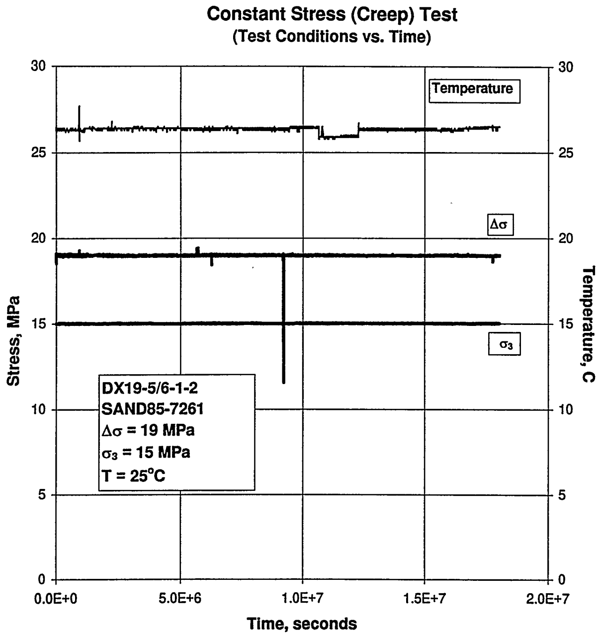
Figure C-67. Test Conditions Versus Time for a Creep Test: Specimen DX19-5/6-1-2; Stage 1 of 1.
