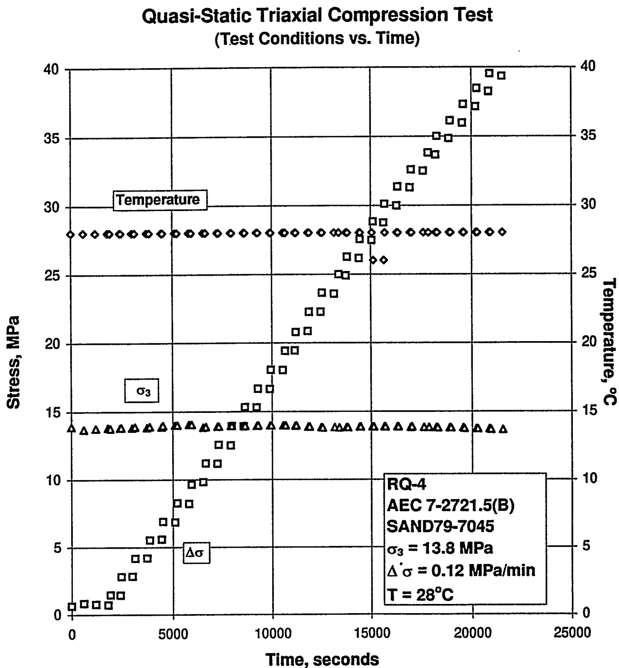
Figure A-7. Test Conditions Versus Time for a Quasi-Static Triaxial Compression Test: Specimen AEC7-2721.5 (B).
