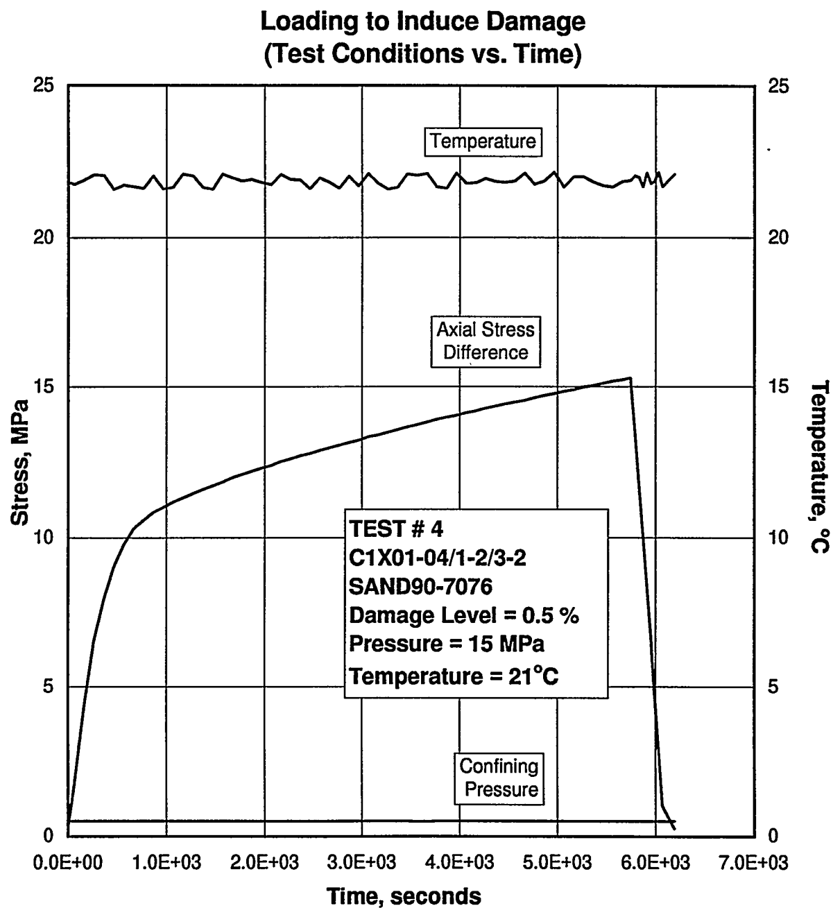
Figure E-71. Test Conditions as a Function of Time During the Quasi-Static Loading to Induce Damage in Specimen C1X01-04/1-2/3-2.
