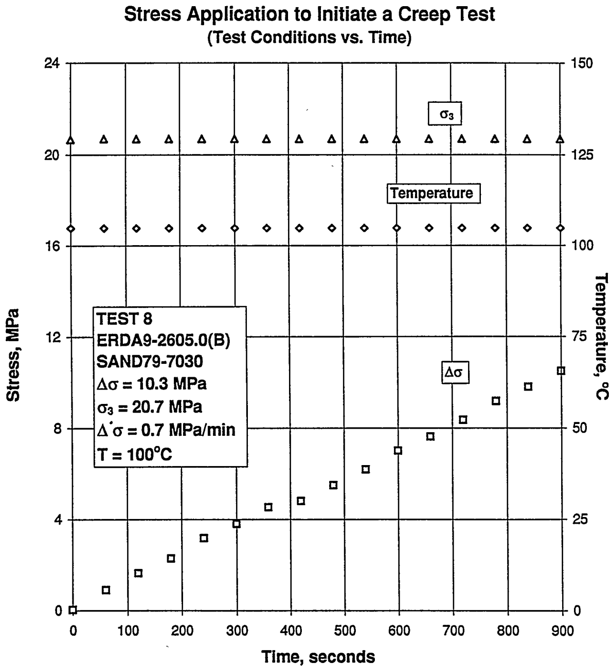
Figure B-101. Test Conditions Versus Time for Stress Application to Initiate a Creep Test: Specimen ERDA9-2605.0 (B); Stage 1 of 1.
