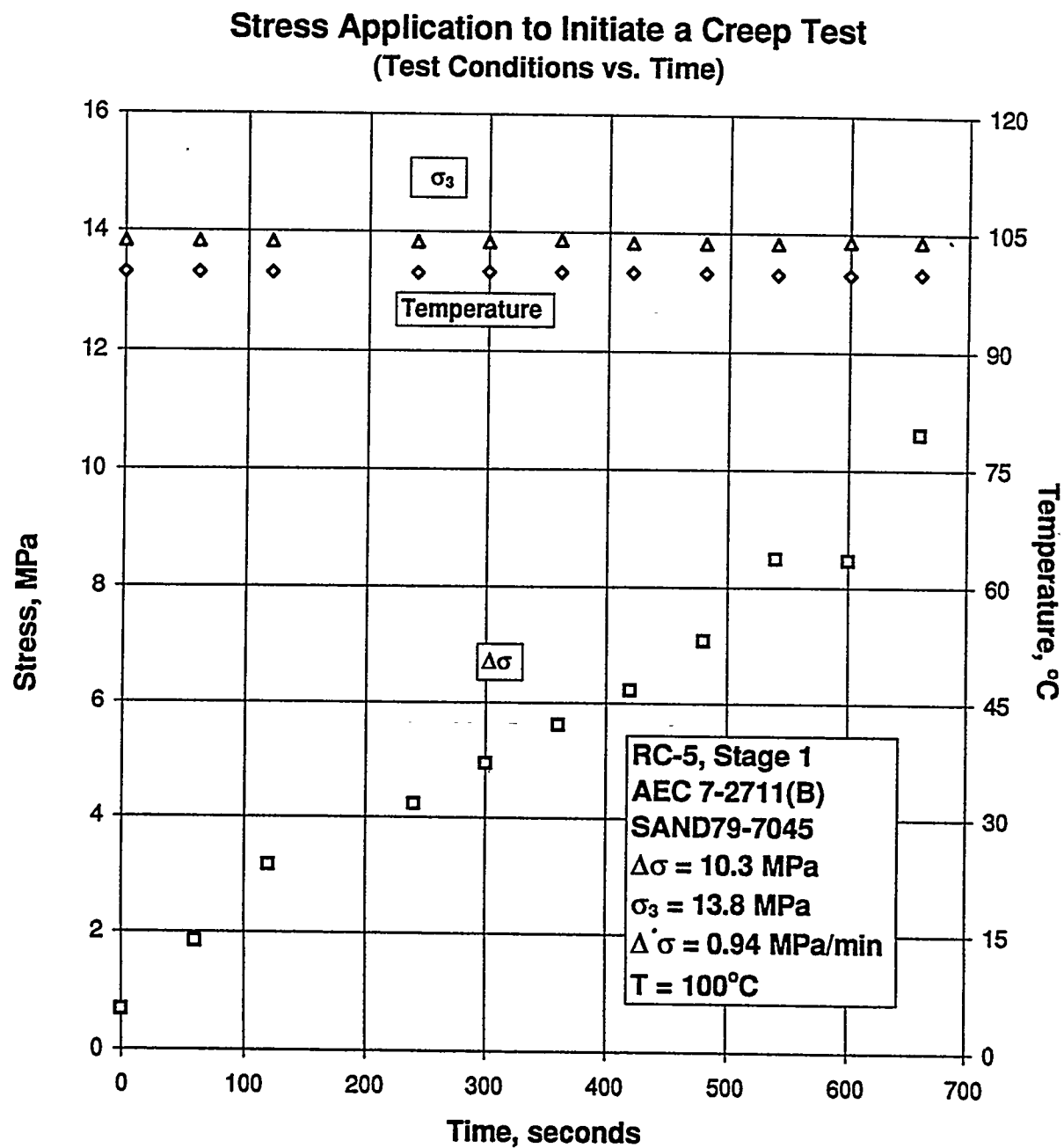
Figure B-183. Test Conditions Versus Time for Stress Application to Initiate a Creep Test: Specimen AEC7-2711 (B); Stage 1 of 2.
