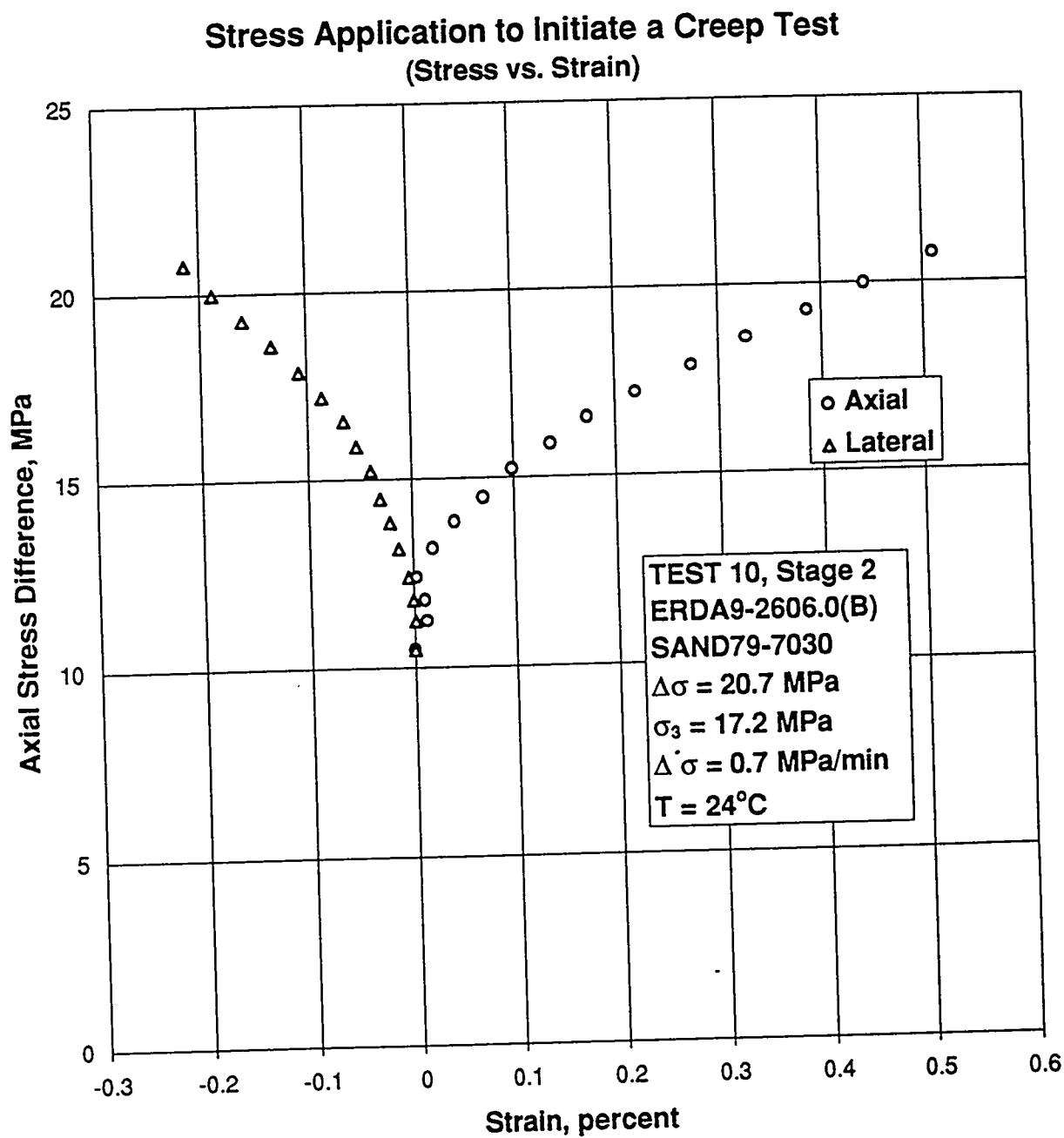
Figure B-118. Axial Stress Difference Versus Axial and Lateral Strain for Stress Application to Initiate a Creep Test: Specimen ERDA9-2606.0 (B); Stage 2 of 2.
