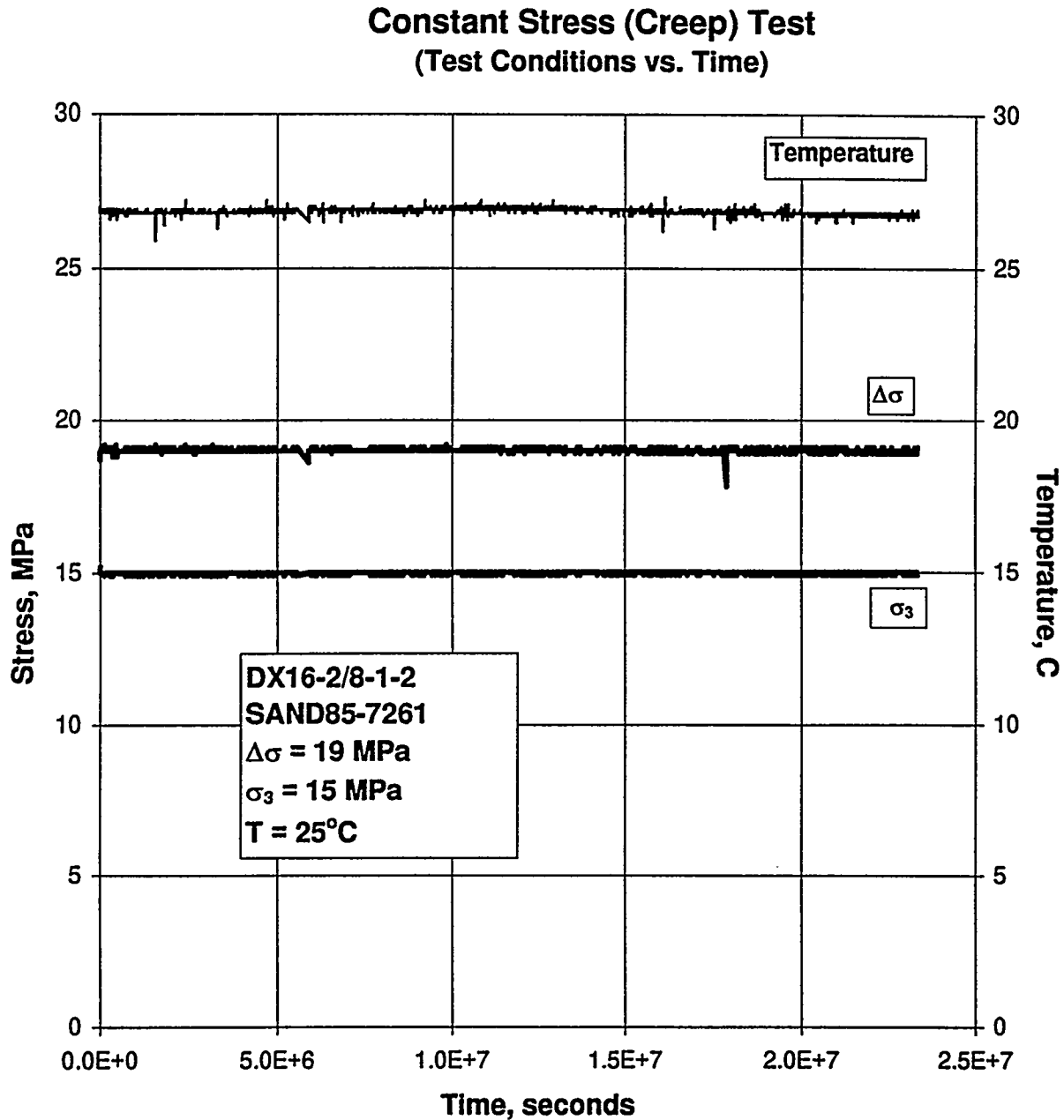
Figure C-65. Test Conditions Versus Time for a Creep Test: Specimen DX16-2/8-1-2; Stage 1 of 1.
