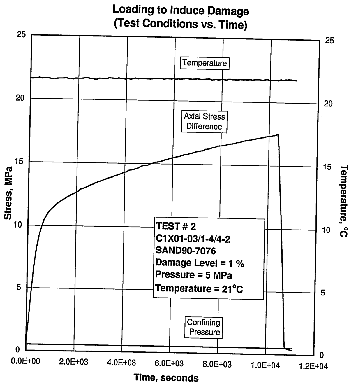
Figure E-47. Test Conditions as a Function of Time During the Quasi-Static Loading to Induce Damage in Specimen C1X01-03/1-4/4-2.
