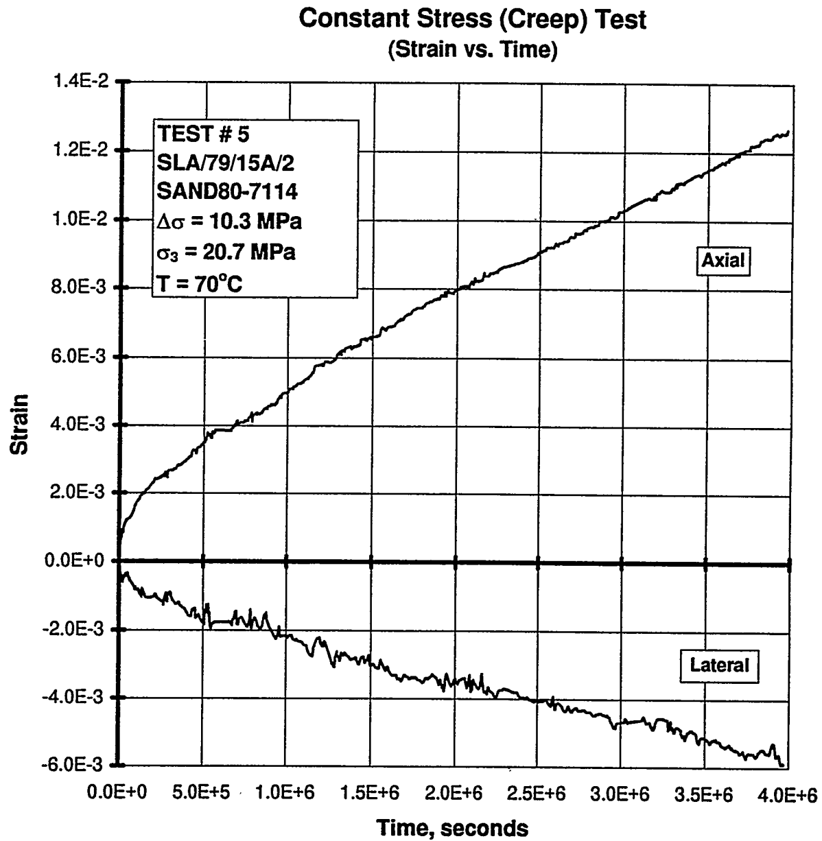
Figure B-40. Axial Strain and Lateral Strain Versus Time for a Creep Test: Specimen SLA/79/15A/2; Stage 1 of 1.
