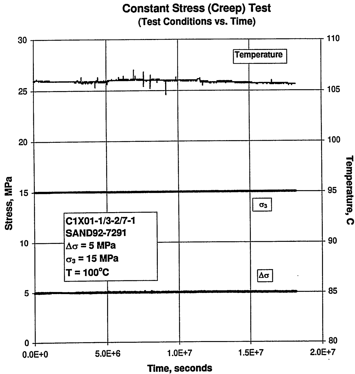
Figure C-11. Test Conditions Versus Time for a Creep Test: Specimen C1X01-1/3-2/7-1; Stage 1 of 1.
