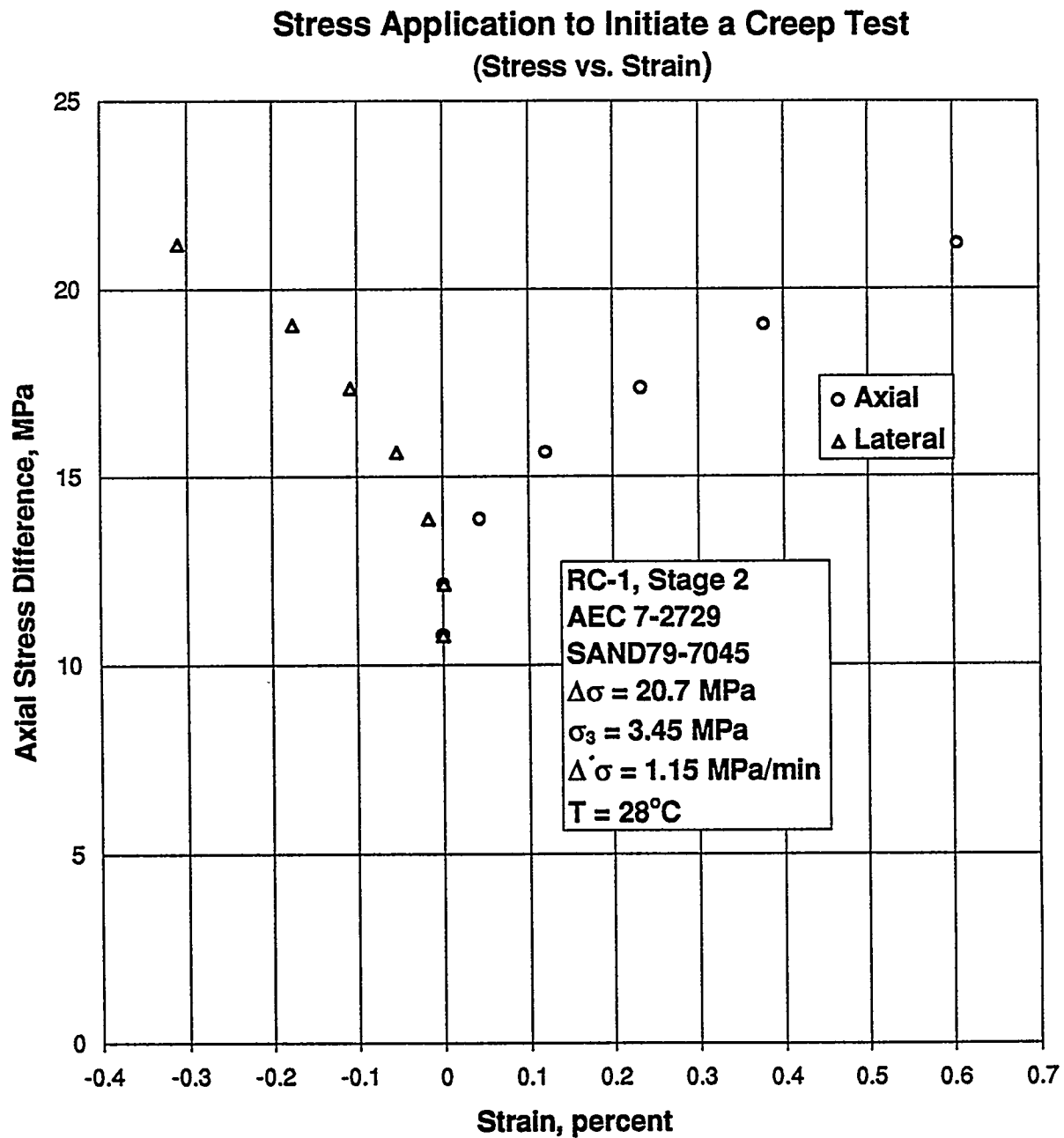
Figure B-148. Axial Stress Difference Versus Axial and Lateral Strain for Stress Application to Initiate a Creep Test: Specimen AEC7-2729; Stage 2 of 3.
