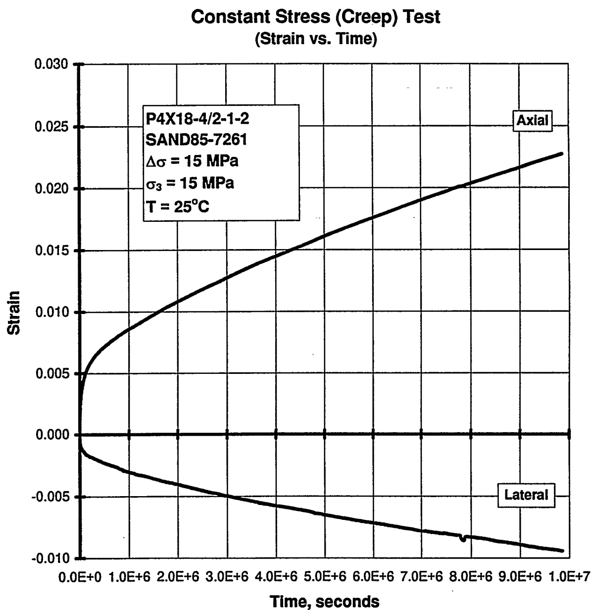
Figure C-44. Axial Strain and Lateral Strain Versus Time for a Creep Test: Specimen P4X18-4/2-1-2; Stage 1 of 1 (Argillaceous Salt).
