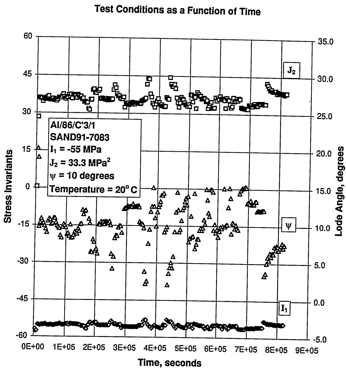
Figure D-3. Test Conditions Versus Time for a Multiaxial Creep Test: Specimen AI/86/C'3/1.
