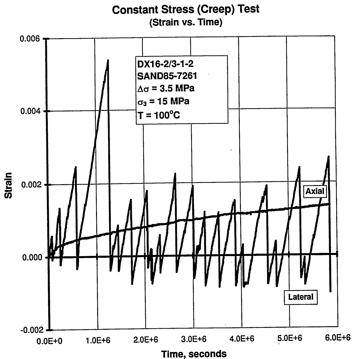
Figure C-78. Axial Strain and Lateral Strain Versus Time for a Creep Test: Specimen DX16-2/3-1-2; Stage 1 of 1.
