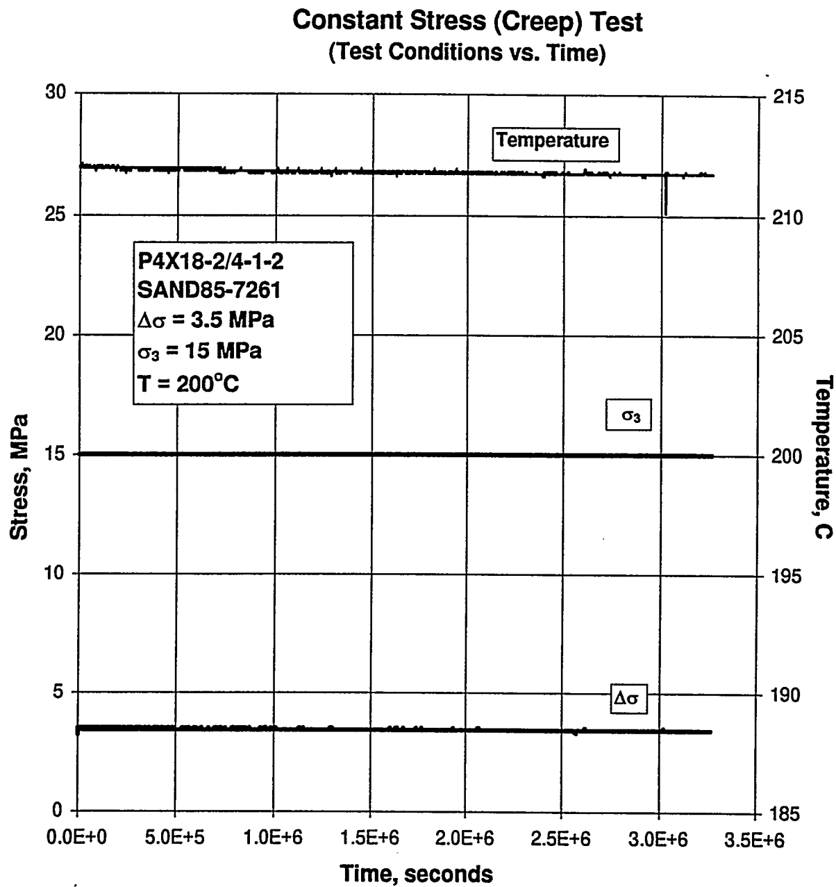
Figure C-53. Test Conditions Versus Time for a Creep Test: Specimen P4X18-2/4-1-2; Stage 1 of 1 (Argillaceous Salt).
