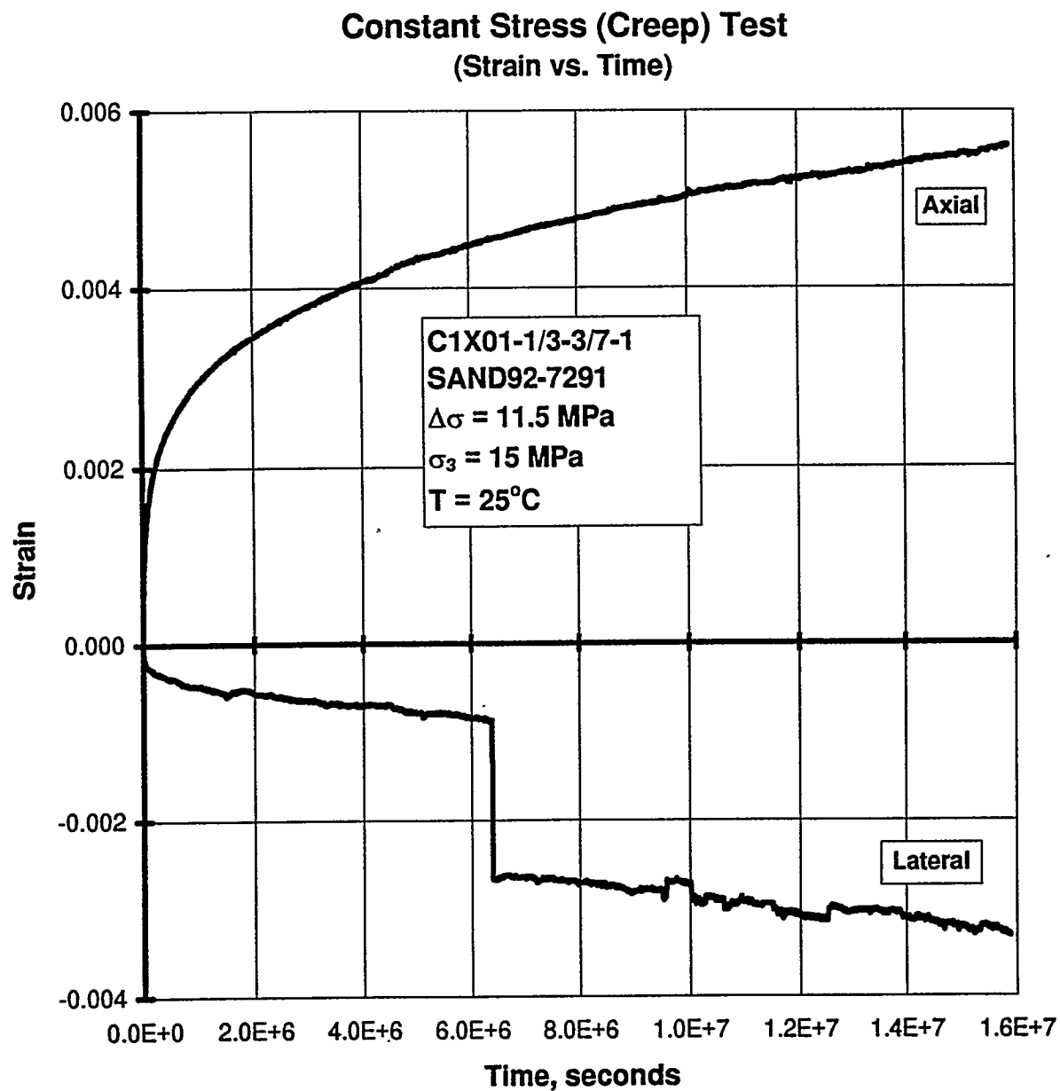
Figure C-2. Axial Strain and Lateral Strain Versus Time for a Creep Test: Specimen C1X01-1/3-3/7-1; Stage 1 of 1.
