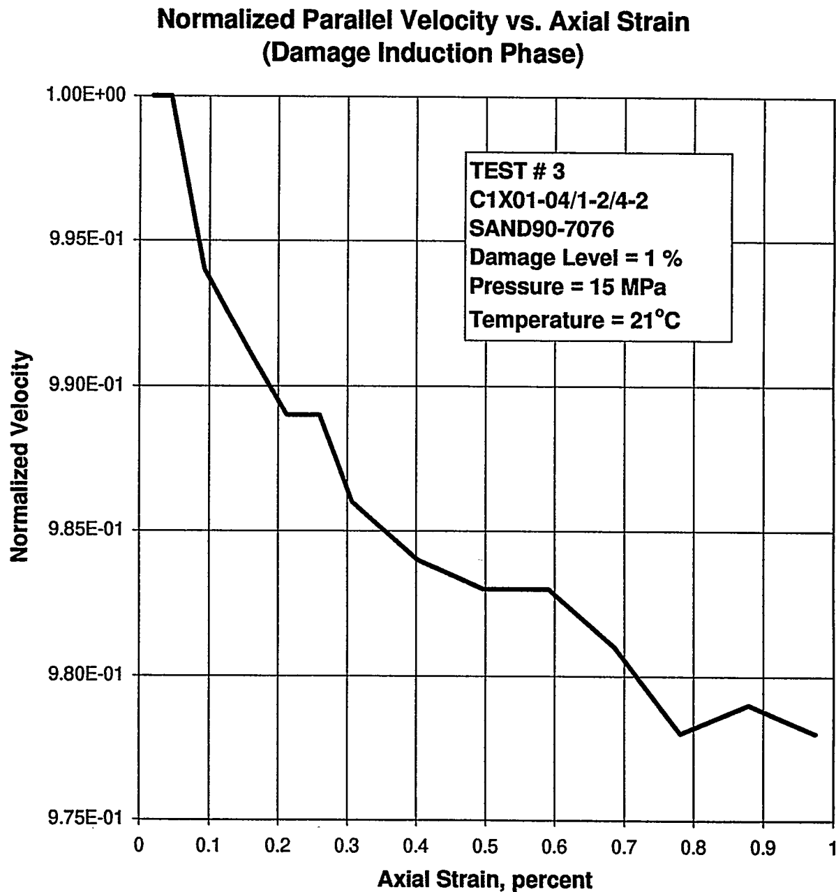
Figure E-64. Normalized Parallel Velocity as a Function of Axial Strain During the Quasi-Static Loading to Induce Damage in Specimen C1X01-04/1-2/4-2.
