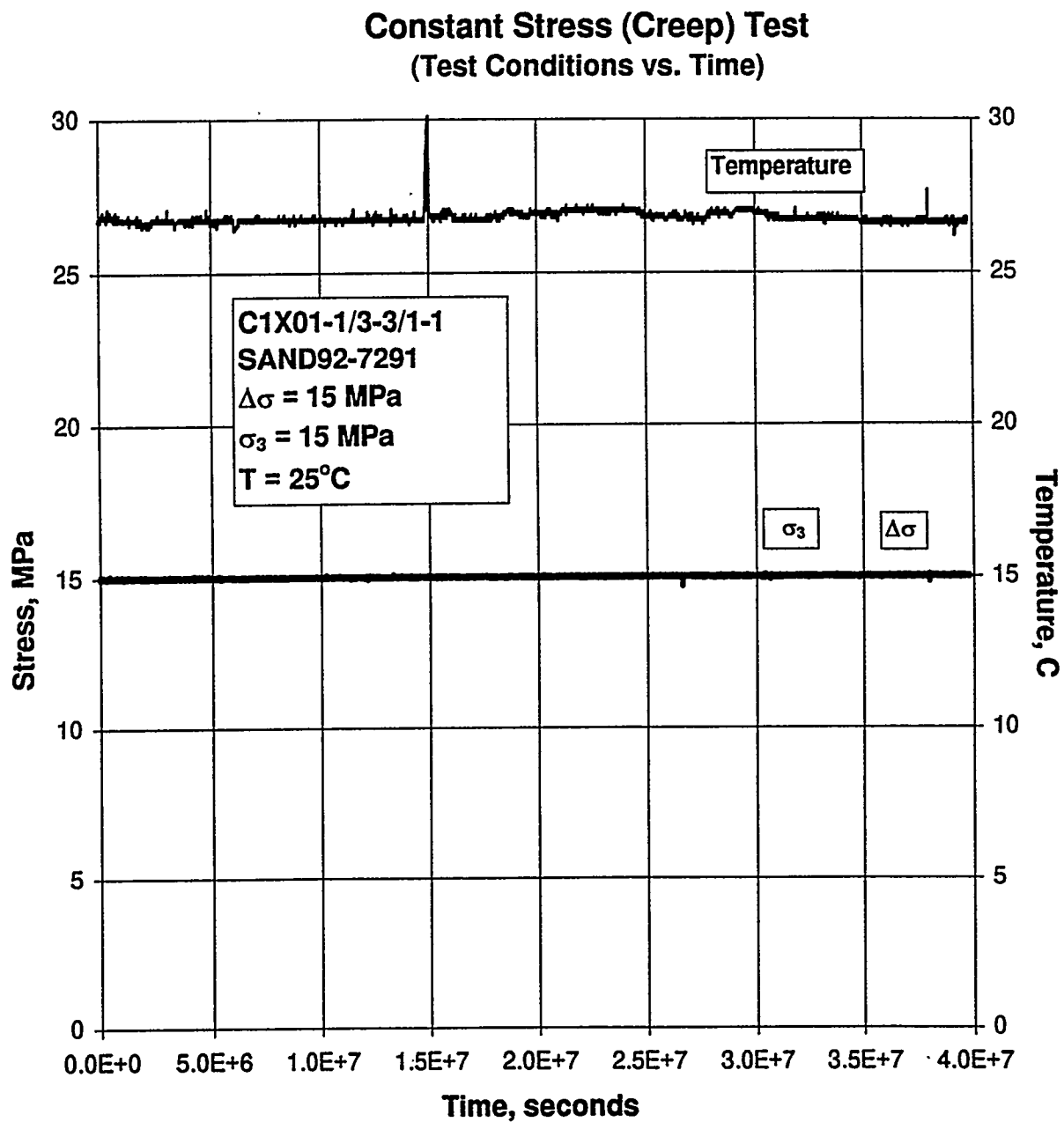
Figure C-3. Test Conditions Versus Time for a Creep Test: Specimen C1X01-1/3-3/1-1; Stage 1 of 1.
