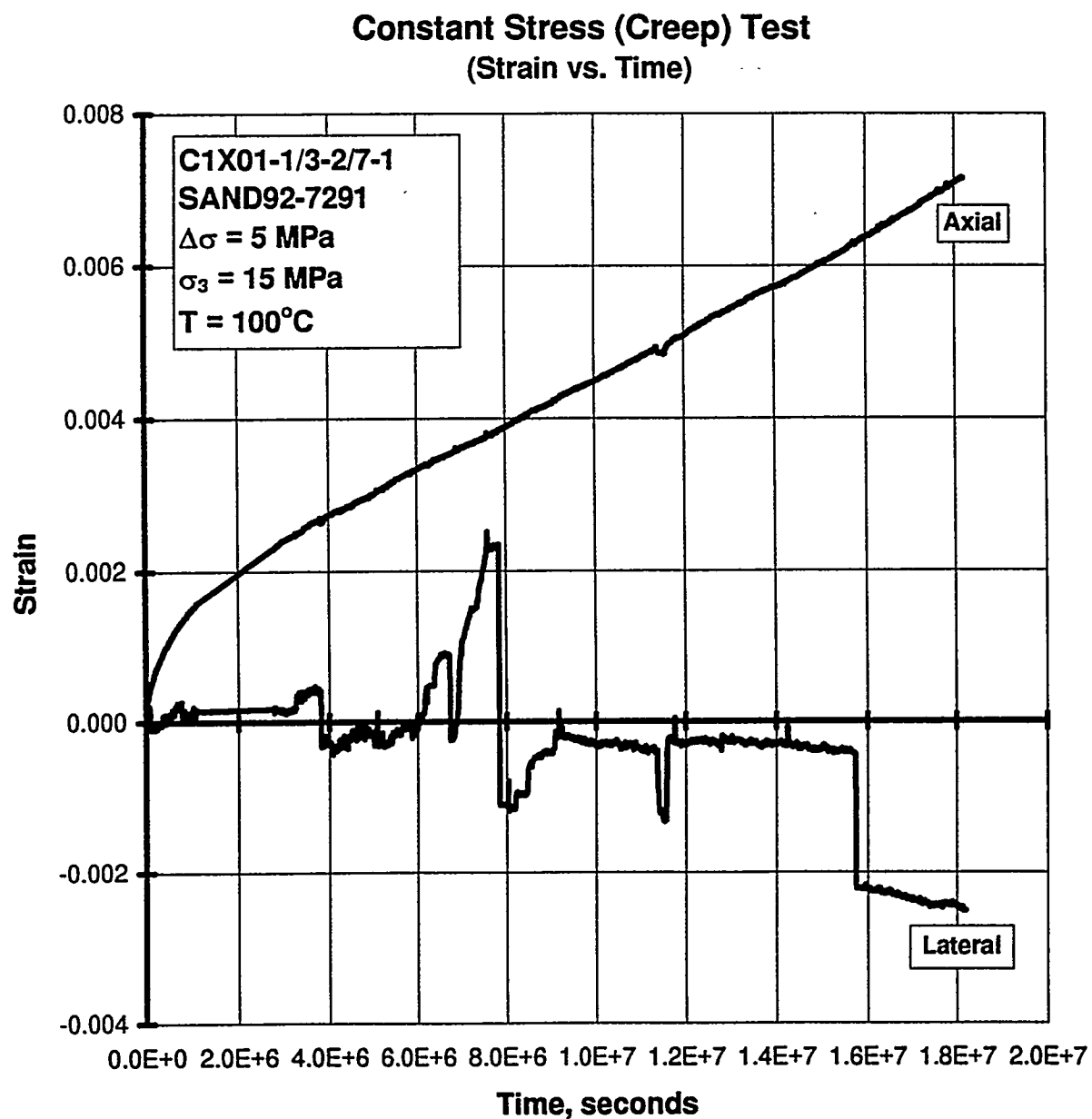
Figure C-12. Axial Strain and Lateral Strain Versus Time for a Creep Test: Specimen C1X01-1/3-2/7-1; Stage 1 of 1.
