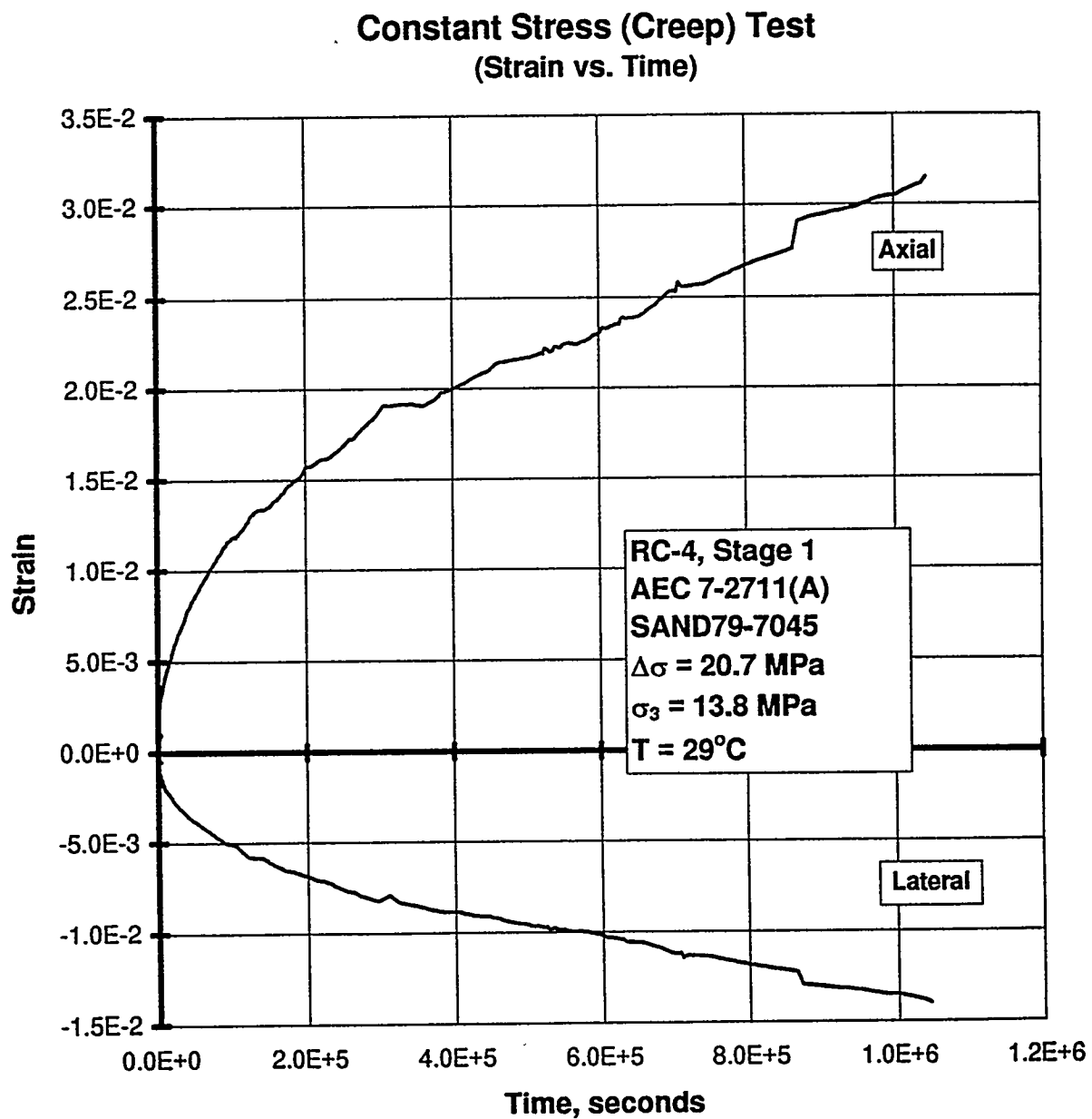
Figure B-178. Axial Strain and Lateral Strain Versus Time for a Creep Test: Specimen AEC7-2711 (A); Stage 1 of 2.
