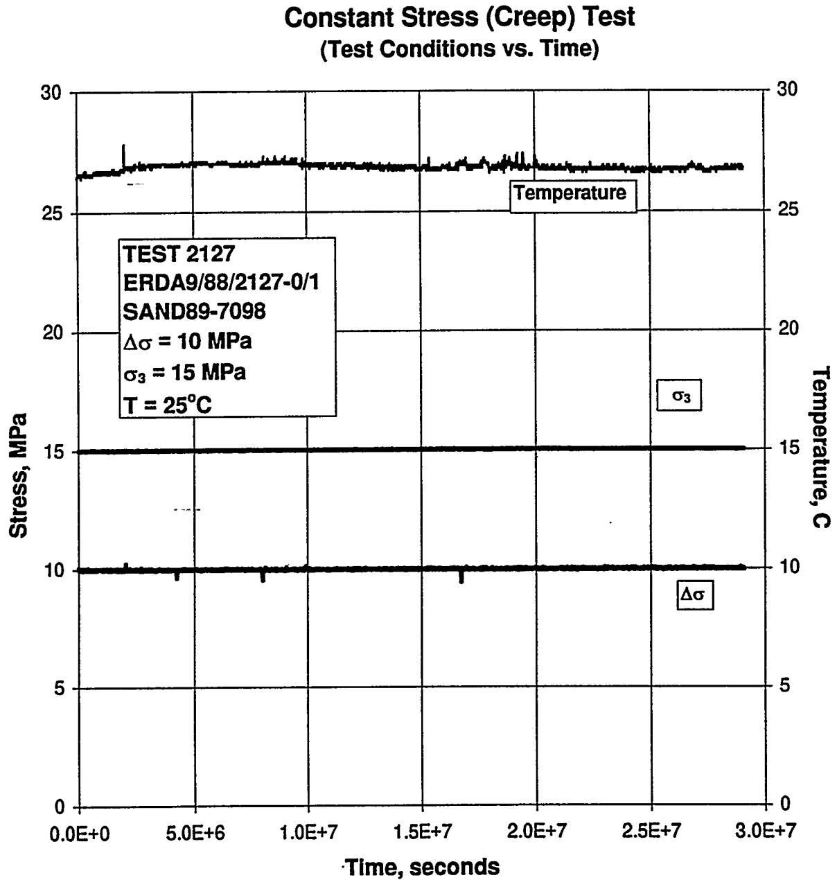
Figure B-1. Test Conditions Versus Time for a Creep Test: Specimen ERDA9/88/2127-0/1; Stage 1 of 1.
