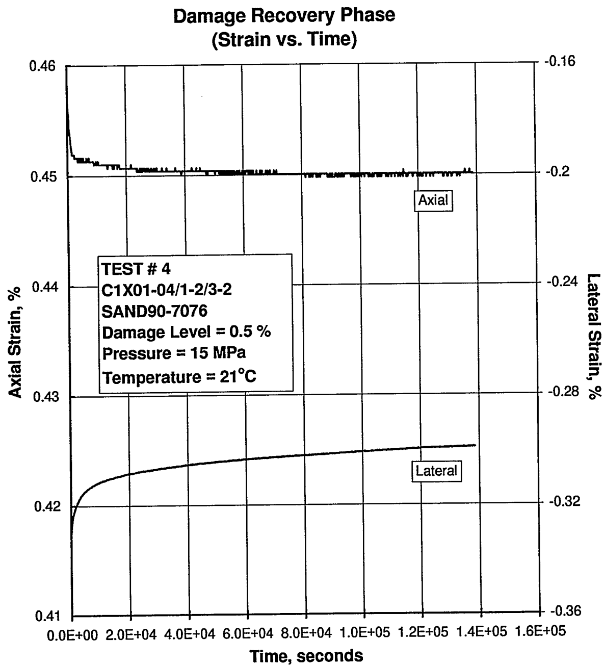
Figure E-78. Axial and Lateral Strain as a Function of Time During the Hydrostatic Loading to Recover Damage in Specimen C1X01-04/1-2/3-2.
