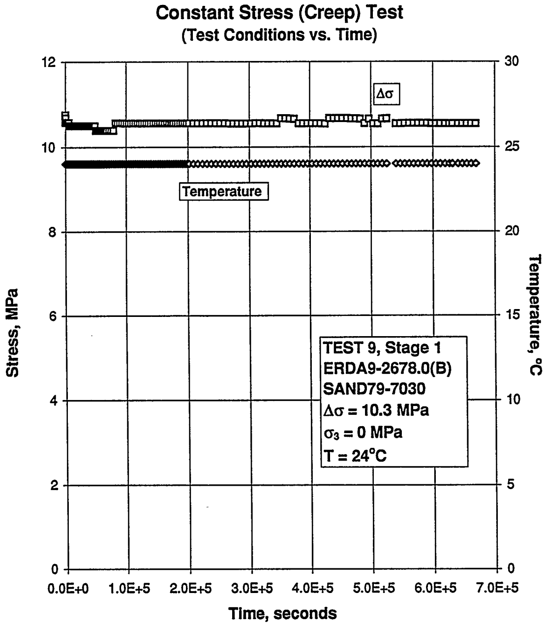
Figure B-107. Test Conditions Versus Time for a Creep Test: Specimen ERDA9-2678.0 (B); Stage 1 of 2.
