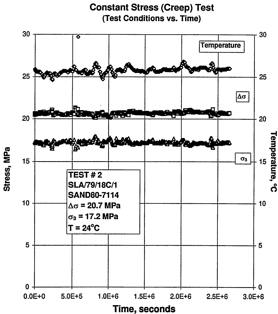
Figure B-20. Test Conditions Versus Time for a Creep Test: Specimen SLA/79/18C/1; Stage 1 of 1.
