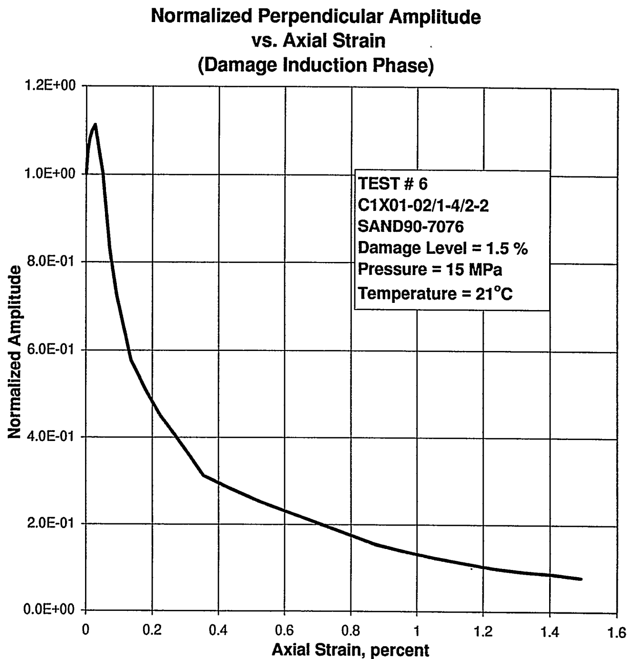
Figure E-97. Normalized Perpendicular Amplitude as a Function of Axial Strain During the Quasi-Static Loading to Induce Damage in Specimen C1X01-02/1-4/2-2.
