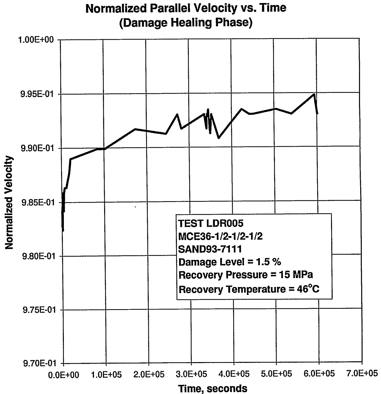
Figure E-28. Normalized Parallel Velocity as a Function of Time During the Hydrostatic Loading to Recover Damage in Specimen MCE36-1/2-1/2-1/2.
