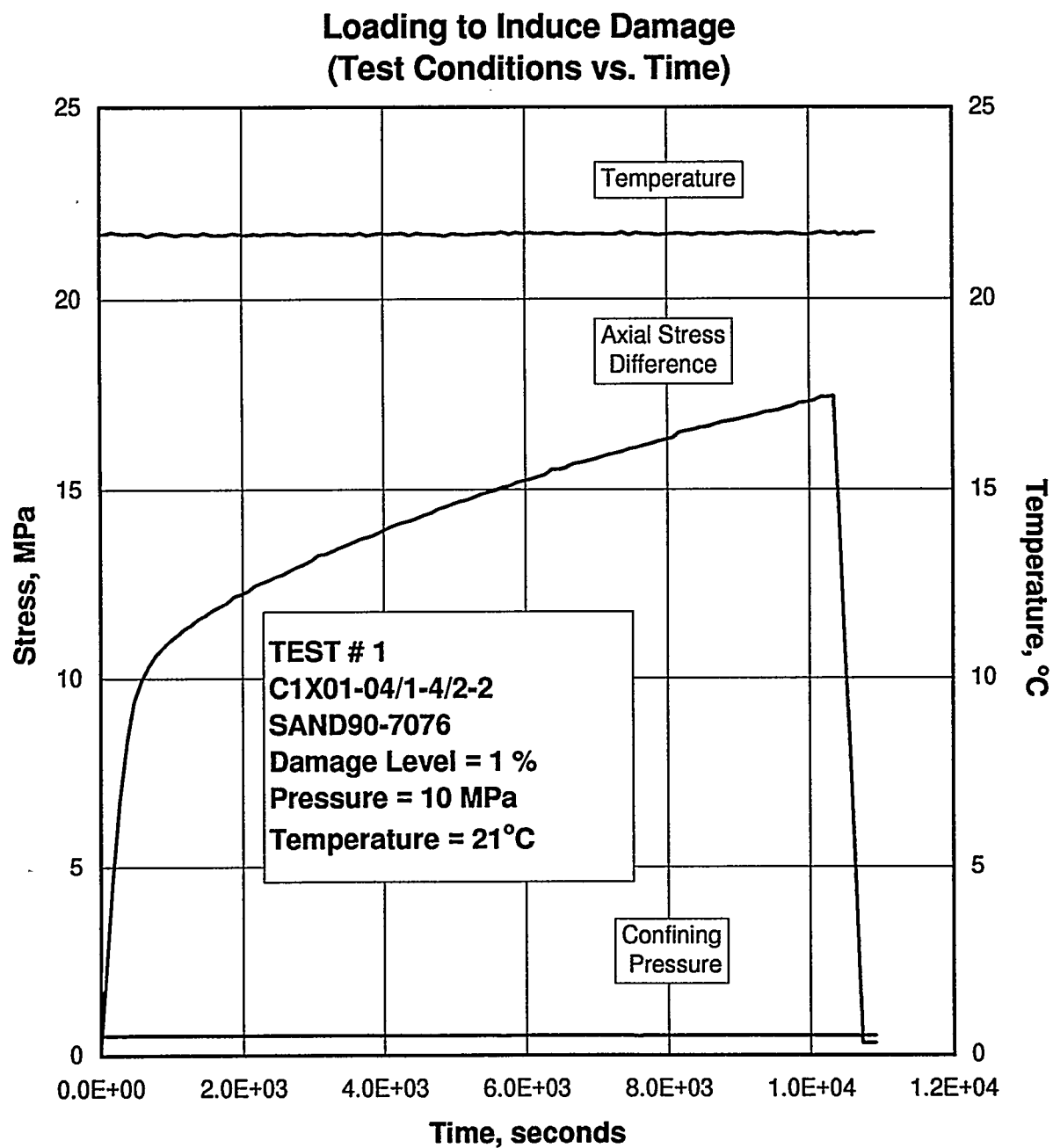
Figure E-35. Test Conditions as a Function of Time During the Quasi-Static Loading to Induce Damage in Specimen C1X01-04/1-4/2-2.
