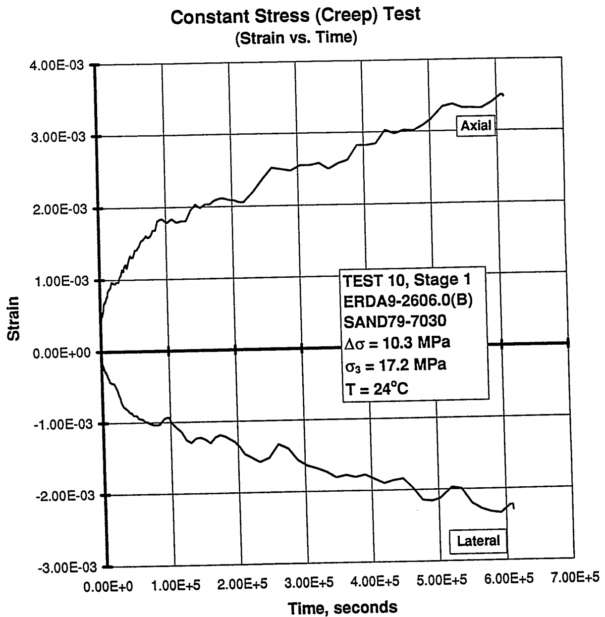
Figure B-116. Axial Strain and Lateral Strain Versus Time for a Creep Test: Specimen ERDA9-2606.0 (B); Stage 1 of 2.
