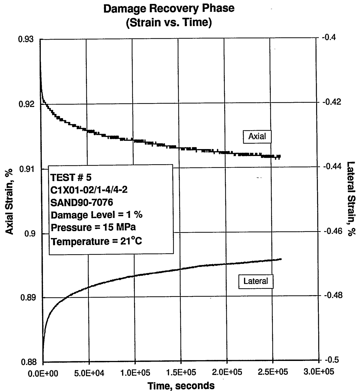
Figure E-90. Axial and Lateral Strain as a Function of Time During the Hydrostatic Loading to Recover Damage in Specimen C1X01-02/1-4/4-2.
