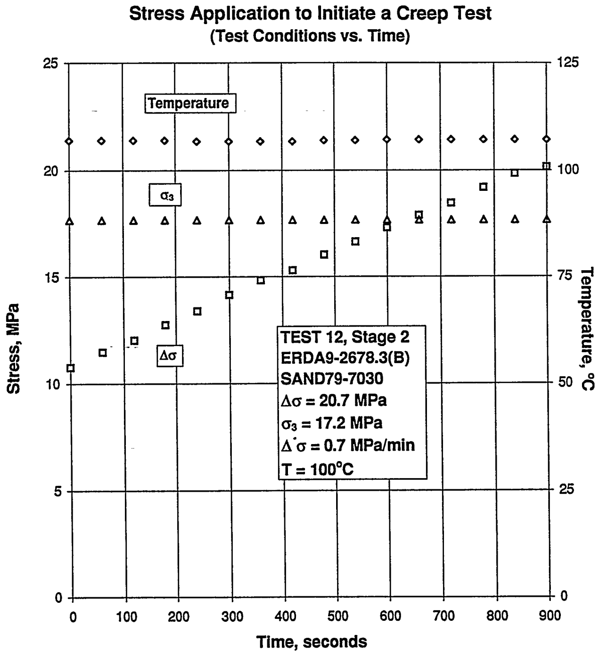
Figure B-131. Test Conditions Versus Time for Stress Application to Initiate a Creep Test: Specimen ERDA9-2678.3 (B); Stage 2 of 2.
