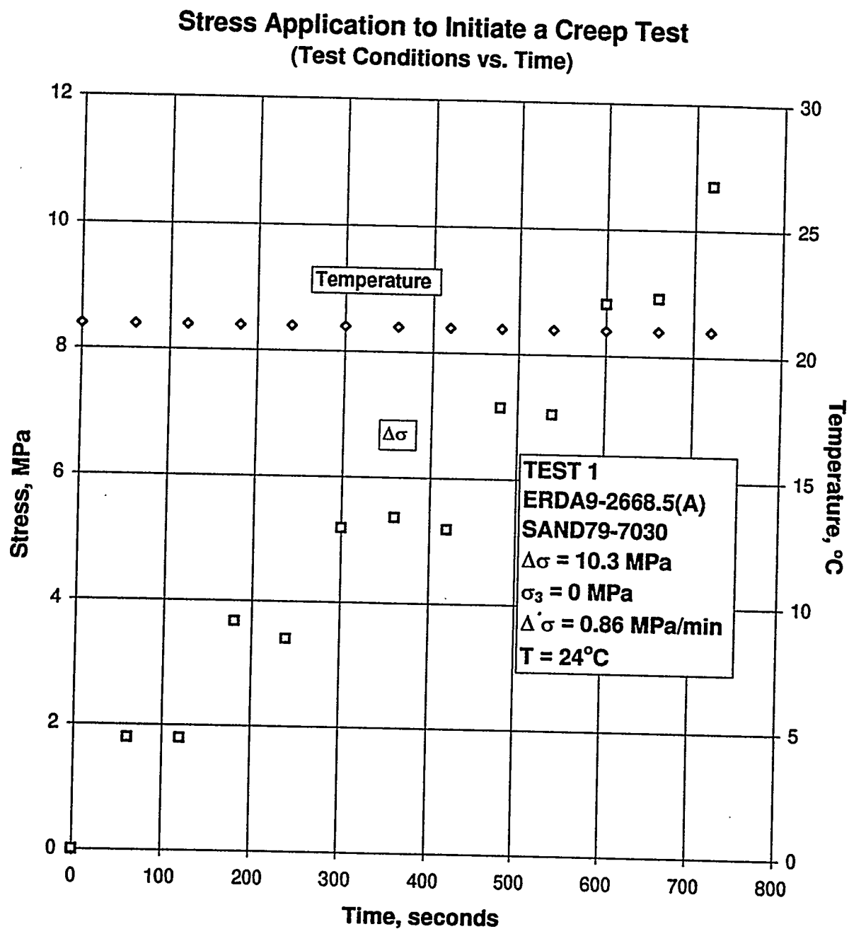
Figure B-73. Test Conditions Versus Time for Stress Application to Initiate a Creep Test: Specimen ERDA9-2668.5 (A); Stage 1 of 1.
