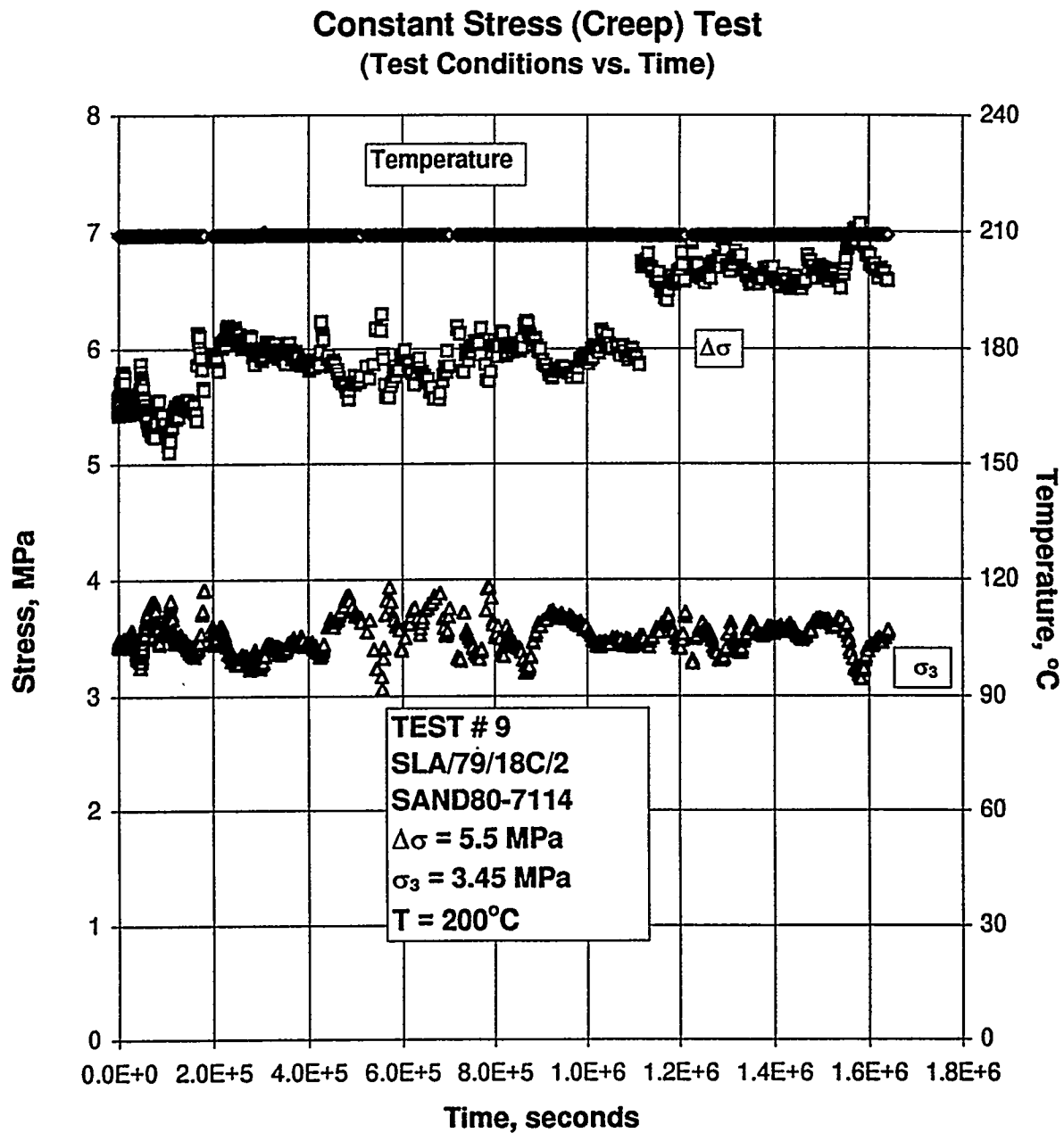
Figure B-55. Test Conditions Versus Time for a Creep Test: Specimen SLA/79/18C/2; Stage 1 of 1.
