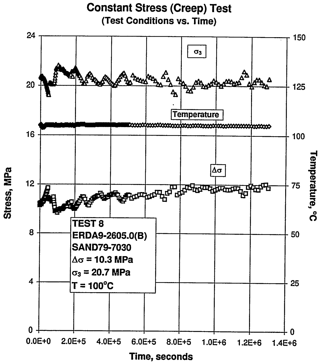
Figure B-103. Test Conditions Versus Time for a Creep Test: Specimen ERDA9-2605.0 (B); Stage 1 of 1.
