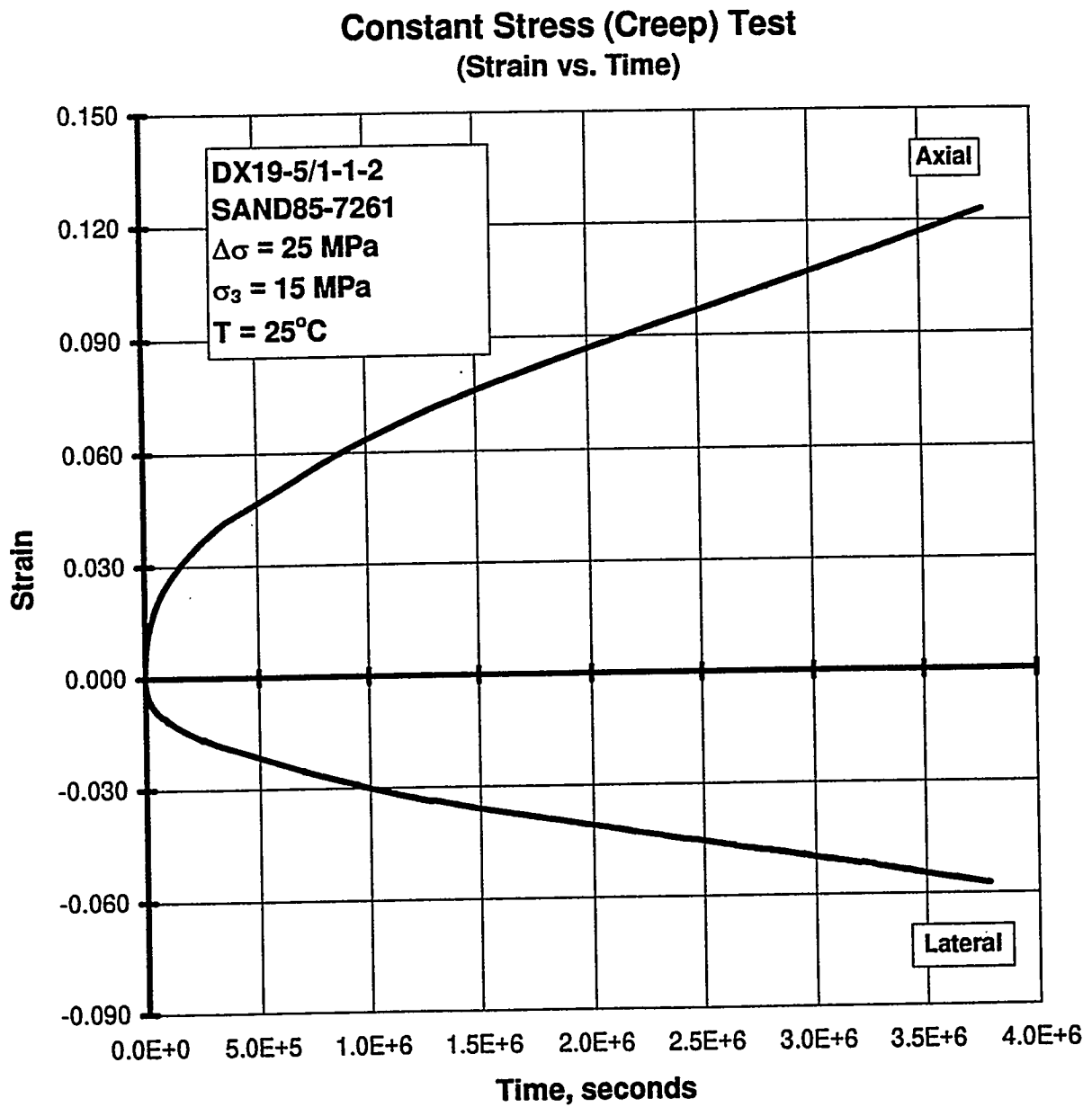
Figure C-72. Axial Strain and Lateral Strain Versus Time for a Creep Test: Specimen DX19-5/1-1-2; Stage 1 of 1.
