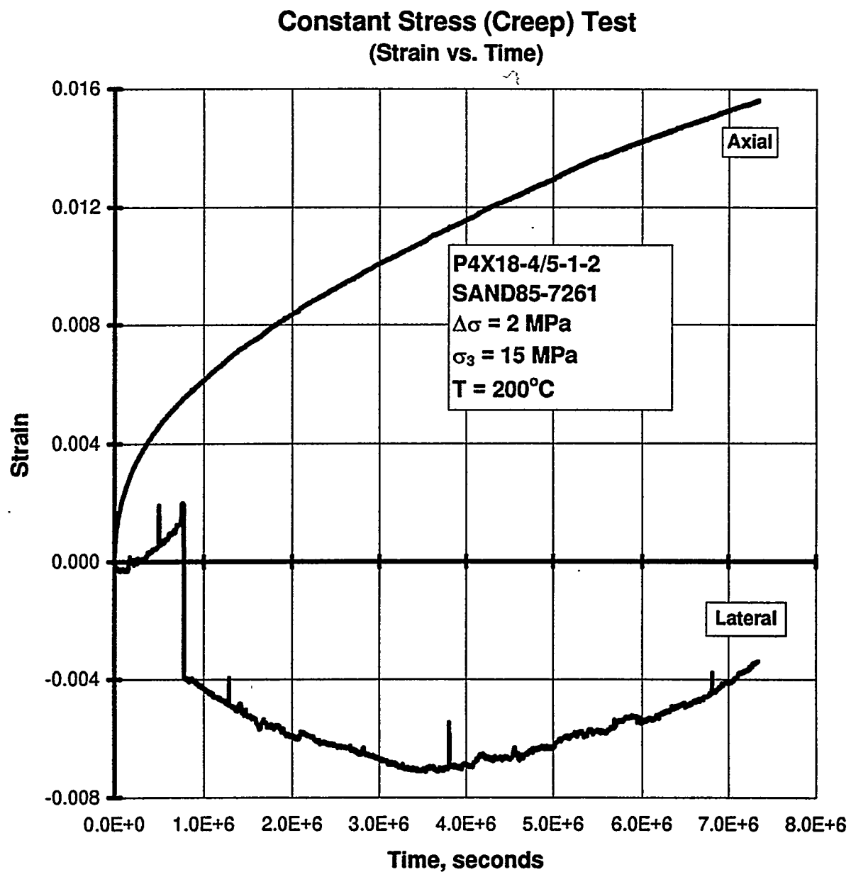
Figure C-52. Axial Strain and Lateral Strain Versus Time for a Creep Test: Specimen P4X18-4/5-1-2; Stage 1 of 1 (Argillaceous Salt).
