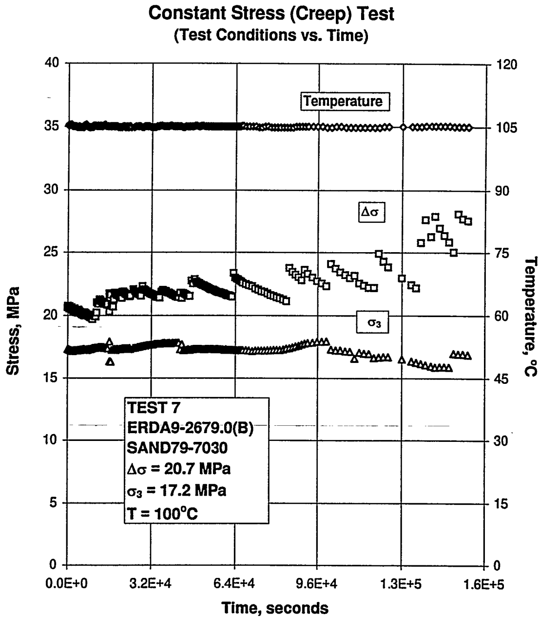
Figure B-99. Test Conditions Versus Time for a Creep Test: Specimen ERDA9-2679.0 (B); Stage 1 of 1 (Specimen Contacted Vessel Wall at End of Test).
