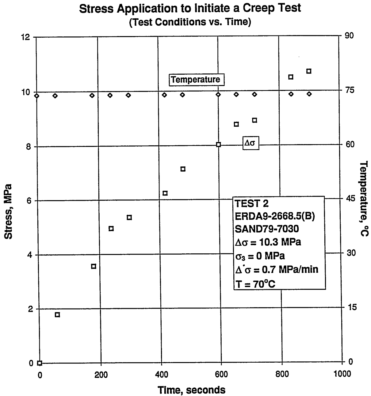
Figure B-77. Test Conditions Versus Time for Stress Application to Initiate a Creep Test: Specimen ERDA9-2668.5 (B); Stage 1 of 1.
