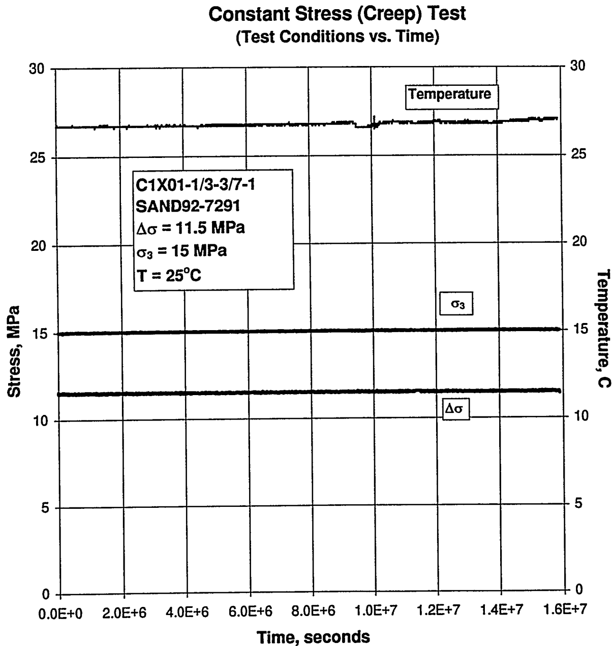
Figure C-1. Test Conditions Versus Time for a Creep Test: Specimen C1X01-1/3-3/7-1; Stage 1 of 1.
