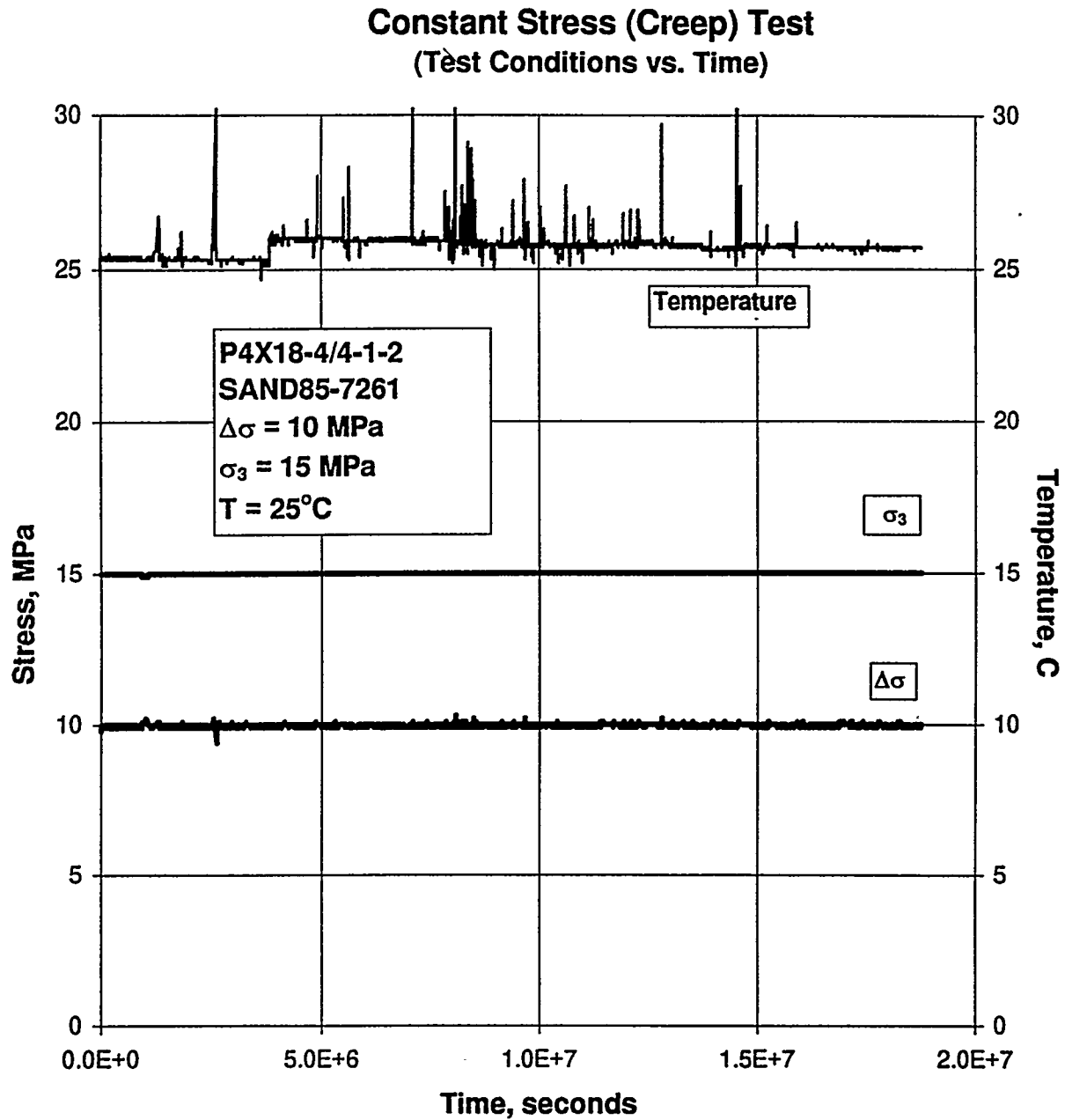
Figure C-37. Test Conditions Versus Time for a Creep Test: Specimen P4X18-4/4-1-2; Stage 1 of 1 (Argillaceous Salt).
