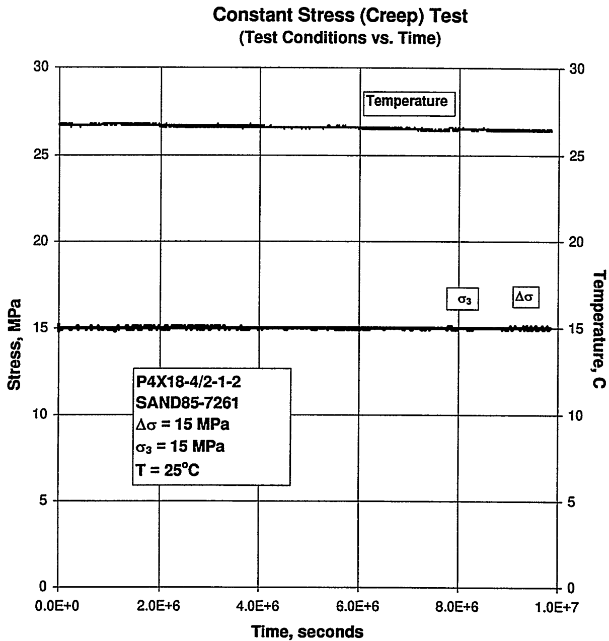
Figure C-43. Test Conditions Versus Time for a Creep Test: Specimen P4X18-4/2-1-2; Stage 1 of 1 (Argillaceous Salt).
