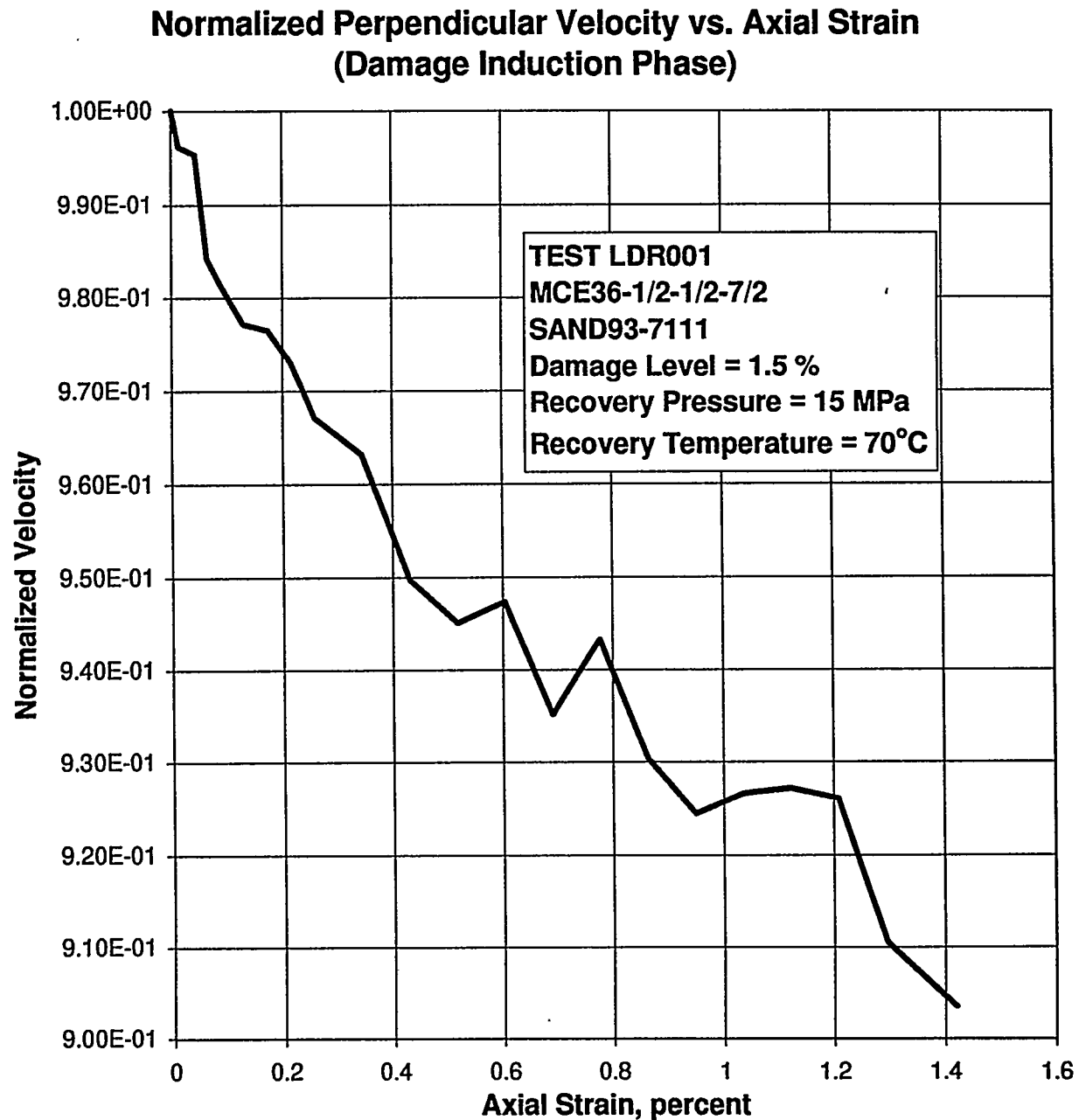
Figure E-5. Normalized Perpendicular Velocity as a Function of Axial Strain During the Quasi-Static Loading to Induce Damage in Specimen MCE36-1/2-1/2-7/2.
