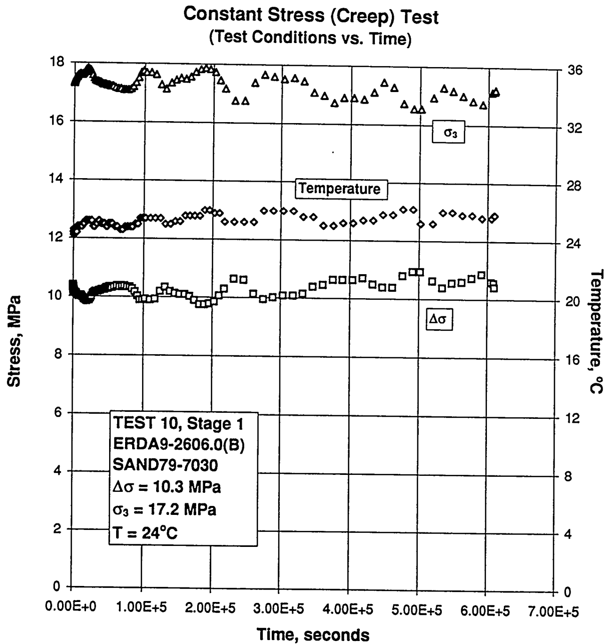
Figure B-115. Test Conditions Versus Time for a Creep Test: Specimen ERDA9-2606.0 (B); Stage 1 of 2.
