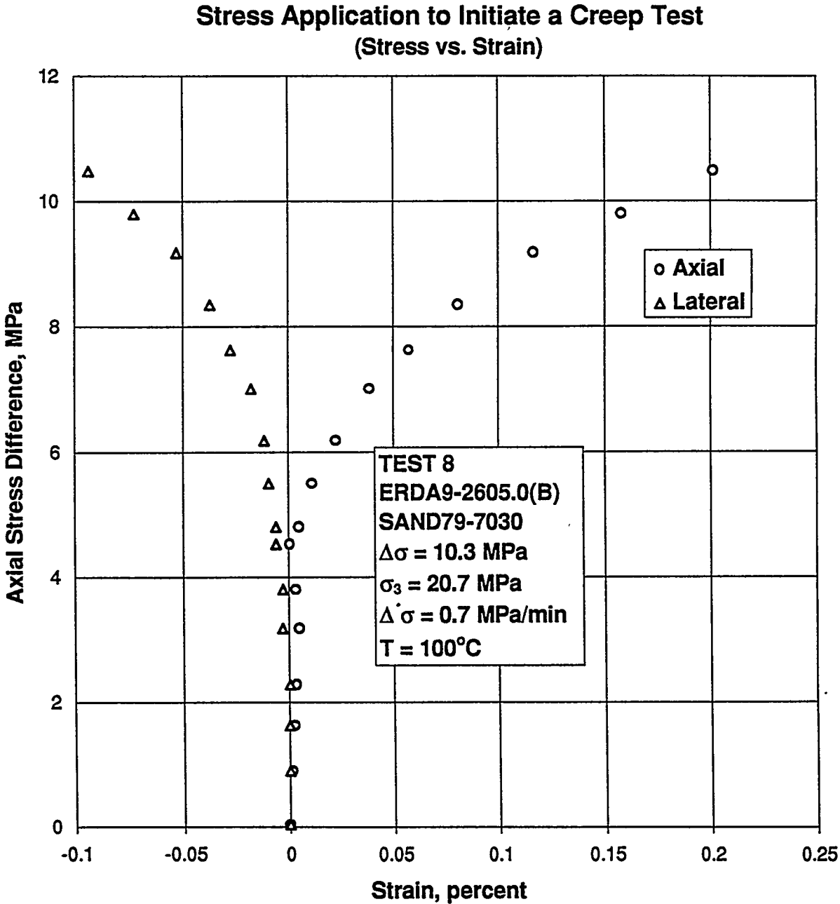
Figure B-102. Axial Stress Difference Versus Axial and Lateral Strain for Stress Application to Initiate a Creep Test: Specimen ERDA9-2605.0 (B); Stage 1 of 1.
