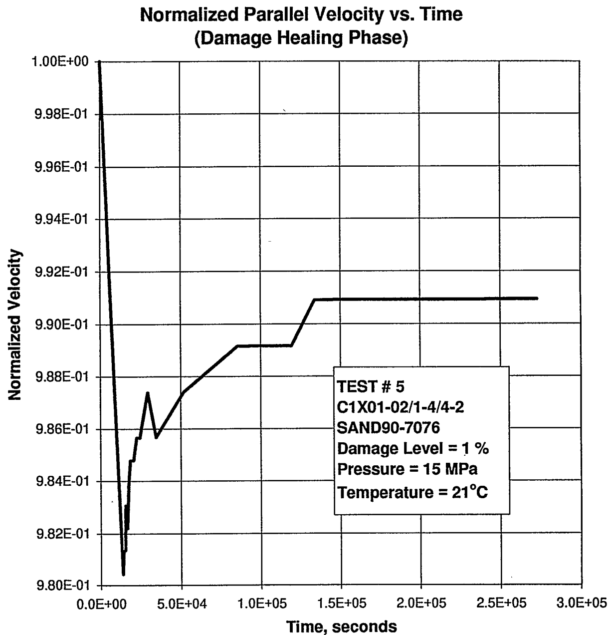
Figure E-94. Normalized Parallel Velocity as a Function of Time During the Hydrostatic Loading to Recover Damage in Specimen C1X01-02/1-4/4-2.
