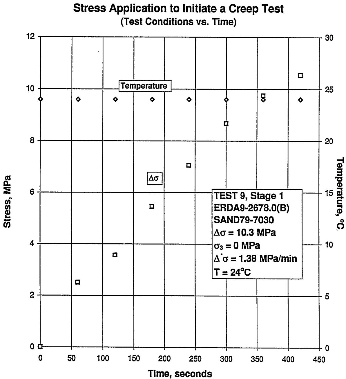
Figure B-105. Test Conditions Versus Time for Stress Application to Initiate a Creep Test: Specimen ERDA9-2678.0 (B); Stage 1 of 2.
