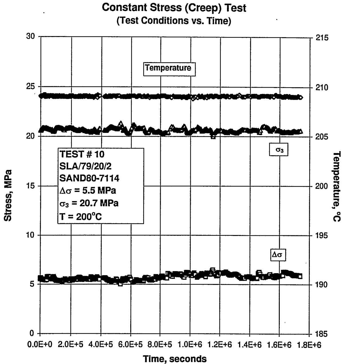
Figure B-59. Test Conditions Versus Time for a Creep Test: Specimen SLA/79/20/2; Stage 1 of 1.
