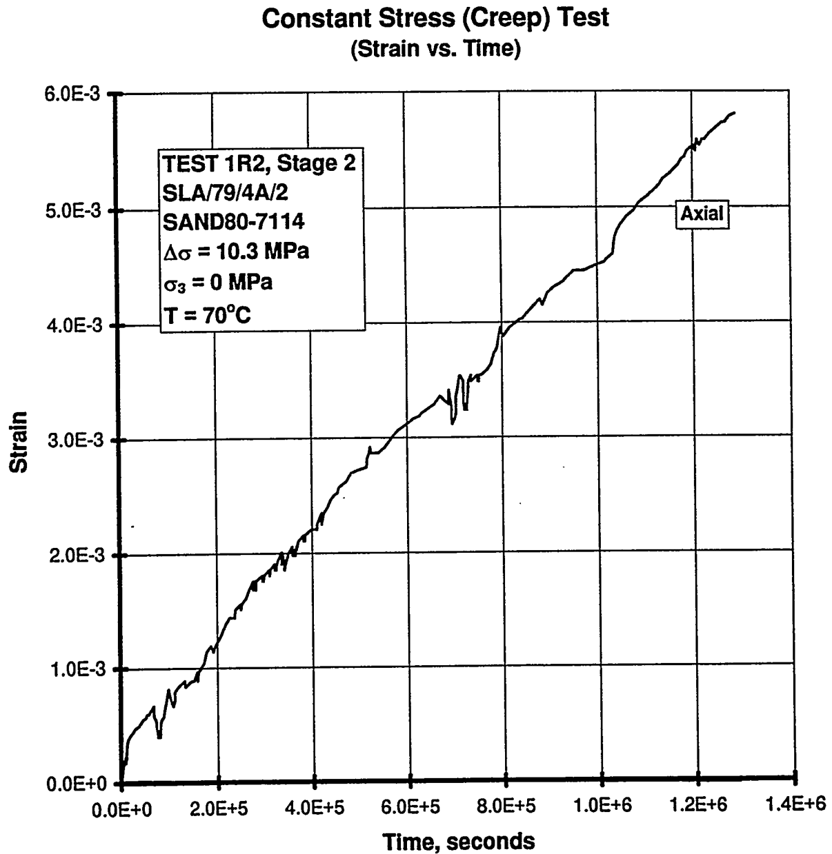
Figure B-17. Axial Strain and Lateral Strain Versus Time for a Creep Test: Specimen SLA/79/4A/2; Stage 2 of 2.
