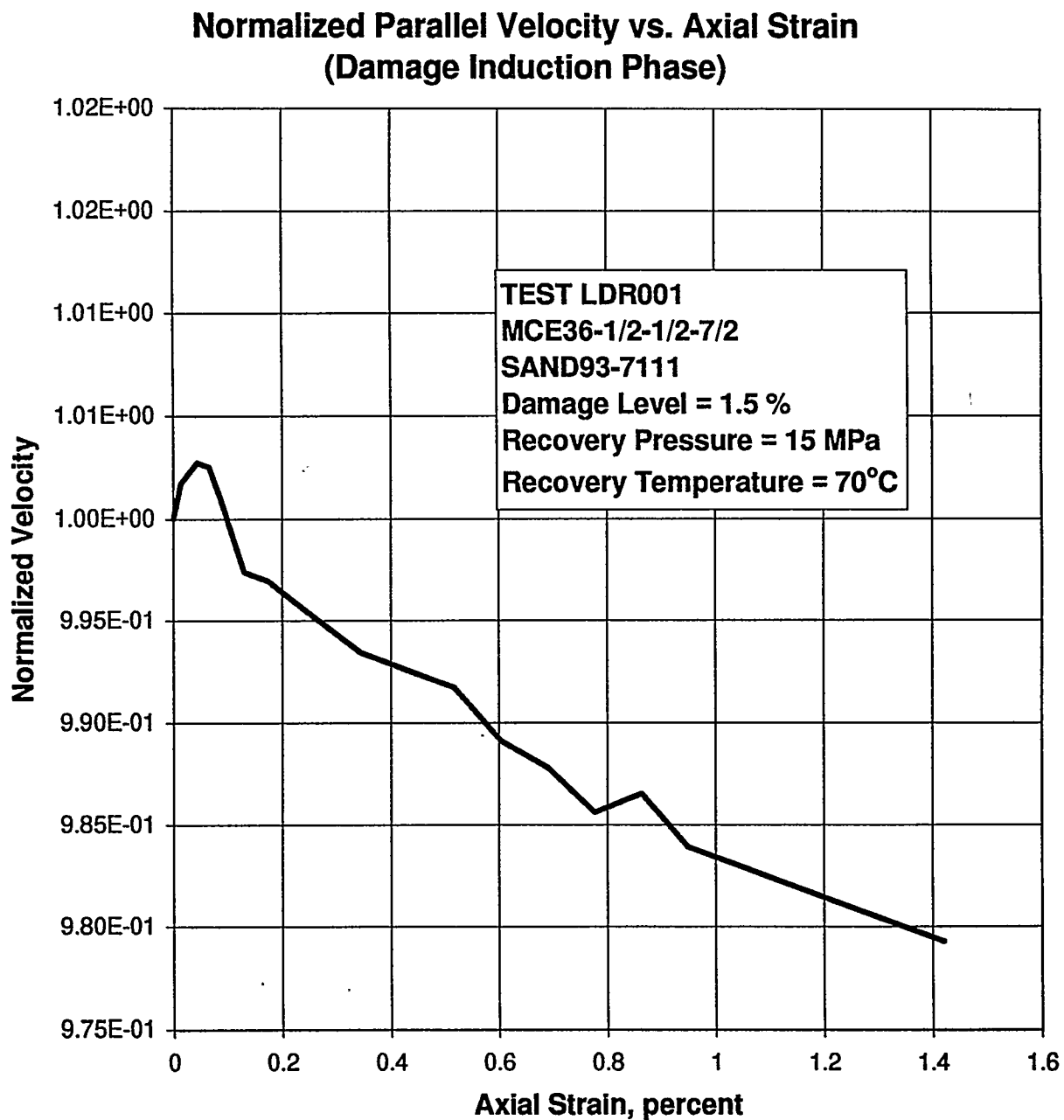
Figure E-6. Normalized Parallel Velocity as a Function of Axial Strain During the Quasi-Static Loading to Induce Damage in Specimen MCE36-1/2-1/2-7/2.
