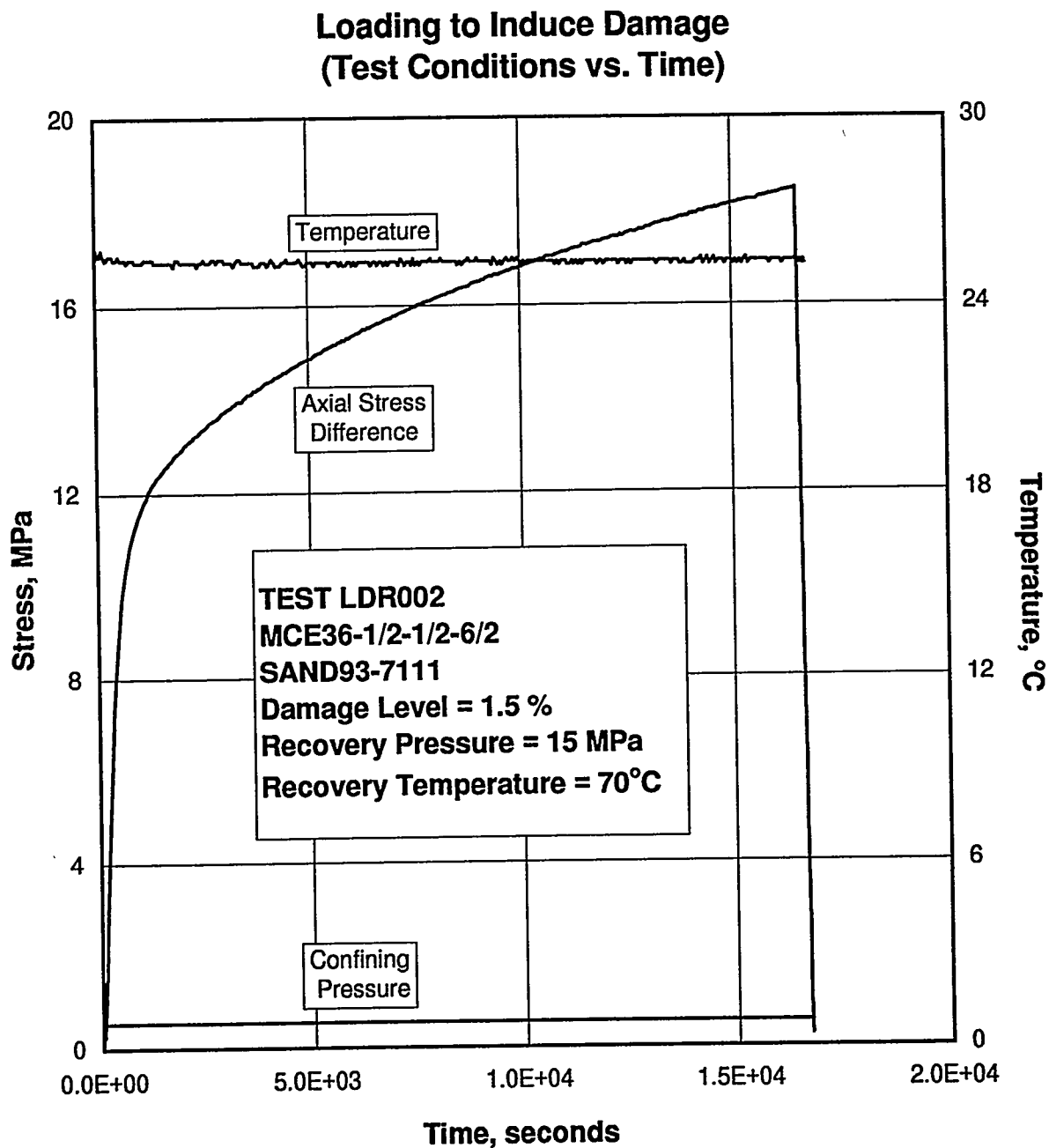
Figure E-7. Test Conditions as a Function of Time During the Quasi-Static Loading to Induce Damage in Specimen MCE36-1/2-1/2-6/2.
