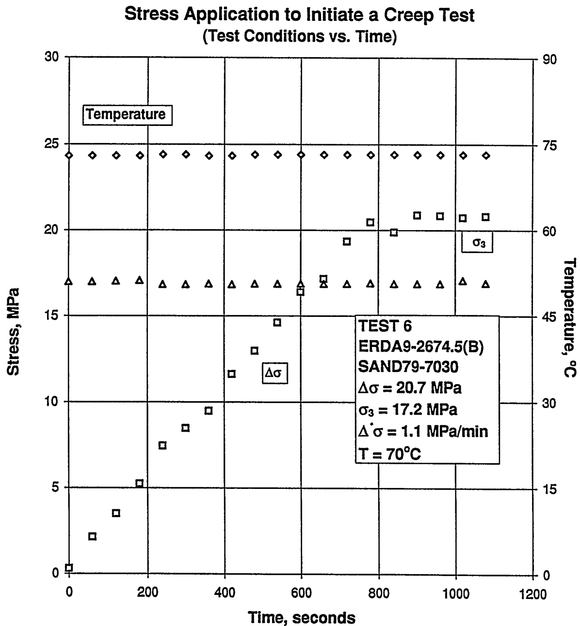
Figure B-93. Test Conditions Versus Time for Stress Application to Initiate a Creep Test: Specimen ERDA9-2674.5 (B); Stage 1 of 1.
