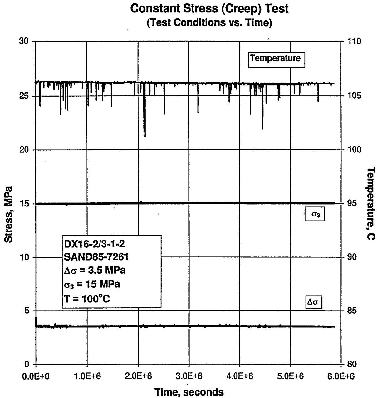
Figure C-77. Test Conditions Versus Time for a Creep Test: Specimen DX16-2/3-1-2; Stage 1 of 1.
