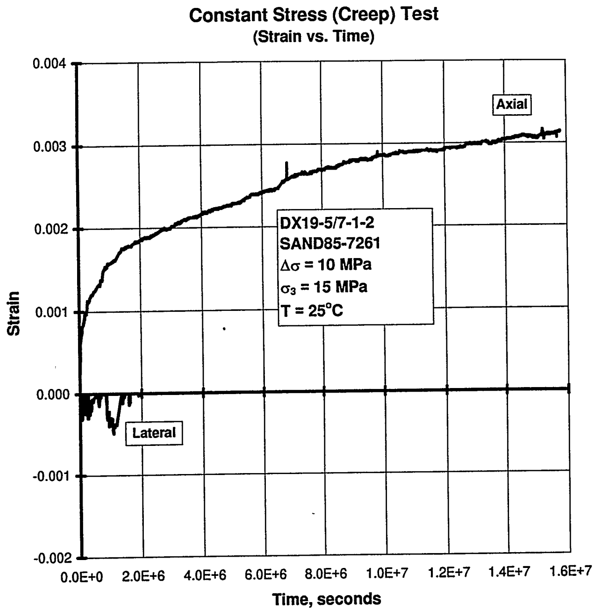
Figure C-58. Axial Strain and Lateral Strain Versus Time for a Creep Test: Specimen DX19-5/7-1-2; Stage 1 of 1.
