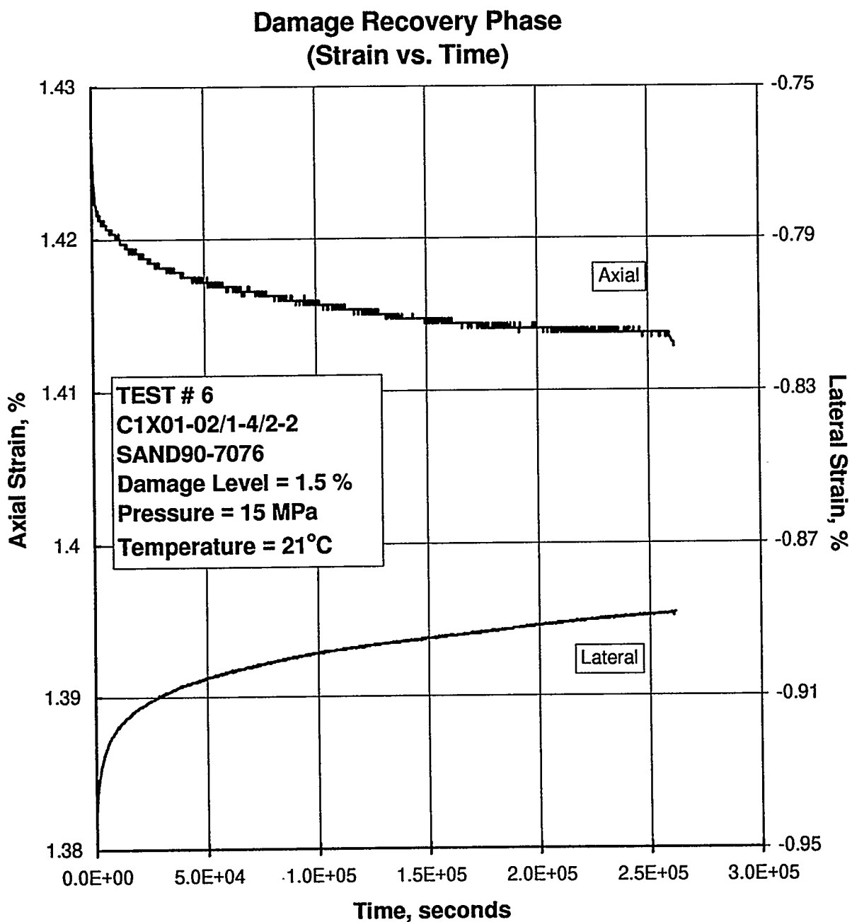
Figure E-102. Axial and Lateral Strain as a Function of Time During the Hydrostatic Loading to Recover Damage in Specimen C1X01-02/1-4/2-2.
