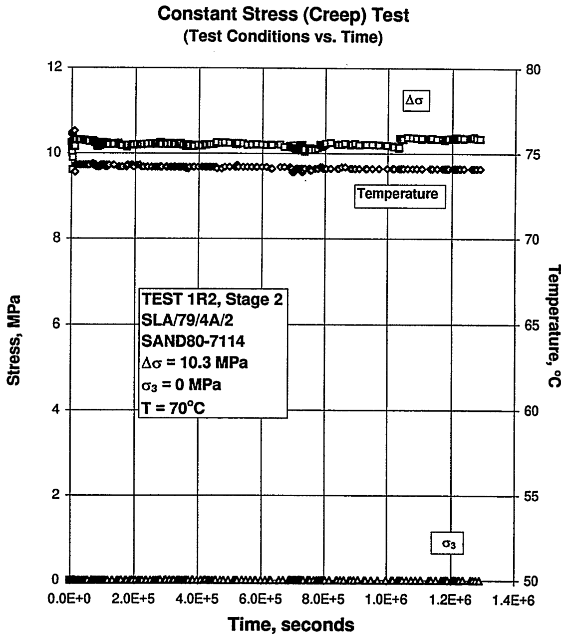
Figure B-16. Test Conditions Versus Time for a Creep Test: Specimen SLA/79/4A/2; Stage 2 of 2.
