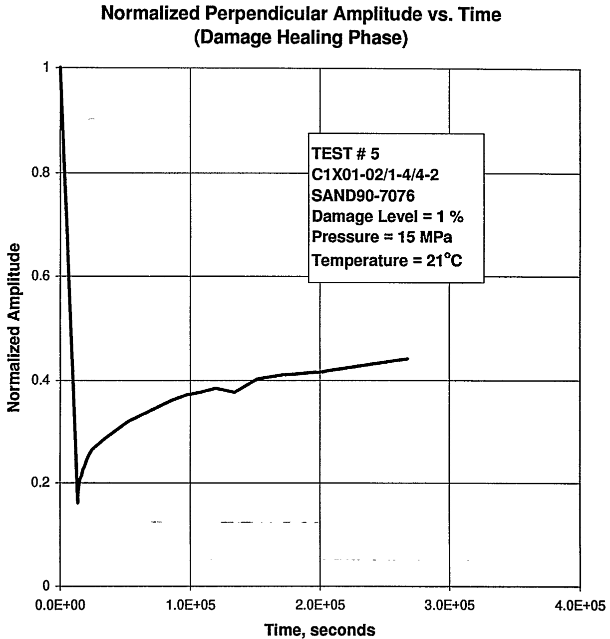
Figure E-91. Normalized Perpendicular Amplitude as a Function of Time During the Hydrostatic Loading to Recover Damage in Specimen C1X01-02/1-4/4-2.
