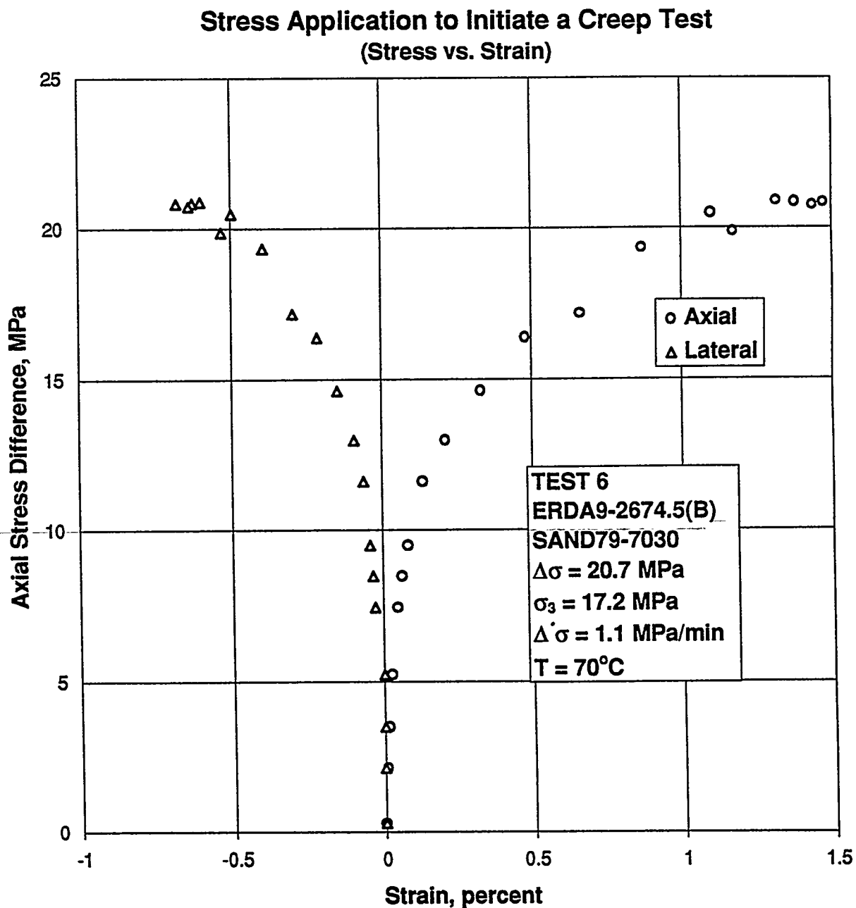
Figure B-94. Axial Stress Difference Versus Axial and Lateral Strain for Stress Application to Initiate a Creep Test: Specimen ERDA9-2674.5 (B); Stage 1 of 1.
