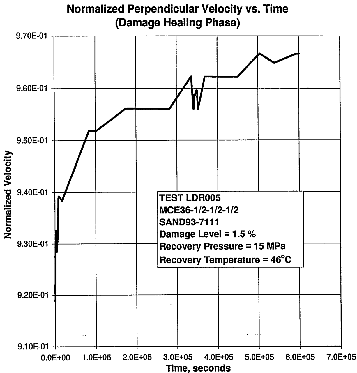
Figure E-27. Normalized Perpendicular Velocity as a Function of Time During the Hydrostatic Loading to Recover Damage in Specimen MCE36-1/2-1/2-1/2.
