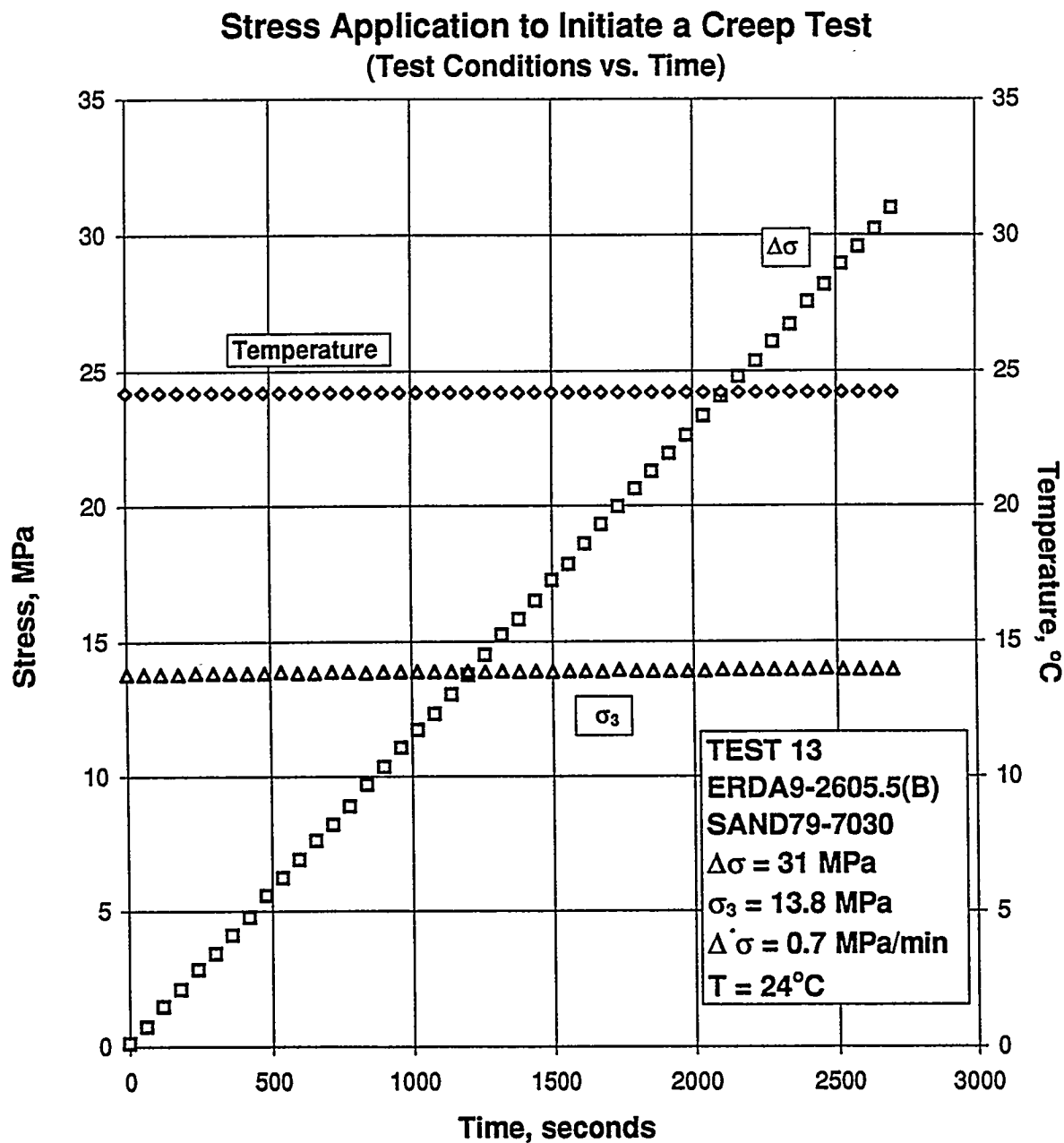
Figure B-135. Test Conditions Versus Time for Stress Application to Initiate a Creep Test: Specimen ERDA9-2605.5 (B); Stage 1 of 1.
