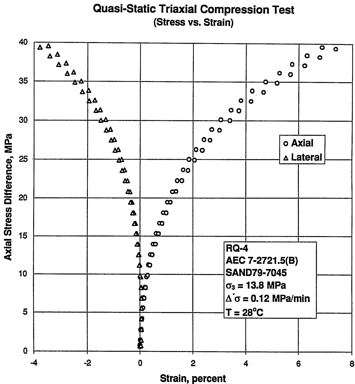
Figure A-8. Axial Stress Difference Versus Axial and Lateral Strain for a Quasi-Static Triaxial Compression Test: Specimen AEC7-2721.5 (B).
