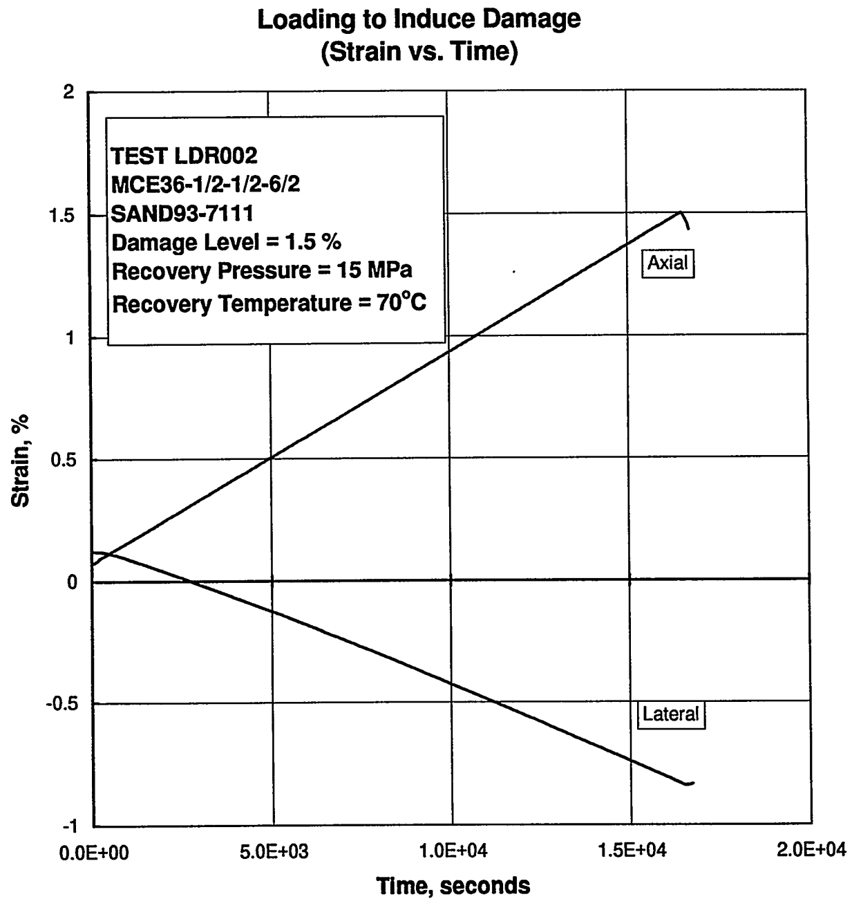
Figure E-8. Axial and Lateral Strain as a Function of Time During the Quasi-Static Loading to Induce Damage in Specimen MCE36-1/2-1/2-6/2.
