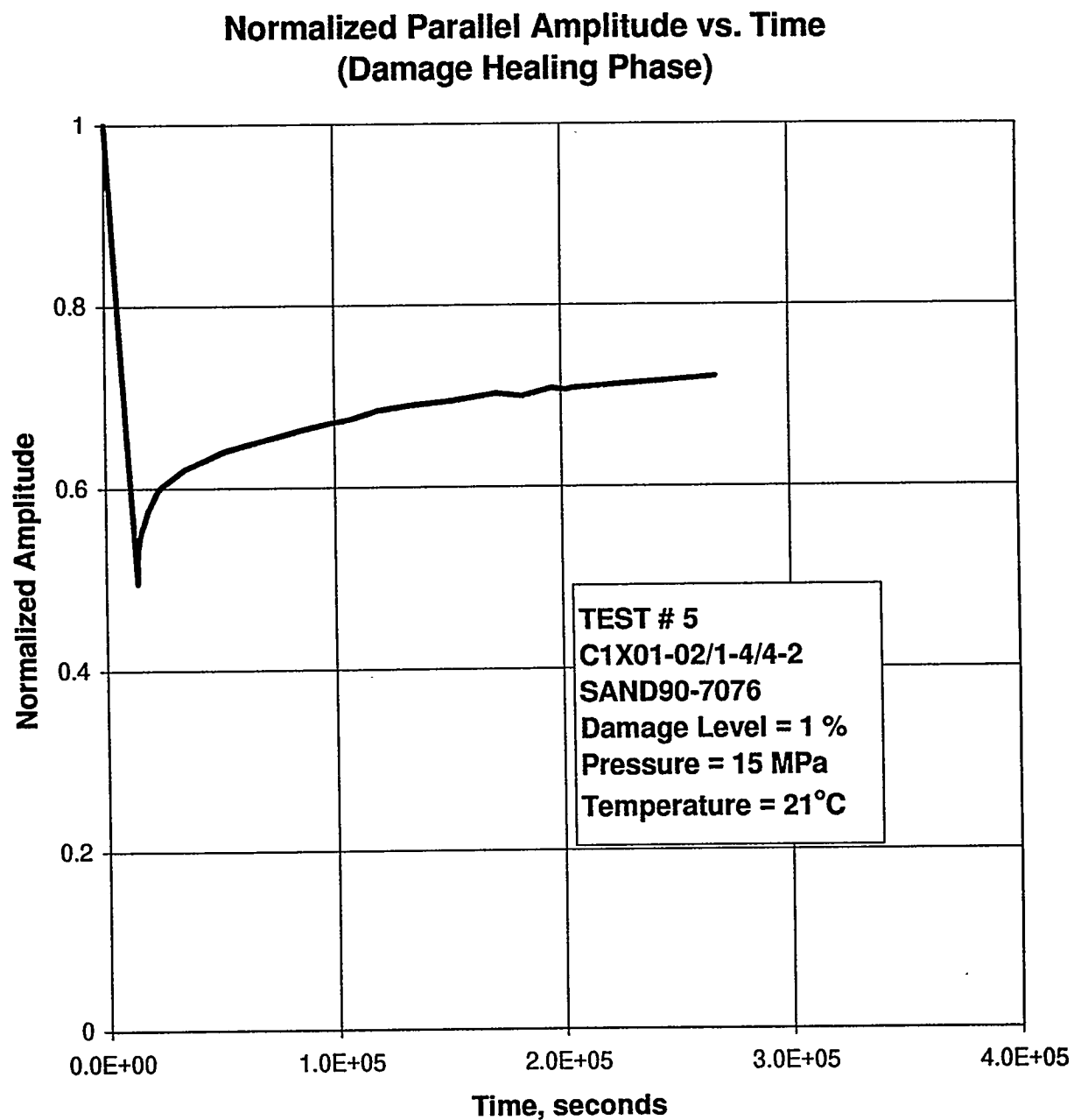
Figure E-92. Normalized Parallel Amplitude as a Function of Time During the Hydrostatic Loading to Recover Damage in Specimen C1X01-02/1-4/4-2.
