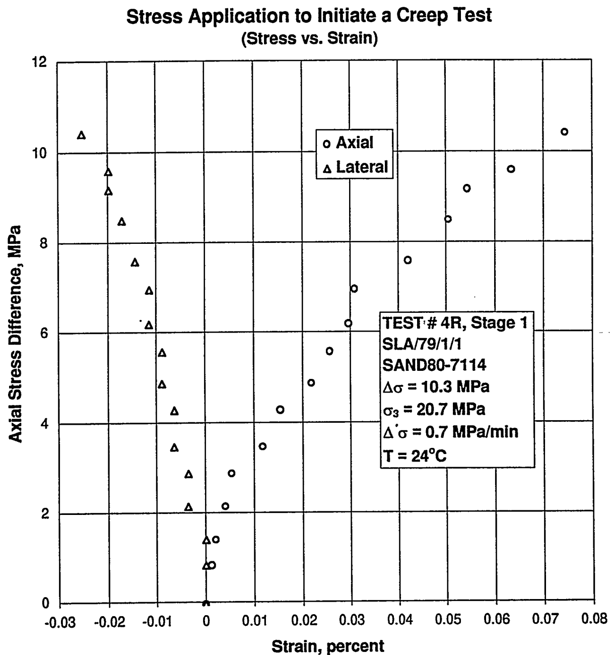
Figure B-31. Axial Stress Difference Versus Axial and Lateral Strain for Stress Application to Initiate a Creep Test: Specimen SLA/79/1/1; Stage 1 of 2.
