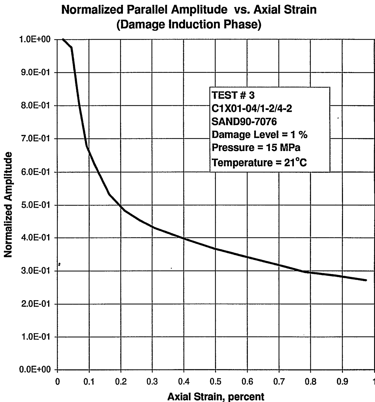
Figure E-62. Normalized Parallel Amplitude as a Function of Axial Strain During the Quasi-Static Loading to Induce Damage in Specimen C1X01-04/1-2/4-2.
