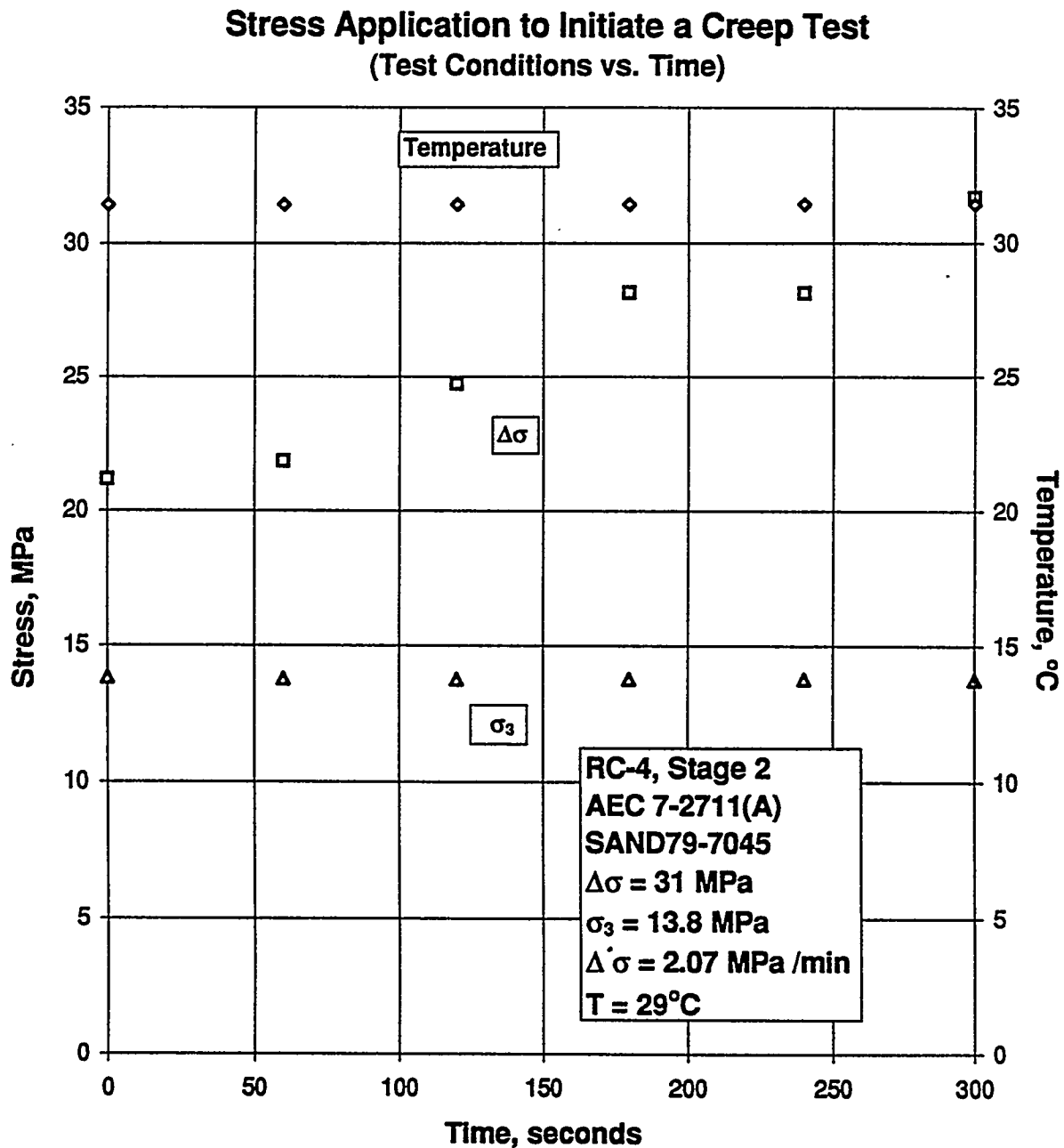
Figure B-179. Test Conditions Versus Time for Stress Application to Initiate a Creep Test: Specimen AEC7-2711 (A); Stage 2 of 2.
