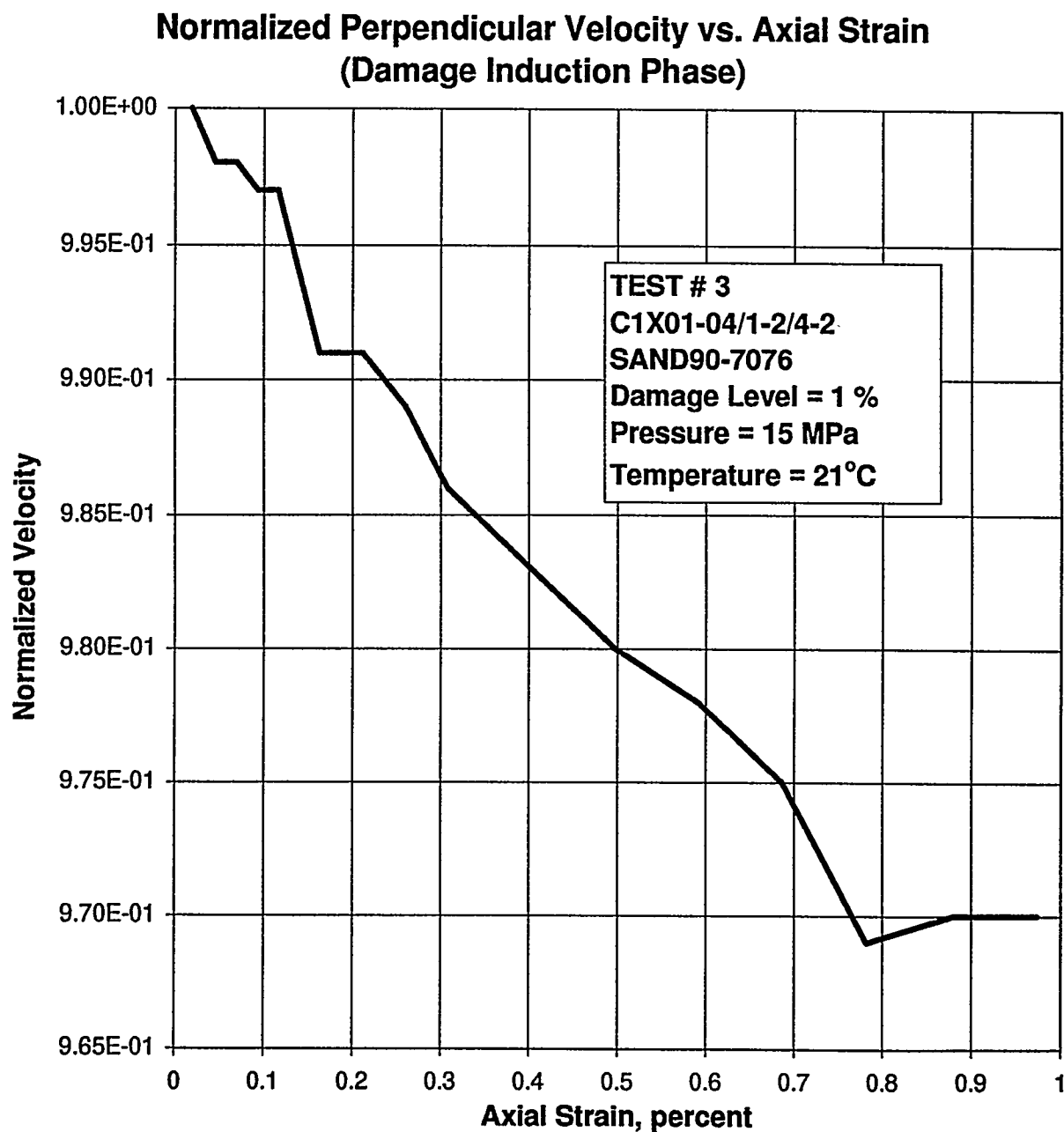
Figure E-63. Normalized Perpendicular Velocity as a Function of Axial Strain During the Quasi-Static Loading to Induce Damage in Specimen C1X01-04/1-2/4-2.
