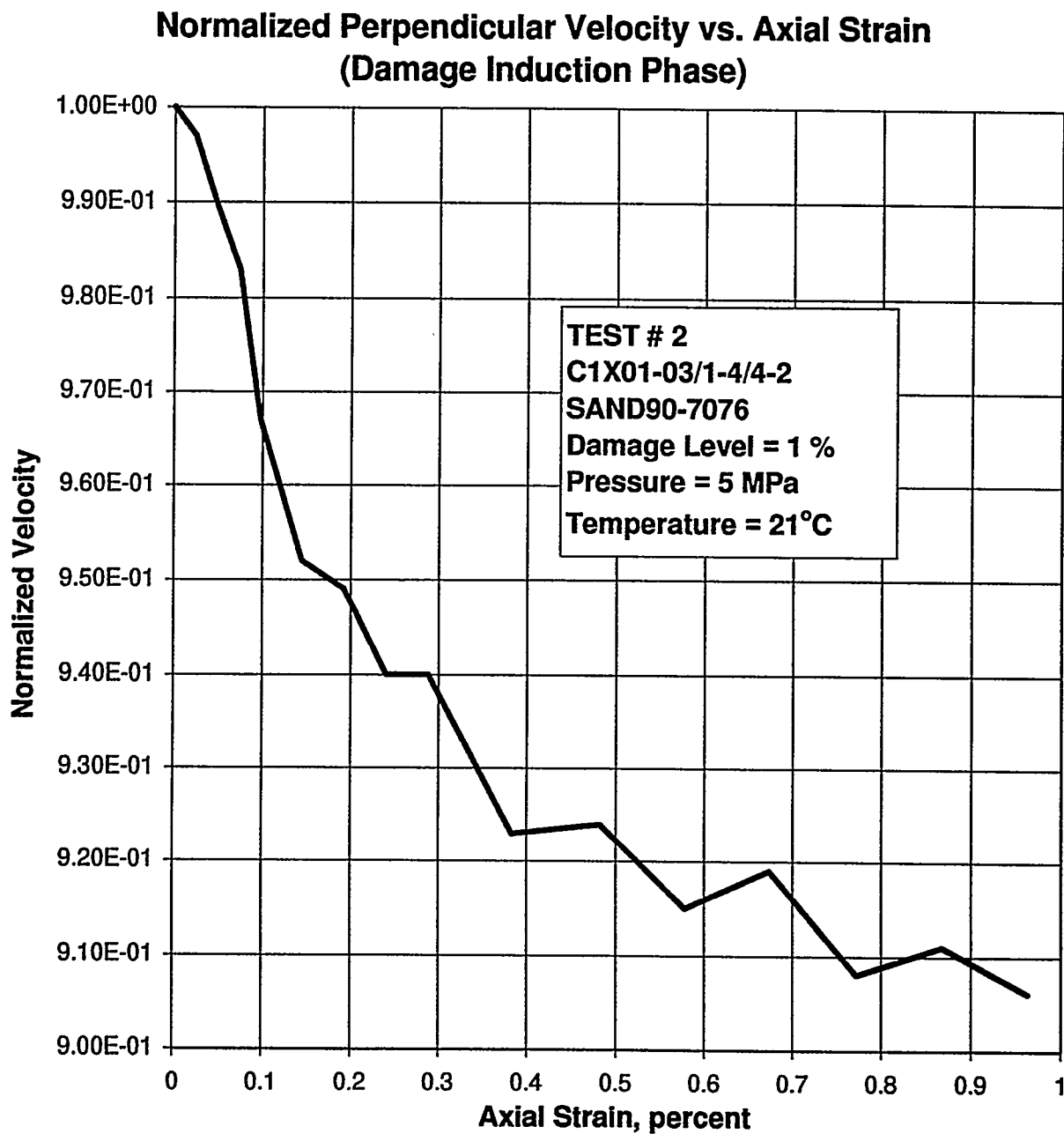
Figure E-51. Normalized Perpendicular Velocity as a Function of Axial Strain During the Quasi-Static Loading to Induce Damage in Specimen C1X01-03/1-4/4-2.
