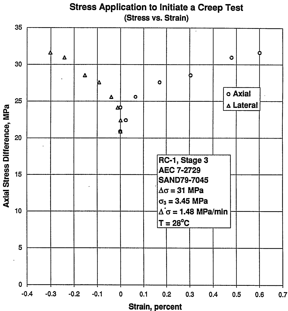
Figure B-152. Axial Stress Difference Versus Axial and Lateral Strain for Stress Application to Initiate a Creep Test: Specimen AEC7-2729; Stage 3 of 3.
