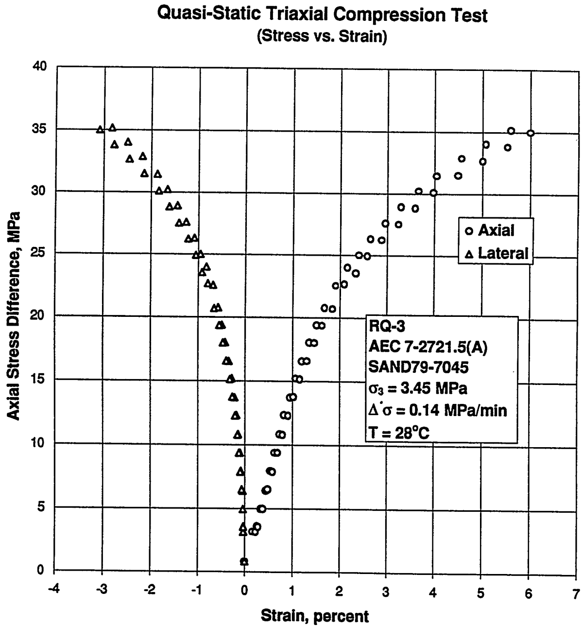
Figure A-6. Axial Stress Difference Versus Axial and Lateral Strain for a Quasi-Static Triaxial Compression Test: Specimen AEC7-2721.5 (A).
