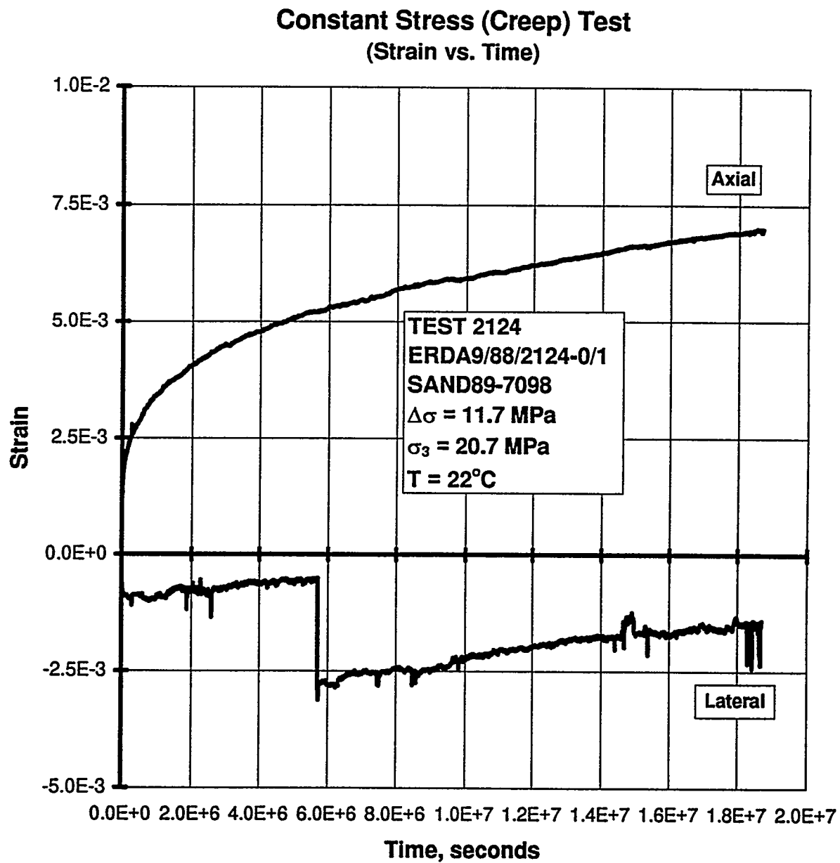
Figure B-4. Axial Strain and Lateral Strain Versus Time for a Creep Test: Specimen ERDA9/88/2124-0/1; Stage 1 of 1.
