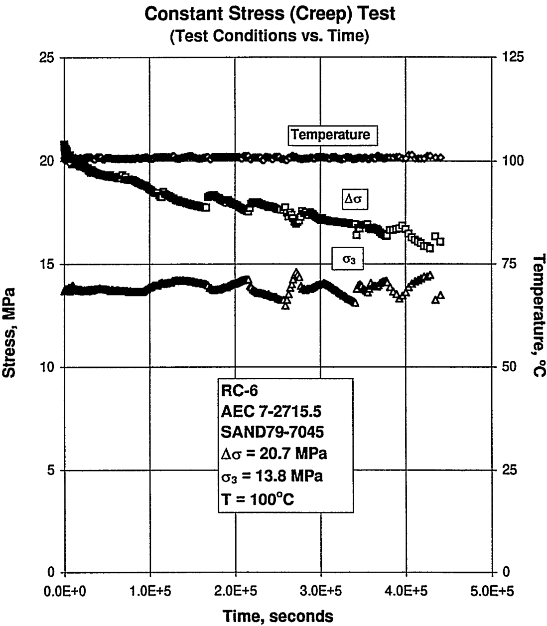
Figure B-193. Test Conditions Versus Time for a Creep Test: Specimen AEC7-2715.5; Stage 1 of 1.
