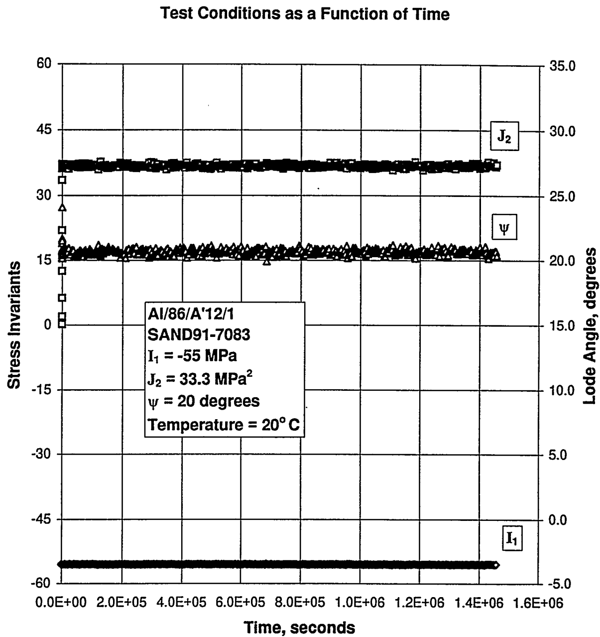
Figure D-9. Test Conditions Versus Time for a Multiaxial Creep Test: Specimen AI/86/A'12/1.
