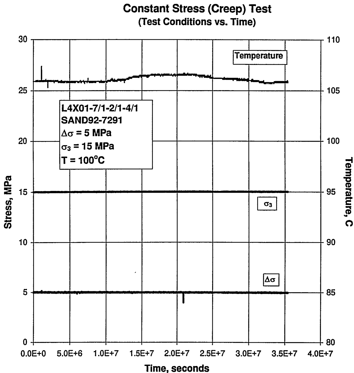
Figure C-29. Test Conditions Versus Time for a Creep Test: Specimen L4X01-7/1-2/1-4/1; Stage 1 of 1 (Argillaceous Salt).
