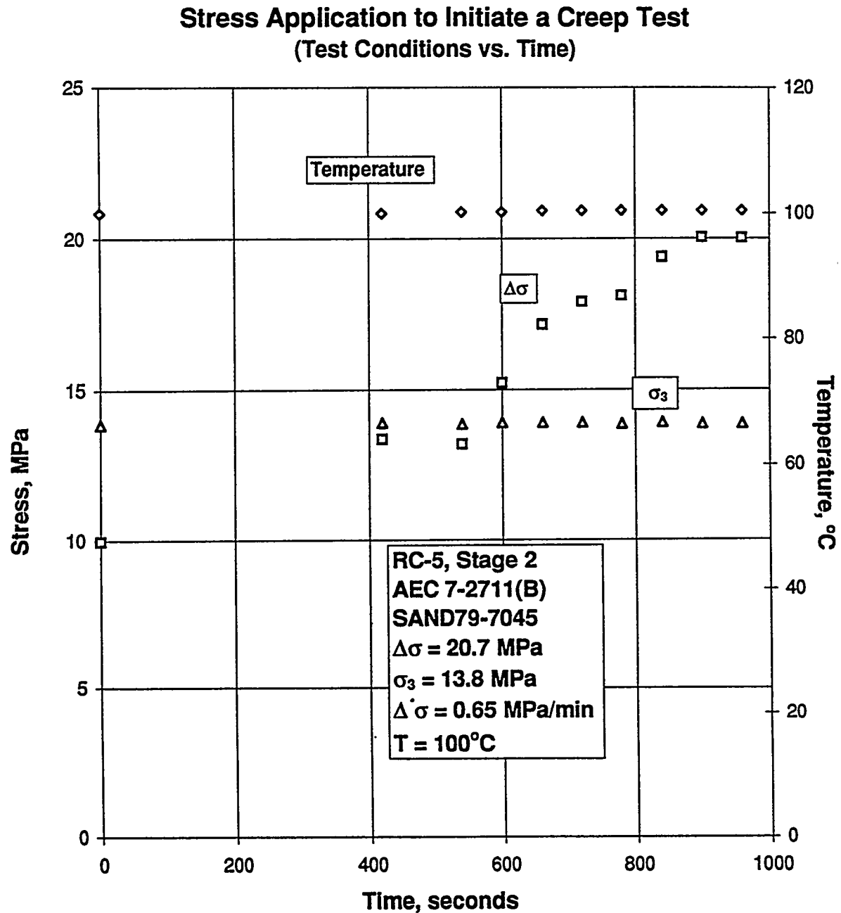
Figure B-187. Test Conditions Versus Time for Stress Application to Initiate a Creep Test: Specimen AEC7-2711 (B); Stage 2 of 2.
