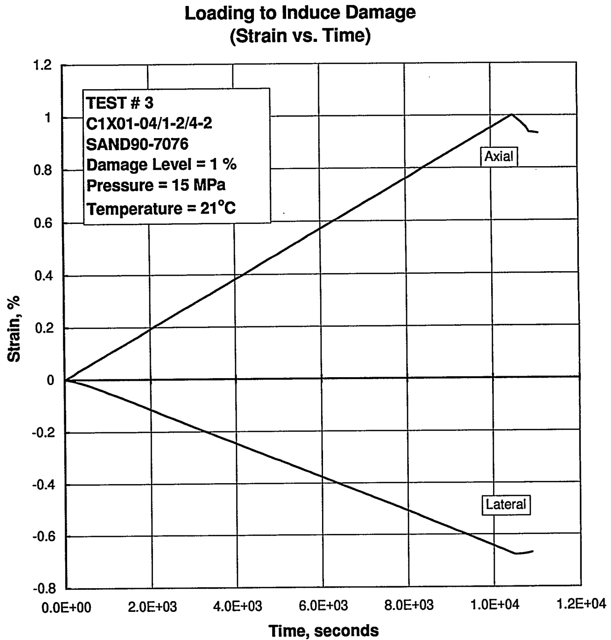
Figure E-60. Axial and Lateral Strain as a Function of Time During the Quasi-Static Loading to Induce Damage in Specimen C1X01-04/1-2/4-2.
