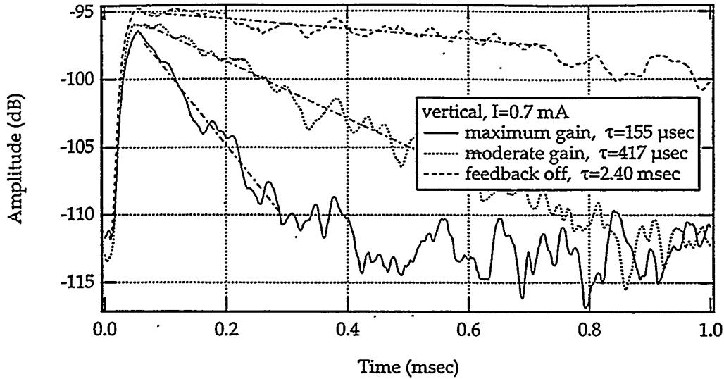
FIGURE 3. Vertical transients for several settings of FB gain for single bunch current of 0.7 mA. Transients are expected to be 10-20 times faster with the preamplifier in the FB loop.
