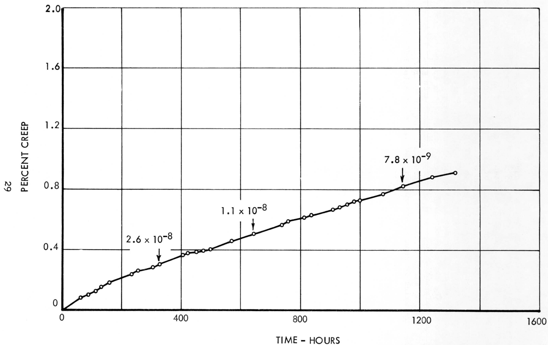
FIGURE 17. CREEP TEST DATA, VAPOR DEPOSITED TUNGSTEN, TESTED AT 2800°F (1538°C) AND 2000 PSI, ( 1.38 \times 10^8 N/m 2 ) IN VACUUM ENVIRONMENT < 1 \times 10^{-8} TORR
