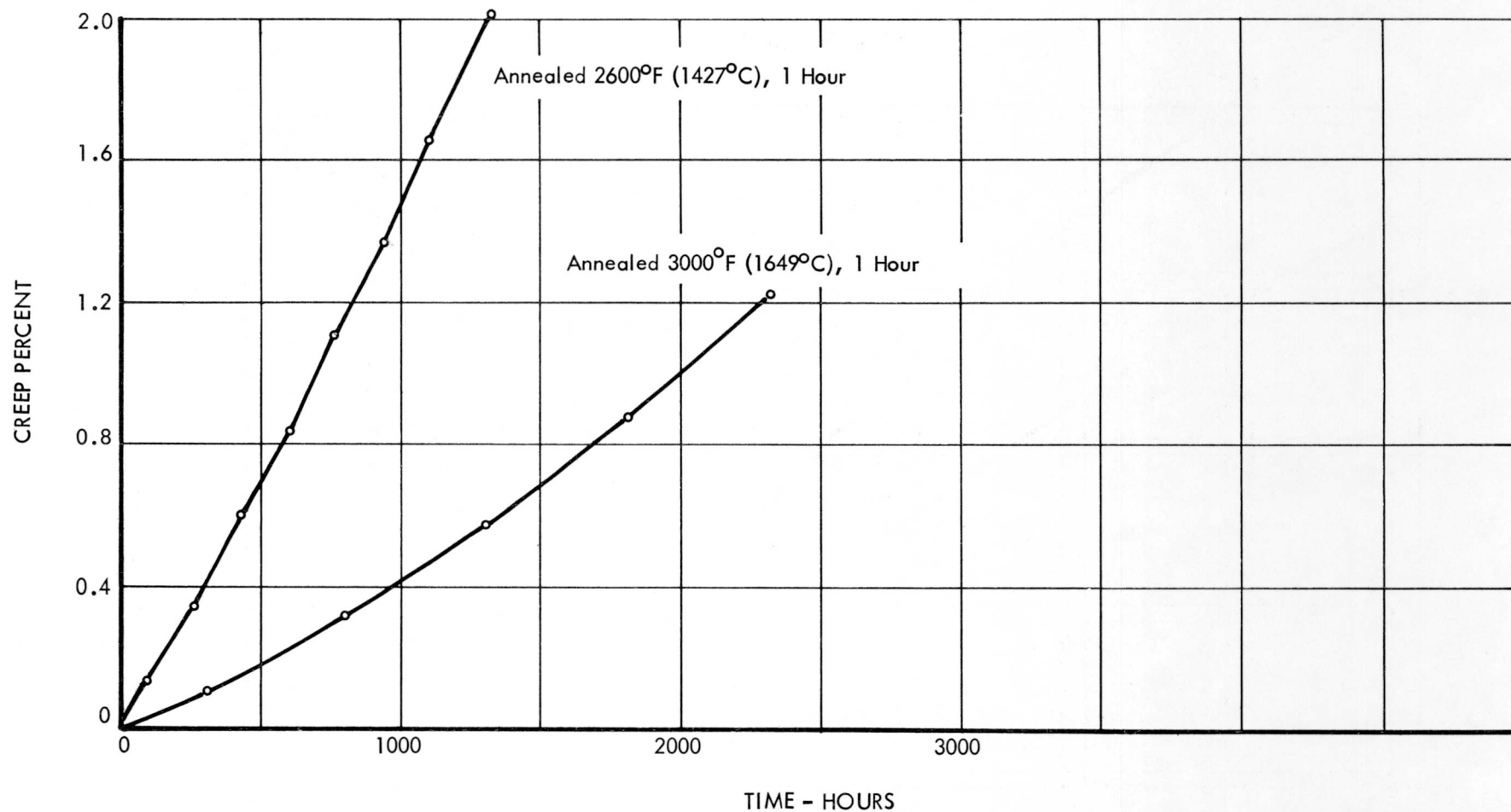
FIGURE 10. CREEP TEST DATA, T-111 ALLOY, TESTED AT 2200°F (1204°C) AND 8 Ksi, ( 5.51 \times 10^7 N/m 2 ), TESTED IN VACUUM ENVIRONMENT < 1 \times 10^{-8} TORR
