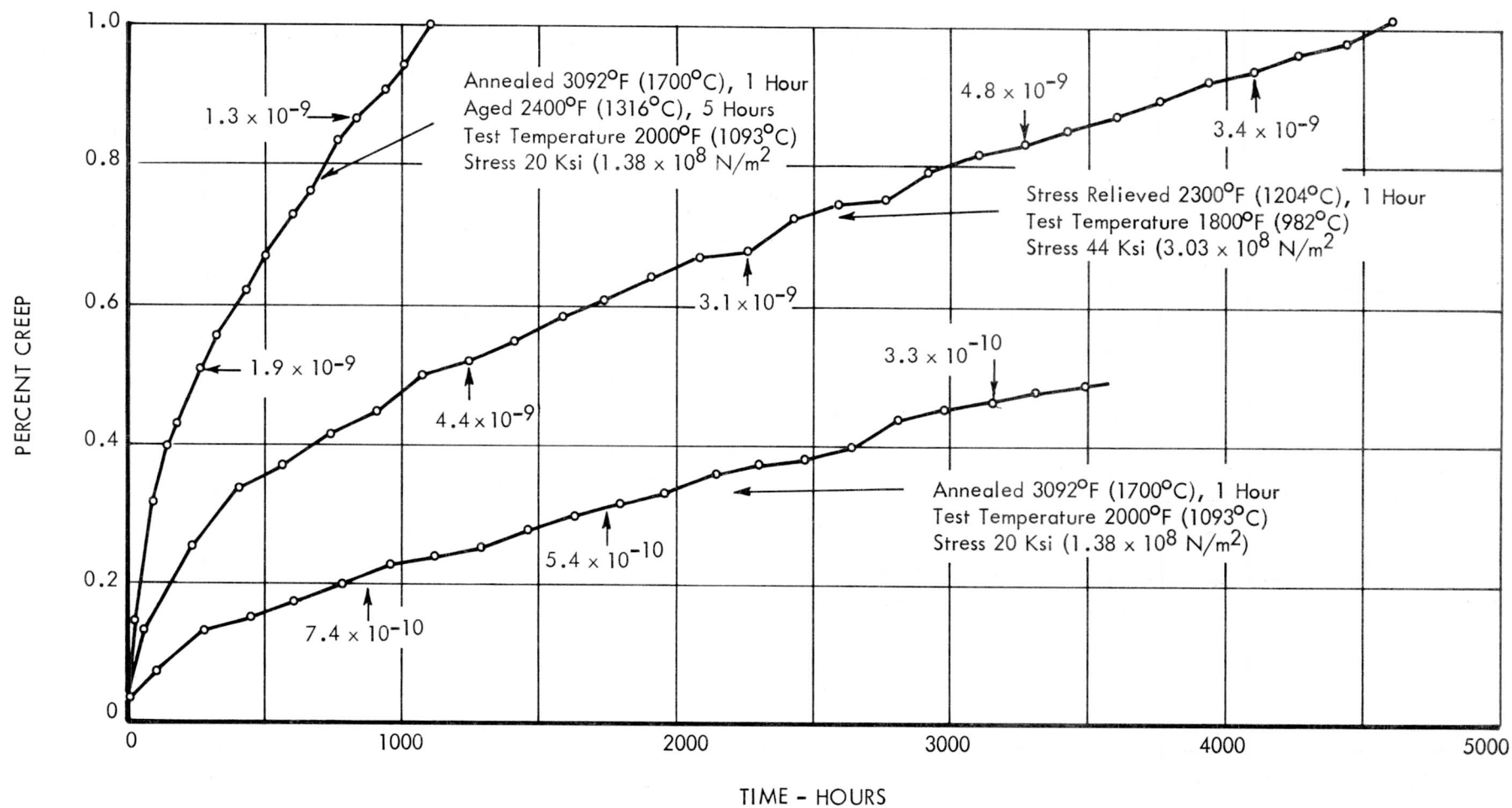
FIGURE 2. CREEP TEST DATA, TZC (HEAT M-91), TESTED IN VACUUM ENVIRONMENT < 1 \times 10^{-8} TORR
