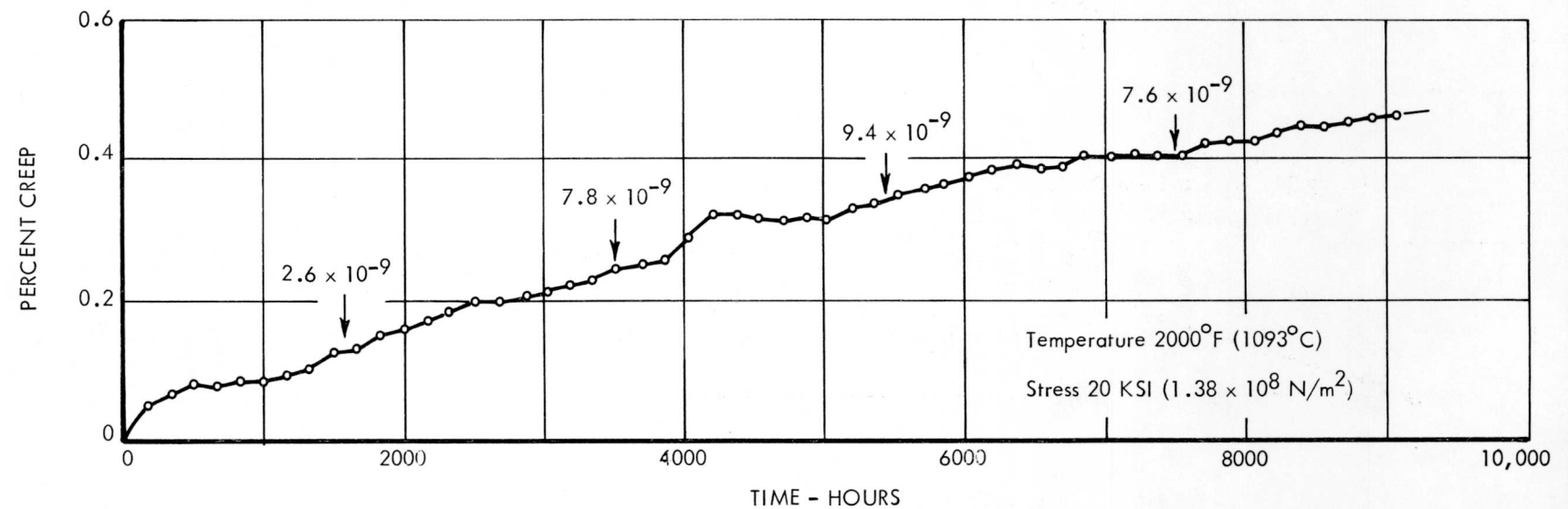
FIGURE 1. CREEP TEST DATA, TZC (HEAT M-80), ANNEALED 3092°F (1700°C) 1 HOUR TESTED IN VACUUM ENVIRONMENT < 1 \times 10^{-8} TORR
