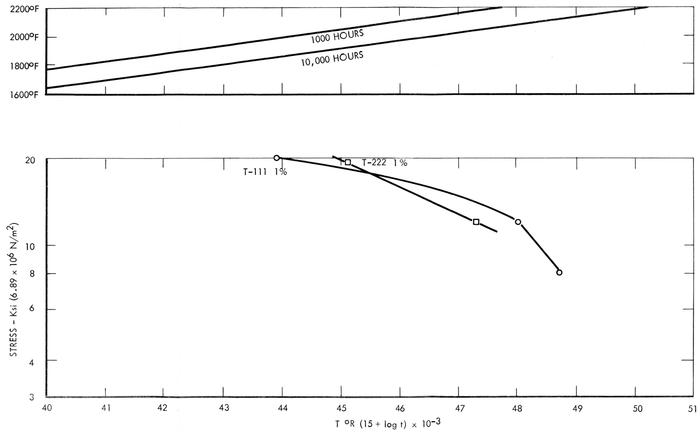
FIGURE 13 LARSON MILLER PLOT, 1% CREEP FOR T-111 AND T-222 ALLOYS ANNEALED 1 HOUR 3000°F (1649°C), TESTED IN VACUUM ENVIRONMENT <1 \times 10^{-8} TORR
