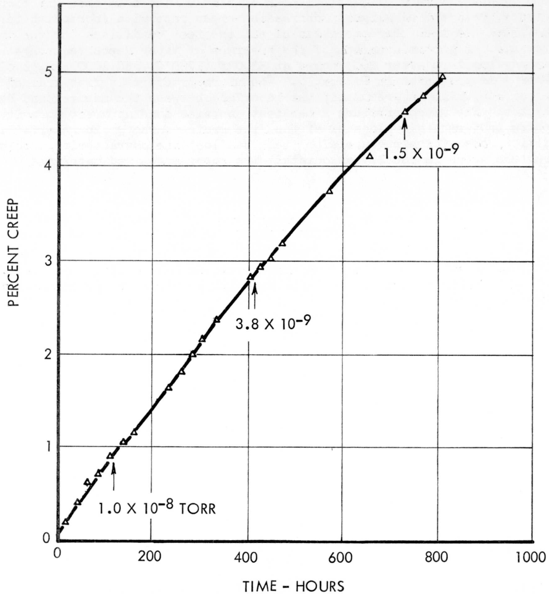
Figure 16. CREEP DATA FOR ARC-MELTED TUNGSTEN, TESTED AT 2800°F (1538°C) IN VACUUM ENVIRONMENT 1 X 10 -8 TORR
