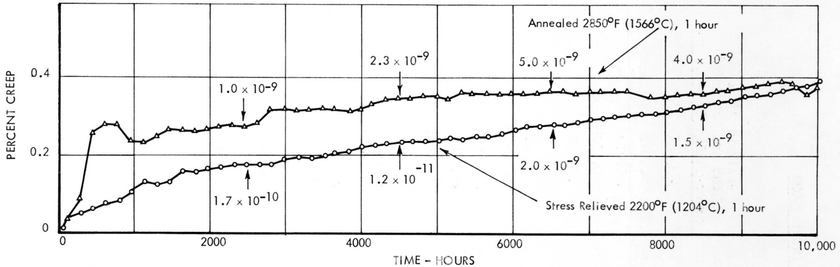
FIGURE 7A. CREEP TEST DATA, TZM HEAT 7502, TESTED AT 2000°F (1093°C) AND 10 Ksi ( 6.90 \times 10^7 N/m 2 ) IN VACUUM ENVIRONMENT < 1 \times 10^{-8} TORR
