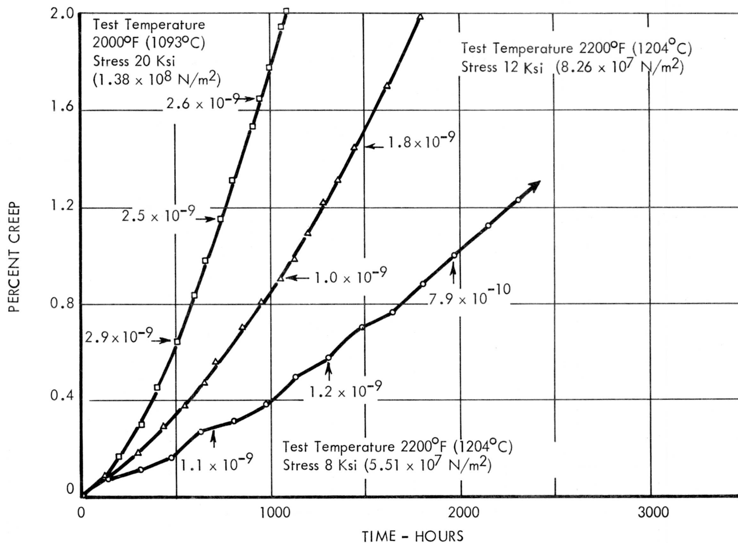
FIGURE 11. CREEP TEST DATA, T-111 (HEAT 70616) ANNEALED 3000°F (1649°C) 1 HOUR, TESTED IN VACUUM ENVIRONMENT < 1 \times 10^{-8} TORR
