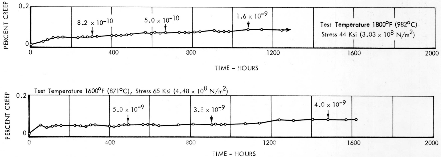
FIGURE 7B. CREEP TEST DATA, TZM HEAT 1175, STRESS RELIEVED 2300°F (1260°C) 1 HOUR, TESTED IN VACUUM ENVIRONMENT < 1 \times 10^{-8} TORR
