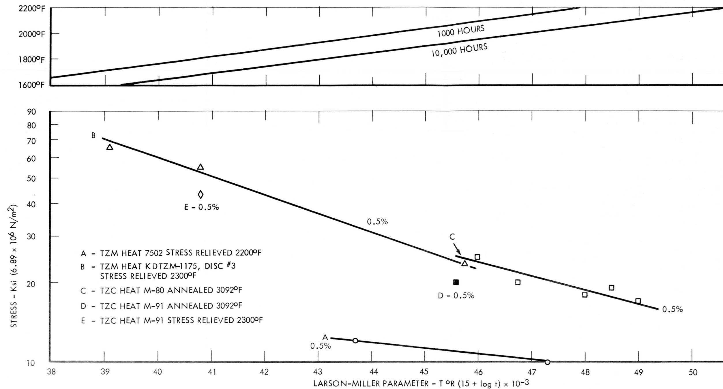
FIGURE 8 LARSON-MILLER PLOT OF DATA FOR 0.5% CREEP IN VARIOUS MOLYBDENUM-BASE ALLOYS
