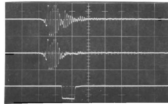
(d) Upper - Amplifier Output, Weld Test, Poor and Good Penetration Lower - Normal Gate A 5 V/cm, 1 \mu sec/cm
