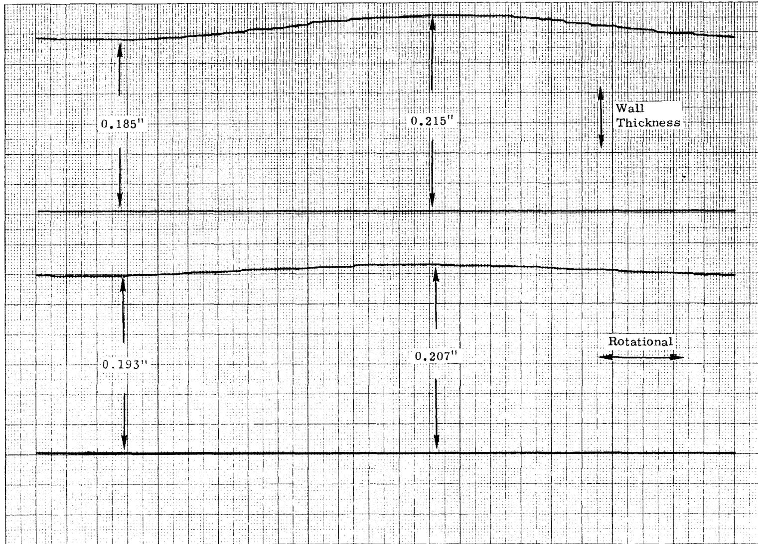
FIGURE 16. Wall Thickness Test, 2 inch Diameter Eccentric, SST Tube
