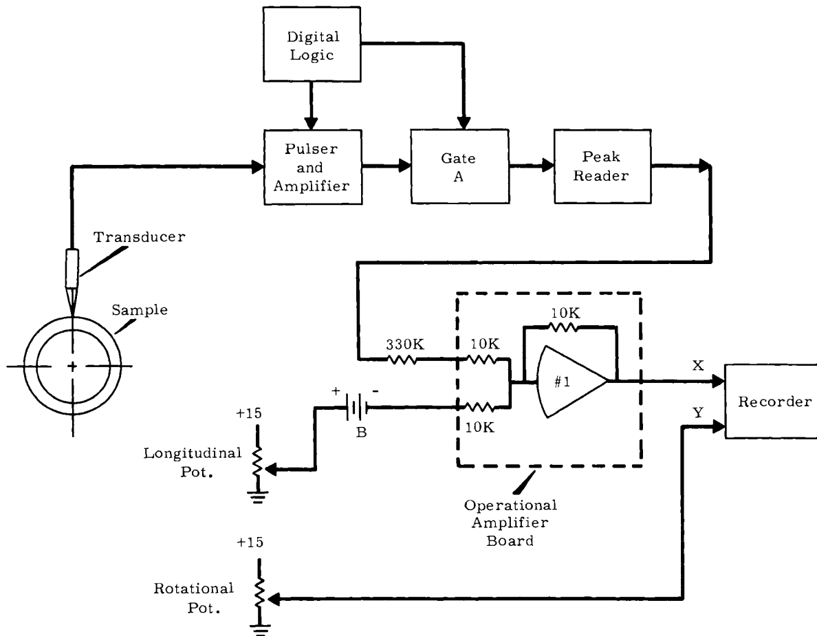
FIGURE 12. Modified Arrangement, Weld Test
