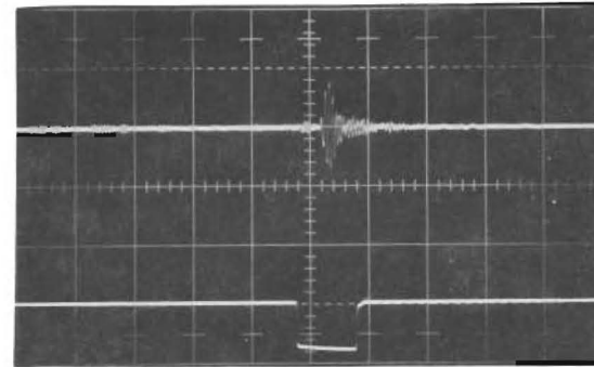
(b) Upper - Amplifier Output, Shear Crack Test 2 V/cm Lower - Normal Gate A 5 V/cm 1 \mu sec/cm
