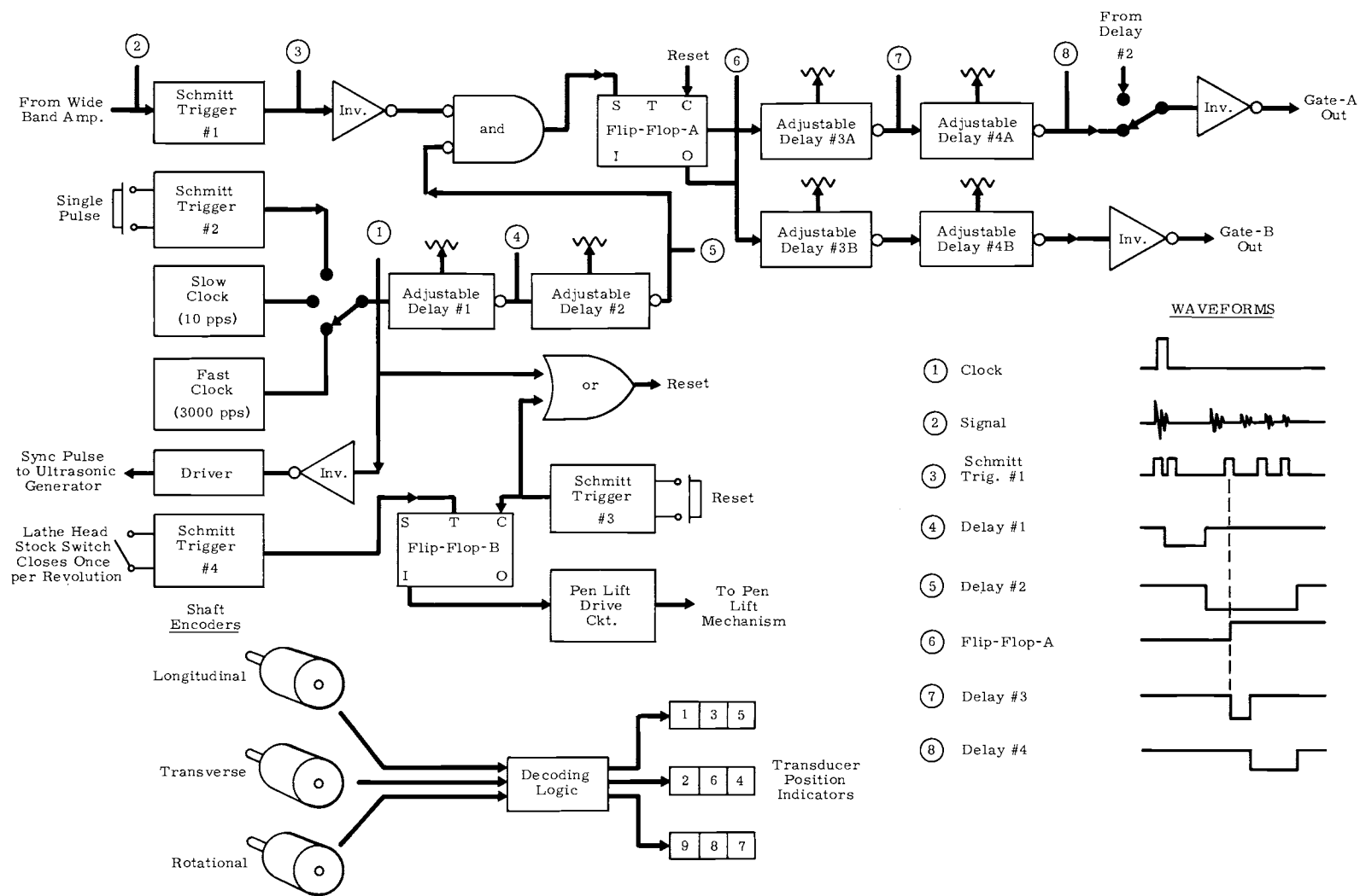
FIGURE 7. Logic Diagram
