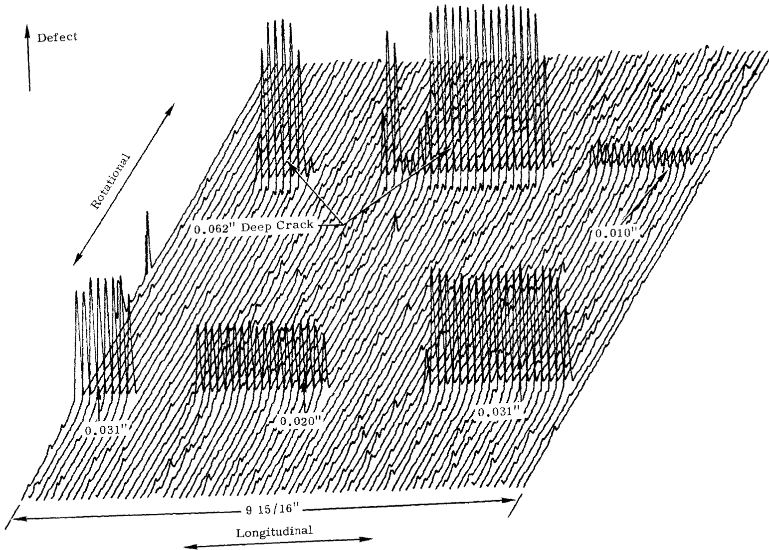
FIGURE 14. Crack Test, 2 inch Diameter x 1/4 inch Wall SST Tubing
