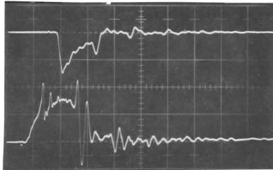
(a) Upper - Transmit Pulse at Preamp. 100 V/cm Lower - Sync Pulse 2 V/cm 0.1 \mu sec/cm
