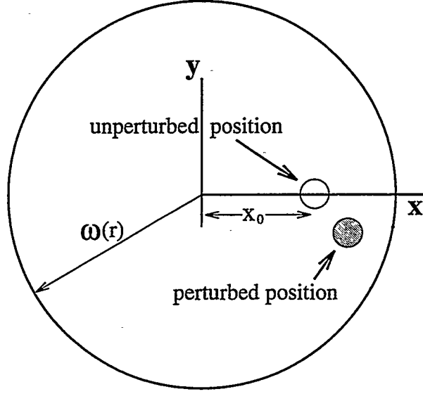
Figure 6.18: A vortex filament surrounded by a continuous vorticity field.
