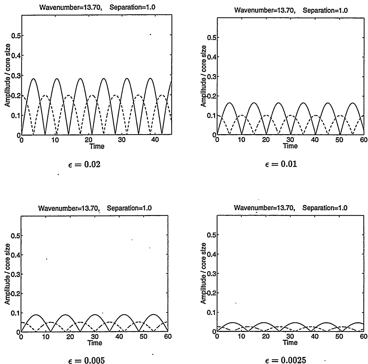
Figure 6.10: Time evolution of the perturbations with different initial amplitudes on a pair of co-rotating vortex filaments. Dashed line : amplitude in the x -direction (spanwise direction); Solid line : amplitude in the y -direction. The coordinate system is rotating with the vortex pair.
