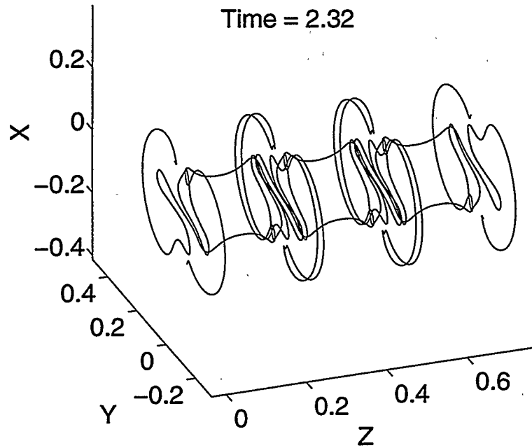
Figure 6.17: Configuration of the vortex pair after the two filaments become tangled together.
