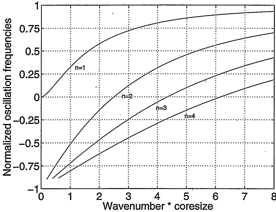
Figure 3.5: Oscillation frequencies of the first four radial modes on a filament with constant vorticity.
