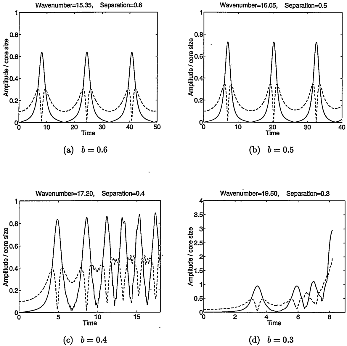
Figure 6.15: Time evolution of the perturbations on a pair of co-rotating vortex filaments with different separations. Dashed line : amplitude in the x -direction (spanwise direction); Solid line : amplitude in the y -direction. The coordinate system is rotating with the vortex pair.
