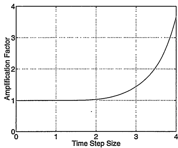
Figure 5.9: Amplification factor of the Prince-Dormand 5(4) method.
