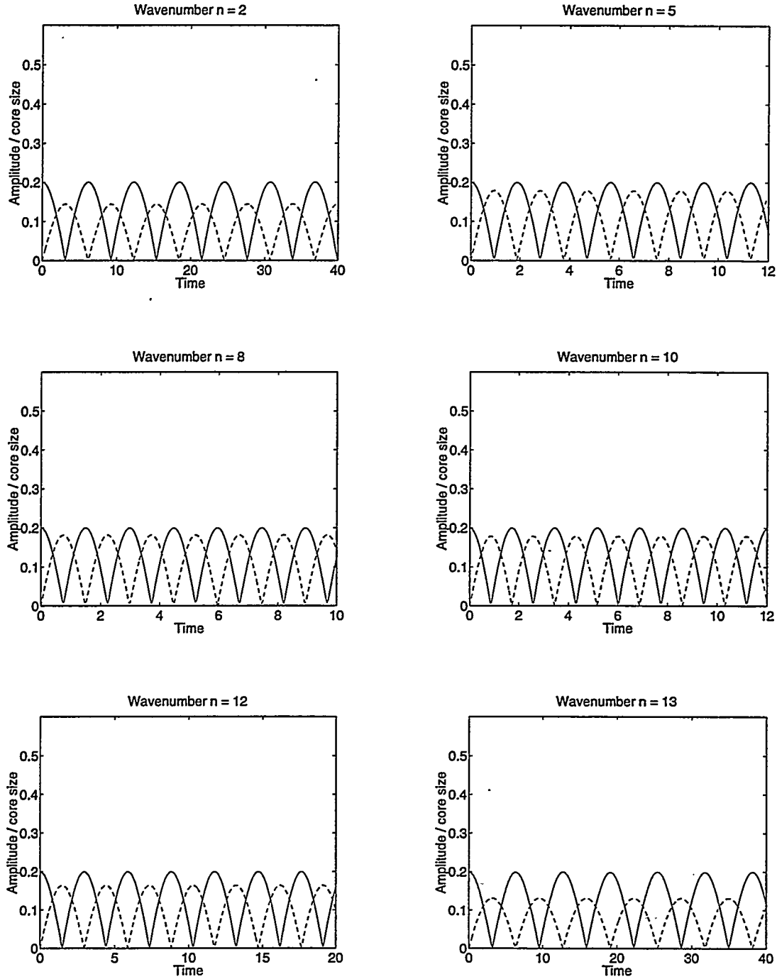
Figure 4.3: Evolution of the amplitude of the perturbation for the ring perturbed at wavenumber n = 2, 5, 8, 10, 12, 13 , respectively. The solid line denotes the amplitude \Delta\rho in the radial direction and the dashed line denotes the amplitude \Delta z in the streamwise direction.
