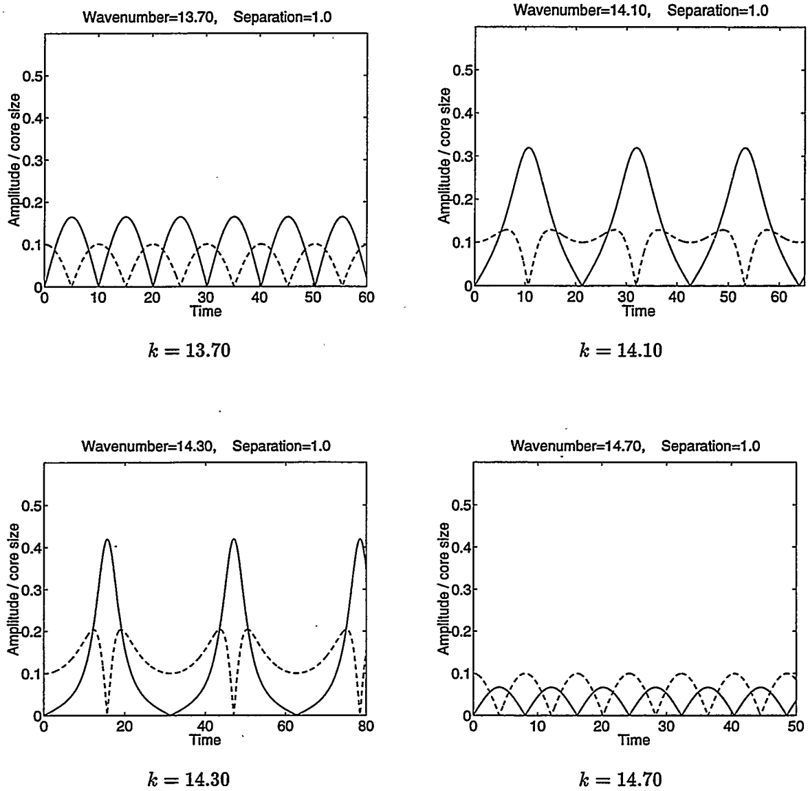
Figure 6.9: Time evolution of the perturbations of different wavenumbers on a pair of co-rotating vortex filaments. Dashed line : amplitude in the x -direction (spanwise direction); Solid line : amplitude in the y -direction. The coordinate system is rotating with the vortex pair.
