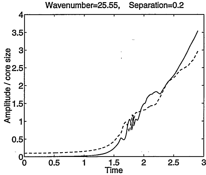
Figure 6.16: Time evolution of the perturbation on a pair of co-rotating vortex filaments. Dashed line : amplitude in the x -direction (spanwise direction); Solid line : amplitude in the y -direction. The coordinate system is rotating with the vortex pair.
