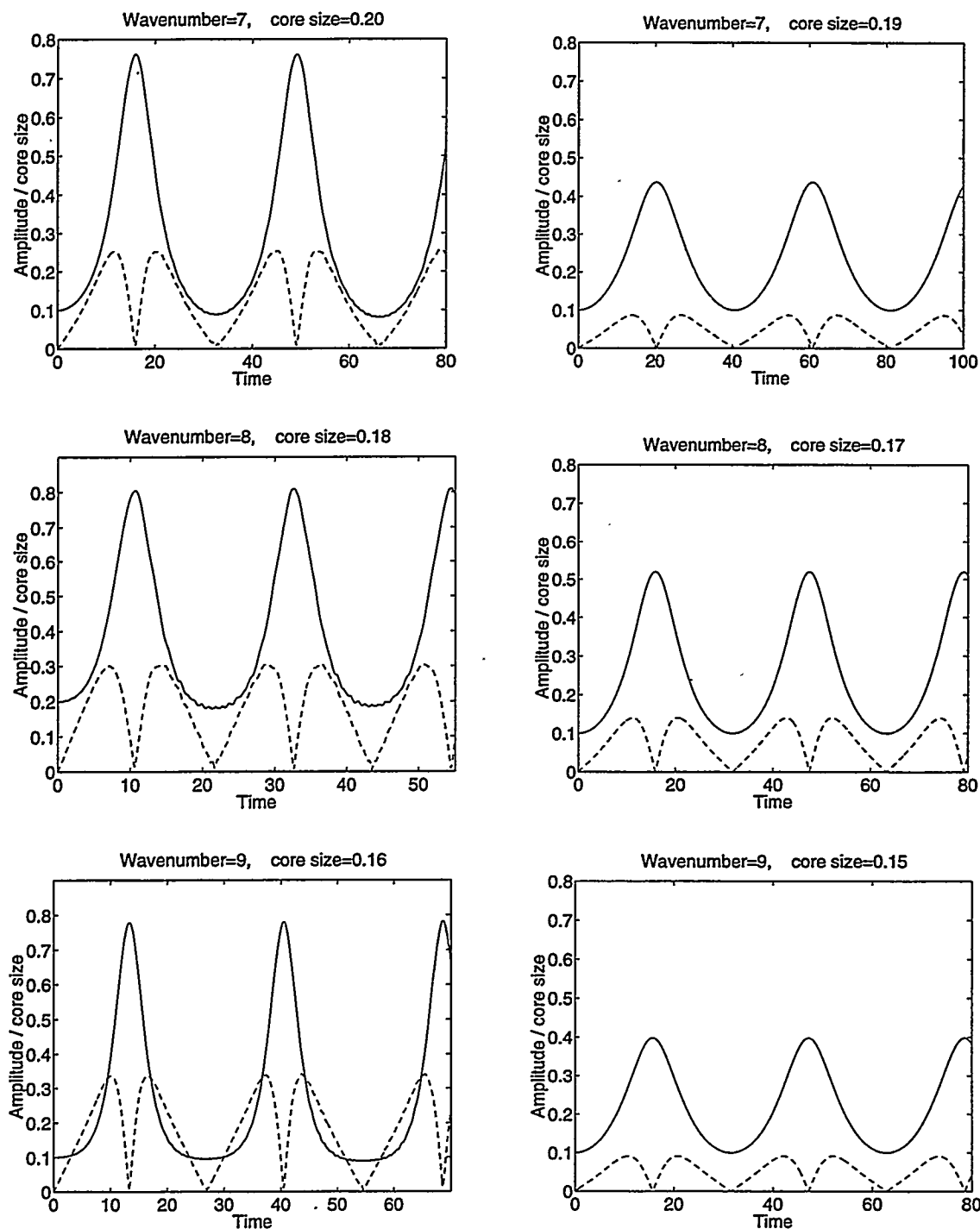
Figure 4.15: Comparison of the evolution of the corresponding unstable mode on a vortex ring for different core sizes. The solid line represents the amplitude in the radial direction and the dashed line represents the amplitude in the streamwise direction.
