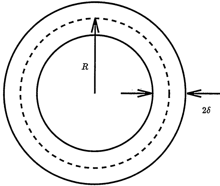
Figure 2.3: A front-on view of a vortex ring with ring radius R and core radius \delta .
