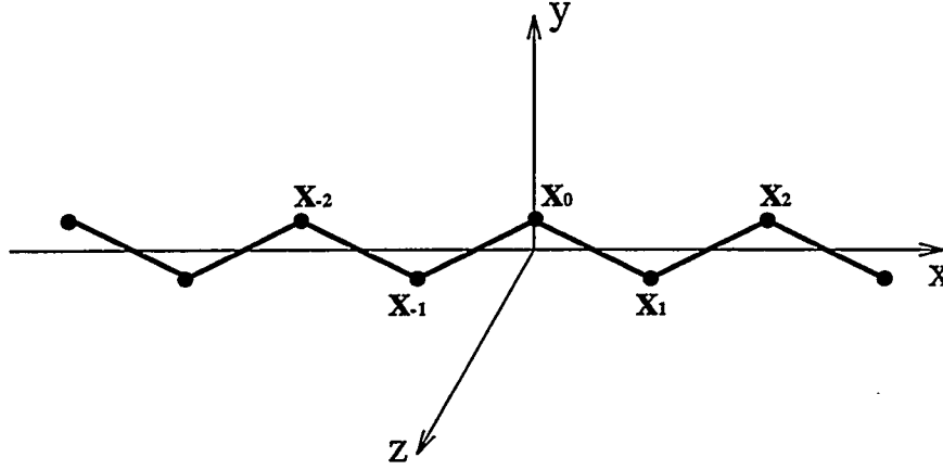
Figure 5.4: A sketch of the highest discrete mode.
