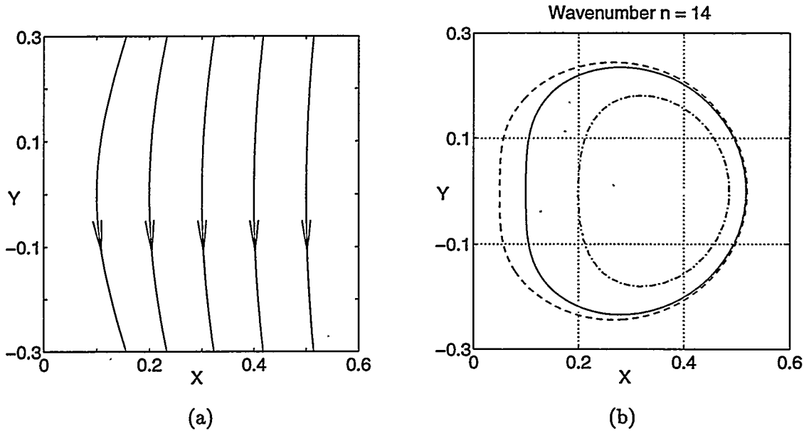
Figure 4.14: (a). A family of hyperbolas and the direction of the motion on them, predicted by the stagnation point flow plus the dispersion relation of sinusoidal waves with small amplitude. (b). The motion of perturbation waves, with respect to the unperturbed filament, obtained in the numerical simulations. --- : initial amplitude \varepsilon = 0.2\delta , - : \varepsilon = 0.1\delta , - \cdot - : \varepsilon = 0.05\delta . All coordinates have been normalized by the core size.
