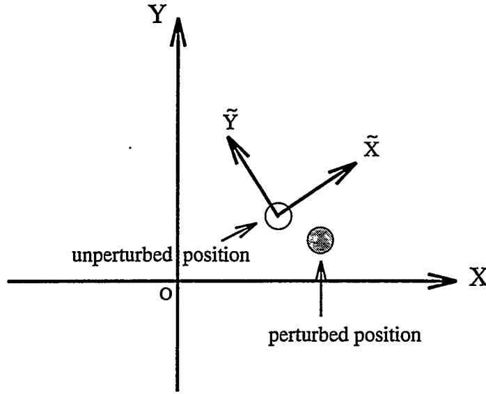
Figure 6.19: The vortex filament and the coordinate system attached to it.
