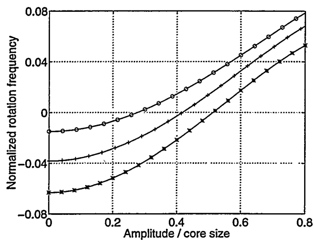
Figure 6.12: Normalized rotation frequency vs amplitude/core radius. -o- : k\delta = 1.40 ; -+- : k\delta = 1.45 ; -*- : k\delta = 1.50 .
