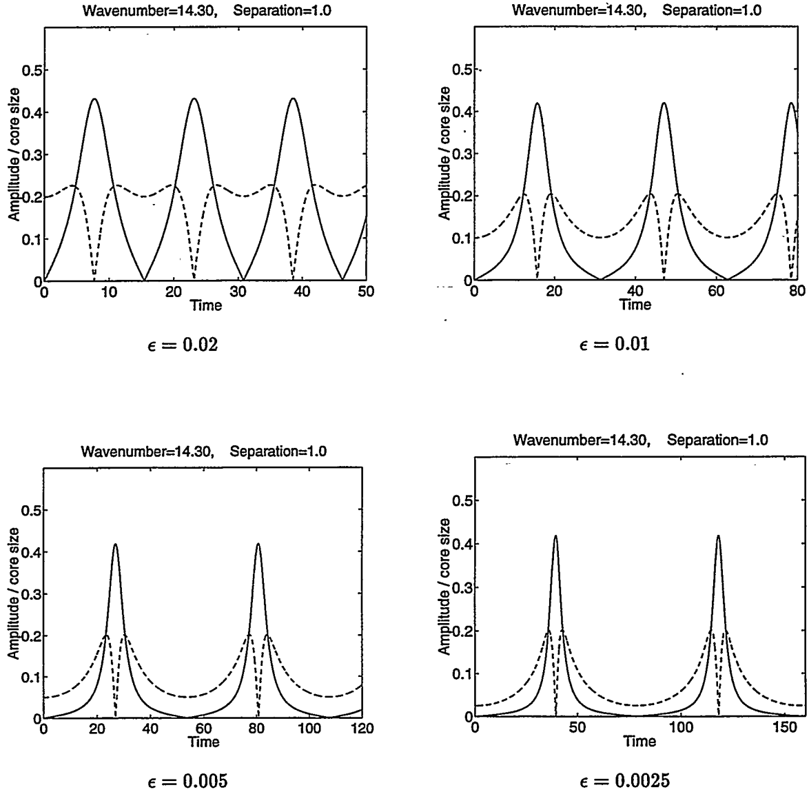
Figure 6.11: Time evolution of the perturbations with different initial amplitudes on a pair of co-rotating vortex filaments. Dashed line : amplitude in the x -direction (spanwise direction); Solid line : amplitude in the y -direction. The coordinate system is rotating with the vortex pair.
