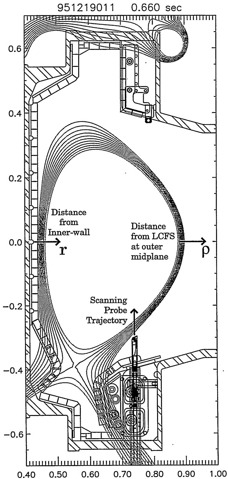
Figure 6.1: Mapping of Scanning Probe to \rho and r along Flux Surfaces (Distances in meters)
