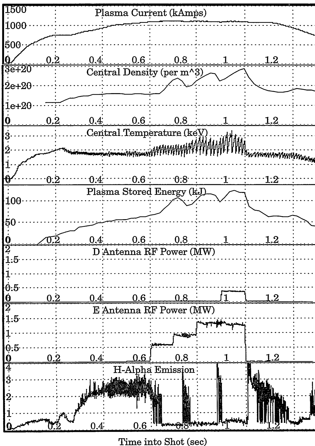
Figure 1.6: Parameter Time Histories for Shot 960126027
