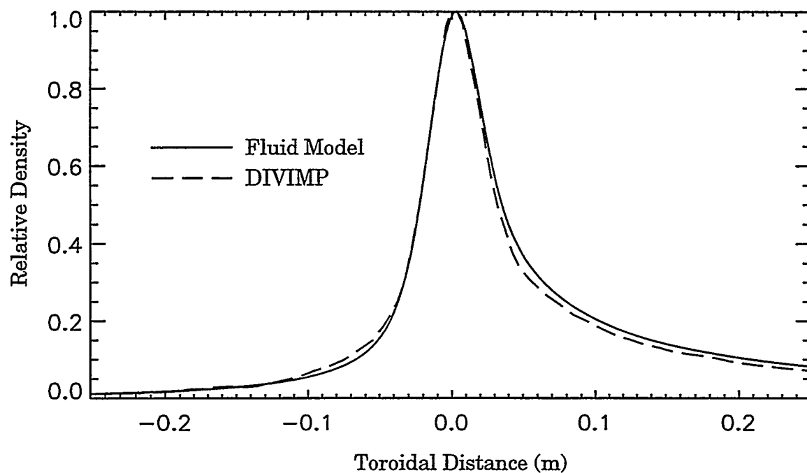
Figure 5.7: Parallel Profile Match to DIVIMP Case A
