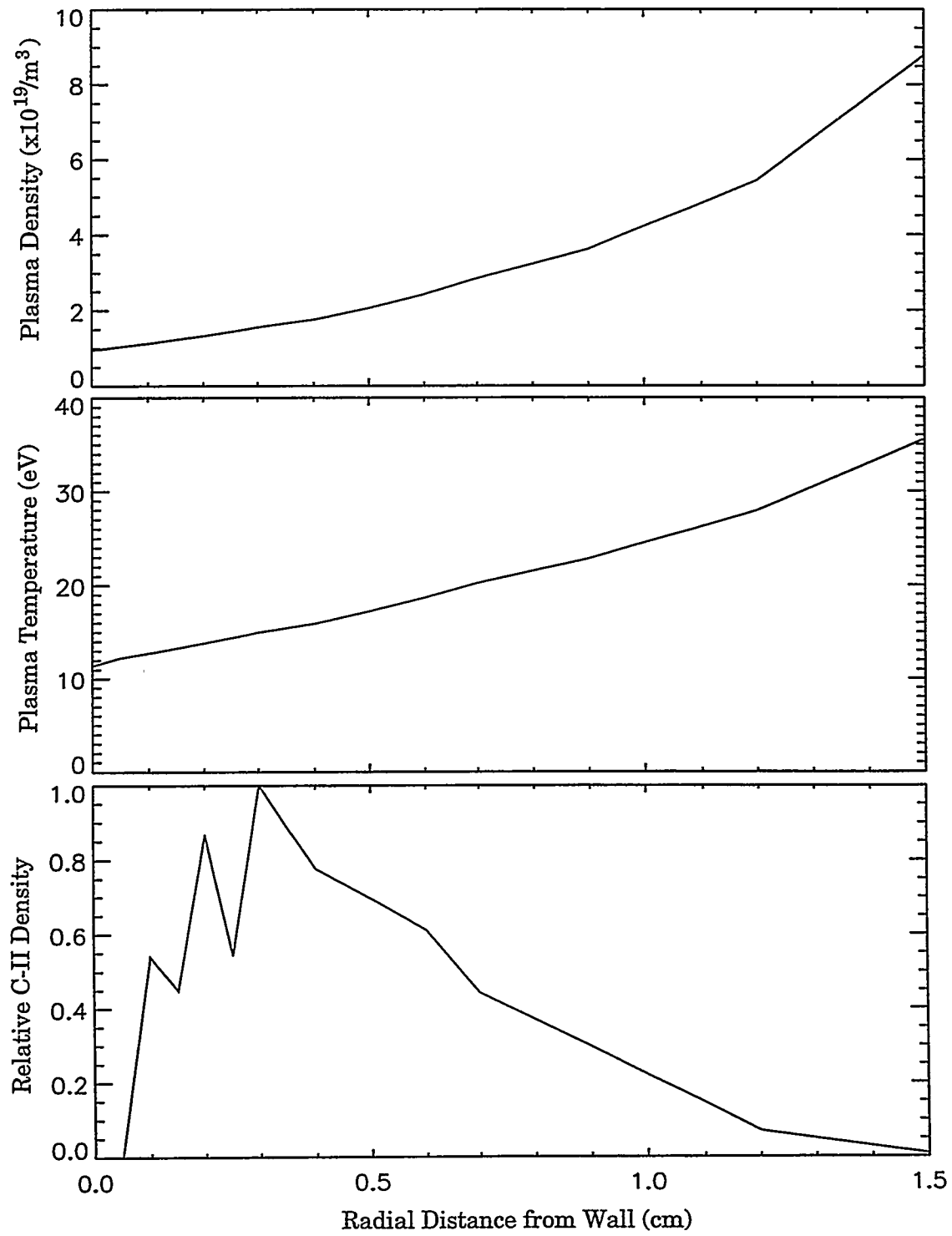
Figure 5.9: Radial Plasma Profiles for DIVIMP Case B
