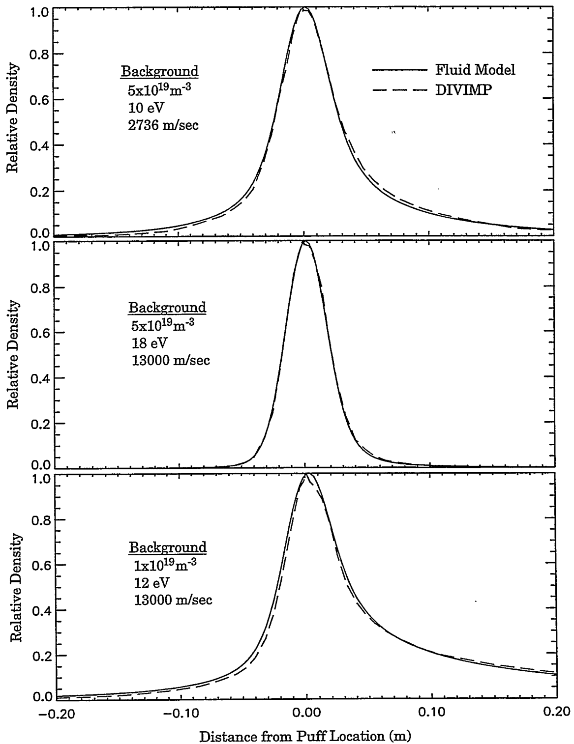
Figure 5.5: 1-D Comparisons of DIVIMP and Fluid Model
