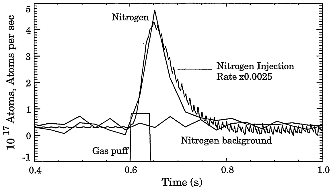
Figure 3.6: Time Dependence of Confined Nitrogen
