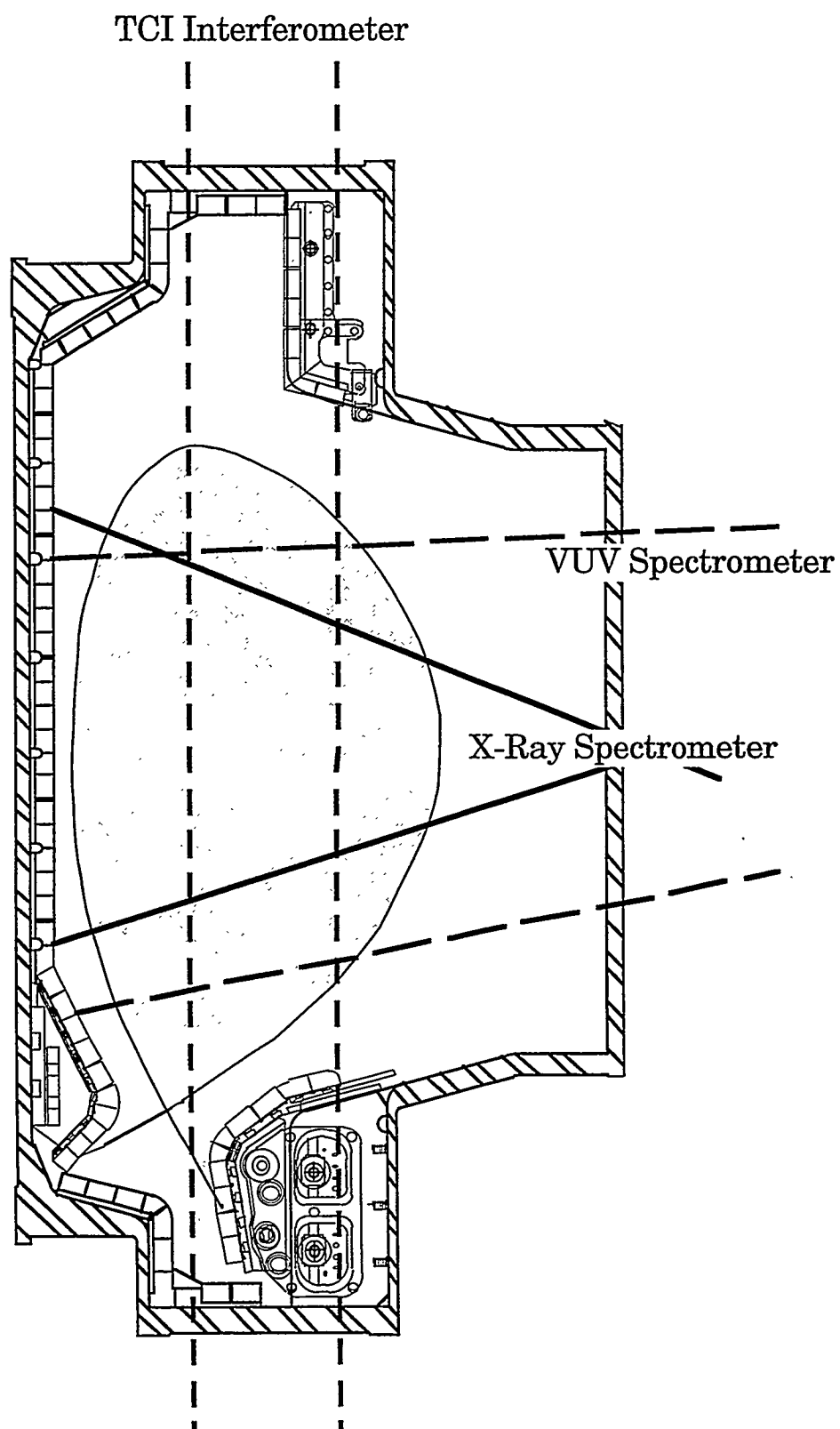
Figure 2.9: Extent of Chords of three C-Mod Core Diagnostics
