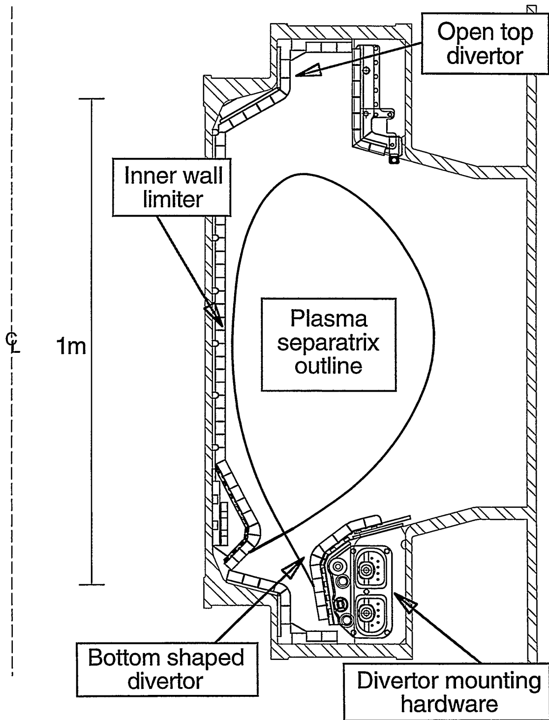
Figure 1.8: C-Mod Plasma Facing Components
