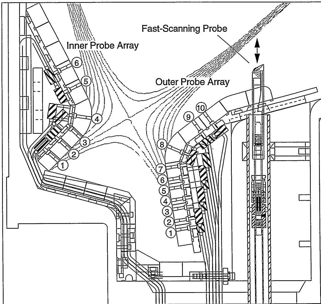
Figure 2.6: Alcator C-Mod Langmuir Probes
