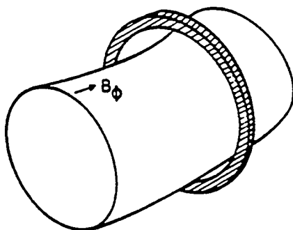
Poloidal limiter
