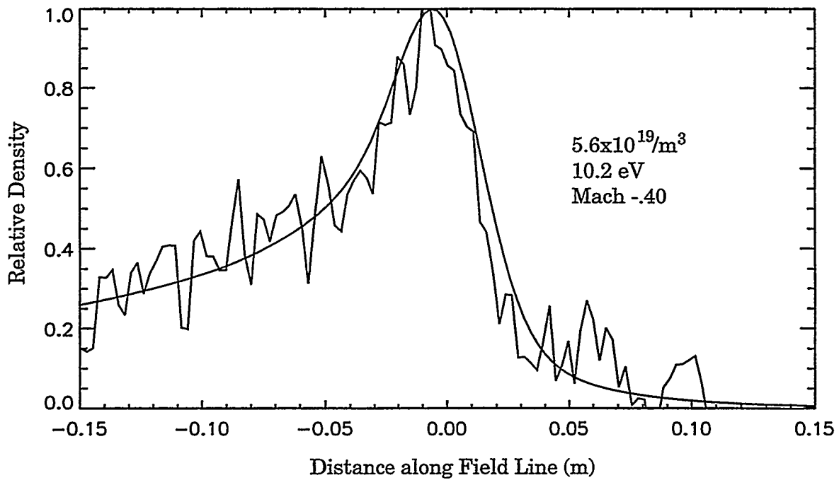
Figure 6.6: Parallel Fluid fit to Shot 951219011
