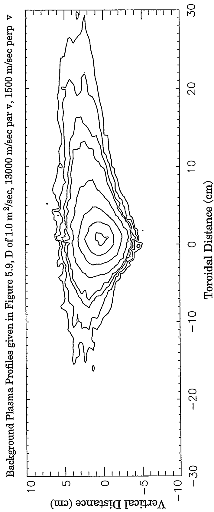
Figure 5.10: DIVIMP Case B Plume
