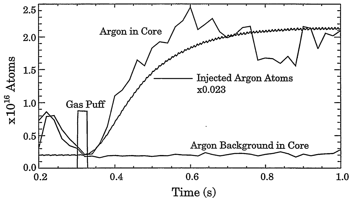
Figure 3.4: Time Dependence of Confined Argon
