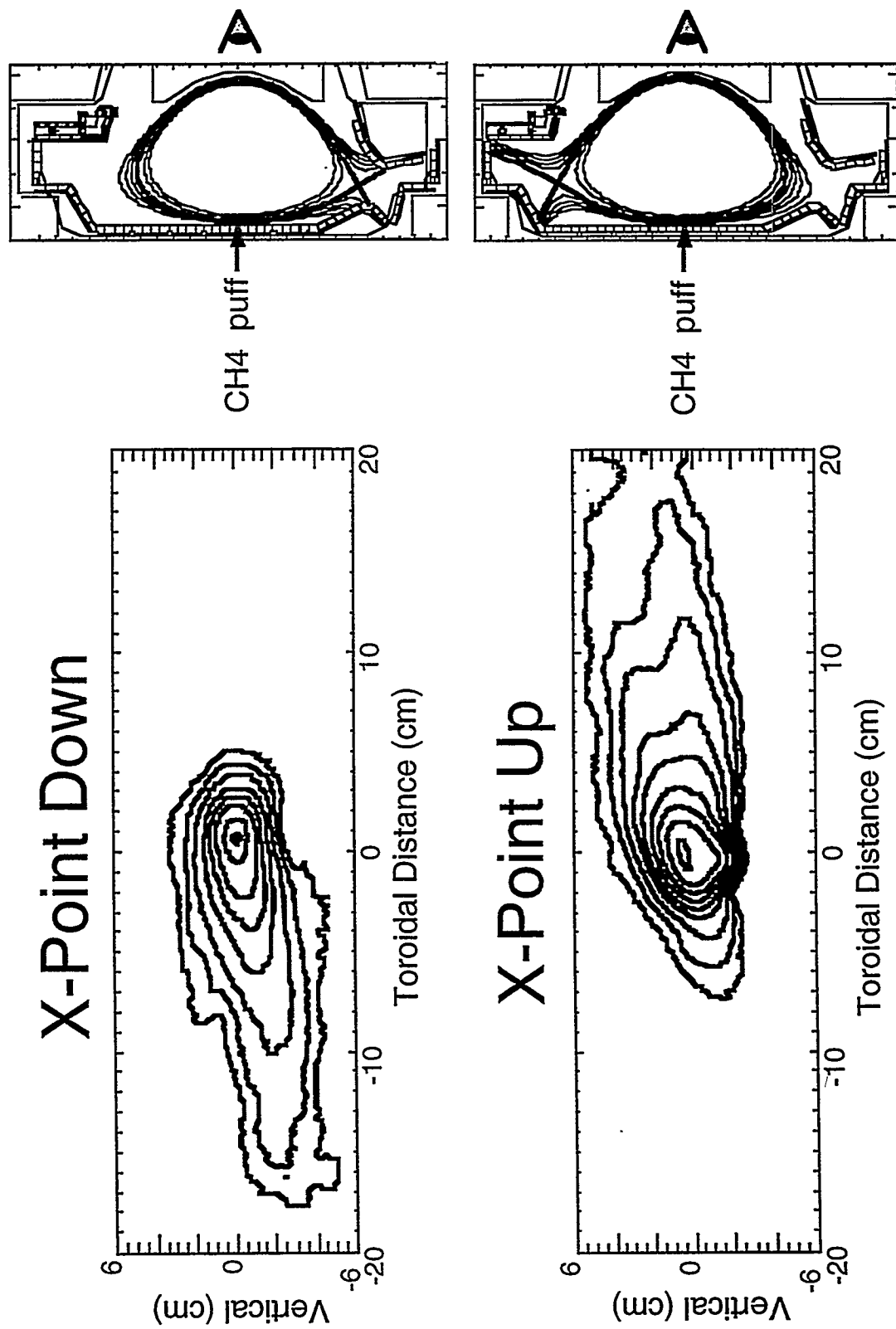
Figure 4.2: C-II Plumes with Lower and Upper X-Points
