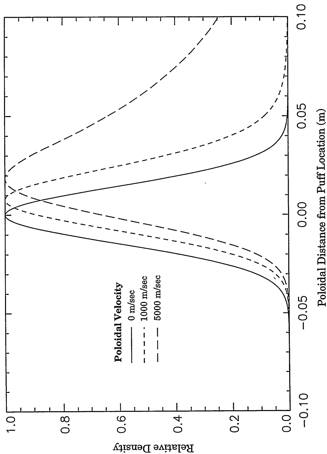
Figure 5.4: Poloidal C-II Density Profiles for Background 5 \times 10^{19} / \text{m}^3 and 12 eV, D of .5 \text{ m}^2 / \text{sec}
