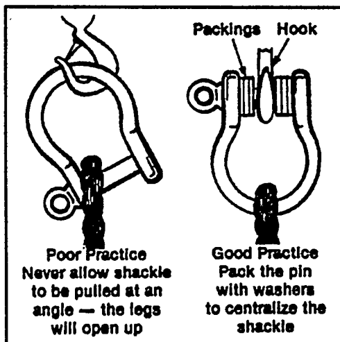
Figure 8-23. Shackles.
