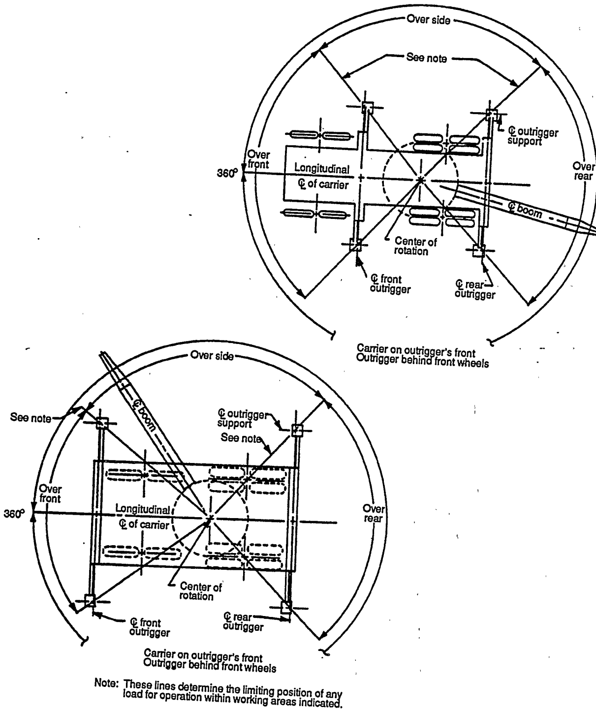
Figure 4-3. Work areas for boom cranes.
