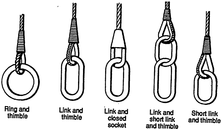
Figure 8-26. Rings and Links.
