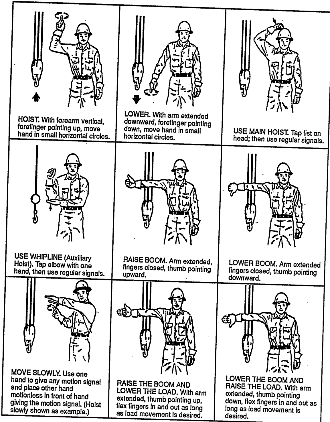
Figure 4-2. Standard Hand Signals for Controlling Mobile Crane Operators
