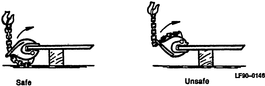
Figure 8-27. Metal-Plate Clamps.
