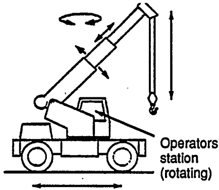
Figure 9-5. Wheel-Mounted Crane— Telescoping Boom (Single Control Station)
