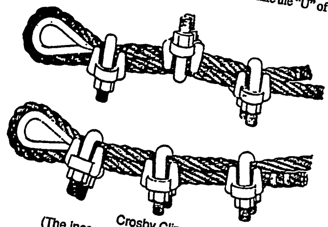
Figure 8-12. Crosby Clips (The wrong way to clip wire rope)
