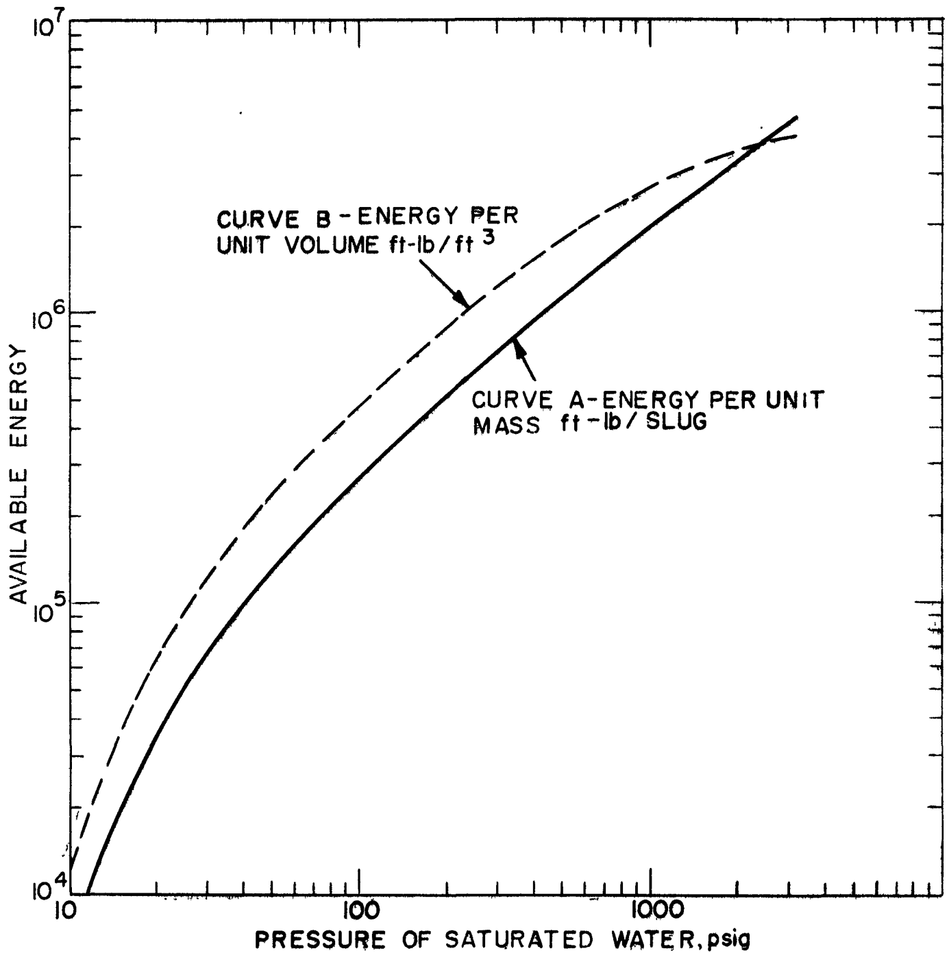
FIGURE I. ENERGY RELEASED ON ISENTROPIC EXPANSION OF SATURATED WATER TO ONE ATMOSPHERE
