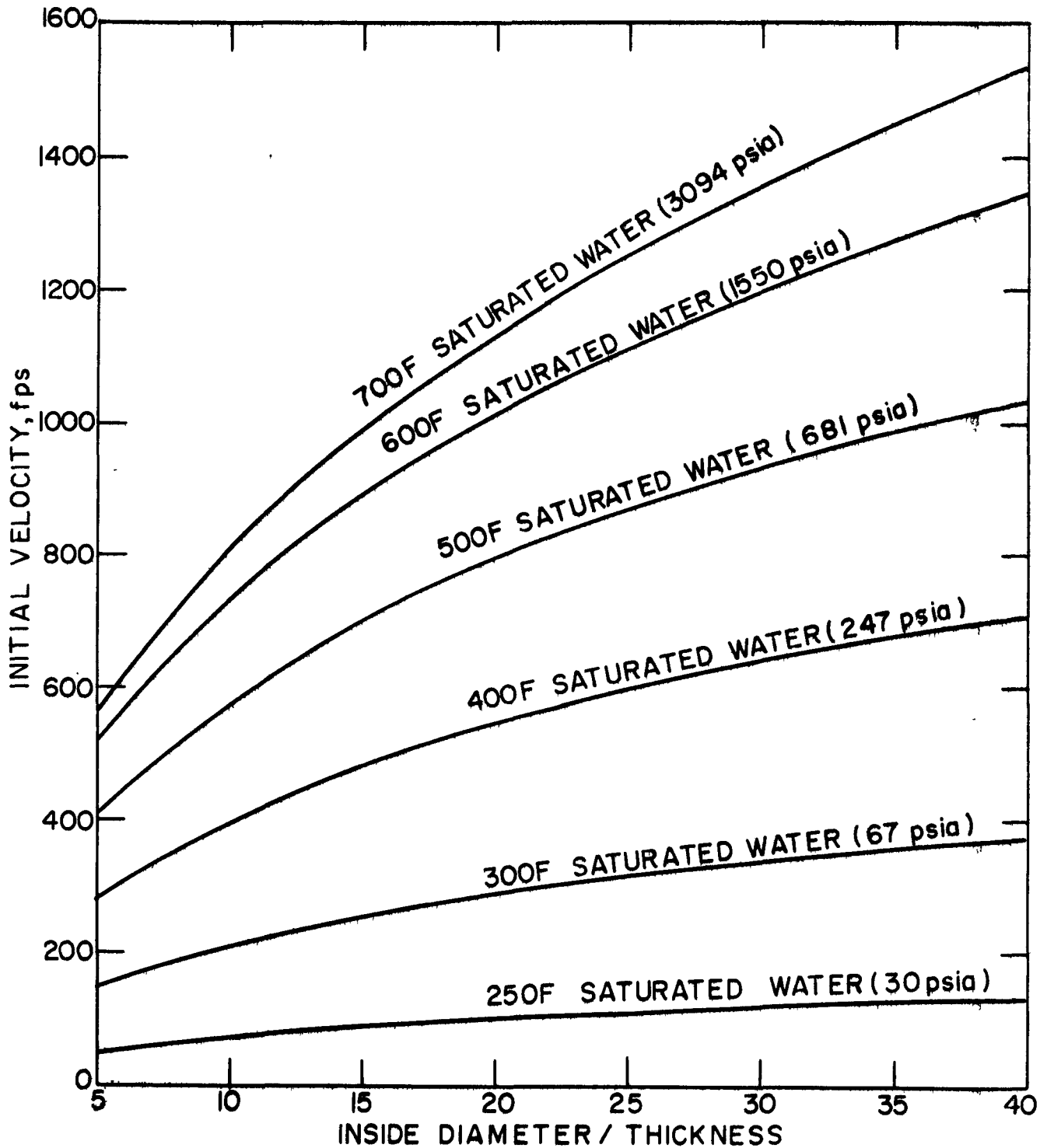
FIGURE 2. INITIAL VELOCITY OF FRAGMENTS OF LONG CYLINDRICAL PRESSURE VESSEL WITH WALLS OF 490 lb/ft 3 DENSITY, ADAPTED FROM GURNEY, BRL-405
