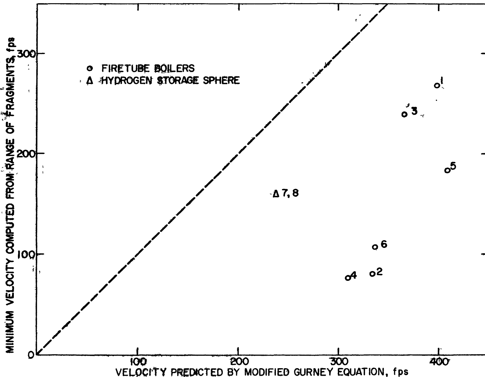
FIGURE 8 COMPARISON OF PREDICTED VELOCITIES OF FRAGMENTS OF EXPLODING PRESSURE VESSEL SHELLS WITH VELOCITIES CALCULATED FROM RANGE OF FRAGMENTS
