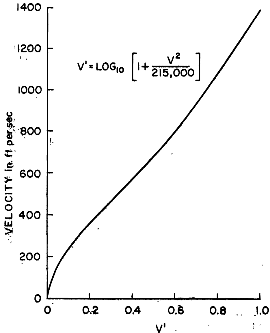
FIG.4 VELOCITY FACTOR ( V' ) FOR IMPACT PENETRATION
