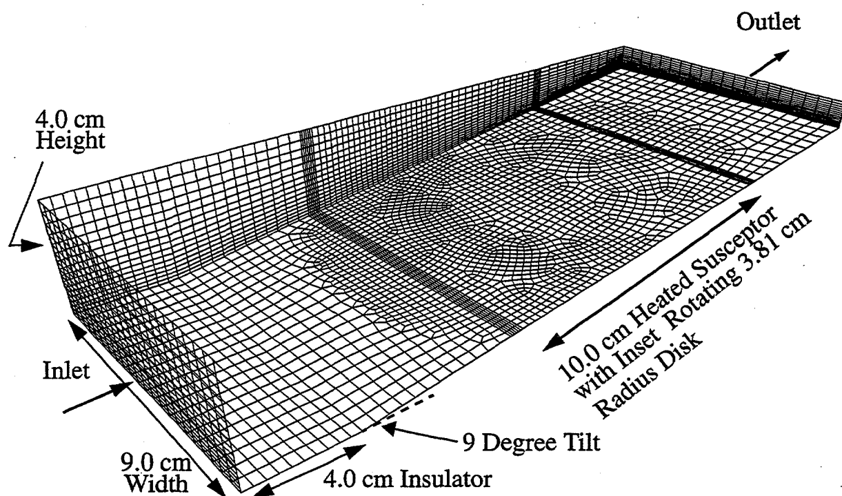
FIG 4.8. Unstructured Finite Element Mesh of CVD Reactor.
