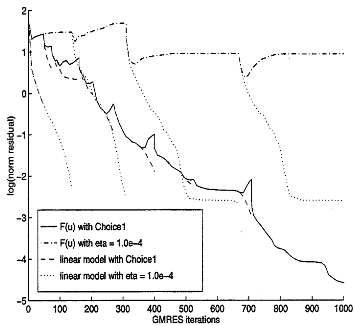
FIG. 4.6. Convergence history, first 1000 GMRES iterations.
