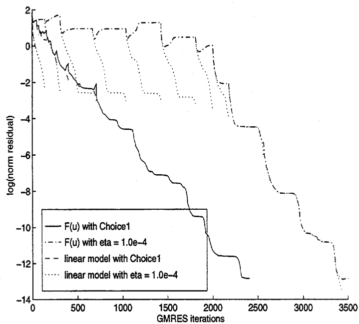
FIG. 4.7. Entire Convergence history.
