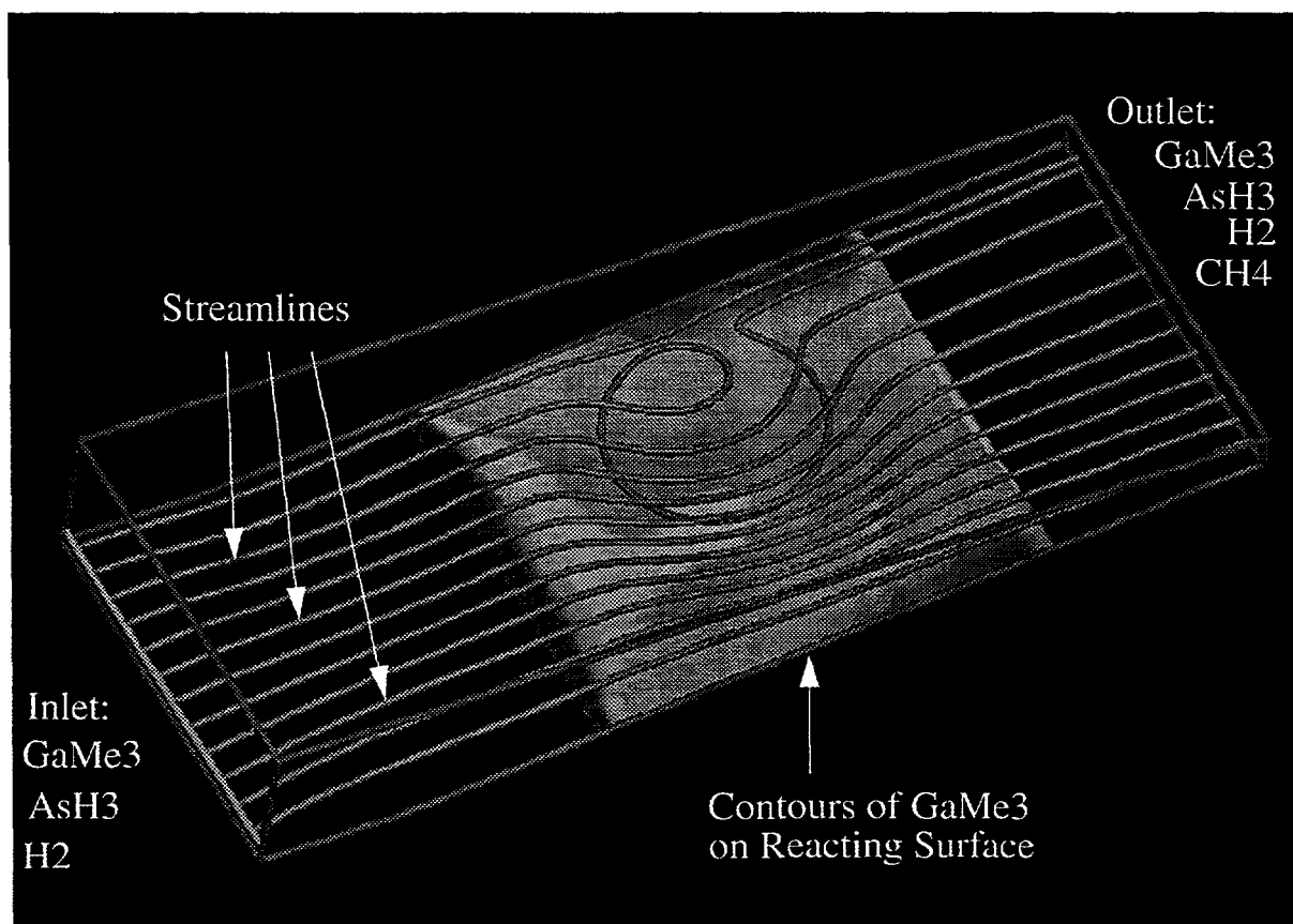
FIG 4.9. Flow Streamlines and Contour Plot of GaMe 3 Mass Fraction in CVD Reactor.
