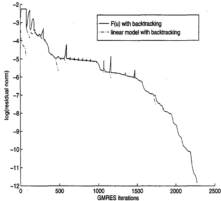
FIG. 4.5. Entire convergence history
