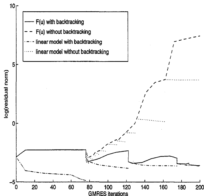
FIG. 4.4. Convergence history, first 200 GMRES iterations.
