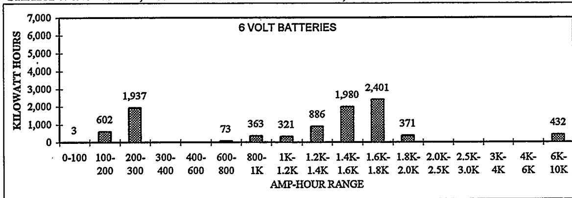
CHART 2-14. VRLA, kWh BY AMP-HOUR RANGE; 6-Vdc BATTERIES
