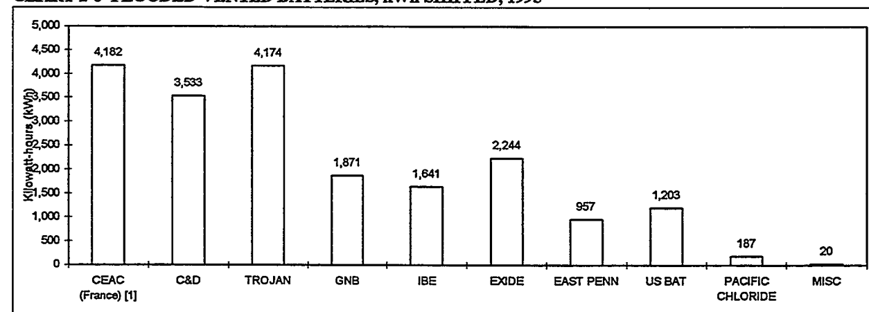
CHART 2-8 FLOODED-VENTED BATTERIES, kWh SHIPPED, 1995
