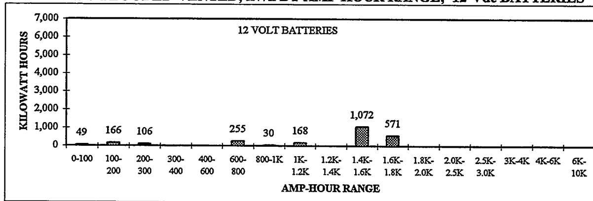
CHART 2-18. FLOODED-VENTED, kWh BY AMP-HOUR RANGE; 12-Vdc BATTERIES
