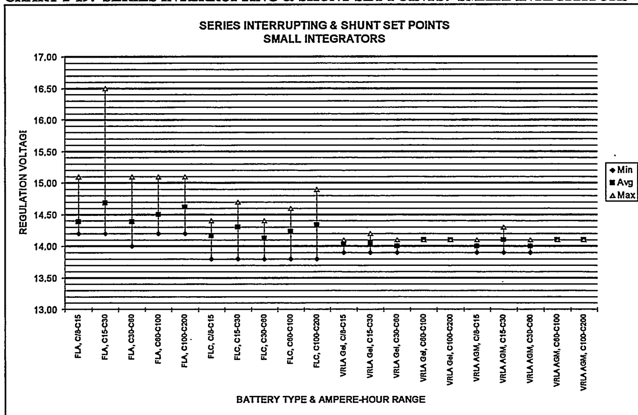
CHART 2-19. SERIES INTERRUPTING & SHUNT SET POINTS: SMALL INTEGRATORS
