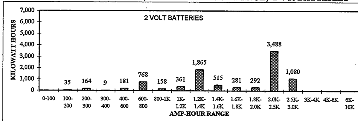
CHART 2-16. FLOODED-VENTED, kWh BY AMP-HOUR RANGE; 2-Vdc BATTERIES
