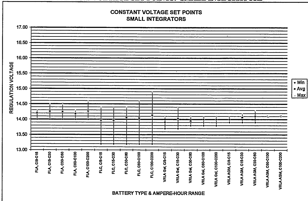
CHART 2-21. CONSTANT VOLTAGE SET POINTS: SMALL INTEGRATORS
