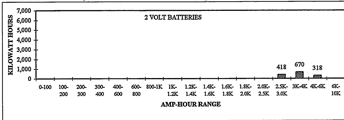
CHART 2-13. VRLA, kWh BY AMP-HOUR RANGE; 2-Vdc BATTERIES
