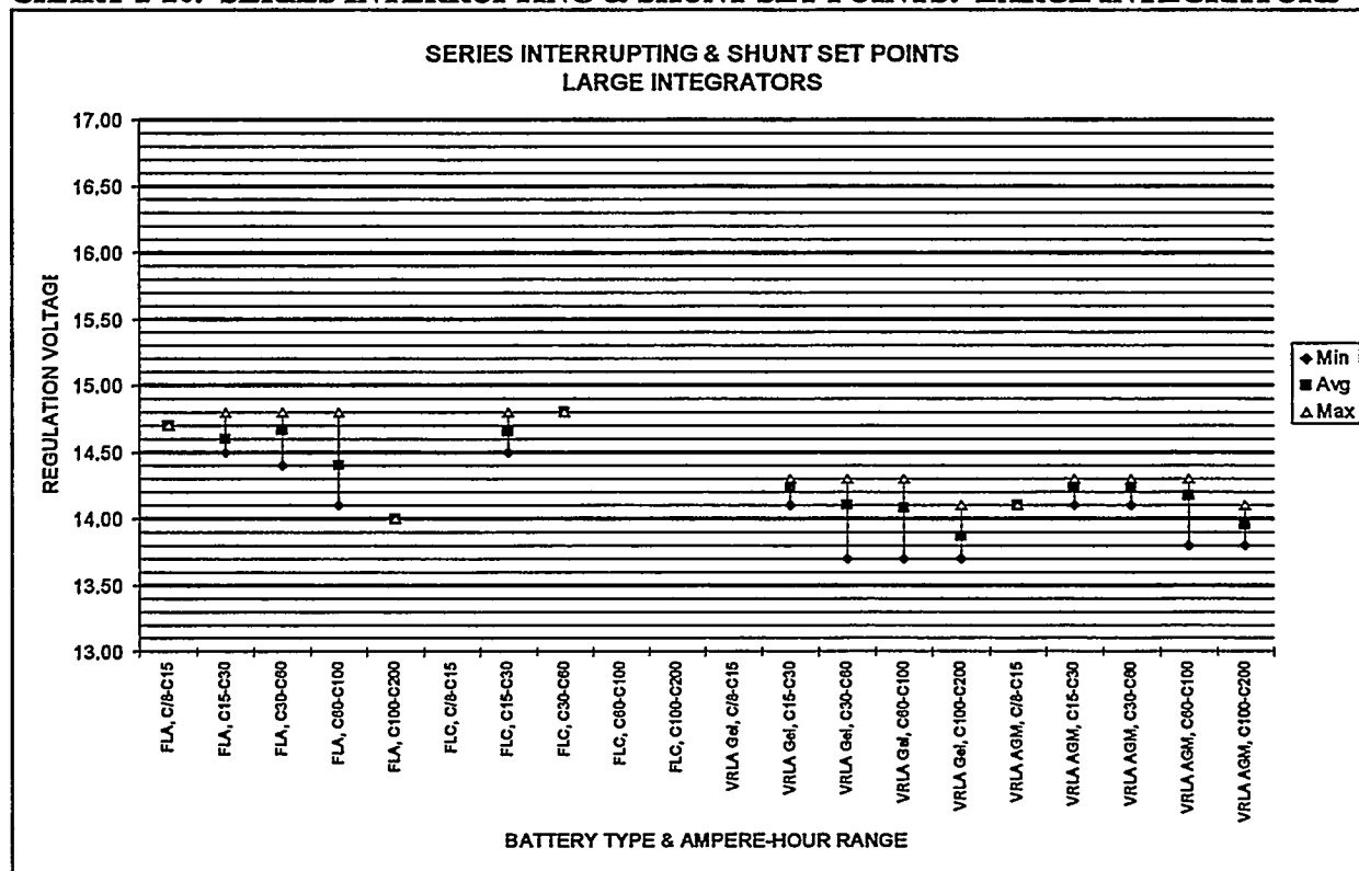
CHART 2-20. SERIES INTERRUPTING & SHUNT SET POINTS: LARGE INTEGRATORS
