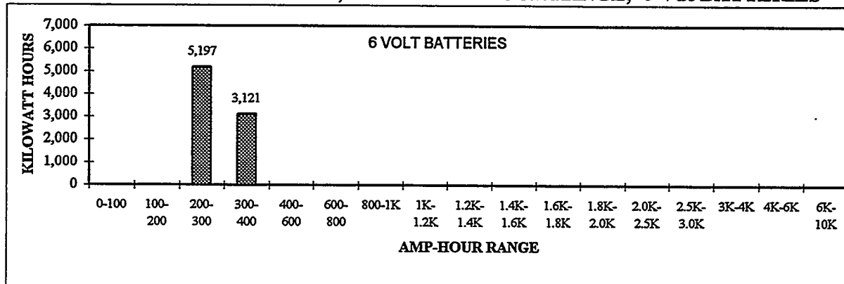
CHART 2-17. FLOODED-VENTED, kWh BY AMP-HOUR RANGE; 6-Vdc BATTERIES
