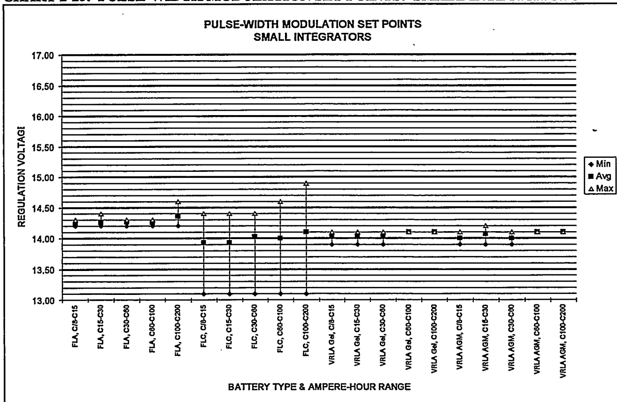
CHART 2-23. PULSE-WIDTH MODULATION SET POINTS: SMALL INTEGRATORS
