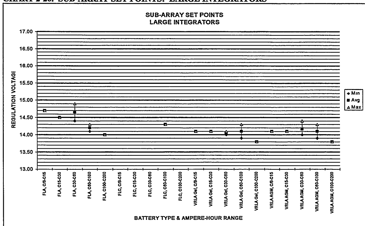
CHART 2-26. SUB-ARRAY SET POINTS: LARGE INTEGRATORS
