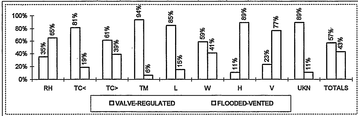
CHART 2-12. TOTALS (100%) BY APPLICATION; kWh (IN %)
