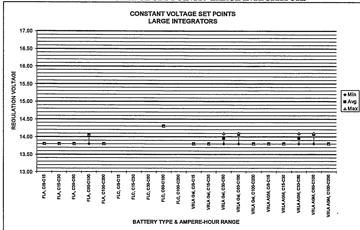
CHART 2-21. CONSTANT VOLTAGE SET POINTS: LARGE INTEGRATORS
